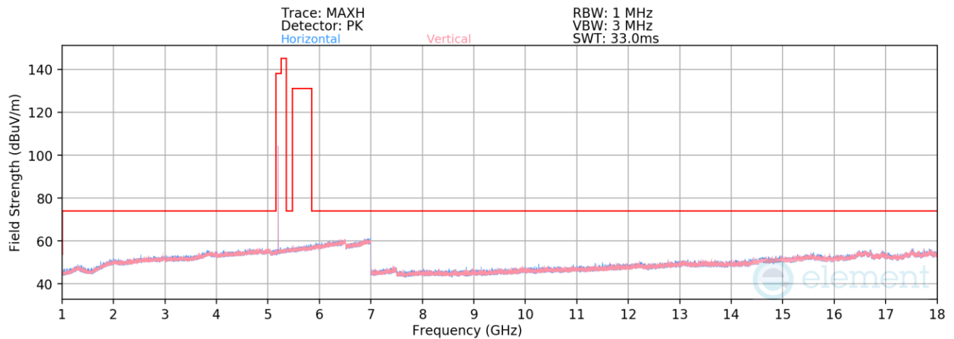
Plot 7-87. Radiated Spurious Emissions 1-18GHz (NB UNII HDRp4 – 5201MHz)
