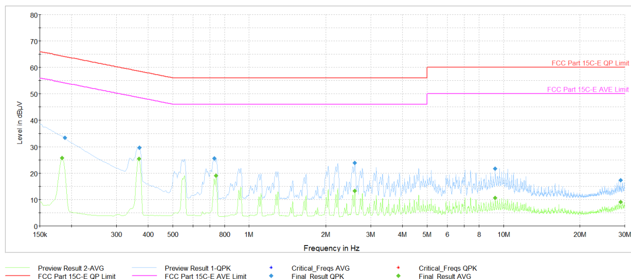
Plot 7-128. AC Line Conducted Plot (NB UNII LE2M – 5201MHz) (L1) with Laptop and USB-C Cable
