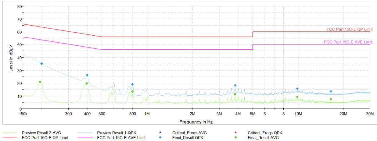
Plot 7-127. AC Line Conducted Plot (NB UNII BDR – 5157MHz) (N) with Laptop and USB-C Cable
