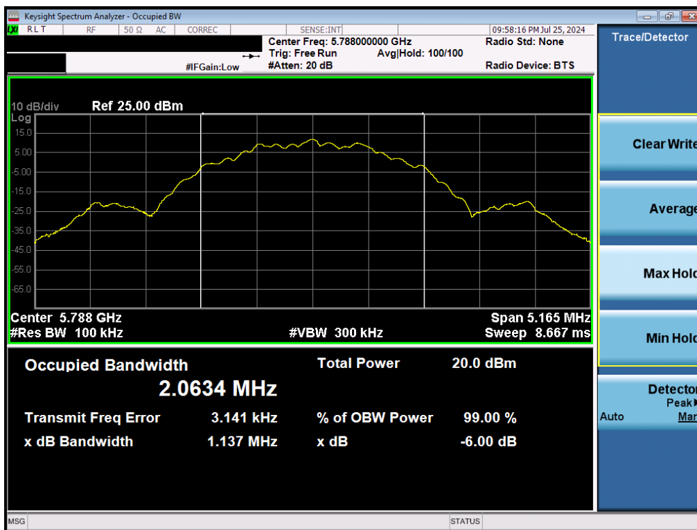
Plot 7-23. 6dB BW & 99% OBW (NB UNII LE2M – 5788MHz)
