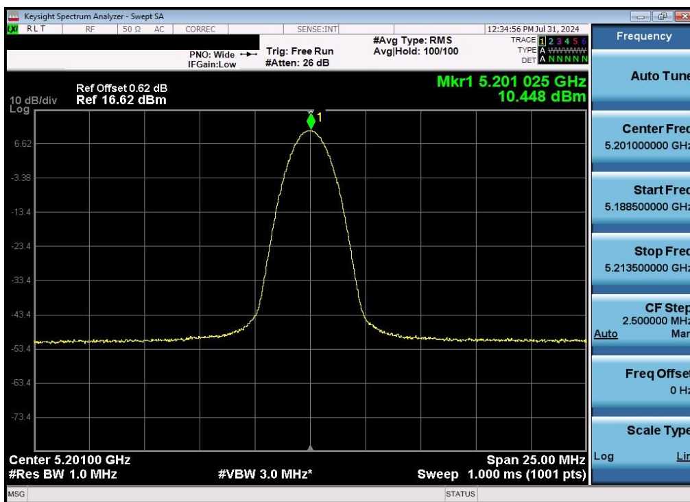
Plot 7-41. FCC PSD (NB UNII LE2M – 5201MHz)
