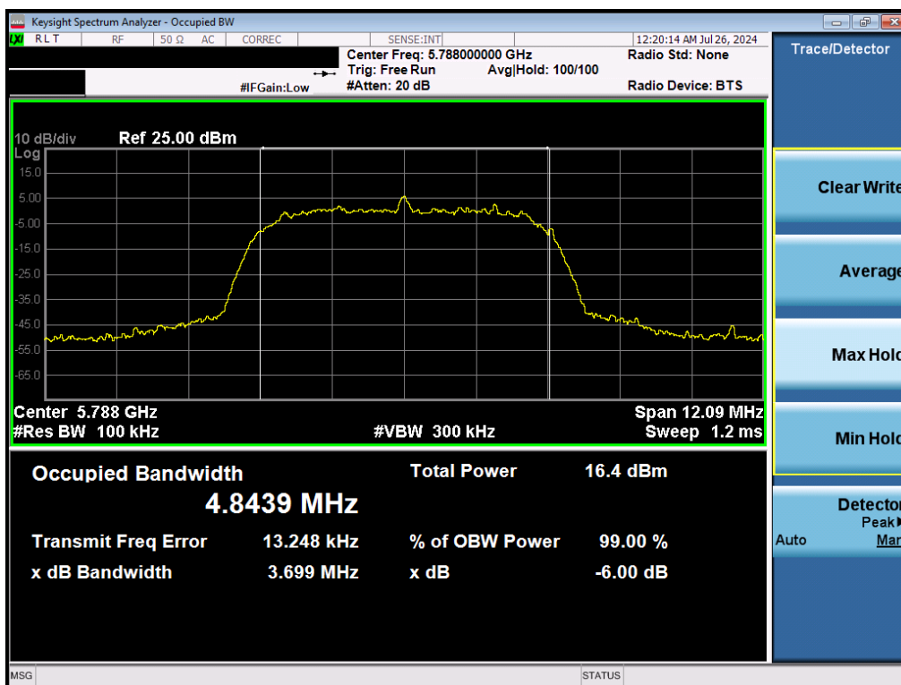
Plot 7-35. 6dB BW & 99% OBW (NB UNII HDRp8 – 5788MHz)
