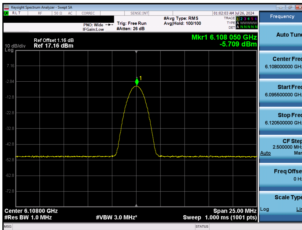
Plot 7-19. PSD (NB UNII BDR – 6108MHz)
