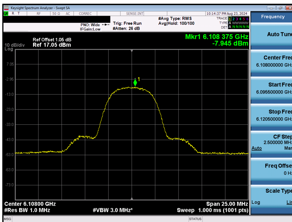
Plot 7-28. PSD (NB UNII HDR8 – 6108MHz)
