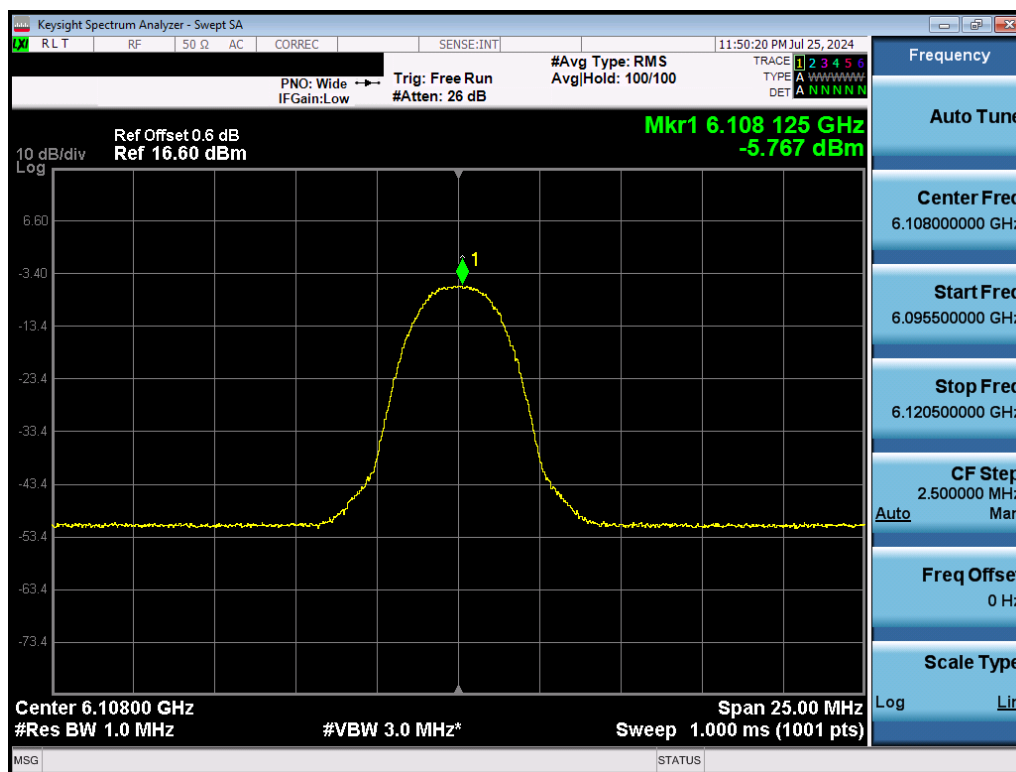
Plot 7-31. PSD (NB UNII HDRp4 – 6108MHz)
