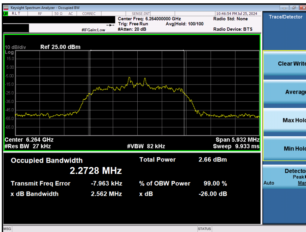
Plot 7-8. 26dB BW & 99% OBW (NB UNII HDR4 – 6264MHz)
