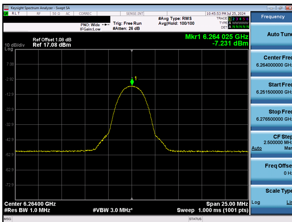
Plot 7-26. PSD (NB UNII HDR4 – 6264MHz)
