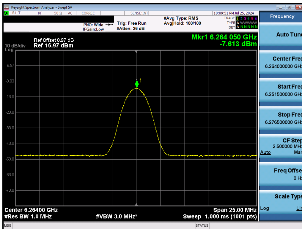
Plot 7-23. PSD (NB UNII LE, 2Mbps – 6264MHz)
