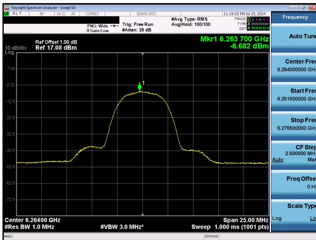
Plot 7-29. PSD (NB UNII HDR8 – 6264MHz)
