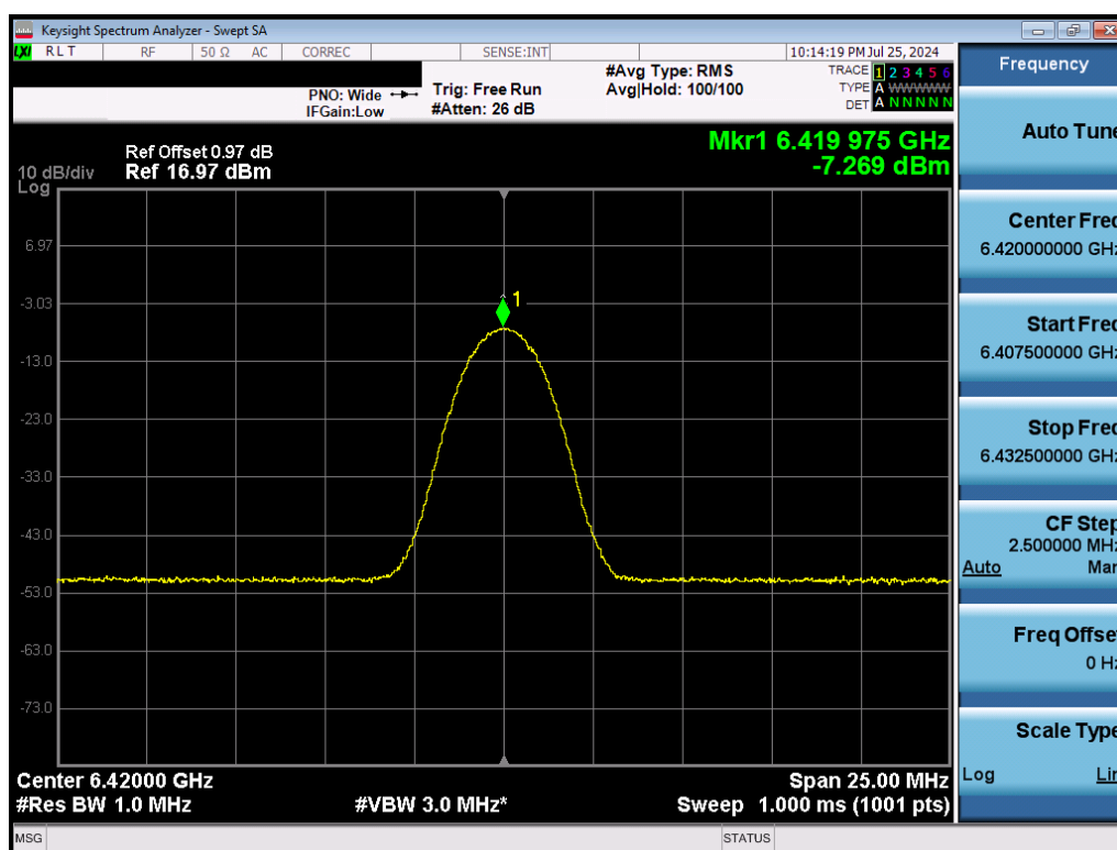
Plot 7-24. PSD (NB UNII LE, 2Mbps – 6420MHz)
