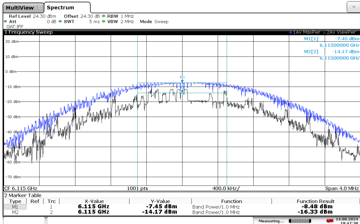
Plot 7-59. Power Density Plot (NB UNII, 6115MHz)
