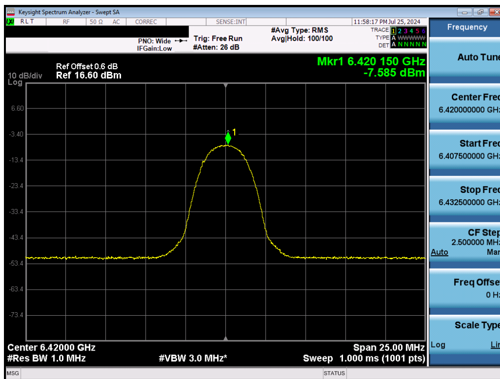
Plot 7-33. PSD (NB UNII HDRp4 – 6420MHz)
