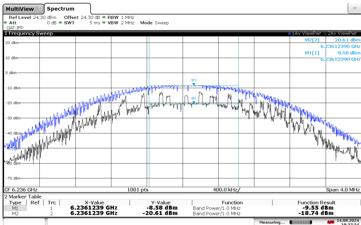
Plot 7-60. Power Density Plot (NB UNII, 6236MHz)
