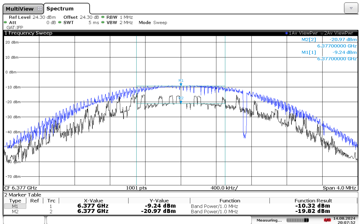
Plot 7-61. Power Density Plot (NB UNII, 6377MHz)
