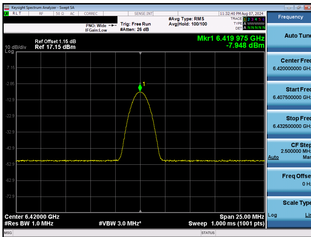
Plot 7-21. PSD (NB UNII BDR – 6420MHz)
