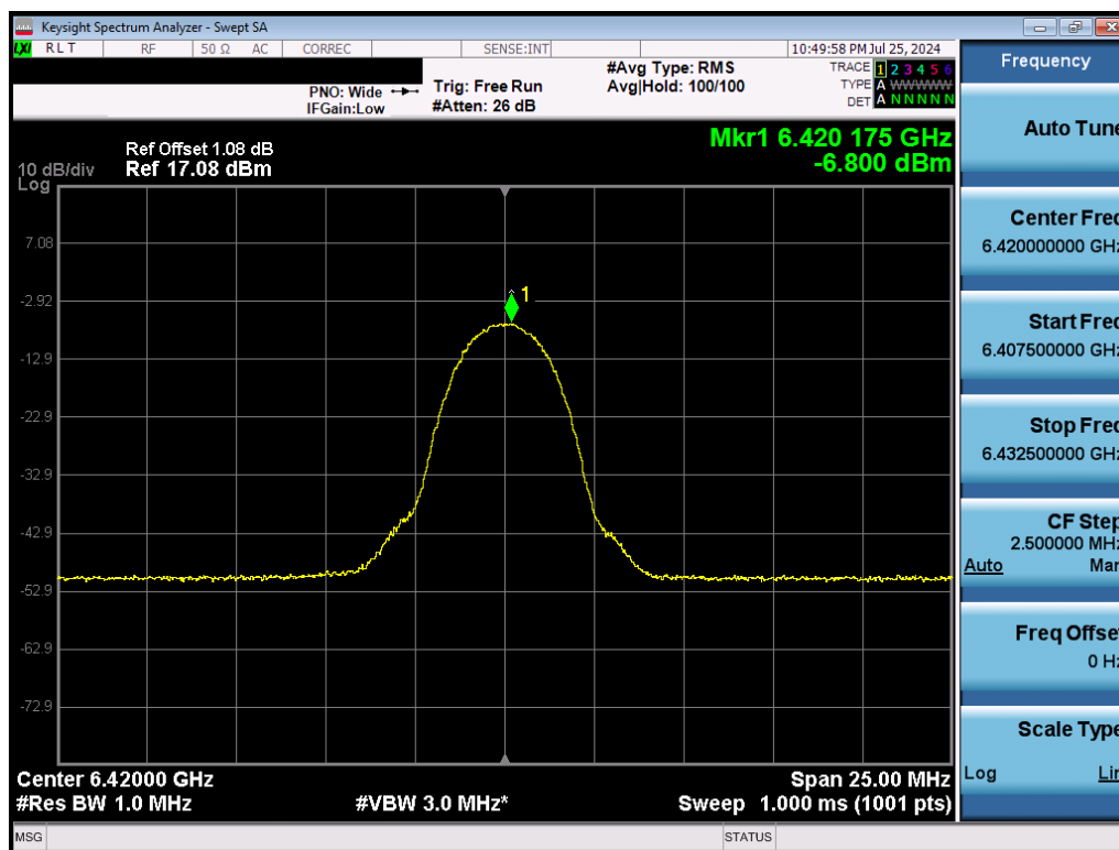
Plot 7-27. PSD (NB UNII HDR4 – 6420MHz)
