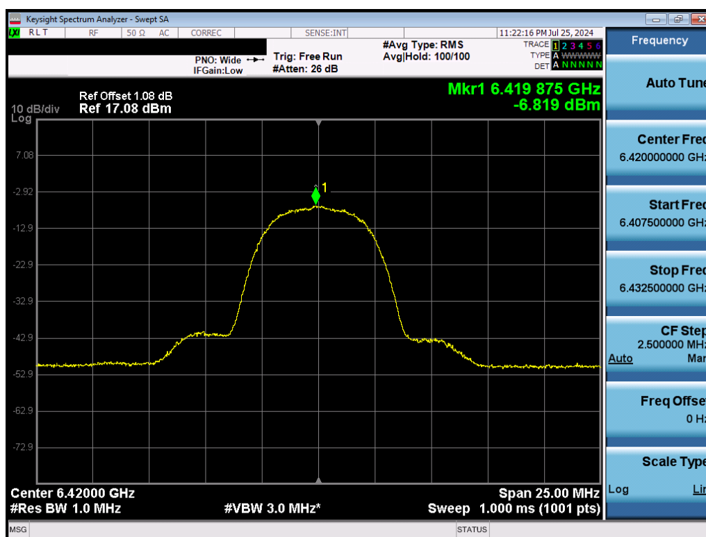
Plot 7-30. PSD (NB UNII HDR8 – 6420MHz)
