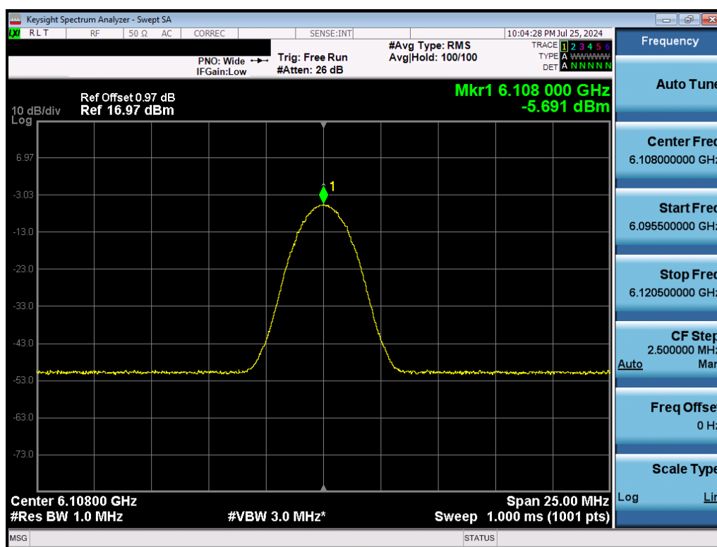
Plot 7-22. PSD (NB UNII LE, 2Mbps – 6108MHz)
