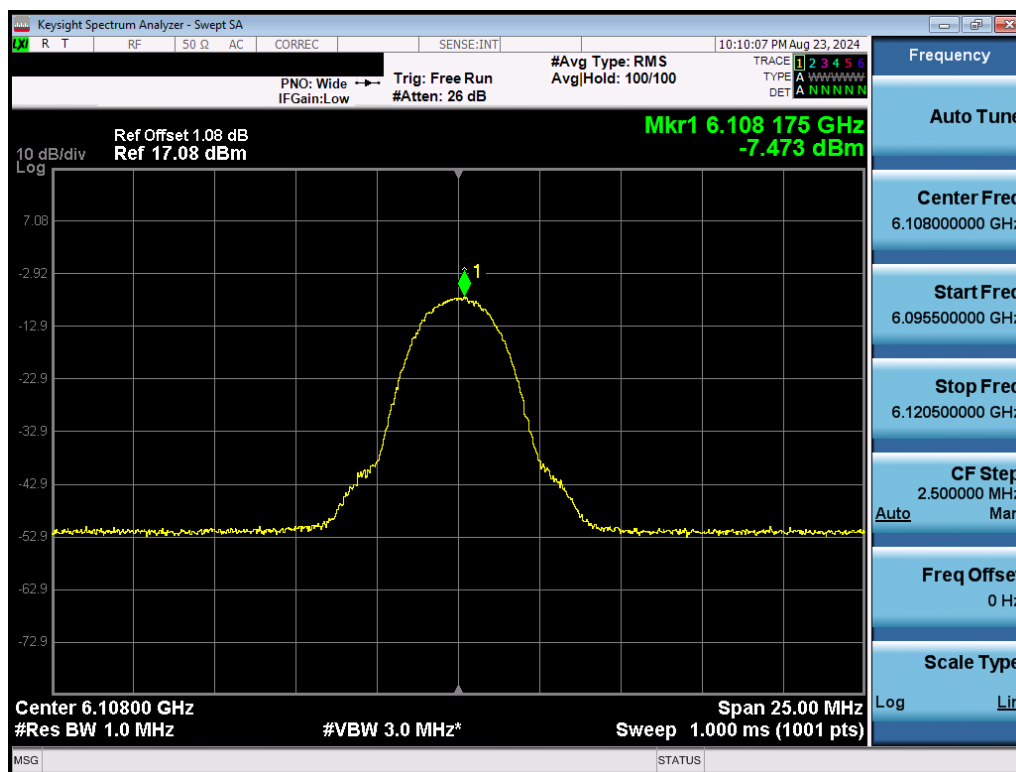
Plot 7-25. PSD (NB UNII HDR4 – 6108MHz)
