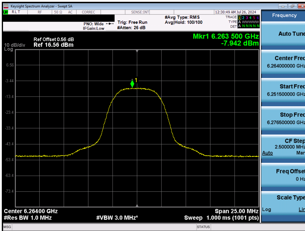
Plot 7-35. PSD (NB UNII HDRp8 - 6264MHz)
