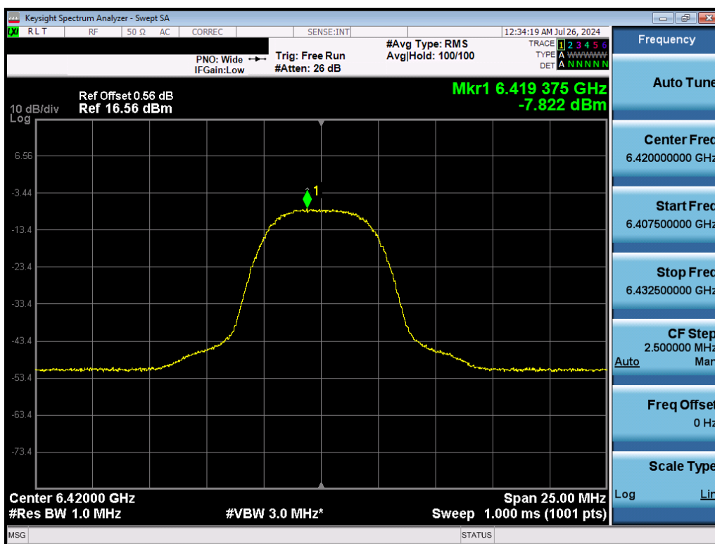
Plot 7-36. PSD (NB UNII HDRp8 - 6420MHz)
