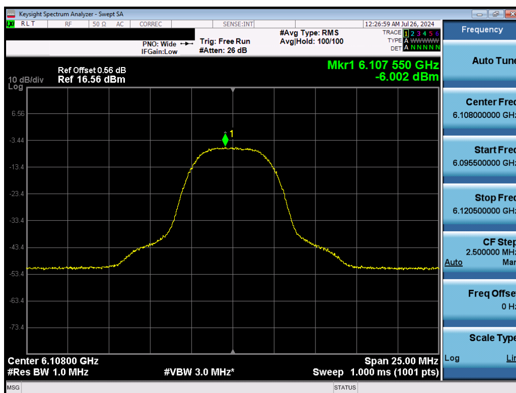
Plot 7-34. PSD (NB UNII HDRp8 – 6108MHz)
