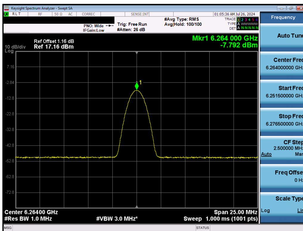
Plot 7-20. PSD (NB UNII BDR – 6264MHz)
