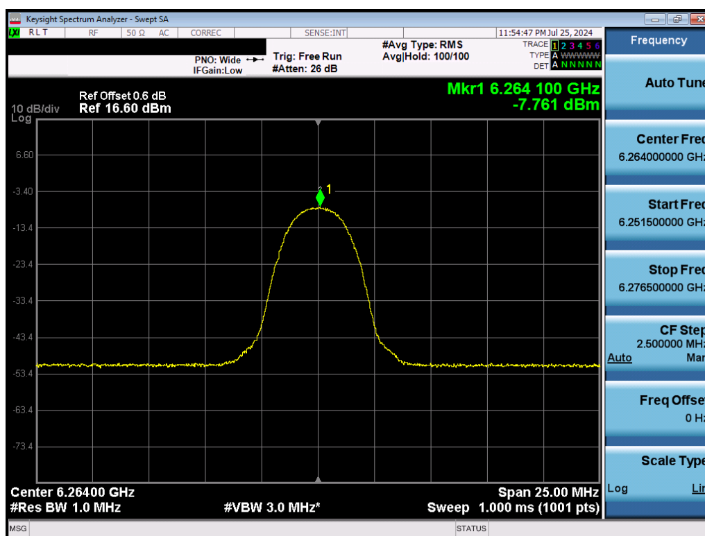
Plot 7-32. PSD (NB UNII HDRp4 – 6264MHz)
