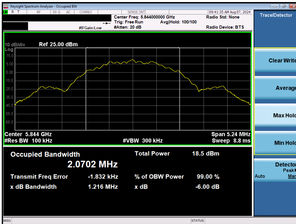
Plot 7-24. 6dB BW & 99% OBW (NB UNII LE2M – 5844MHz)
