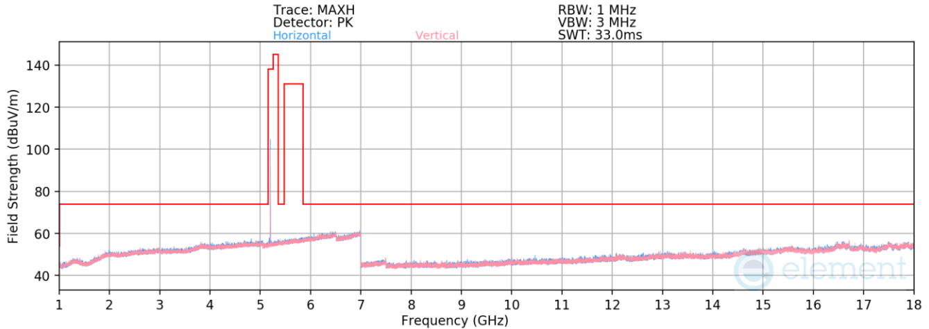
Plot 7-78. Radiated Spurious Emissions 1-18GHz (NB UNII LE2M – 5201MHz)
