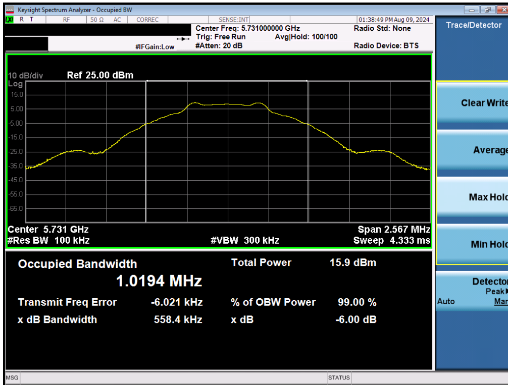
Plot 7-19. 6dB BW & 99% OBW (NB UNII BDR – 5731MHz)
