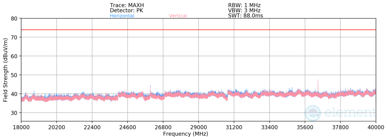
Plot 7-79. Radiated Spurious Emission 18-40GHz (NB UNII LE2M – 5201MHz)
