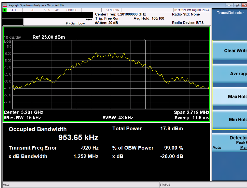
Plot 7-2. 26dB BW & 99% OBW (NB UNII BDR – 5201MHz)
