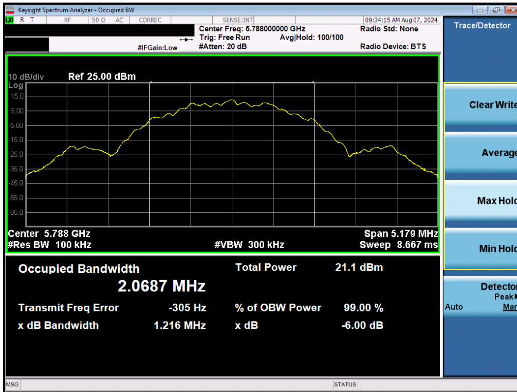
Plot 7-23. 6dB BW & 99% OBW (NB UNII LE2M – 5788MHz)
