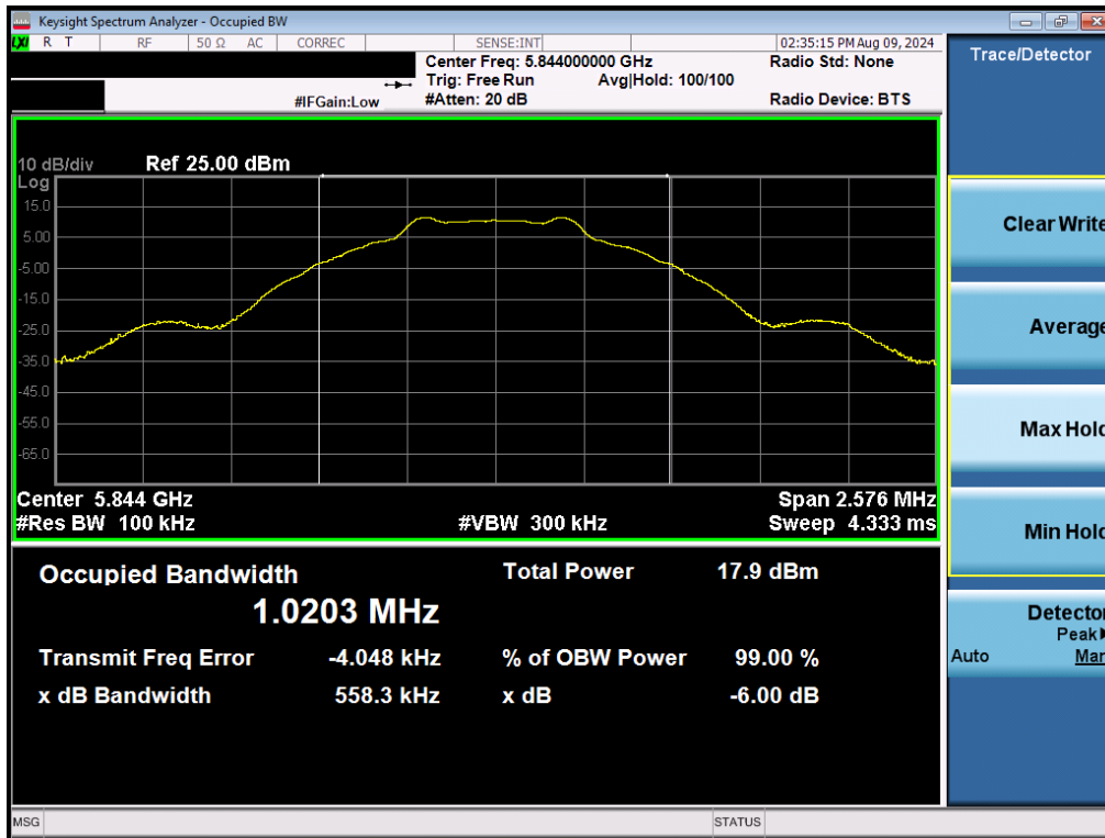
Plot 7-21. 6dB BW & 99% OBW (NB UNII BDR – 5844MHz)
