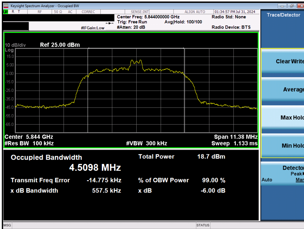
Plot 7-30. 6dB BW & 99% OBW (NB UNII HDR8 – 5844MHz)
