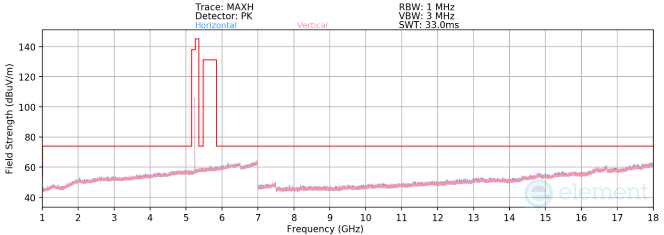
Plot 7-83. Radiated Spurious Emissions 1-18GHz (NB UNII HDR4 – 5245MHz)
