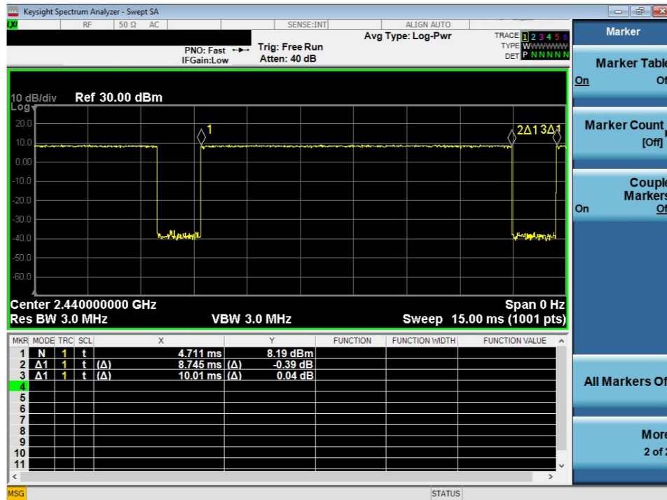
Figure 7-2 2.4 GHz Bluetooth Transmission Plot - Variant 2
