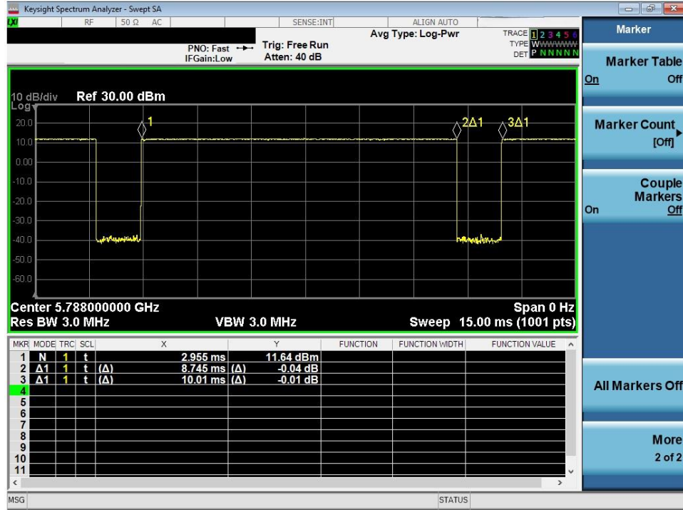
Figure 7-6 NB UNII-3 Transmission Plot - Variant 2
