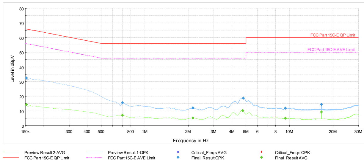
Plot 7-52. AC Line Conducted Plot with Bluetooth HDR (L1, 4Mbps - Ch.73 with host PC and USB-C cable)
