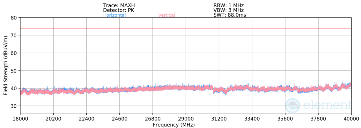
Plot 7-42. Radiated Spurious Emissions Above 18GHz (4Mbps, HDR4, – Ch. 38)
