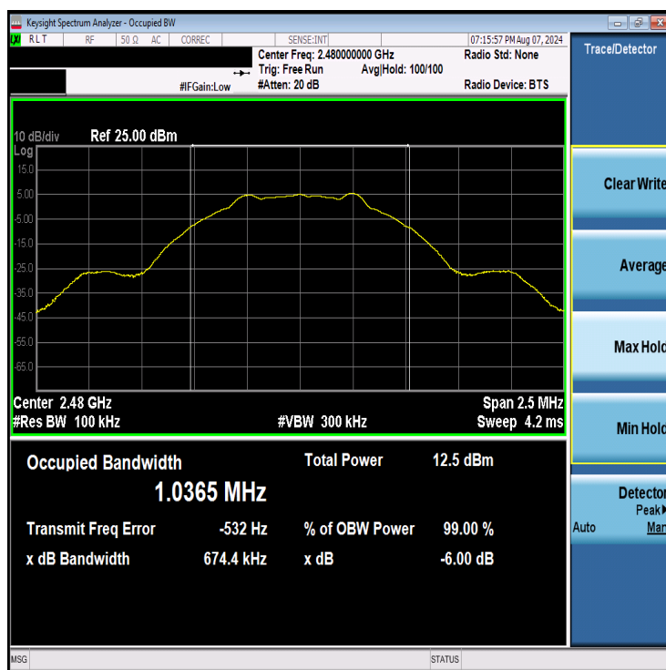
Plot 7-3. 6dB BW & 99% OBW Plot (Bluetooth (LE), 1Mbps – Ch. 39)
