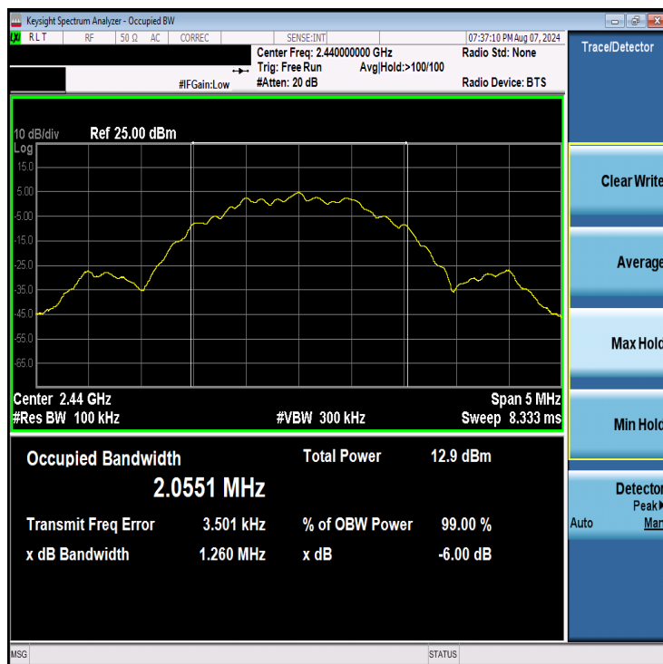
Plot 7-5. 6dB BW & 99% OBW Plot (Bluetooth (LE), 2Mbps – Ch. 19)
