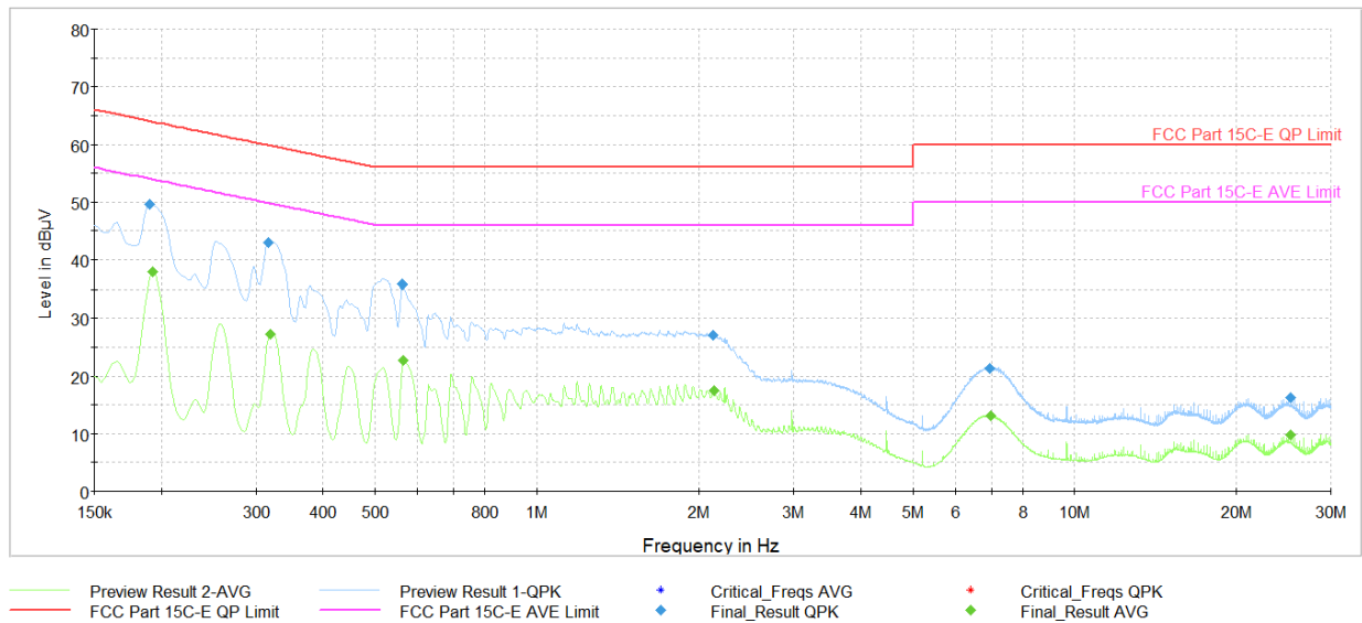
Plot 7-32. AC Line Conducted Plot with Bluetooth LE (L1, 1Mbps – Ch.39 with host PC with USB-C cable)
