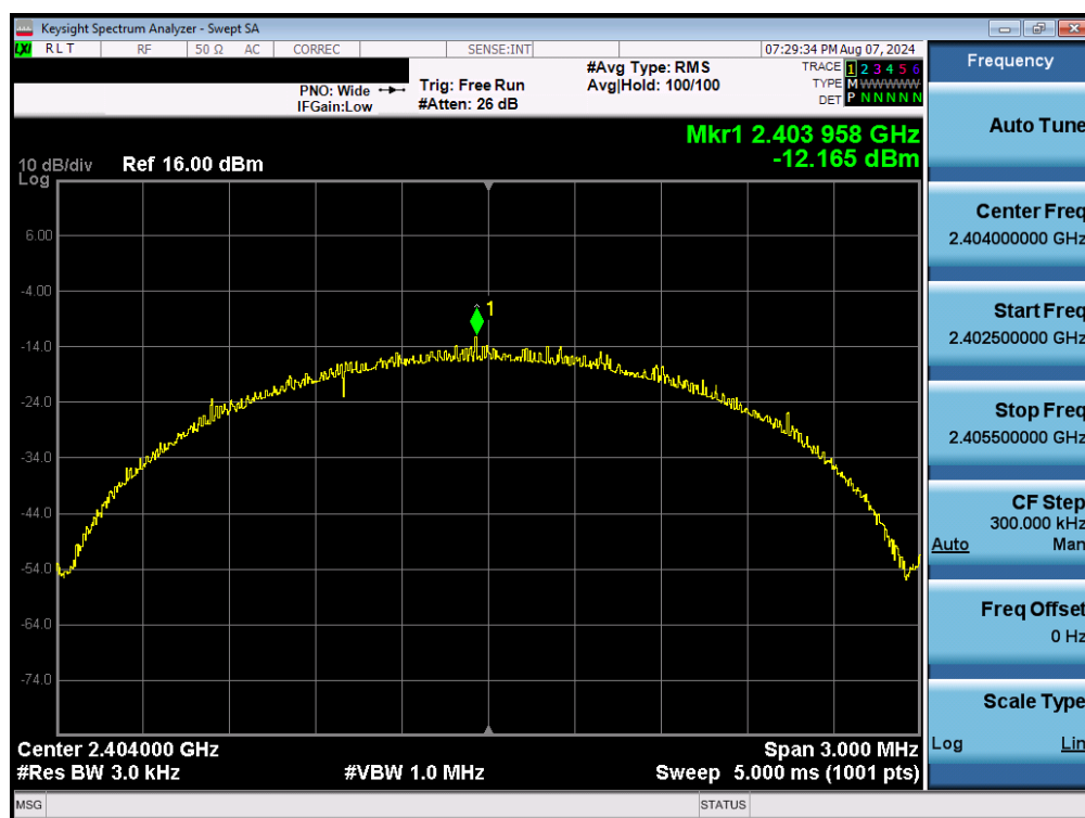
Plot 7-10. Power Spectral Density Plot (Bluetooth (LE), 2Mbps, – Ch. 1)
