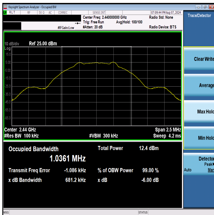
Plot 7-2. 6dB BW & 99% OBW Plot (Bluetooth (LE), 1Mbps – Ch. 19)
