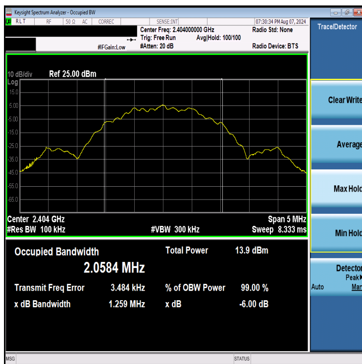
Plot 7-4. 6dB BW & 99% OBW Plot (Bluetooth (LE), 2Mbps – Ch. 1)
