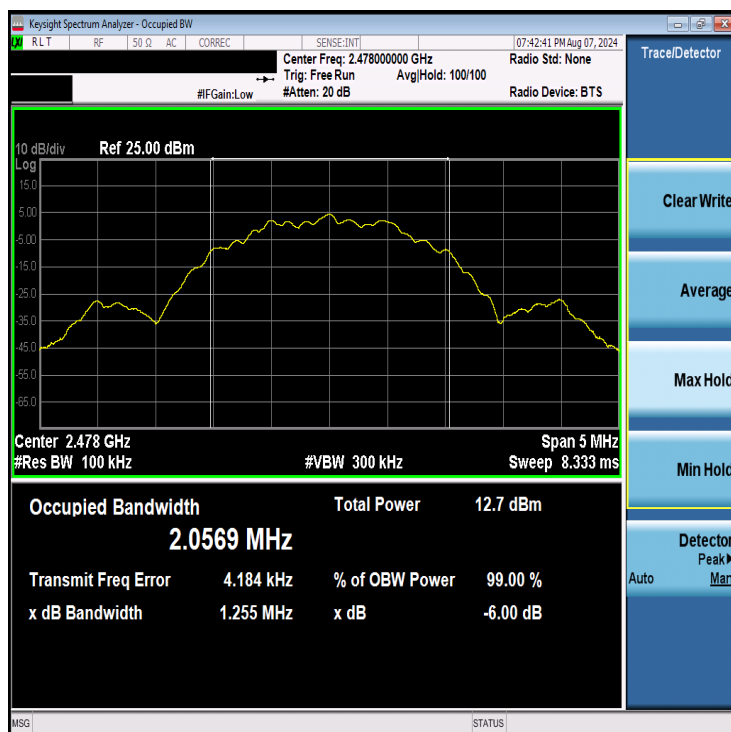
Plot 7-6. 6dB BW & 99% OBW Plot (Bluetooth (LE), 2Mbps – Ch. 38)
