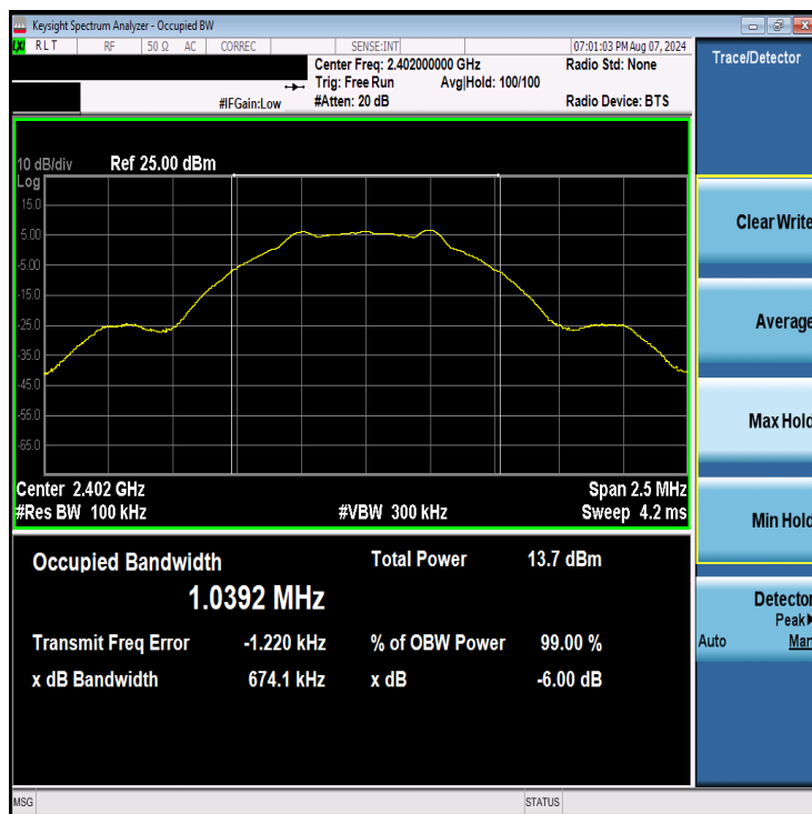
Plot 7-1. 6dB BW & 99% OBW Plot (Bluetooth (LE), 1Mbps – Ch. 0)
