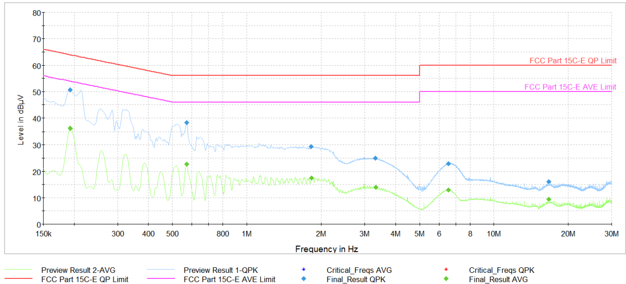
Plot 7-33. AC Line Conducted Plot with Bluetooth LE (N, 1Mbps – Ch.39, with host PC with USB-C cable)
