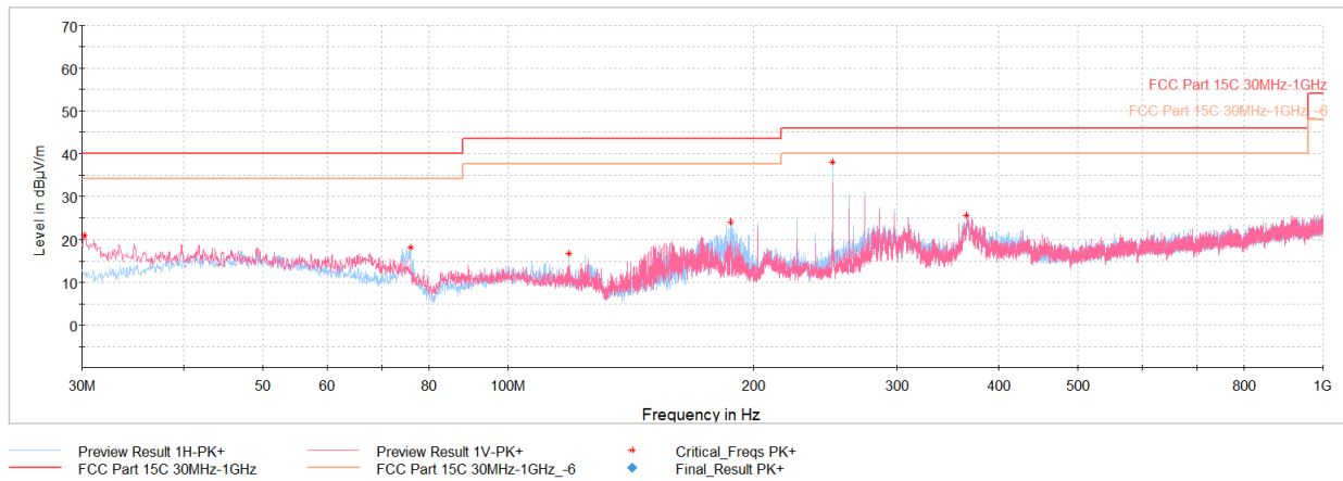
Plot 7-31. Radiated Spurious Emissions Below 1GHz (1Mbps – Ch.39, Pol. H & V, with host PC with USB-C cable)
