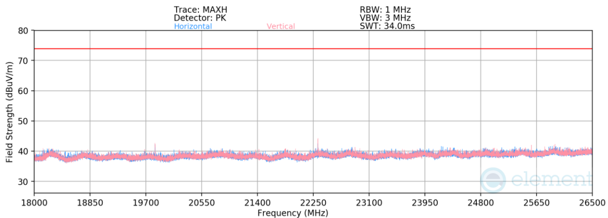
Plot 7-32. Radiated Spurious Emissions above 18GHz (GFSK – Ch.78)
