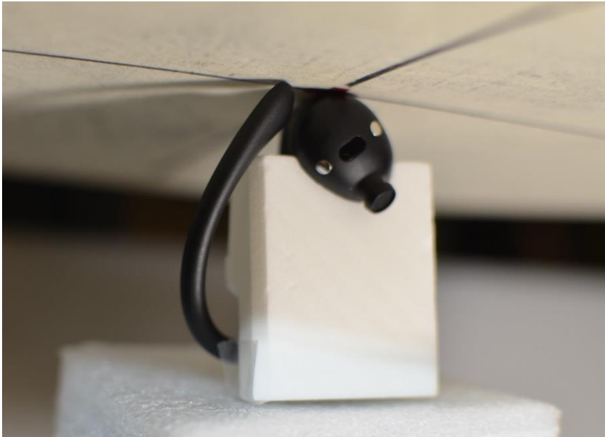
SAR Test Setup Photo 5: Body-Worn, Bottom position, Right Earbud, 0 mm
