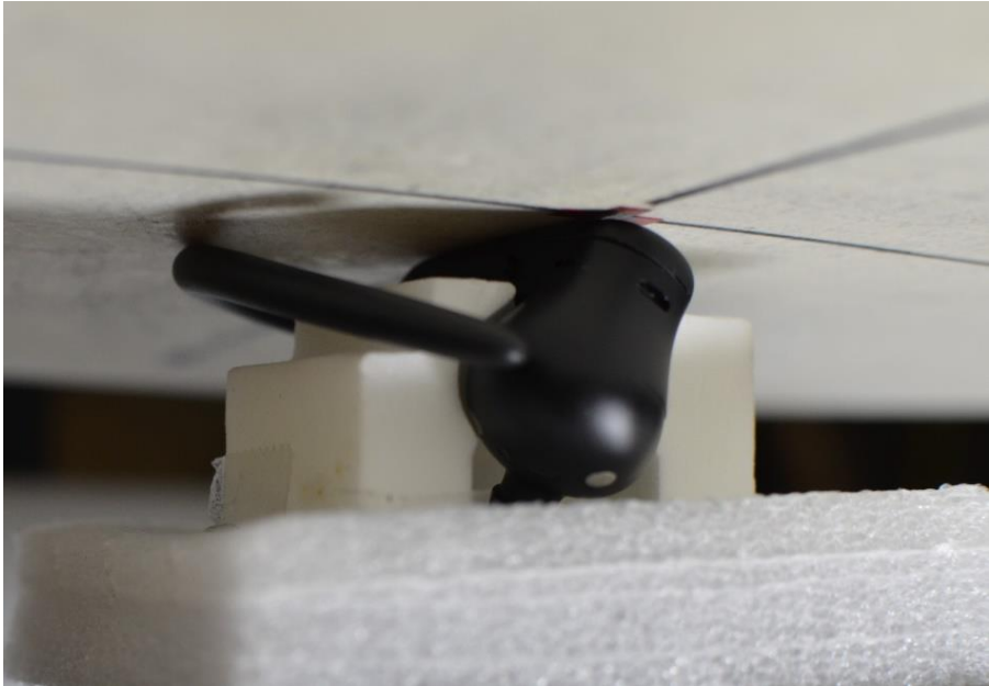
SAR Test Setup Photo 3: Body-Worn, Button position, Right Earbud, 0 mm
