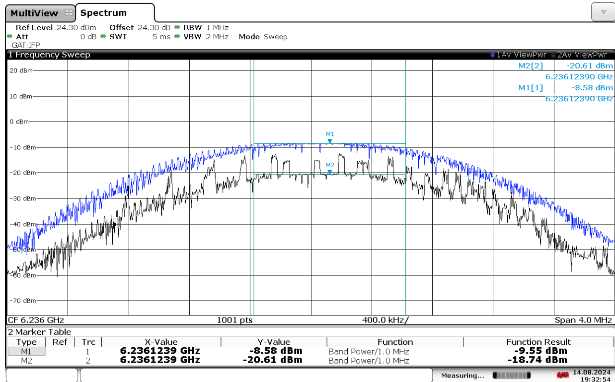
Plot 7-60. Power Spectral Density Plot (NB UNII BDR, 6236MHz)
