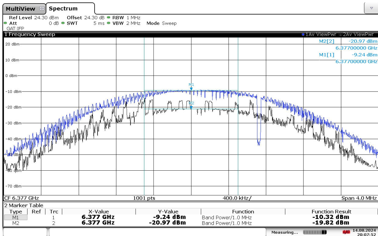
Plot 7-61. Power Spectral Density Plot (NB UNII BDR, 6377MHz)
