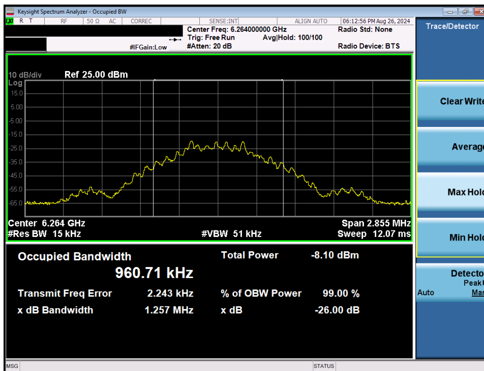
Plot 7-2. 26dB BW & 99% OBW (NB UNII BDR – 6264MHz)
