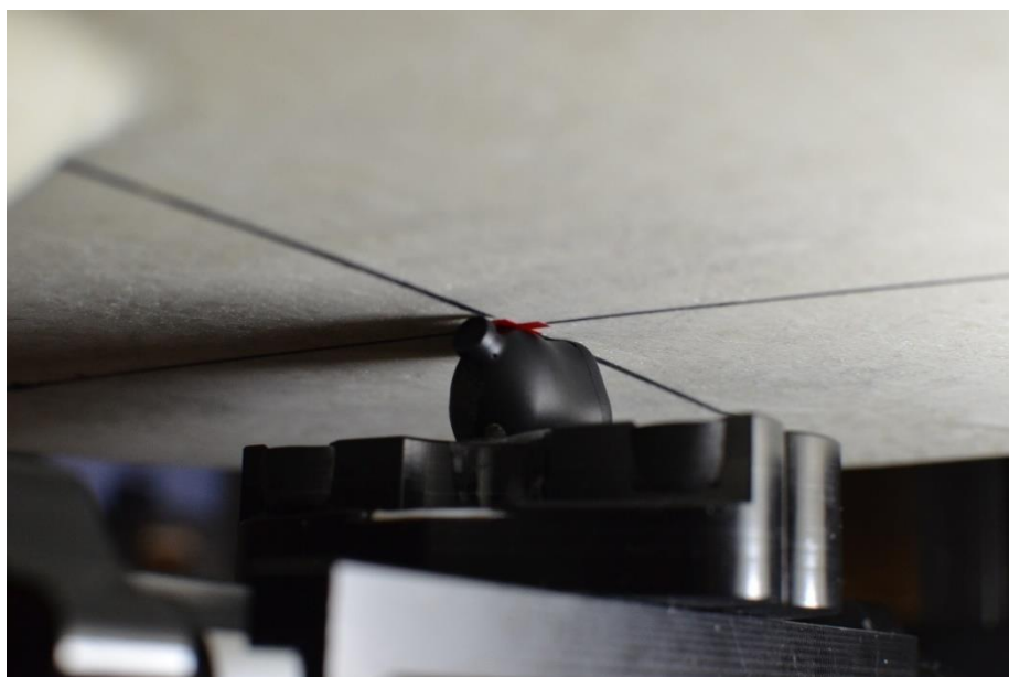
SAR Test Setup Photo 2: Head, Right Earbud, 3 Point, 0 mm
