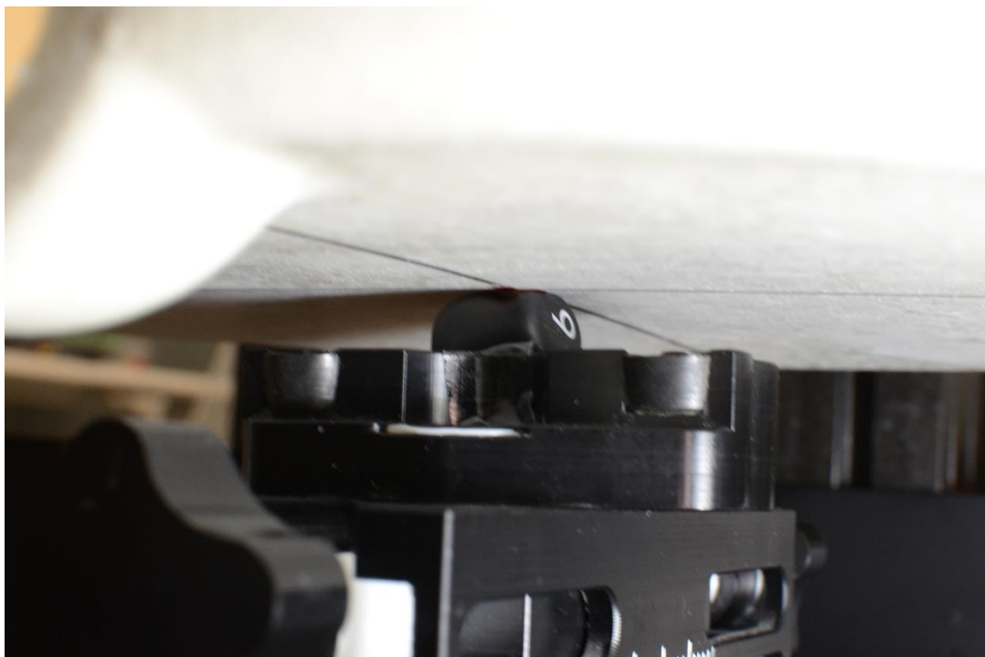
SAR Test Setup Photo 5: Body-Worn, Right Earbud, S2, 0 mm
