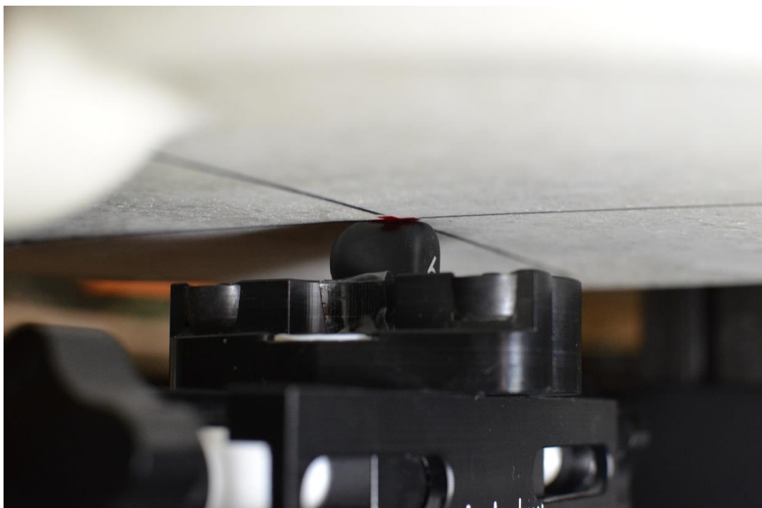
SAR Test Setup Photo 6: Body-Worn, Right Earbud, S3, 0 mm
