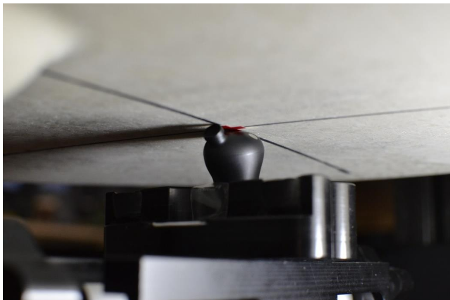
SAR Test Setup Photo 1: Head, Right Earbud, 2 Point, 0 mm
