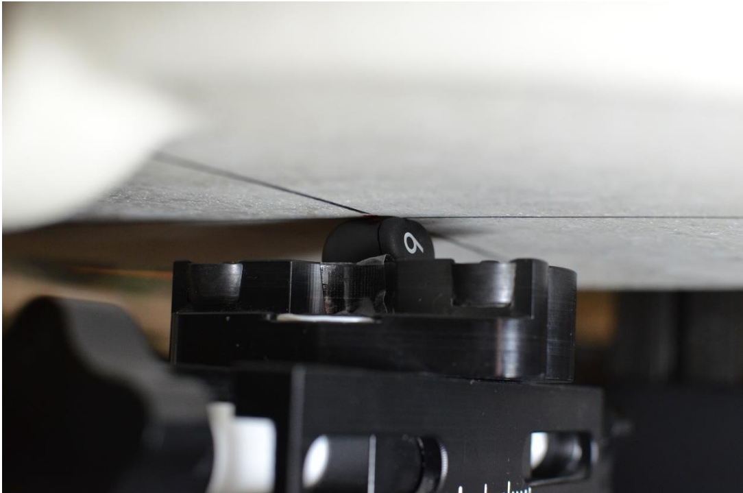
SAR Test Setup Photo 7: Body-Worn, Right Earbud, S4, 0 mm
