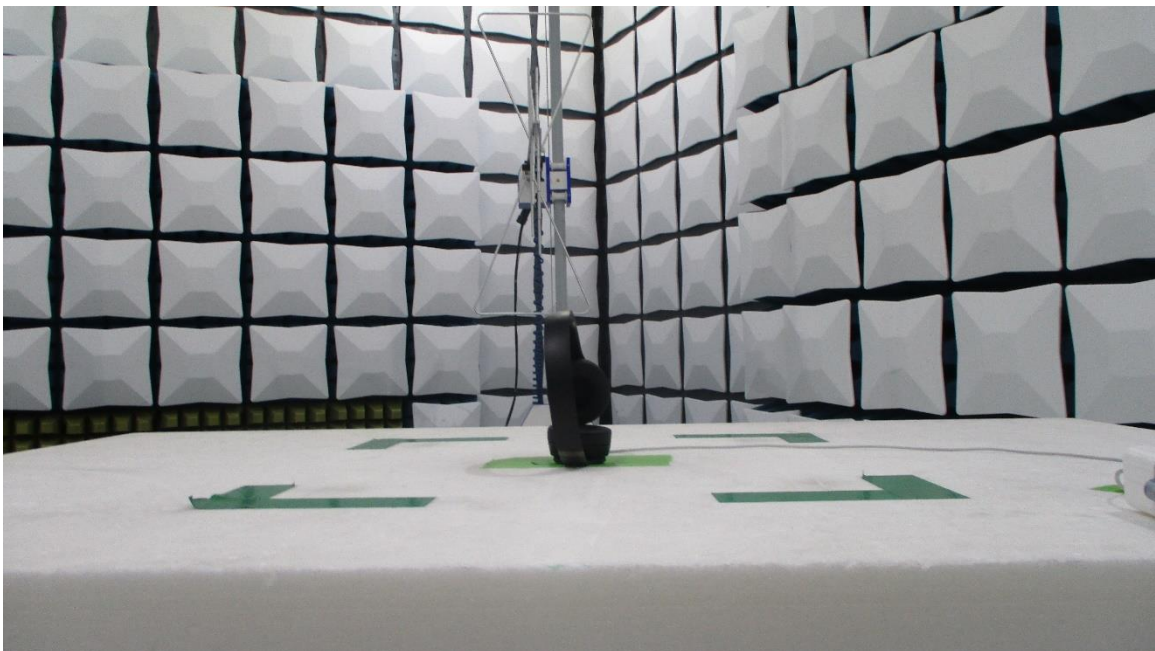
Figure 12: 30MHz-1GHz Test Setup (Rear View)
