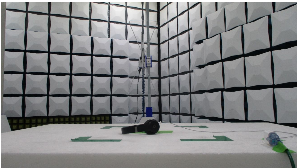
Figure 14: 30MHz-1GHz Test Setup (Rear View)
