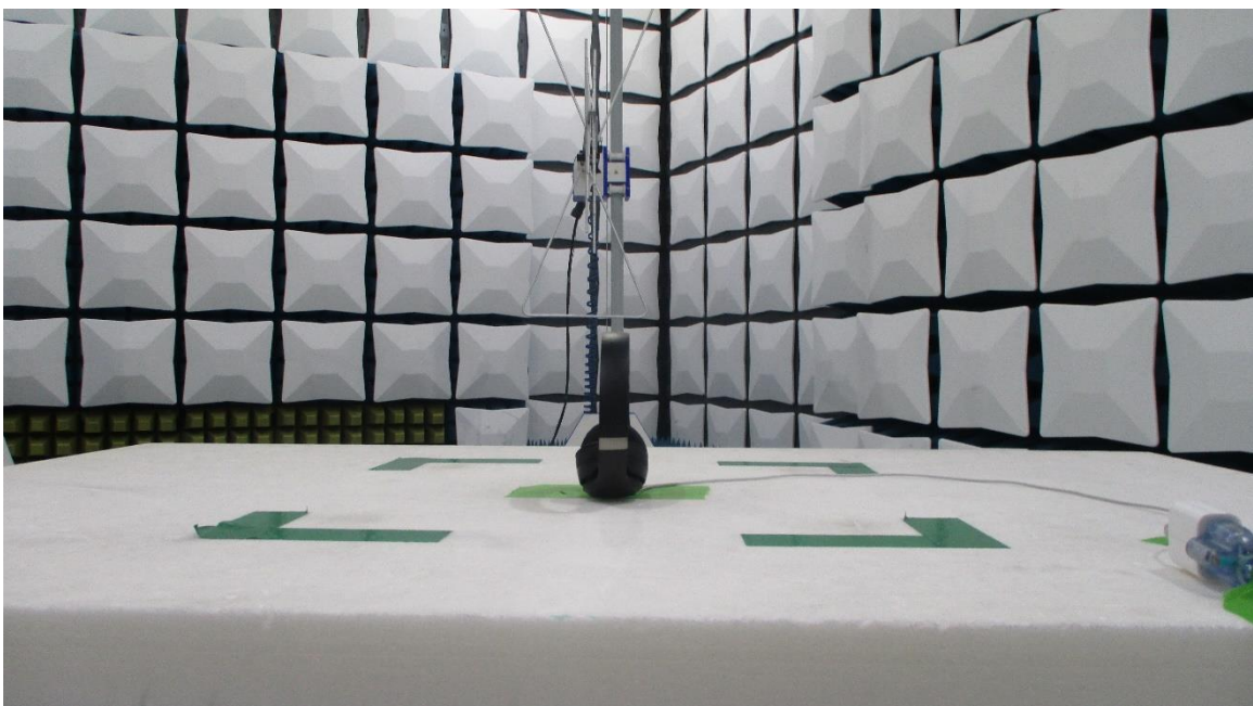
Figure 16: 30MHz-1GHz Test Setup (Rear View)
