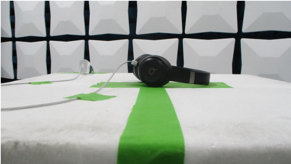
Figure 7: 1-18GHz Test Setup (Front View)
