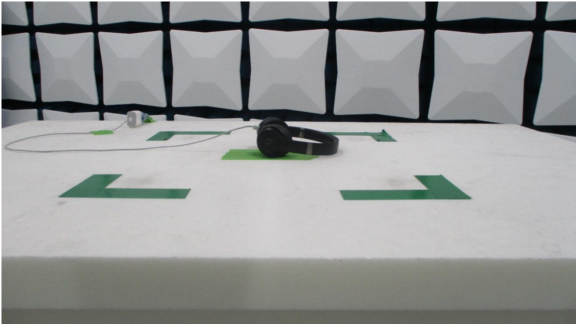
Figure 13: 30MHz-1GHz Test Setup (Front View)
