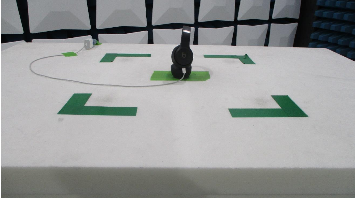
Figure 11: 30MHz-1GHz Test Setup (Front View)
