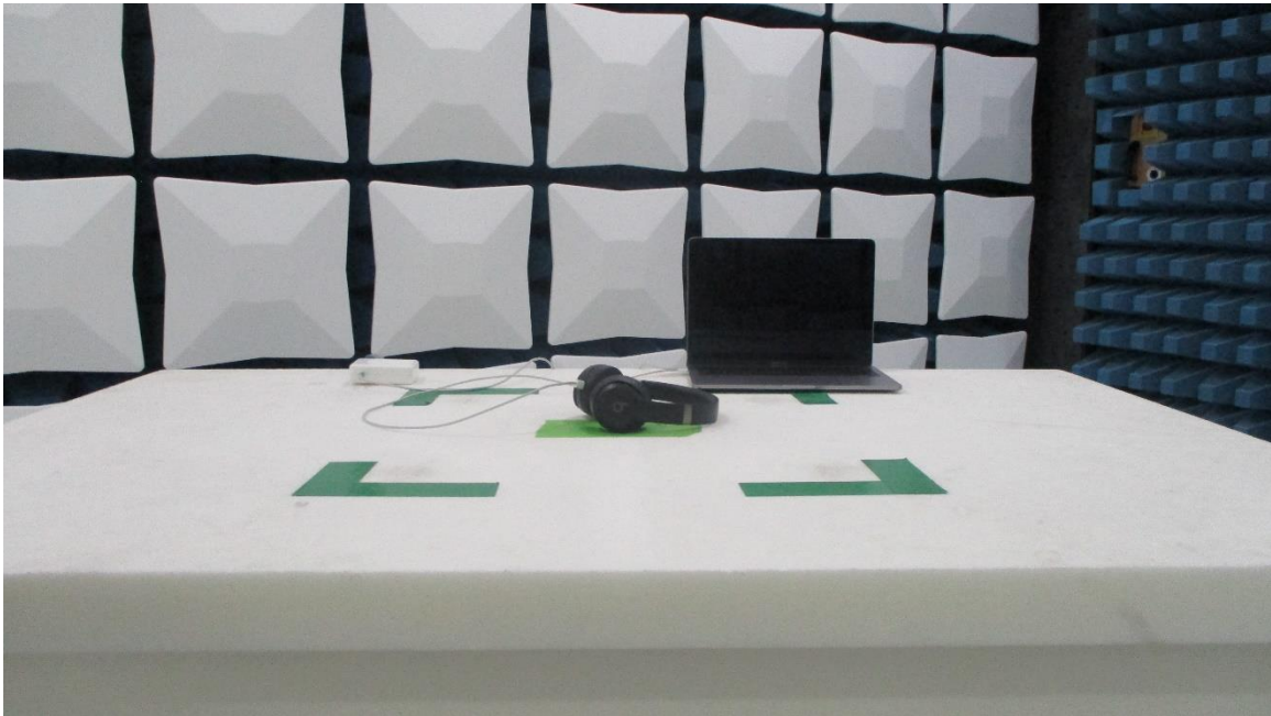
Figure 19: 30MHz-1GHz Test Setup (Front View)
