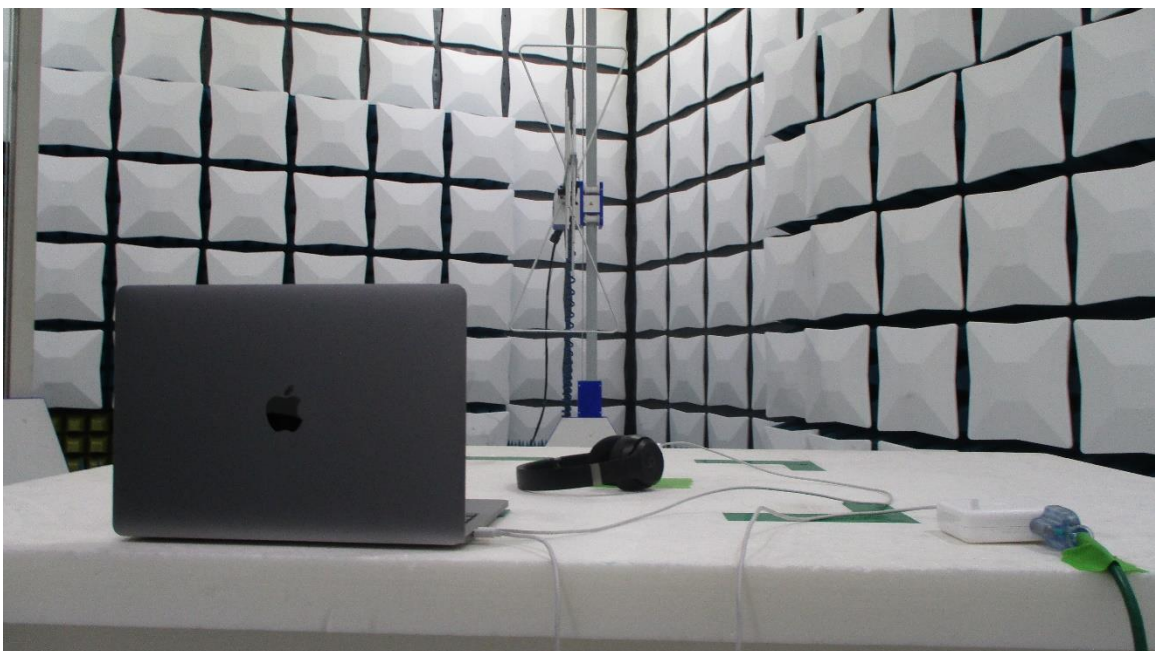
Figure 20: 30MHz-1GHz Test Setup (Rear View)
