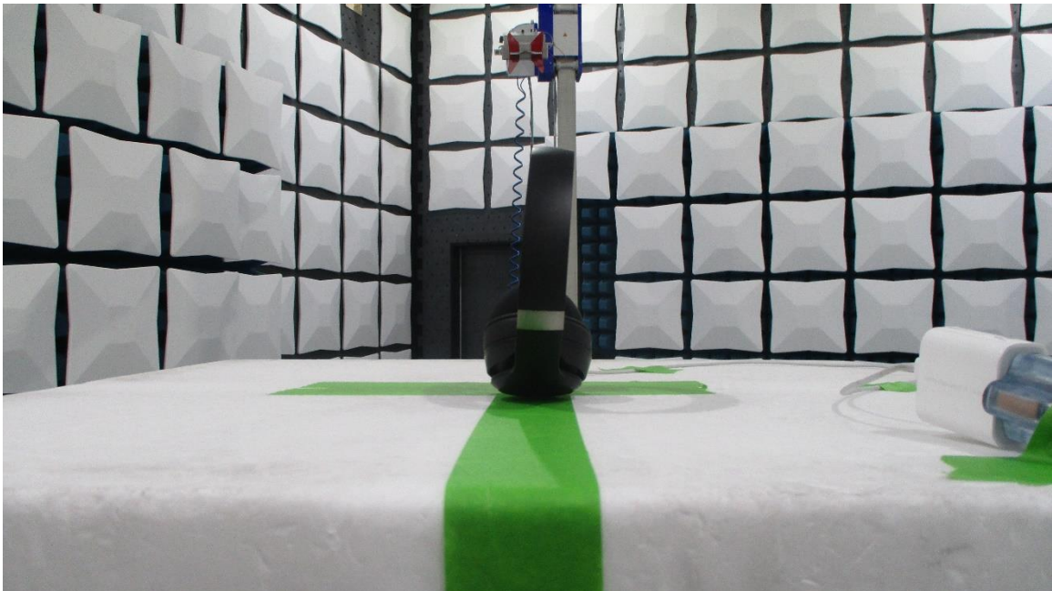
Figure 10: 1-18GHz Test Setup (Rear View)
