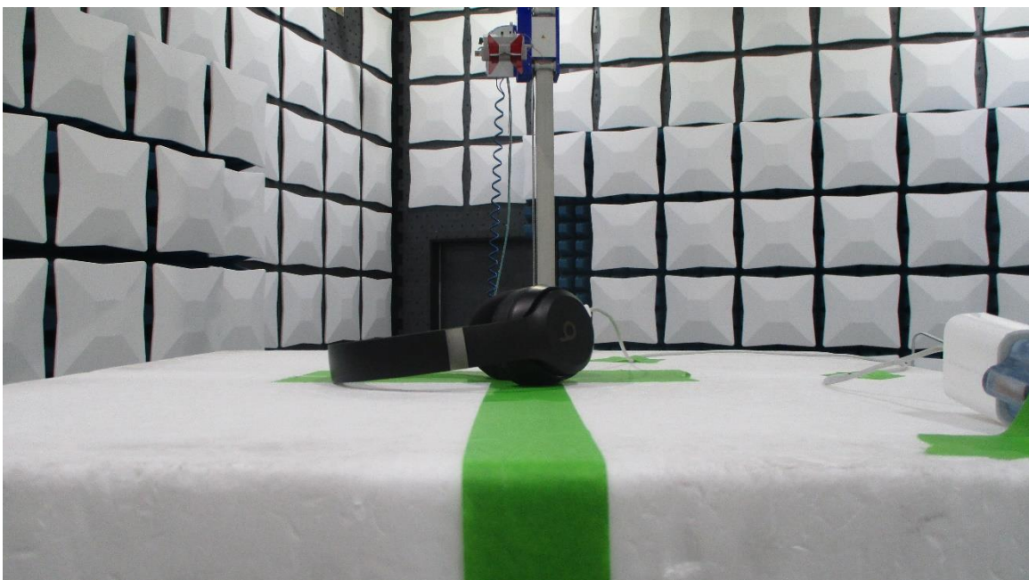
Figure 8: 1-18GHz Test Setup (Rear View)
