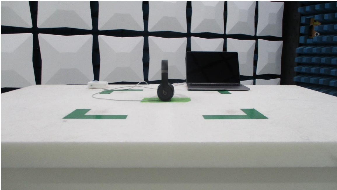
Figure 21: 30MHz-1GHz Test Setup (Front View)
