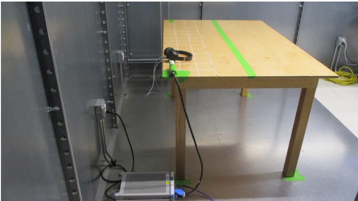
Figure 2: AC Line Conducted Emissions (Side View)
