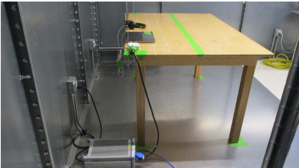
Figure 4: AC Line Conducted Emissions (Side View)
