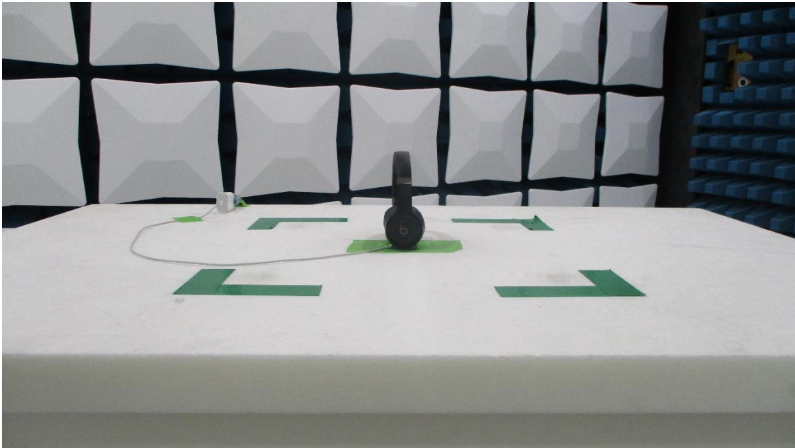
Figure 15: 30MHz-1GHz Test Setup (Front View)
