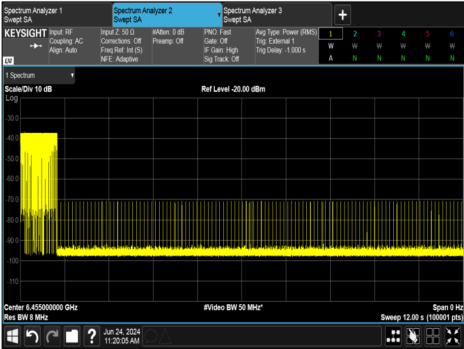
Figure 453 - U-NII-6, Minimum Bandwidth (AWGN Mid)
