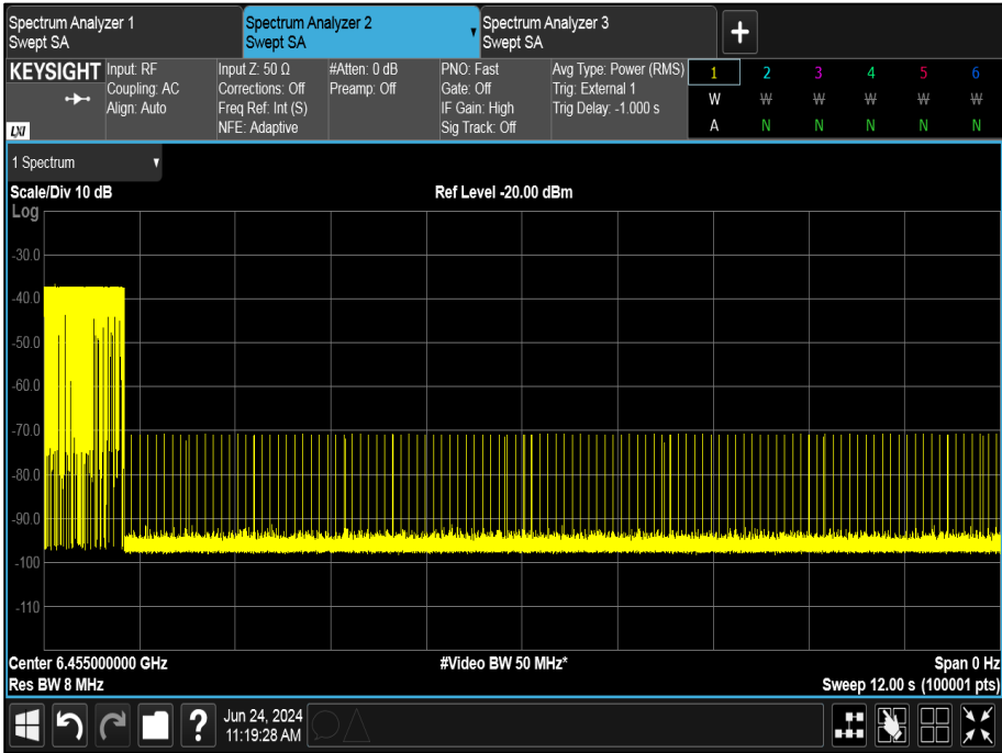
Figure 452 - U-NII-6, Minimum Bandwidth (AWGN Low)
