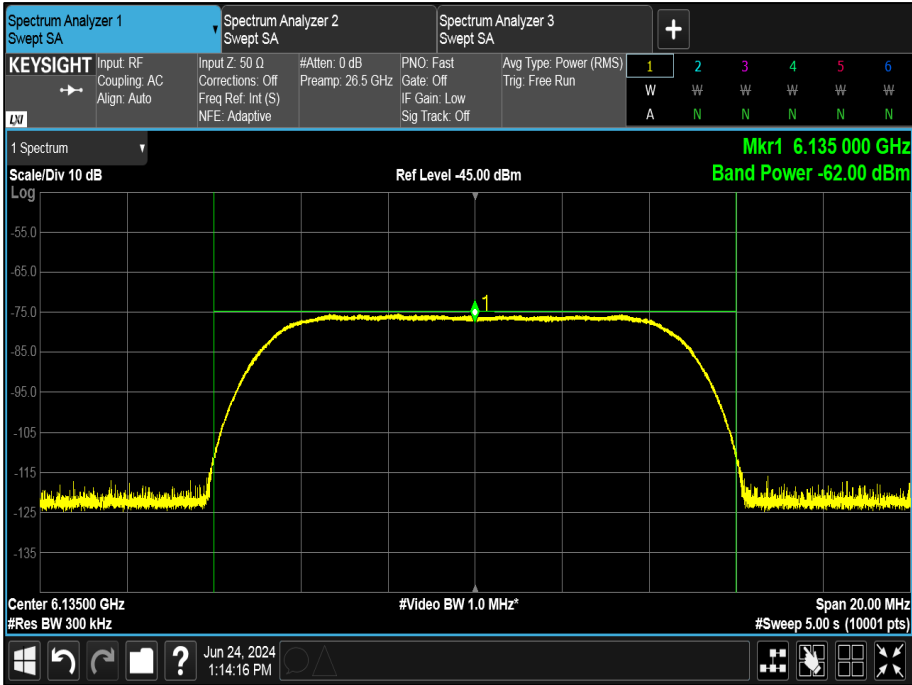
Figure 446 - Example of AWGN Signal
