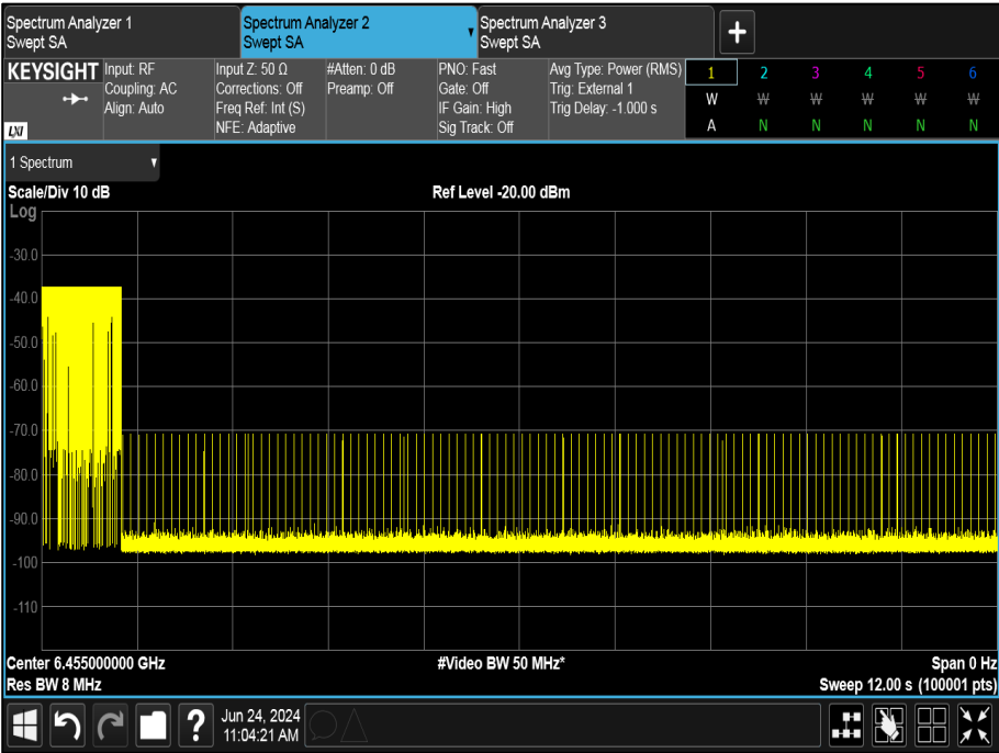
Figure 454 - U-NII-6, Minimum Bandwidth (AWGN High)
