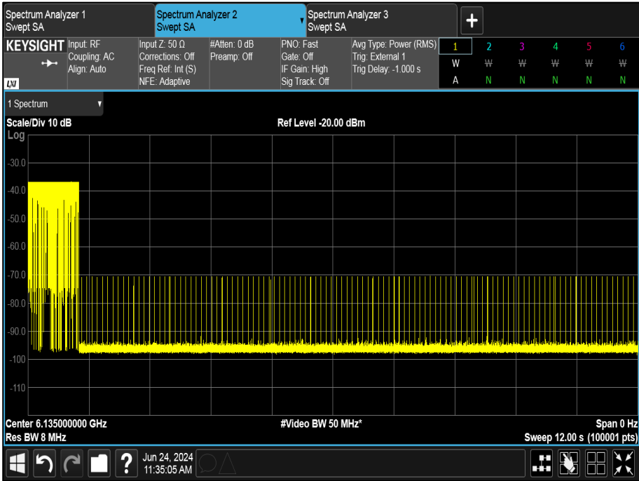
Figure 450 - U-NII-5, Minimum Bandwidth (AWGN High)
