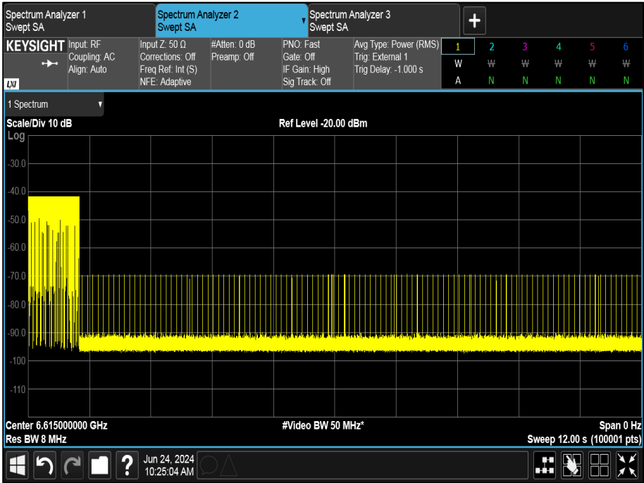
Figure 457 - U-NII-7, Minimum Bandwidth (AWGN Mid)
