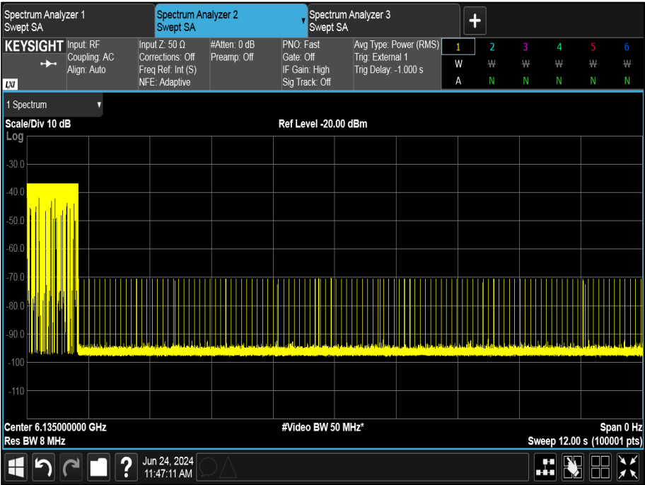
Figure 448 - U-NII-5, Minimum Bandwidth (AWGN Low)
