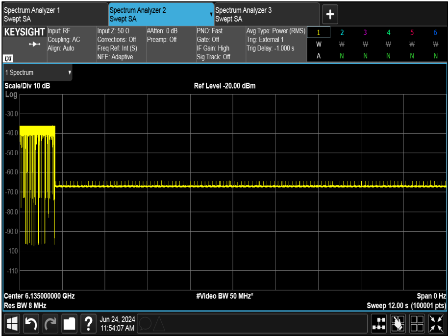
Figure 447 - U-NII-5, Minimum Bandwidth
