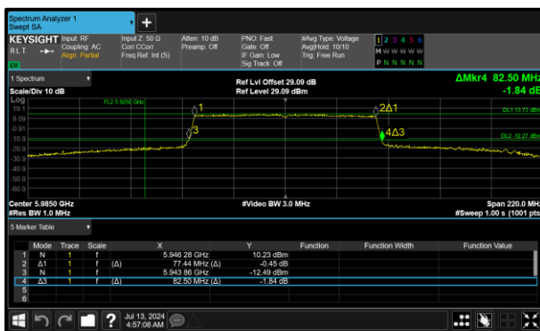
Figure 117 - 802.11ax HE80 SU SP Minimum 26 dB BW
