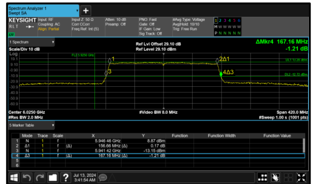
Figure 92 - 802.11ax HE160 SU SP Maximum 99% OBW
