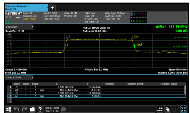
Figure 120 - 802.11ax HE160 SU SP Maximum 26 dB BW
