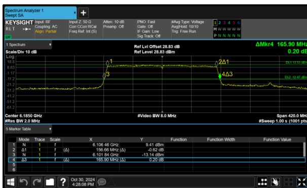
Figure 119 - 802.11ax HE160 SU SP Minimum 26 dB BW
