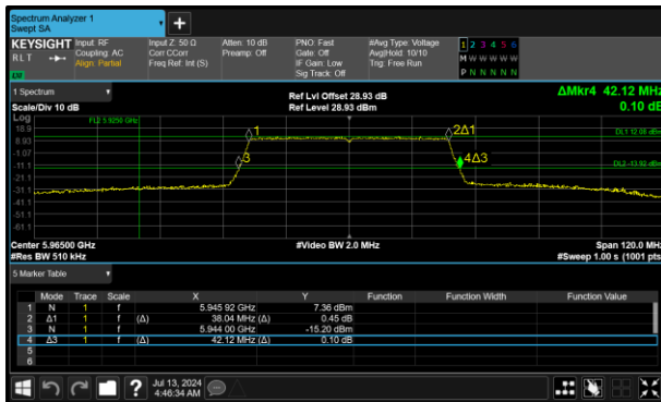
Figure 115 - 802.11ax HE40 SU SP Minimum 26 dB BW
