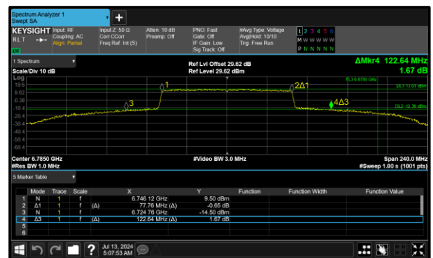
Figure 118 - 802.11ax HE80 SU SP Maximum 26 dB BW
