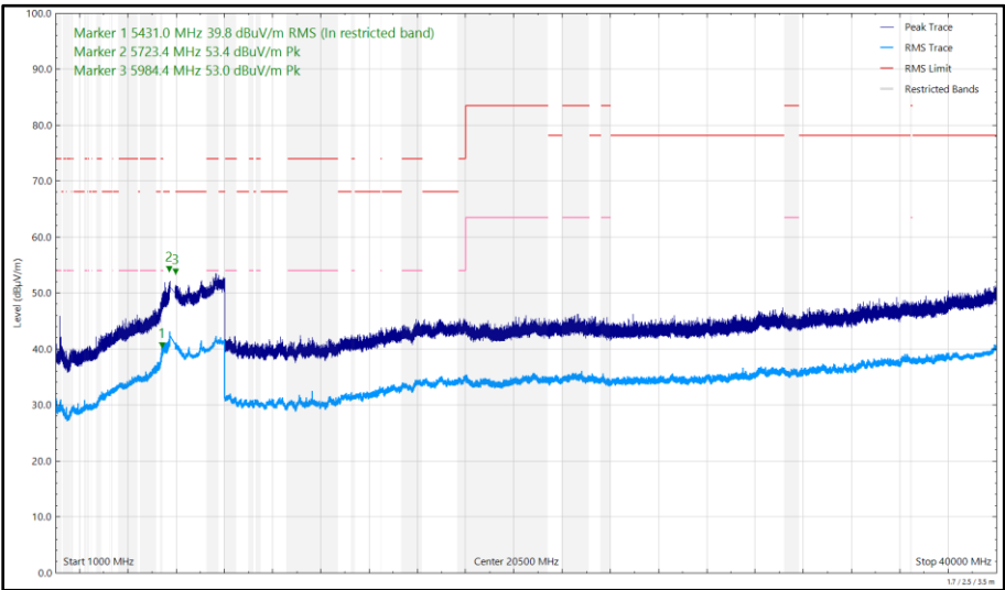
Figure 645 - U-NII-3 - 5825 MHz (CH165), HE20, RU26-0, CDD, Core 0 + Core 1, 1 GHz to 40 GHz, Vertical
