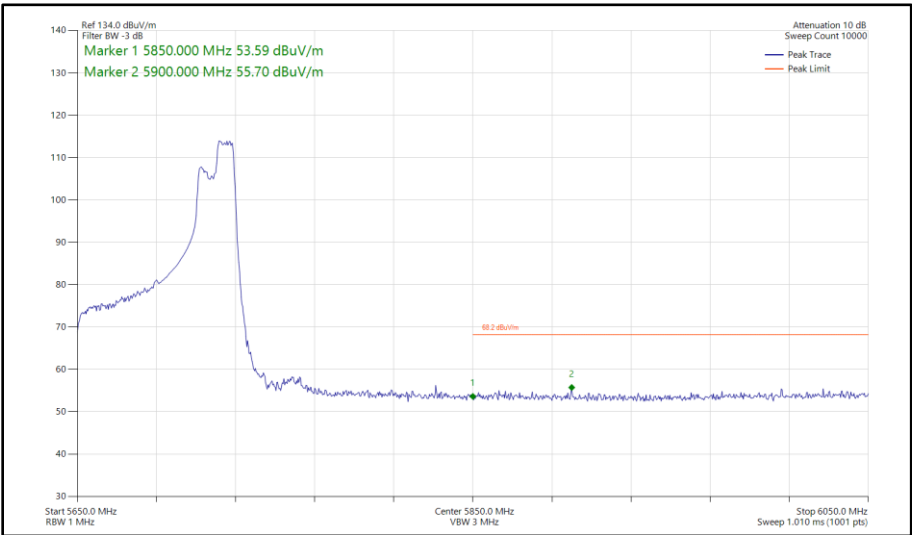
Figure 504 - 802.11ax HE80, RU 106-60, SISO, Core 0 - 5690 MHz Band Edge Frequency 5850 MHz
