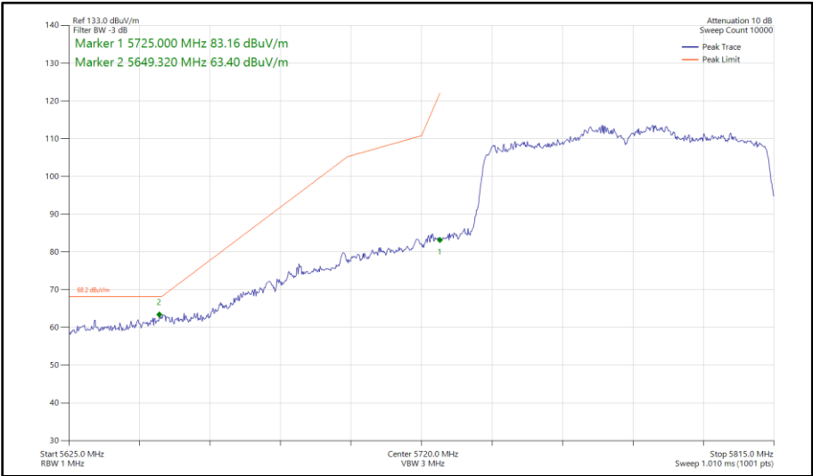
Figure 525 - 802.11ac VHT80, CDD, Core 0 - Core 1 - 5775 MHz Band Edge Frequency 5725 MHz
