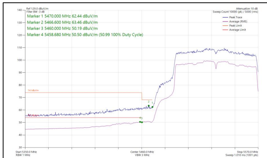
Figure 492 - 802.11ac VHT80, SISO, Core 0 - 5530 MHz Band Edge Frequency 5470 MHz
