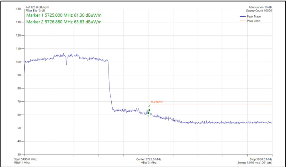
Figure 579 - 802.11ax HE160, SU, SDM, Core 0 - Core 1 - 5570 MHz Band Edge Frequency 5725 MHz
