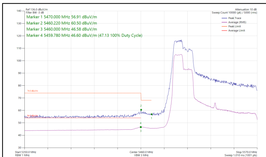
Figure 539 - 802.11ax HE80, RU 106-53, SDM, Core 0 - Core 1 - 5530 MHz Band Edge Frequency 5470 MHz
