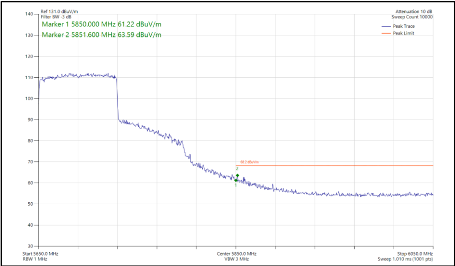
Figure 503 - 802.11ax HE80, SU, SISO, Core 0 - 5690 MHz Band Edge Frequency 5850 MHz
