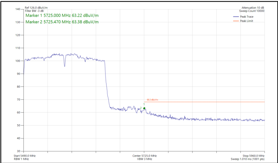
Figure 578 - 802.11ac VHT160, SDM, Core 0 - Core 1 - 5570 MHz Band Edge Frequency 5725 MHz
