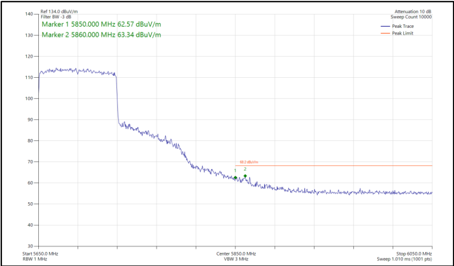
Figure 518 - 802.11ax HE80, SU, SISO, Core 1 - 5690 MHz Band Edge Frequency 5850 MHz
