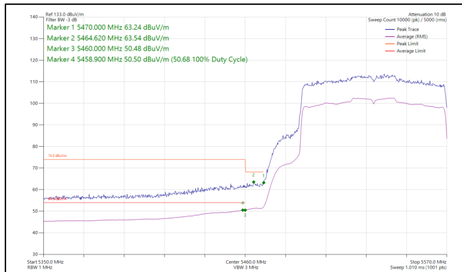
Figure 508 - 802.11ax HE80, SU, SISO, Core 1 - 5530 MHz Band Edge Frequency 5470 MHz
