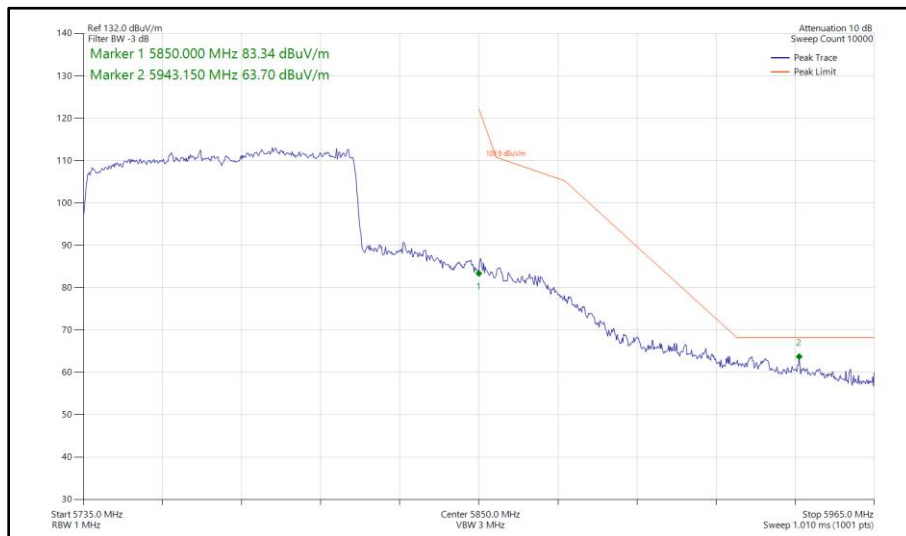
Figure 550 - 802.11ax HE80, SU, SDM, Core 0 - Core 1 - 5775 MHz Band Edge Frequency 5850 MHz
