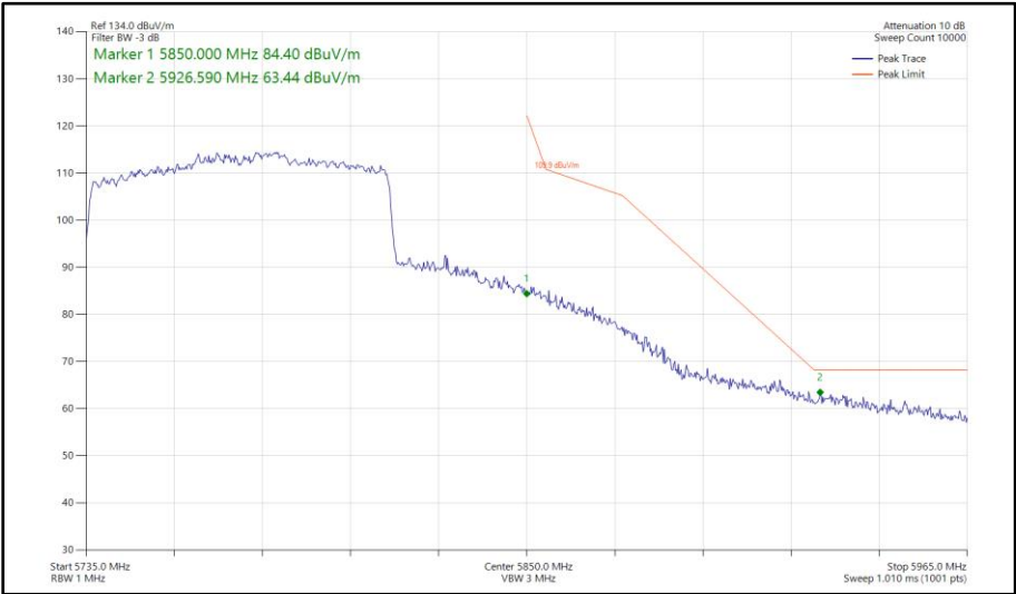
Figure 535 - 802.11ax HE80, SU, CDD, Core 0 - Core 1 - 5775 MHz Band Edge Frequency 5850 MHz
