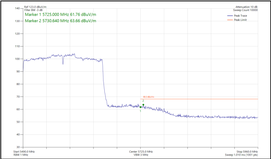
Figure 561 - 802.11ax HE160, SU, SISO, Core 0 - 5570 MHz Band Edge Frequency 5725 MHz
