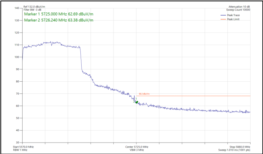
Figure 499 - 802.11ax HE80, SU, SISO, Core 0 - 5610 MHz Band Edge Frequency 5725 MHz
