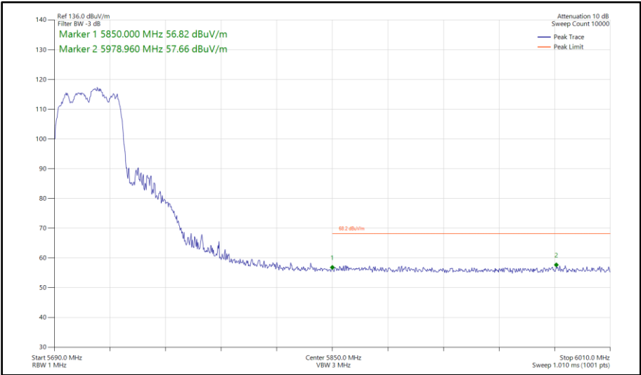
Figure 490 - 802.11ac VHT40, TxBF, Core 0 - Core 1 - 5710 MHz Band Edge Frequency 5850 MHz
