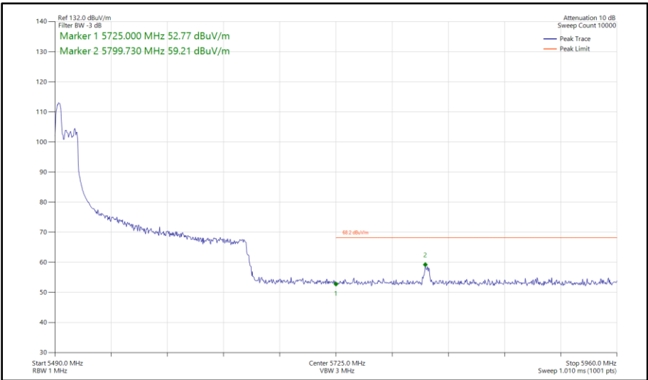
Figure 574 - 802.11ax HE160, RU 52-37P, CDD, Core 0 - Core 1 - 5570 MHz Band Edge Frequency 5725 MHz
