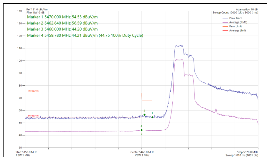
Figure 494 - 802.11ax HE80, RU 106-53, SISO, Core 0 - 5530 MHz Band Edge Frequency 5470 MHz
