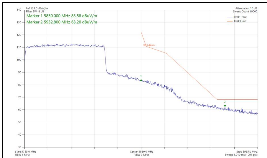
Figure 505 - 802.11ax HE80, SU, SISO, Core 0 - 5775 MHz Band Edge Frequency 5850 MHz
