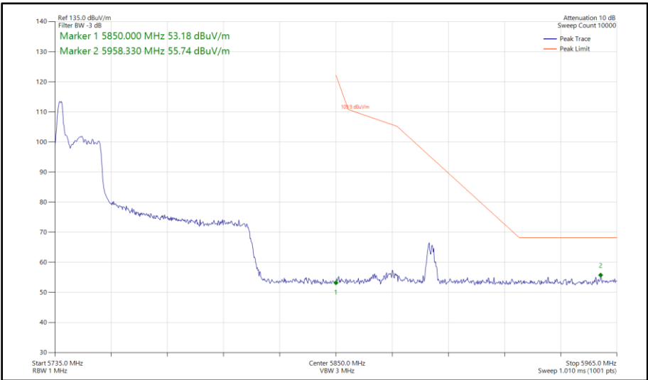
Figure 536 - 802.11ax HE80, RU 26-0, CDD, Core 0 - Core 1 - 5775 MHz Band Edge Frequency 5850 MHz
