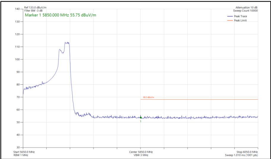
Figure 519 - 802.11ax HE80, RU 106-60, SISO, Core 1 - 5690 MHz Band Edge Frequency 5850 MHz
