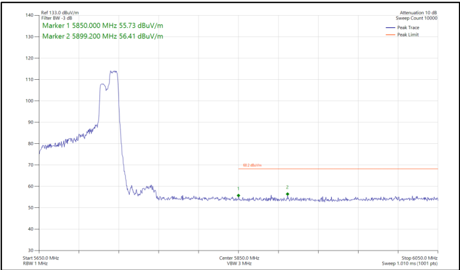
Figure 549 - 802.11ax HE80, RU 106-60, SDM, Core 0 - Core 1 - 5690 MHz Band Edge Frequency 5850 MHz
