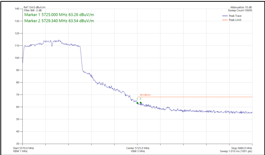
Figure 543 - 802.11ac VHT80, SDM, Core 0 - Core 1 - 5610 MHz Band Edge Frequency 5725 MHz
