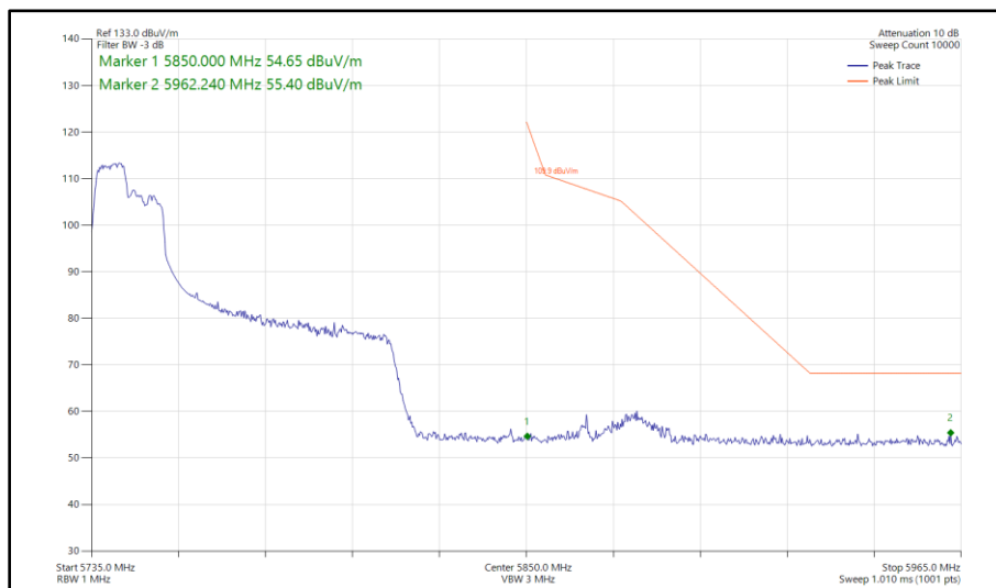
Figure 506 - 802.11ax HE80, RU 106-53, SISO, Core 0 - 5775 MHz Band Edge Frequency 5850 MHz
