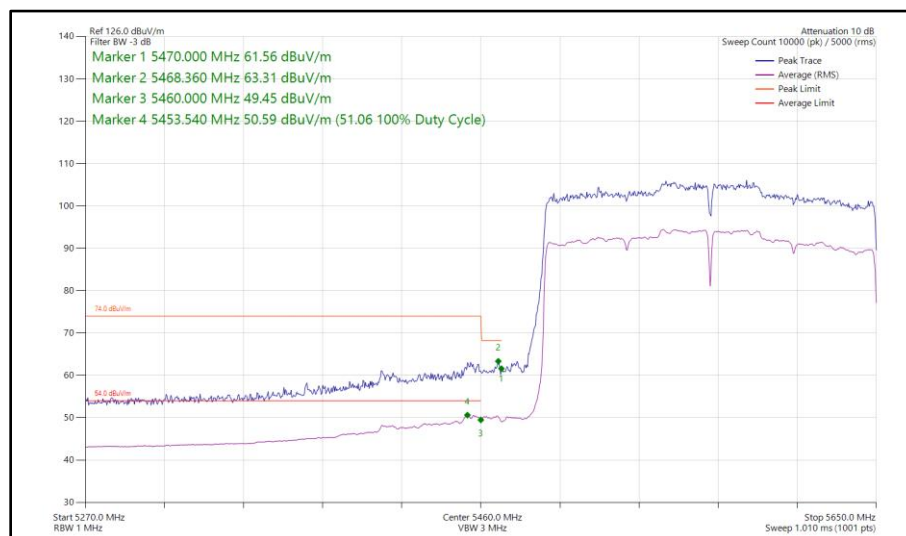
Figure 564 - 802.11ax HE160, SU, SISO, Core 1 - 5570 MHz Band Edge Frequency 5470 MHz
