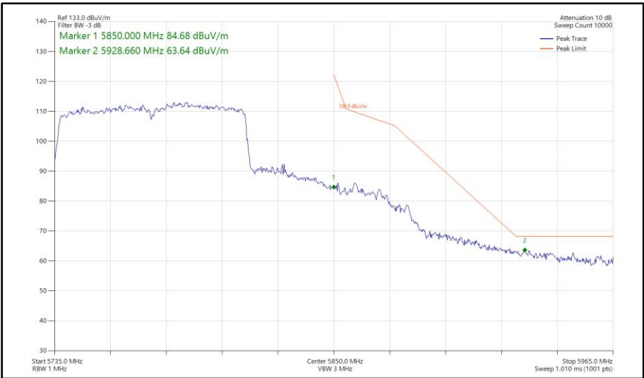
Figure 532 - 802.11ac VHT80, CDD, Core 0 - Core 1 - 5775 MHz Band Edge Frequency 5850 MHz
