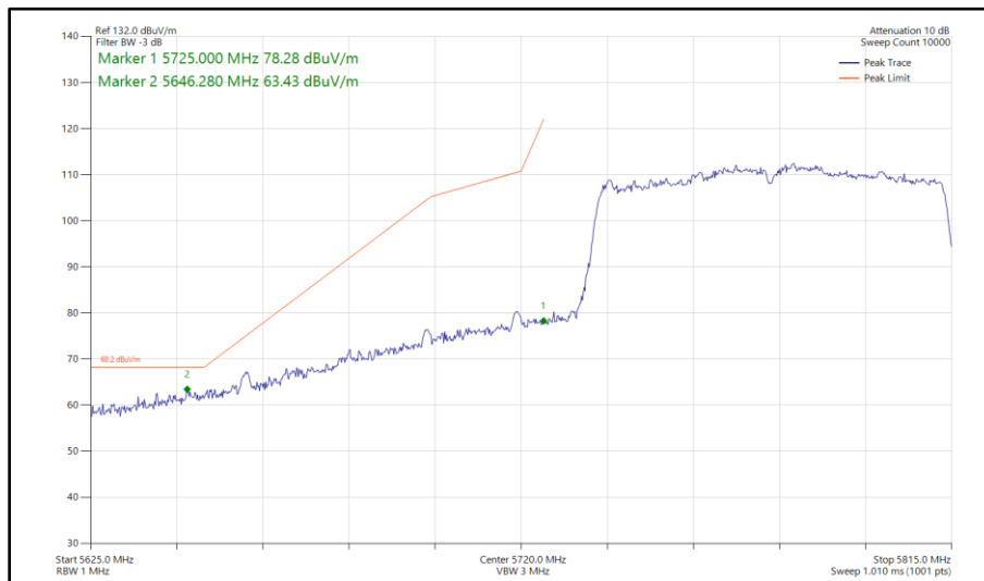
Figure 540 - 802.11ac VHT80, SDM, Core 0 - Core 1 - 5775 MHz Band Edge Frequency 5725 MHz
