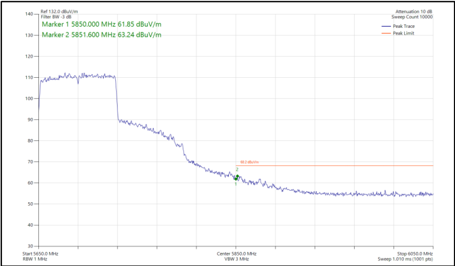
Figure 501 - 802.11ac VHT80, SISO, Core 0 - 5690 MHz Band Edge Frequency 5850 MHz
