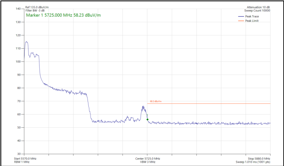
Figure 530 - 802.11ax HE80, RU 52-37, CDD, Core 0 - Core 1 - 5610 MHz Band Edge Frequency 5725 MHz
