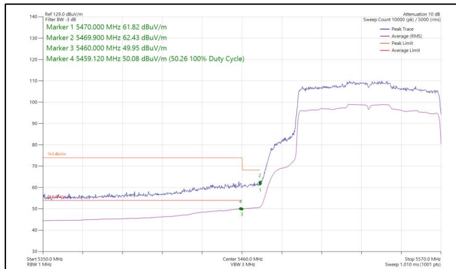
Figure 493 - 802.11ax HE80, SU, SISO, Core 0 - 5530 MHz Band Edge Frequency 5470 MHz
