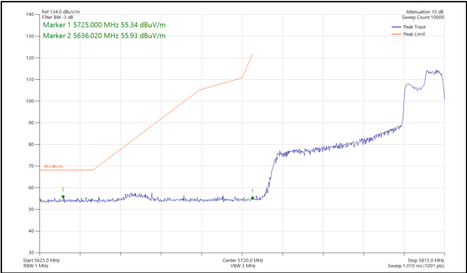
Figure 527 - 802.11ax HE80, RU 106-60, CDD, Core 0 - Core 1 - 5775 MHz Band Edge Frequency 5725 MHz
