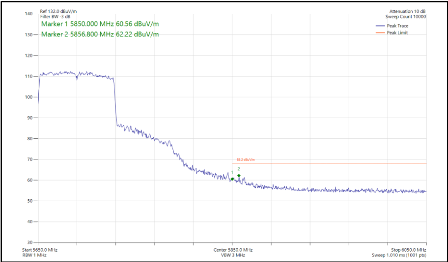
Figure 546 - 802.11ac VHT80, SDM, Core 0 - Core 1 - 5690 MHz Band Edge Frequency 5850 MHz
