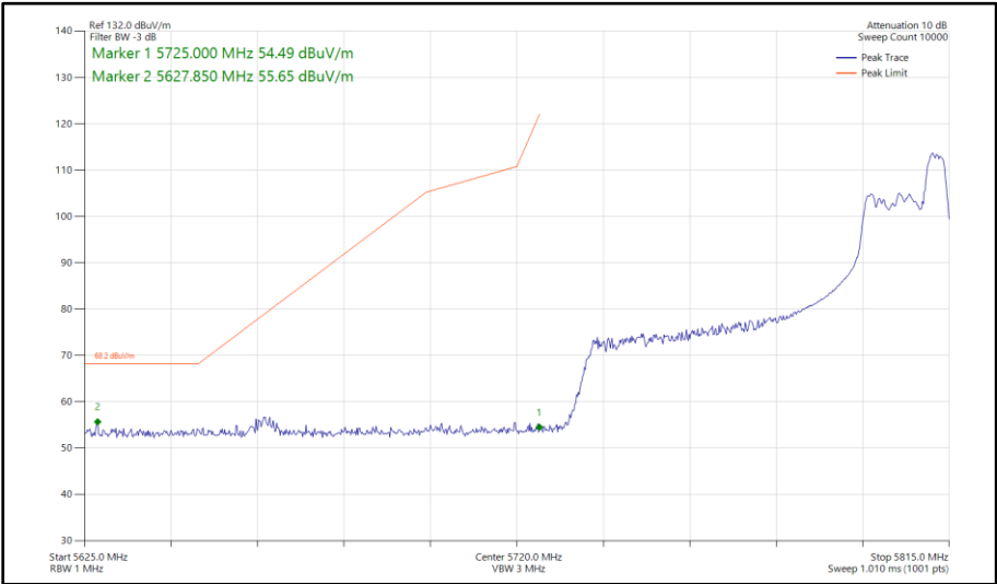
Figure 497 - 802.11ax HE80, RU 52-52, SISO, Core 0 - 5775 MHz Band Edge Frequency 5725 MHz
