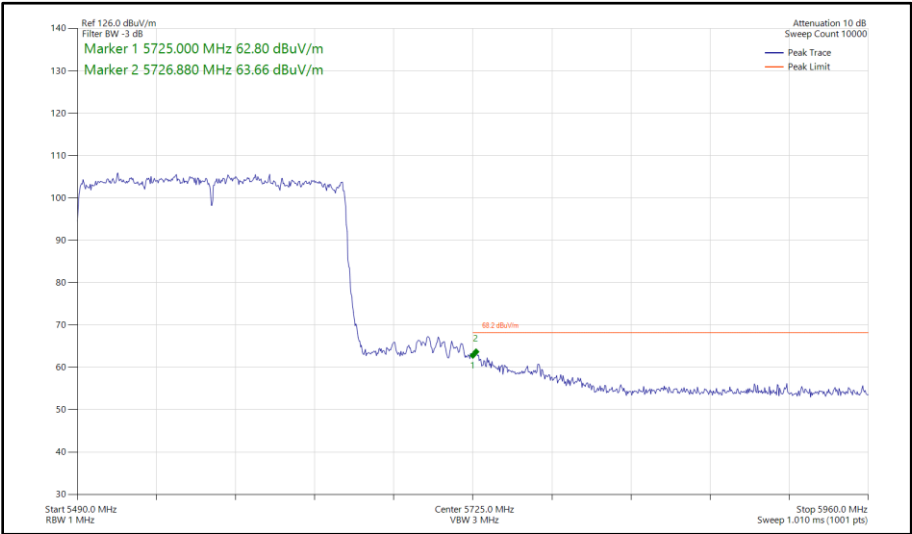
Figure 573 - 802.11ax HE160, SU, CDD, Core 0 - Core 1 - 5570 MHz Band Edge Frequency 5725 MHz
