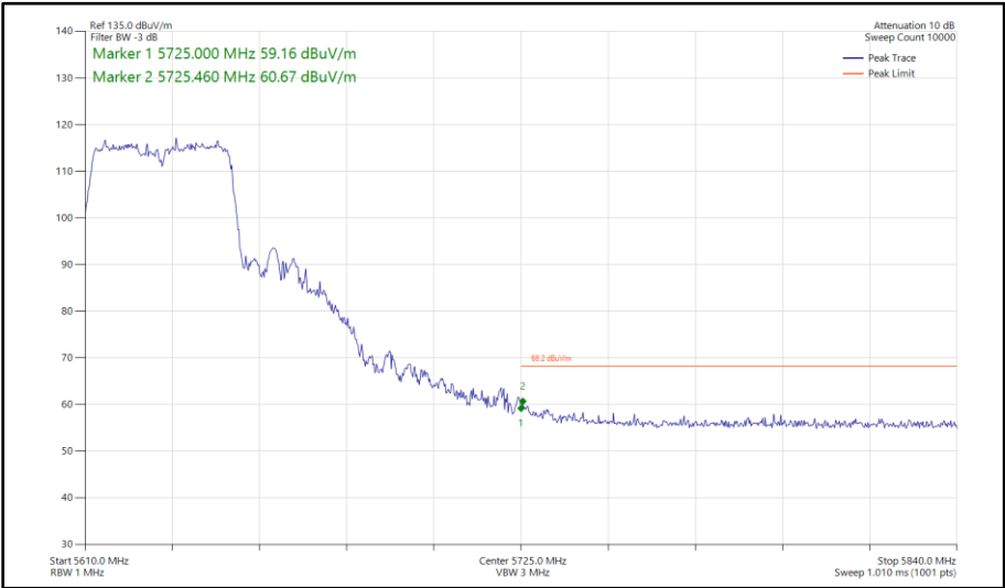
Figure 488 - 802.11ac VHT40, TxBF, Core 0 - Core 1 - 5630 MHz Band Edge Frequency 5725 MHz
