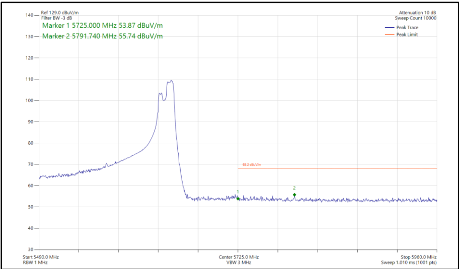
Figure 562 - 802.11ax HE160, RU 106-60S, SISO, Core 0 - 5570 MHz Band Edge Frequency 5725 MHz
