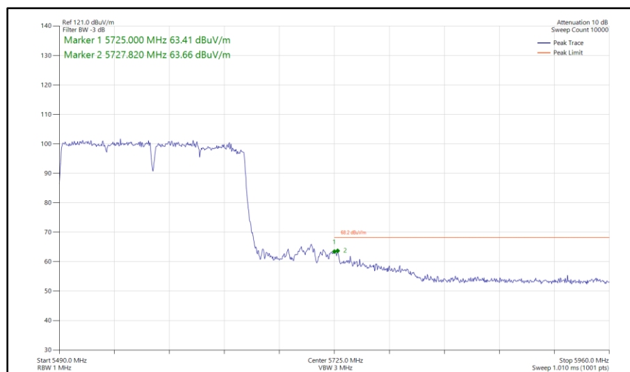
Figure 560 - 802.11ac VHT160, SISO, Core 0 - 5570 MHz Band Edge Frequency 5725 MHz
