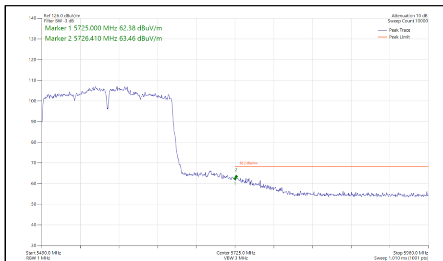
Figure 566 - 802.11ac VHT160, SISO, Core 1 - 5570 MHz Band Edge Frequency 5725 MHz
