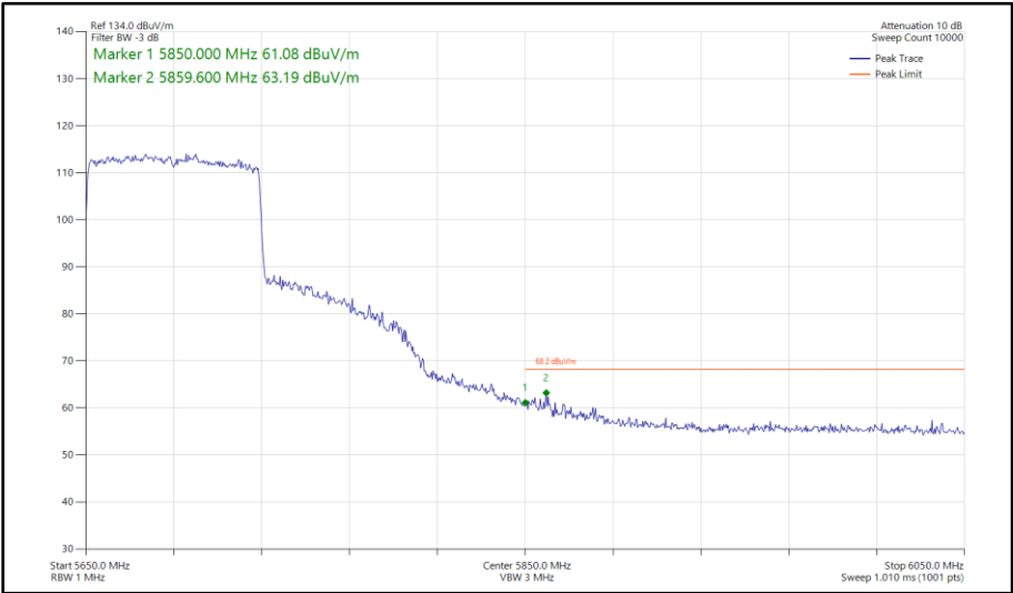
Figure 533 - 802.11ax HE80, SU, CDD, Core 0 - Core 1 - 5690 MHz Band Edge Frequency 5850 MHz
