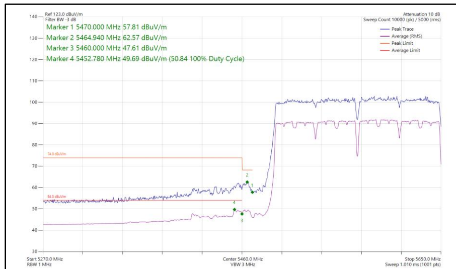
Figure 563 - 802.11ac VHT160, SISO, Core 1 - 5570 MHz Band Edge Frequency 5470 MHz
