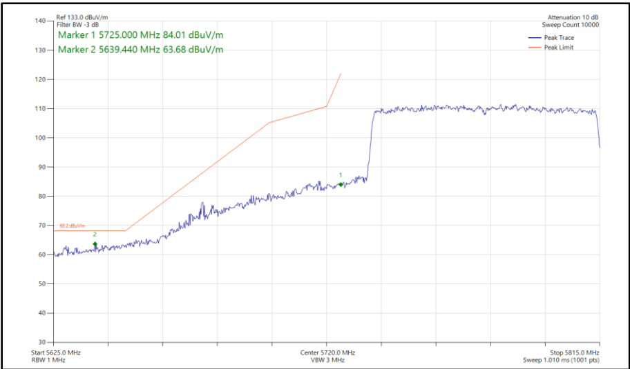
Figure 526 - 802.11ax HE80, SU, CDD, Core 0 - Core 1 - 5775 MHz Band Edge Frequency 5725 MHz
