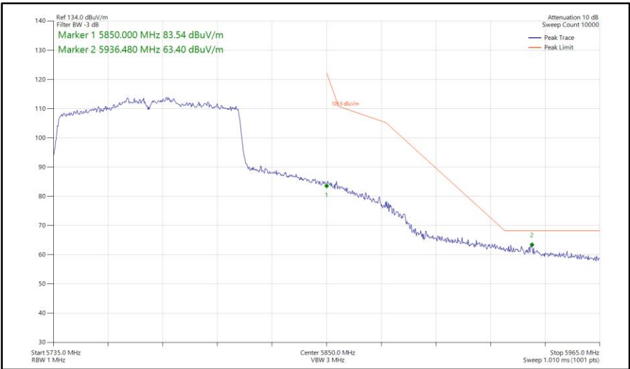
Figure 517 - 802.11ac VHT80, SISO, Core 1 - 5775 MHz Band Edge Frequency 5850 MHz
