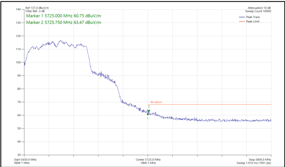
Figure 489 - 802.11ac VHT40, TxBF, Core 0 - Core 1 - 5670 MHz Band Edge Frequency 5725 MHz
