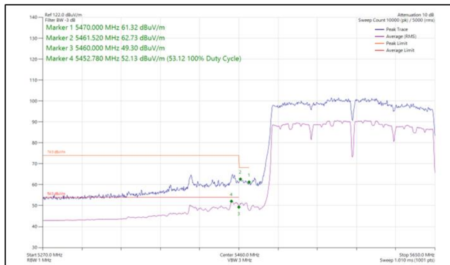
Figure 557 - 802.11ac VHT160, SISO, Core 0 - 5570 MHz Band Edge Frequency 5470 MHz
