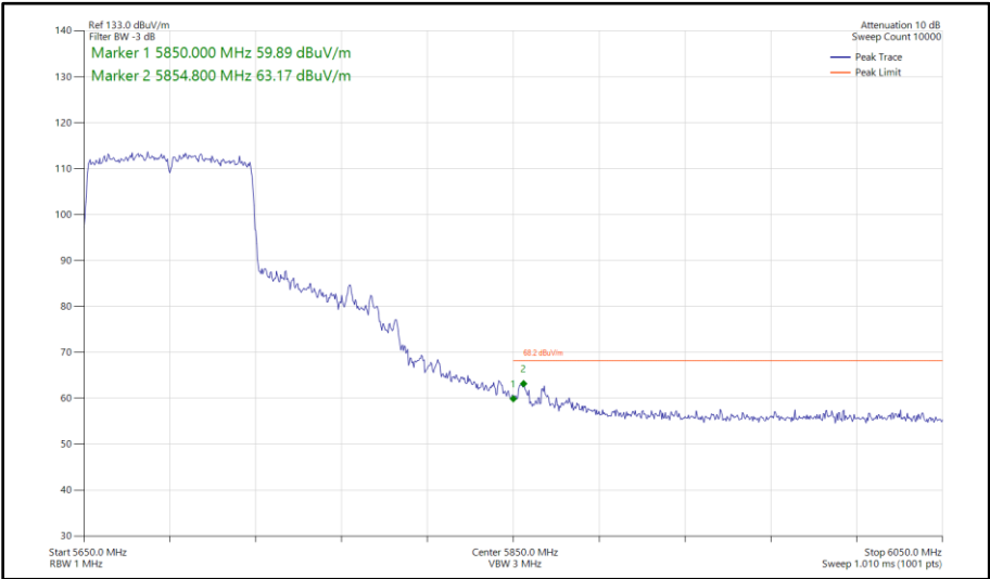
Figure 531 - 802.11ac VHT80, CDD, Core 0 - Core 1 - 5690 MHz Band Edge Frequency 5850 MHz
