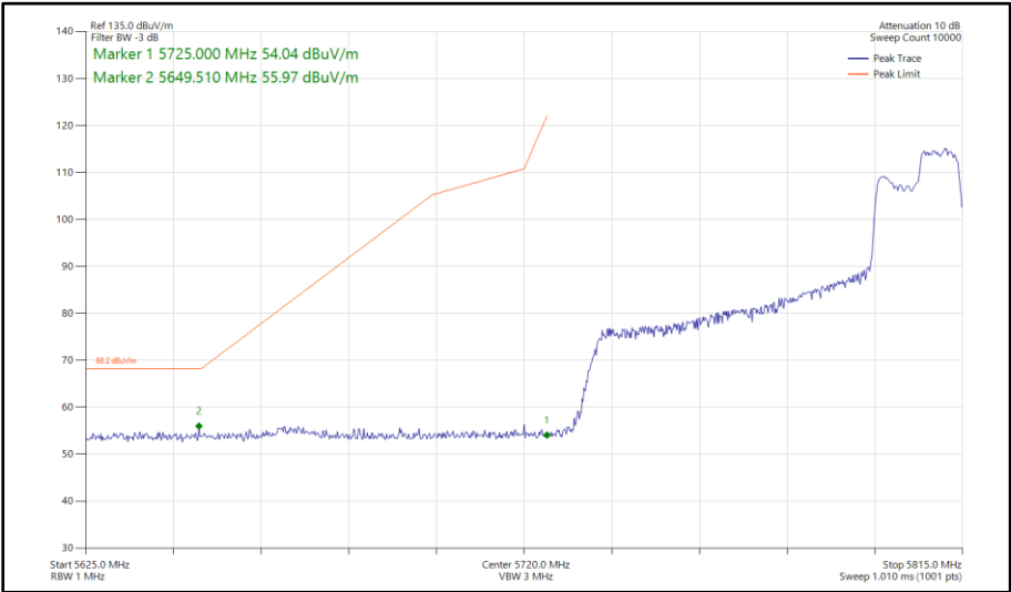
Figure 542 - 802.11ax HE80, RU 106-60, SDM, Core 0 - Core 1 - 5775 MHz Band Edge Frequency 5725 MHz
