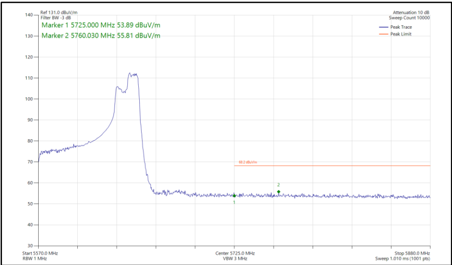
Figure 500 - 802.11ax HE80, RU 106-60, SISO, Core 0 - 5610 MHz Band Edge Frequency 5725 MHz
