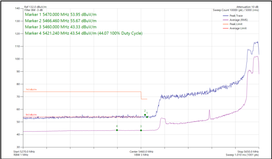
Figure 577 - 802.11ax HE160, RU 106-60S, SDM, Core 0 - Core 1 - 5570 MHz Band Edge Frequency 5470 MHz
