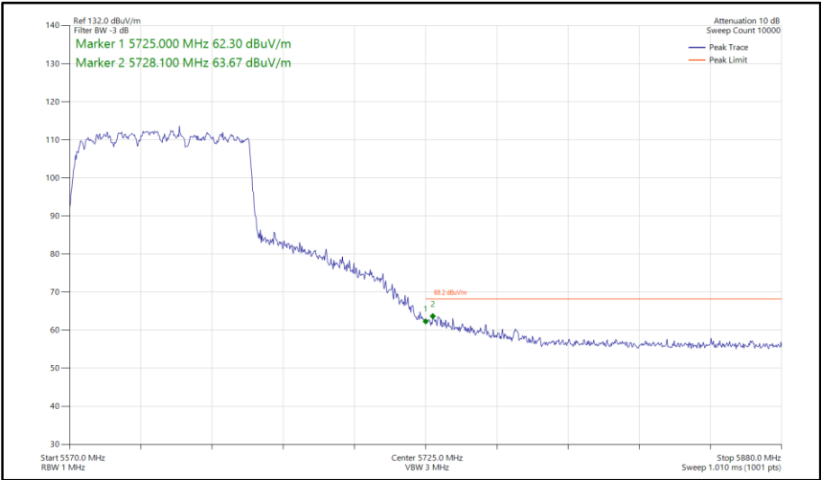
Figure 554 - 802.11ac VHT80, TxBF, Core 0 - Core 1 - 5610 MHz Band Edge Frequency 5725 MHz
