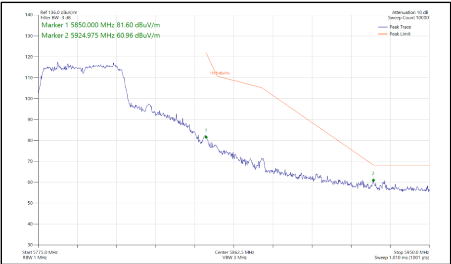
Figure 491 - 802.11ac VHT40, TxBF, Core 0 - Core 1 - 5795 MHz Band Edge Frequency 5850 MHz
