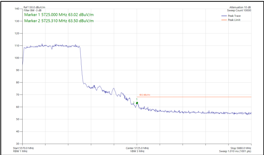
Figure 513 - 802.11ac VHT80, SISO, Core 1 - 5610 MHz Band Edge Frequency 5725 MHz
