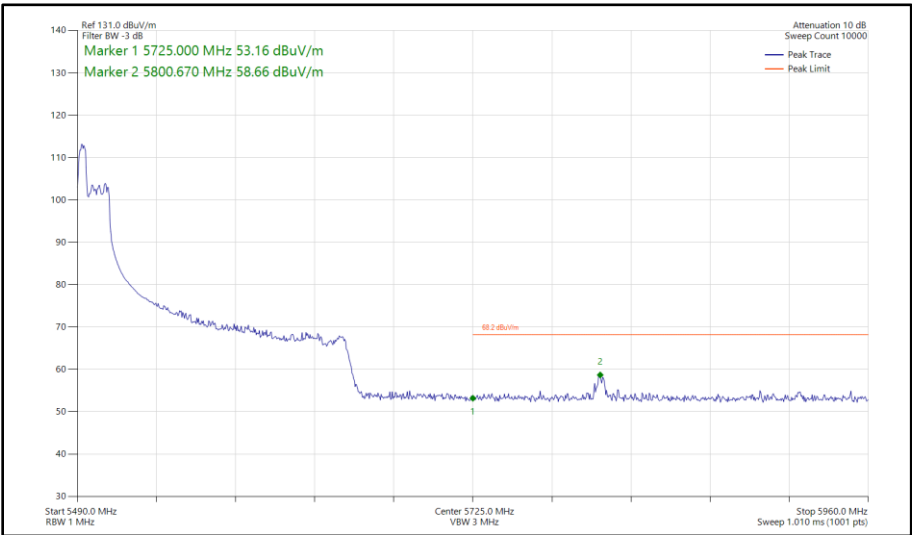
Figure 568 - 802.11ax HE160, RU 52-37P, SISO, Core 1 - 5570 MHz Band Edge Frequency 5725 MHz
