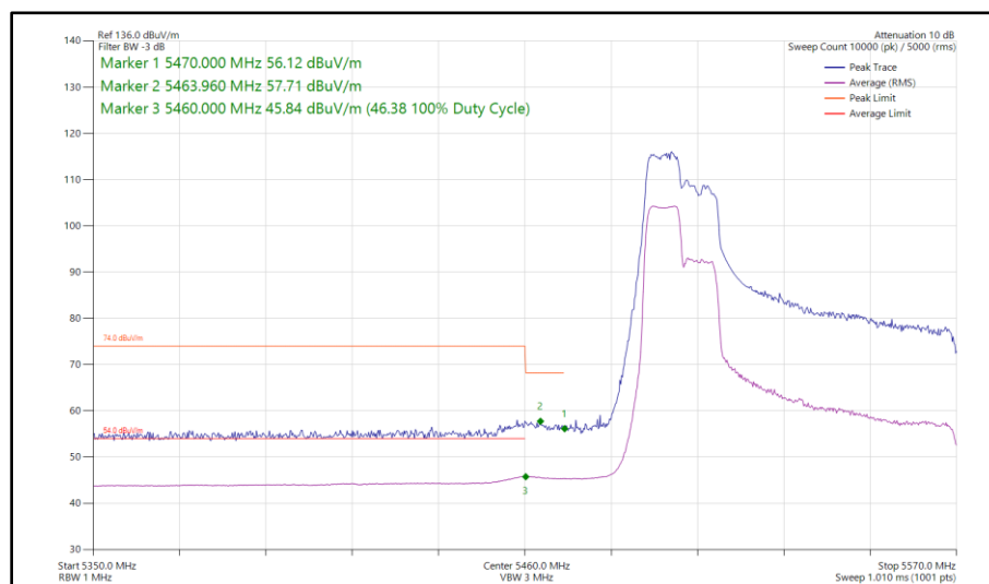
Figure 509 - 802.11ax HE80, RU 106-53, SISO, Core 1 - 5530 MHz Band Edge Frequency 5470 MHz
