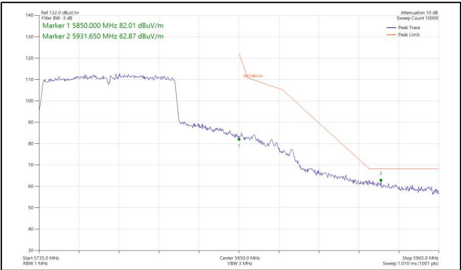
Figure 502 - 802.11ac VHT80, SISO, Core 0 - 5775 MHz Band Edge Frequency 5850 MHz
