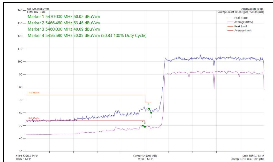
Figure 570 - 802.11ax HE160, SU, CDD, Core 0 - Core 1 - 5570 MHz Band Edge Frequency 5470 MHz
