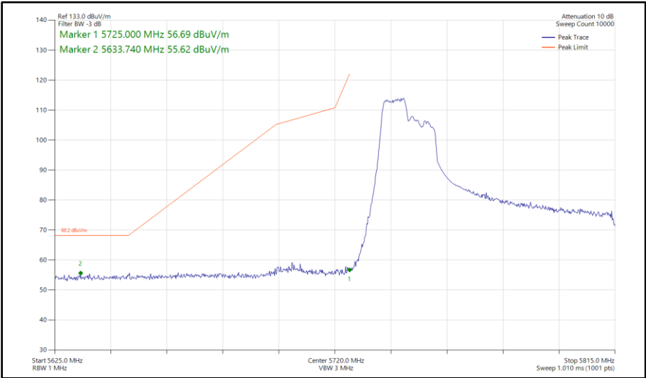
Figure 512 - 802.11ax HE80, RU 106-53, SISO, Core 1 - 5775 MHz Band Edge Frequency 5725 MHz
