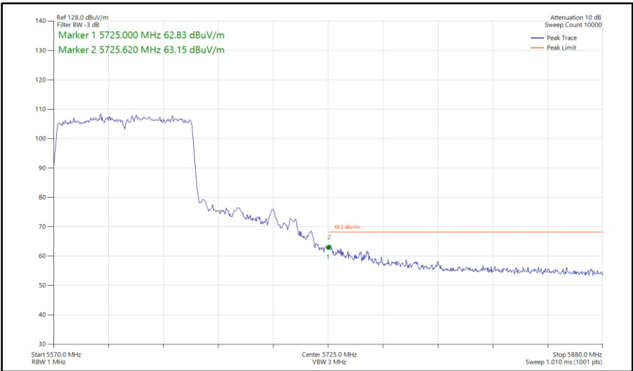
Figure 498 - 802.11ac VHT80, SISO, Core 0 - 5610 MHz Band Edge Frequency 5725 MHz
