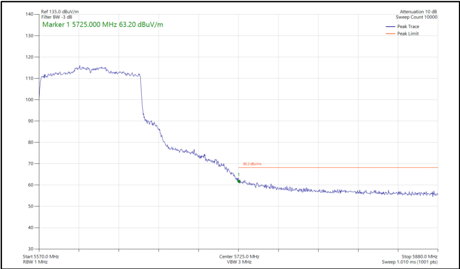
Figure 544 - 802.11ax HE80, SU, SDM, Core 0 - Core 1 - 5610 MHz Band Edge Frequency 5725 MHz
