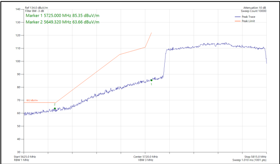
Figure 496 - 802.11ax HE80, SU, SISO, Core 0 - 5775 MHz Band Edge Frequency 5725 MHz
