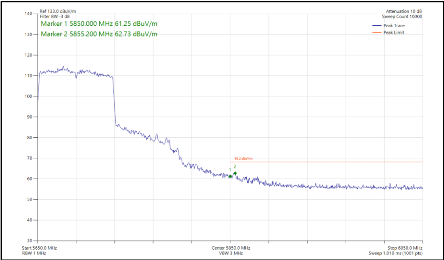
Figure 516 - 802.11ac VHT80, SISO, Core 1 - 5690 MHz Band Edge Frequency 5850 MHz
