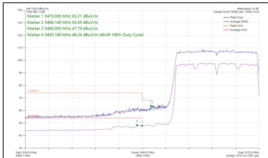
Figure 537 - 802.11ac VHT80, SDM, Core 0 - Core 1 - 5530 MHz Band Edge Frequency 5470 MHz
