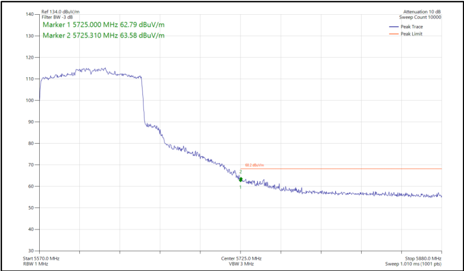
Figure 514 - 802.11ax HE80, SU, SISO, Core 1 - 5610 MHz Band Edge Frequency 5725 MHz
