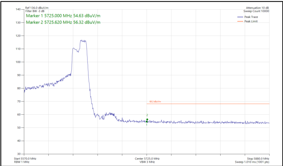
Figure 545 - 802.11ax HE80, RU 106-60, SDM, Core 0 - Core 1 - 5610 MHz Band Edge Frequency 5725 MHz
