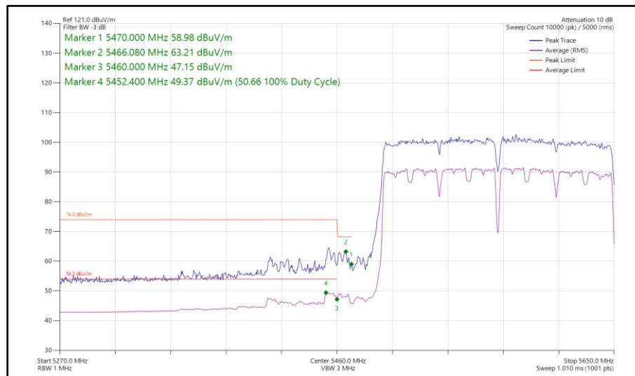
Figure 575 - 802.11ac VHT160, SDM, Core 0 - Core 1 - 5570 MHz Band Edge Frequency 5470 MHz
