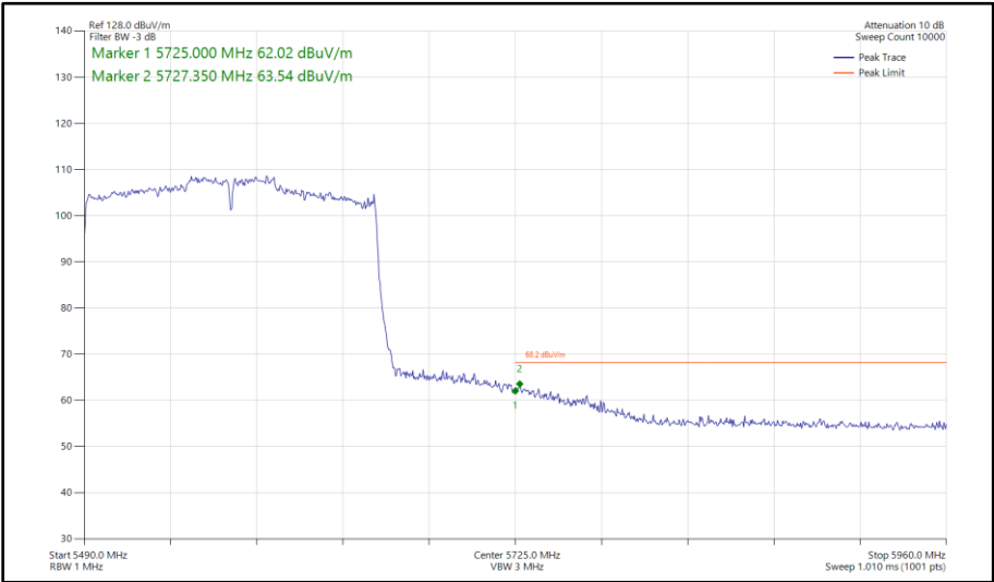
Figure 567 - 802.11ax HE160, SU, SISO, Core 1 - 5570 MHz Band Edge Frequency 5725 MHz
