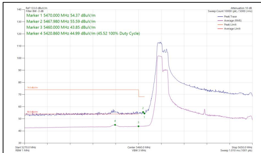
Figure 565 - 802.11ax HE160, RU 106-53P, SISO, Core 1 - 5570 MHz Band Edge Frequency 5470 MHz
