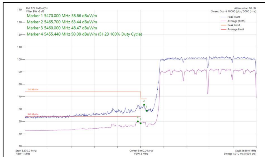
Figure 569 - 802.11ac VHT160, CDD, Core 0 - Core 1 - 5570 MHz Band Edge Frequency 5470 MHz
