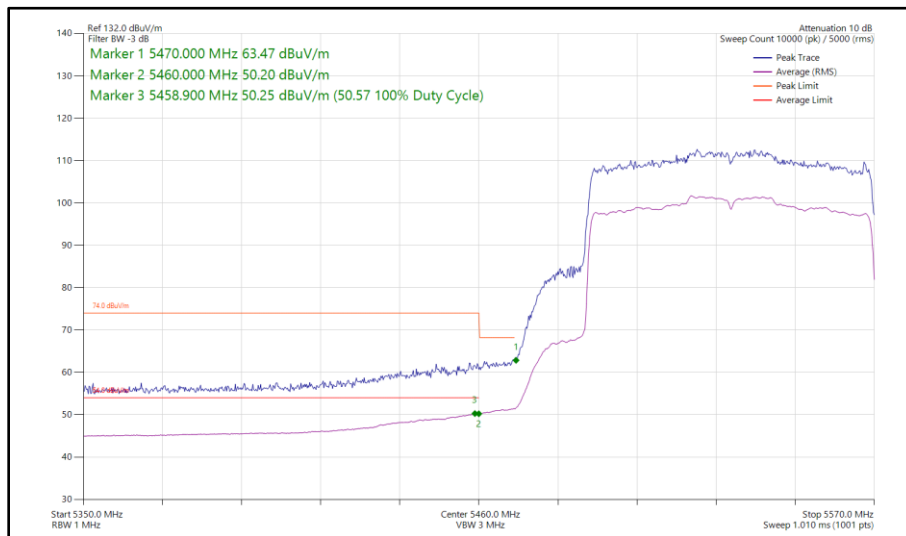
Figure 523 - 802.11ax HE80, SU, CDD, Core 0 - Core 1 - 5530 MHz Band Edge Frequency 5470 MHz
