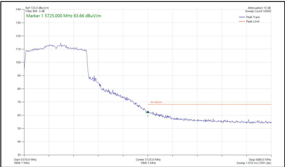
Figure 528 - 802.11ac VHT80, CDD, Core 0 - Core 1 - 5610 MHz Band Edge Frequency 5725 MHz
