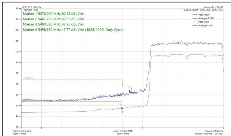
Figure 538 - 802.11ax HE80, SU, SDM, Core 0 - Core 1 - 5530 MHz Band Edge Frequency 5470 MHz
