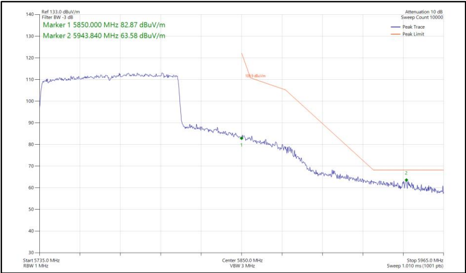
Figure 520 - 802.11ax HE80, SU, SISO, Core 1 - 5775 MHz Band Edge Frequency 5850 MHz
