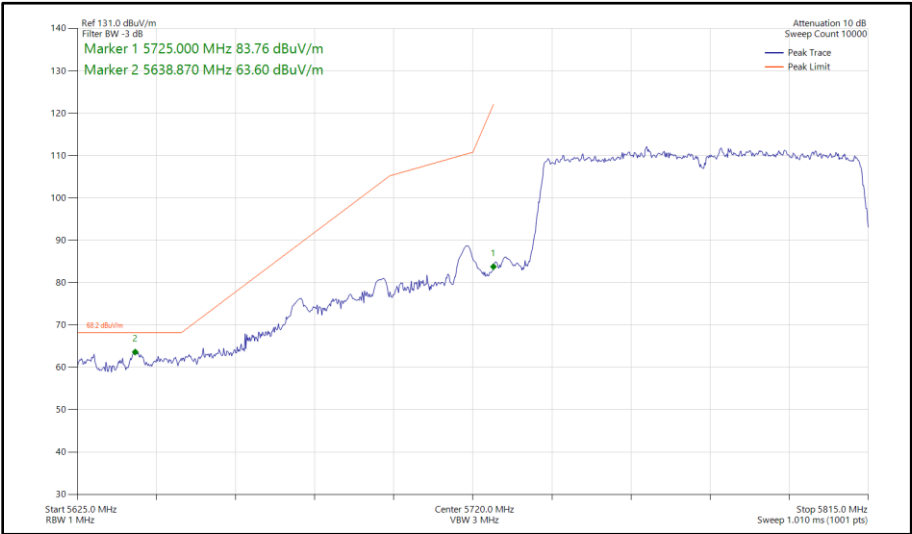
Figure 495 - 802.11ac VHT80, SISO, Core 0 - 5775 MHz Band Edge Frequency 5725 MHz
