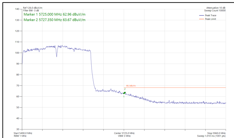
Figure 572 - 802.11ac VHT160, CDD, Core 0 - Core 1 - 5570 MHz Band Edge Frequency 5725 MHz
