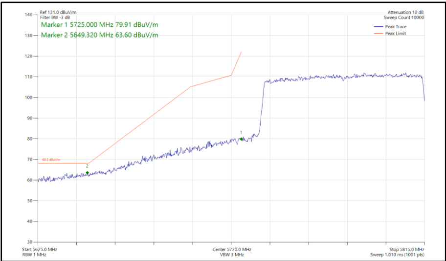
Figure 511 - 802.11ax HE80, SU, SISO, Core 1 - 5775 MHz Band Edge Frequency 5725 MHz
