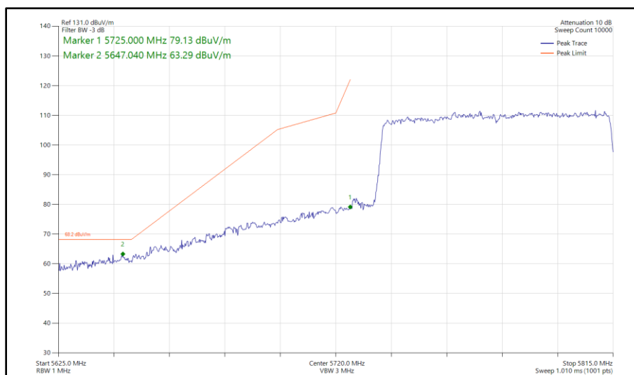
Figure 541 - 802.11ax HE80, SU, SDM, Core 0 - Core 1 - 5775 MHz Band Edge Frequency 5725 MHz
