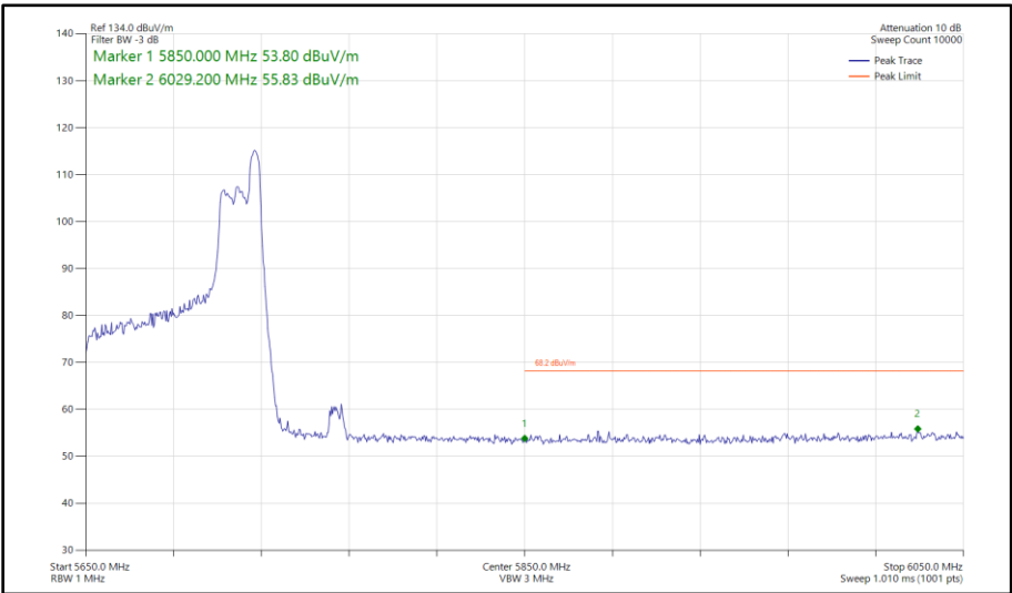
Figure 534 - 802.11ax HE80, RU 52-52, CDD, Core 0 - Core 1 - 5690 MHz Band Edge Frequency 5850 MHz
