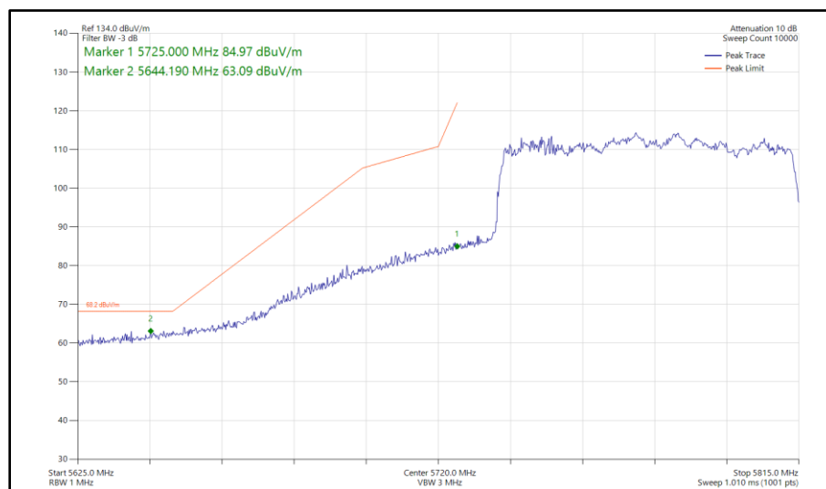
Figure 553 - 802.11ac VHT80, TxBF, Core 0 - Core 1 - 5775 MHz Band Edge Frequency 5725 MHz
