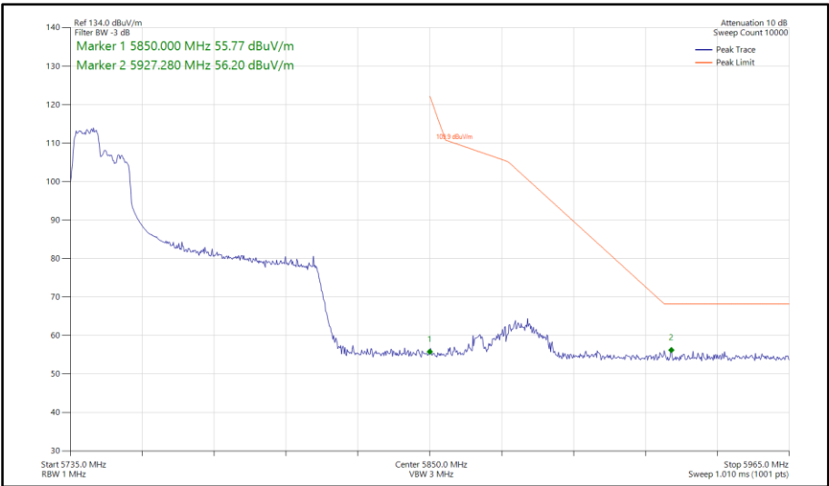
Figure 521 - 802.11ax HE80, RU 106-53, SISO, Core 1 - 5775 MHz Band Edge Frequency 5850 MHz
