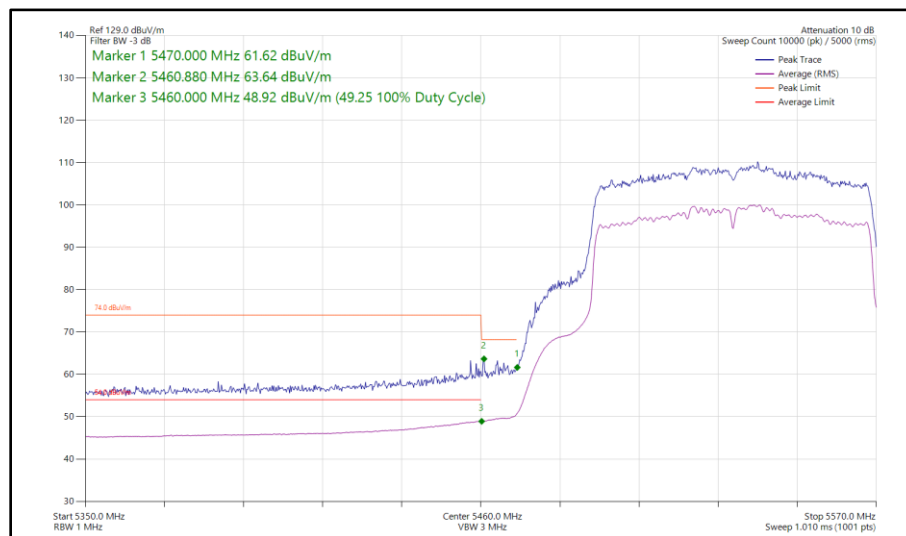
Figure 552 - 802.11ac VHT80, TxBF, Core 0 - Core 1 - 5530 MHz Band Edge Frequency 5470 MHz
