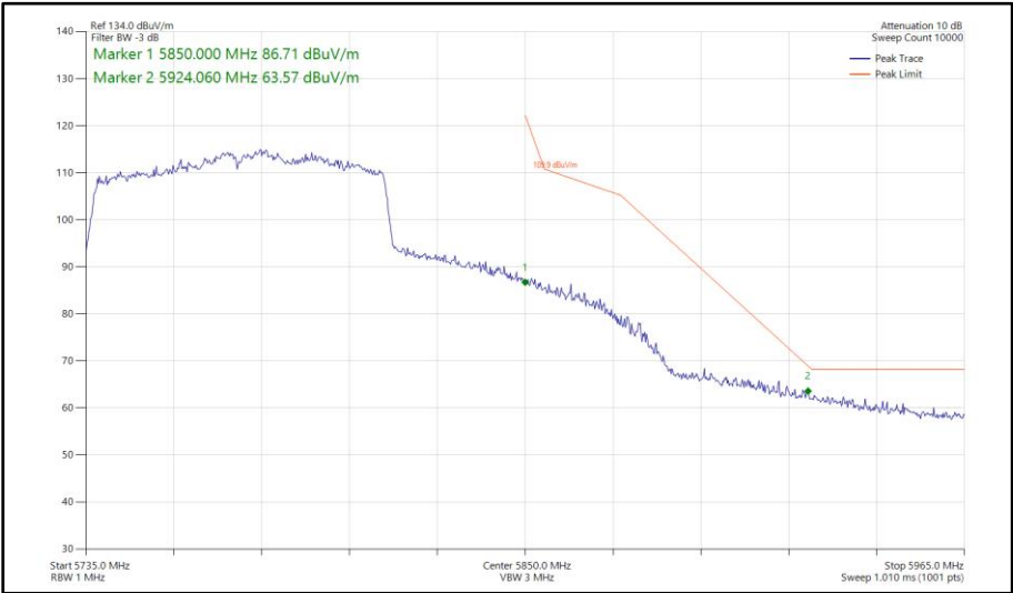
Figure 556 - 802.11ac VHT80, TxBF, Core 0 - Core 1 - 5775 MHz Band Edge Frequency 5850 MHz
