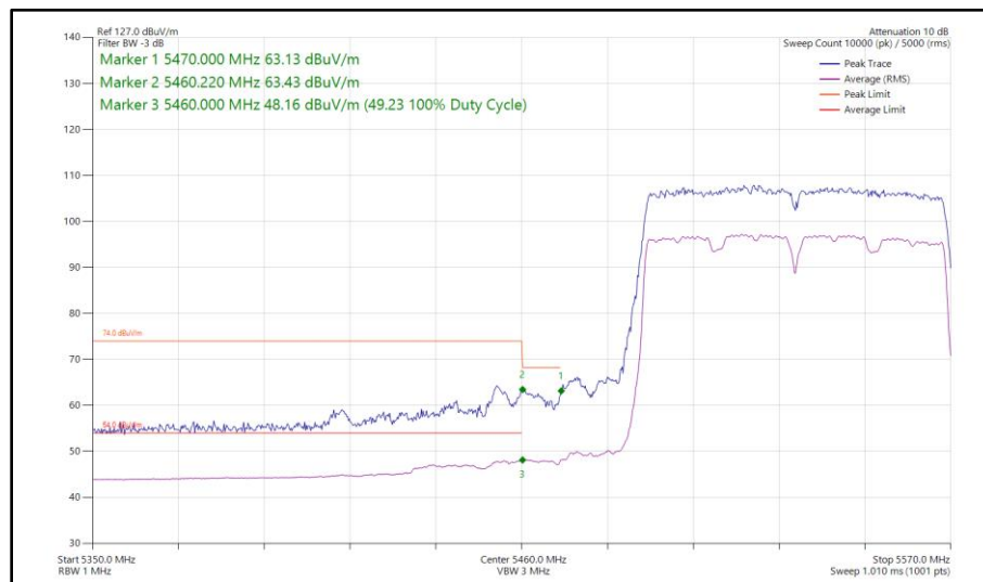
Figure 522 - 802.11ac VHT80, CDD, Core 0 - Core 1 - 5530 MHz Band Edge Frequency 5470 MHz
