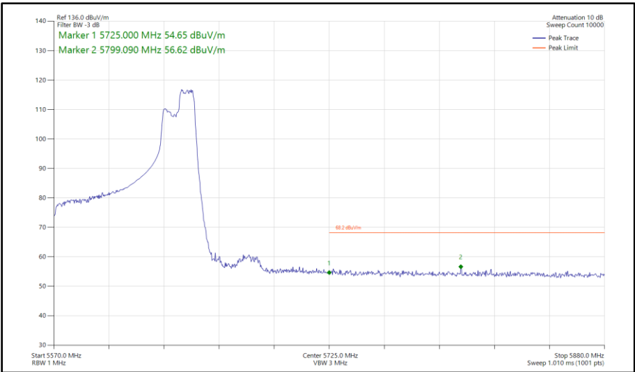
Figure 515 - 802.11ax HE80, RU 106-60, SISO, Core 1 - 5610 MHz Band Edge Frequency 5725 MHz
