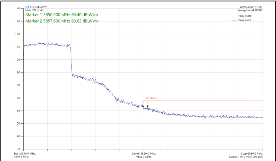
Figure 548 - 802.11ax HE80, SU, SDM, Core 0 - Core 1 - 5690 MHz Band Edge Frequency 5850 MHz
