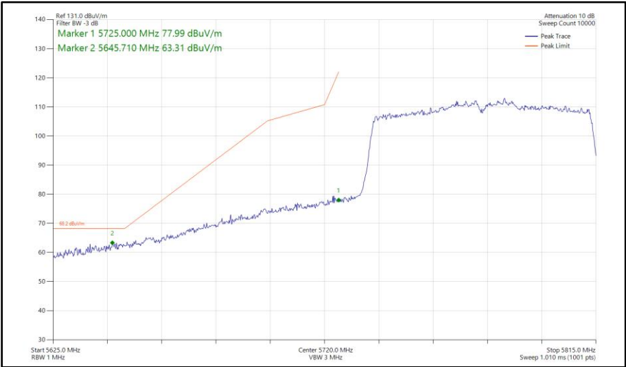
Figure 510 - 802.11ac VHT80, SISO, Core 1 - 5775 MHz Band Edge Frequency 5725 MHz
