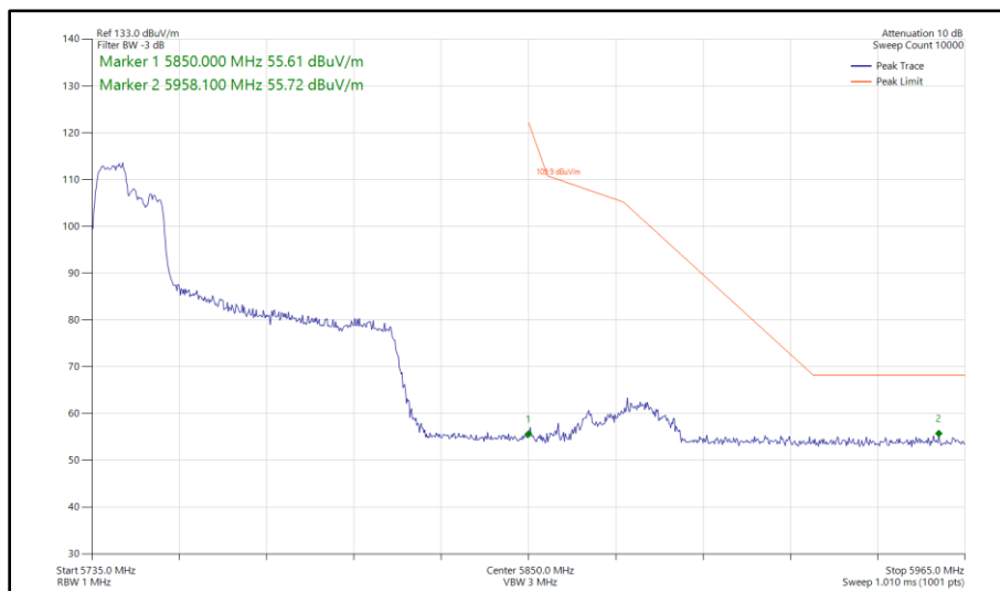
Figure 551 - 802.11ax HE80, RU 106-53, SDM, Core 0 - Core 1 - 5775 MHz Band Edge Frequency 5850 MHz
