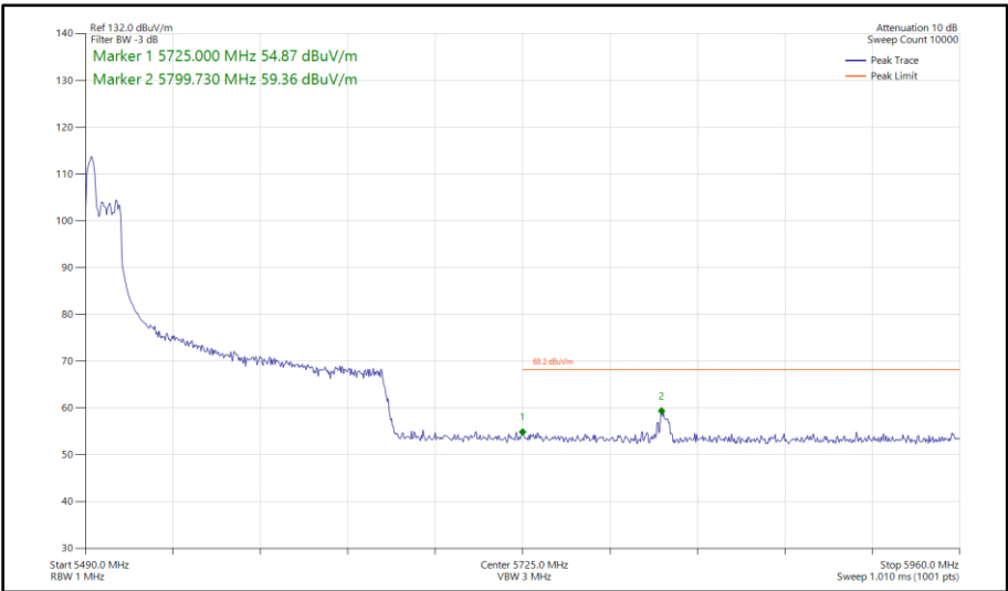
Figure 580 - 802.11ax HE160, RU 52-37P, SDM, Core 0 - Core 1 - 5570 MHz Band Edge Frequency 5725 MHz
