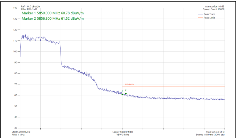
Figure 555 - 802.11ac VHT80, TxBF, Core 0 - Core 1 - 5690 MHz Band Edge Frequency 5850 MHz
