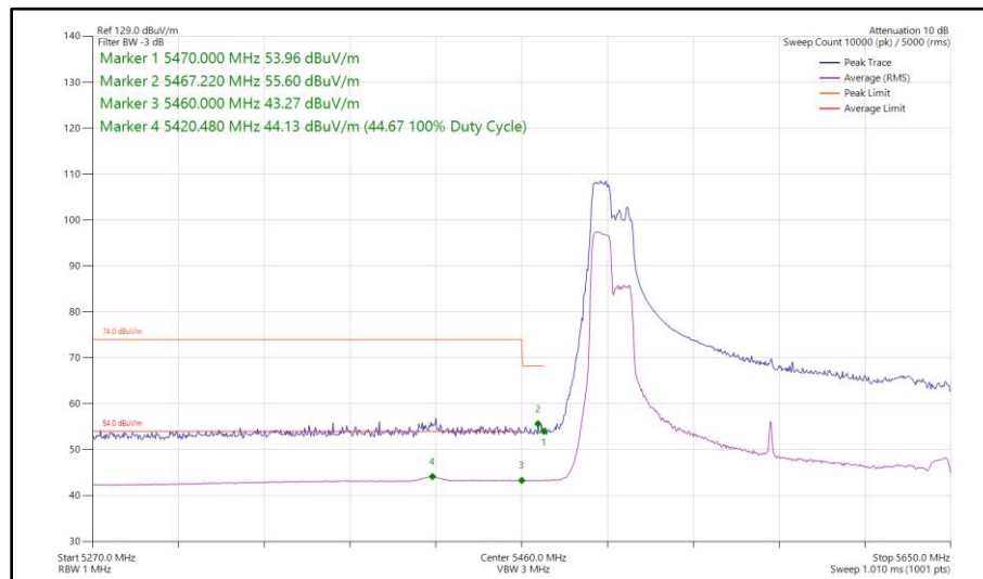
Figure 559 - 802.11ax HE160, RU 106-53P, SISO, Core 0 - 5570 MHz Band Edge Frequency 5470 MHz
