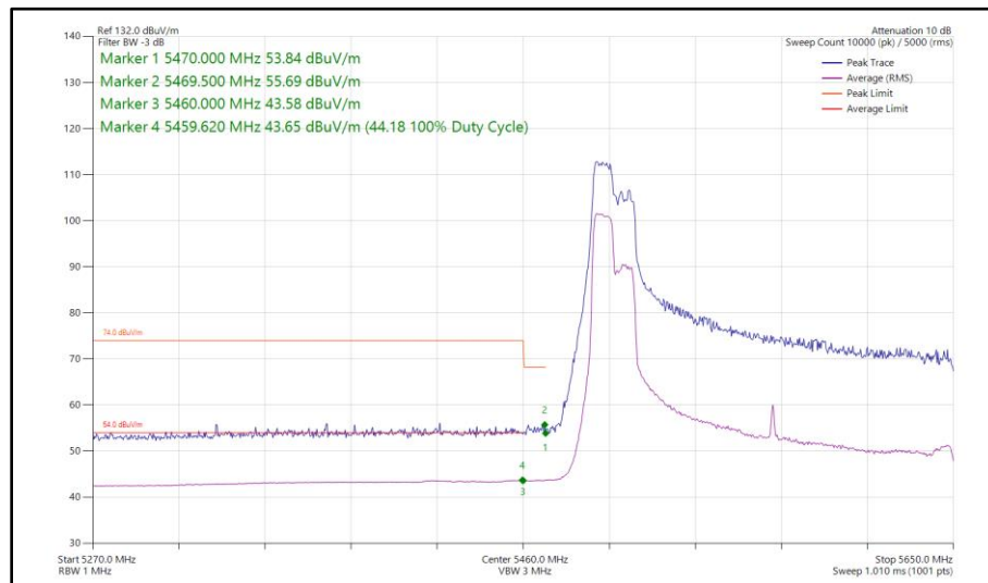
Figure 571 - 802.11ax HE160, RU 106-53P, CDD, Core 0 - Core 1 - 5570 MHz Band Edge Frequency 5470 MHz
