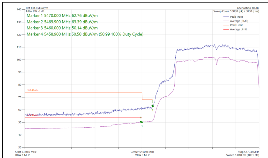
Figure 507 - 802.11ac VHT80, SISO, Core 1 - 5530 MHz Band Edge Frequency 5470 MHz
