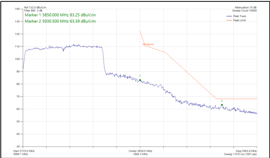
Figure 547 - 802.11ac VHT80, SDM, Core 0 - Core 1 - 5775 MHz Band Edge Frequency 5850 MHz
