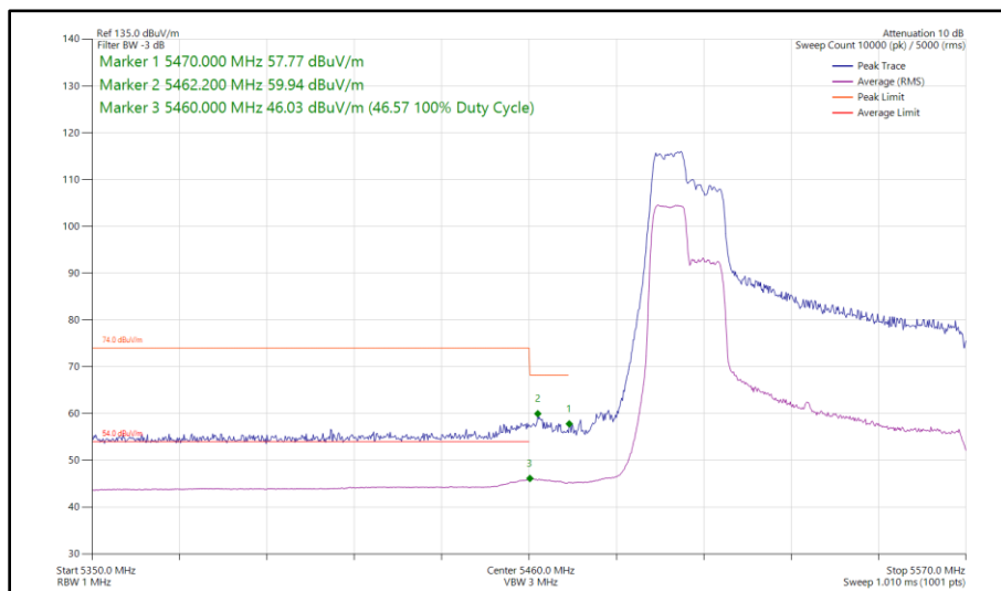
Figure 524 - 802.11ax HE80, RU 106-53, CDD, Core 0 - Core 1 - 5530 MHz Band Edge Frequency 5470 MHz
