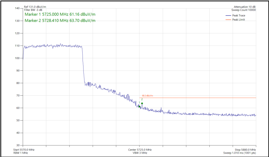
Figure 529 - 802.11ax HE80, SU, CDD, Core 0 - Core 1 - 5610 MHz Band Edge Frequency 5725 MHz
