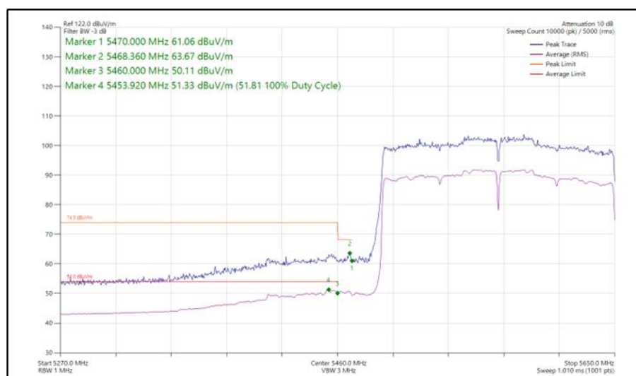
Figure 558 - 802.11ax HE160, SU, SISO, Core 0 - 5570 MHz Band Edge Frequency 5470 MHz
