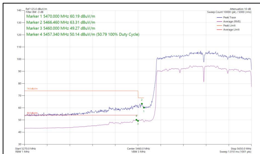
Figure 576 - 802.11ax HE160, SU, SDM, Core 0 - Core 1 - 5570 MHz Band Edge Frequency 5470 MHz
