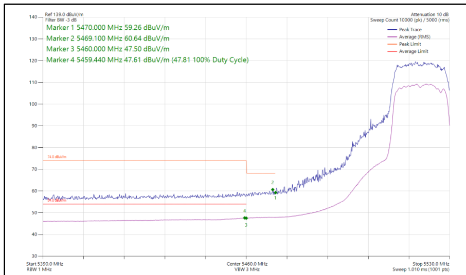
Figure 402 - 802.11ac VHT20, TxBF, Core 0 - Core 1 - 5520 MHz Band Edge Frequency 5470 MHz
