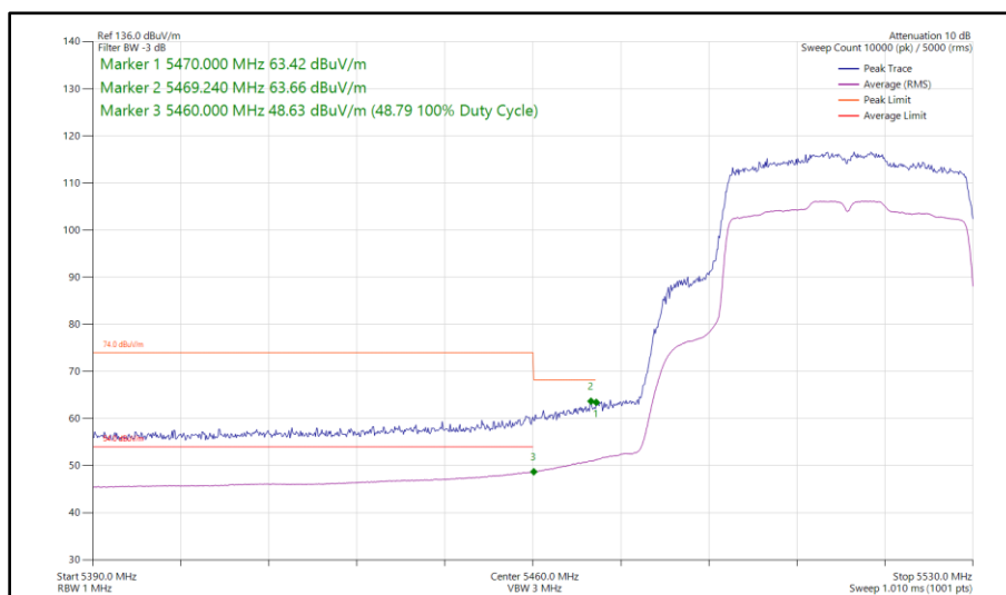
Figure 433 - 802.11ax HE40, SU, SISO, Core 1 - 5510 MHz Band Edge Frequency 5470 MHz
