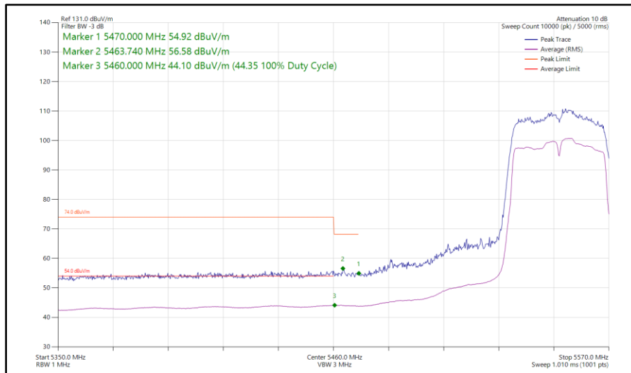
Figure 411 - 802.11n HT40, SISO, Core 0 - 5550 MHz Band Edge Frequency 5470 MHz
