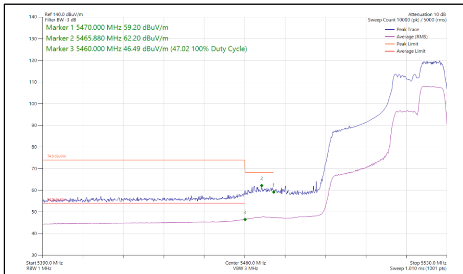
Figure 434 - 802.11ax HE40, RU 106-56, SISO, Core 1 - 5510 MHz Band Edge Frequency 5470 MHz
