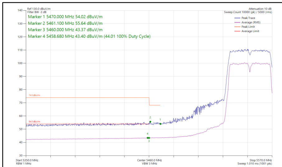
Figure 453 - 802.11n HT40, CDD, Core 0 - Core 1 - 5550 MHz Band Edge Frequency 5470 MHz
