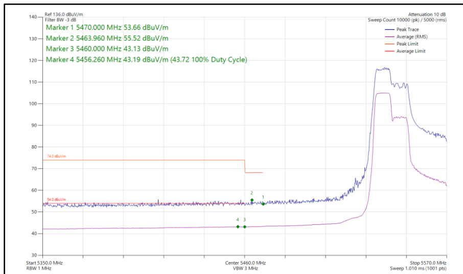
Figure 436 - 802.11ax HE40, RU 106-53, SISO, Core 1 - 5550 MHz Band Edge Frequency 5470 MHz
