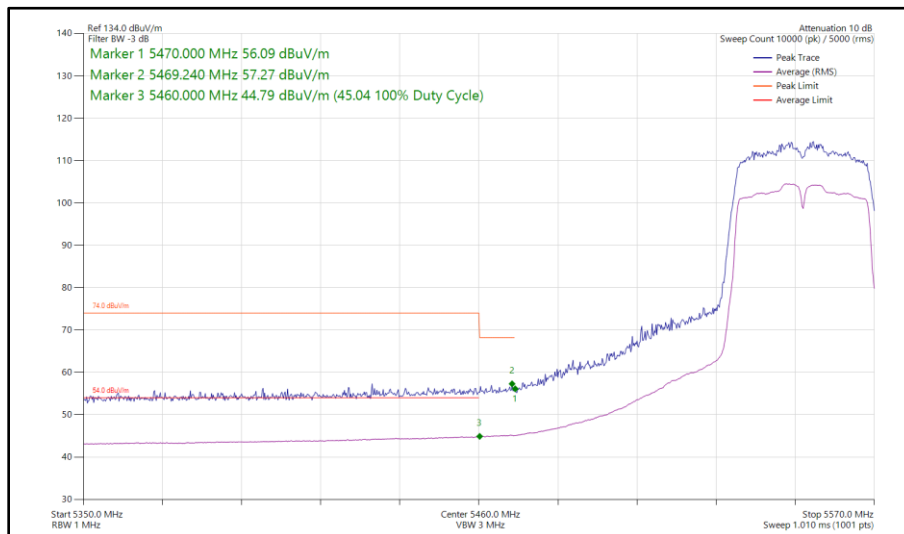
Figure 432 - 802.11n HT40, SISO, Core 1 - 5550 MHz Band Edge Frequency 5470 MHz
