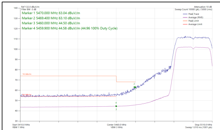
Figure 317 - 802.11n HT20, SISO, Core 0 - 5500 MHz Band Edge Frequency 5470 MHz
