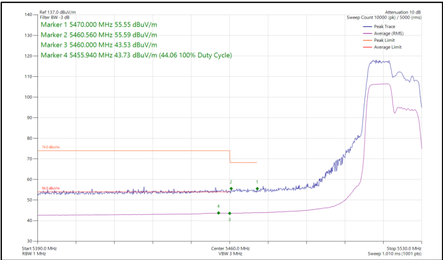
Figure 350 - 802.11ax HE20, RU 106-53, SISO, Core 1 - 5520 MHz Band Edge Frequency 5470 MHz
