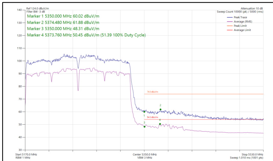
Figure 209 - 802.11ac VHT160, SDM, Core 0 - Core 1 - 5250 MHz Band Edge Frequency 5350 MHz
