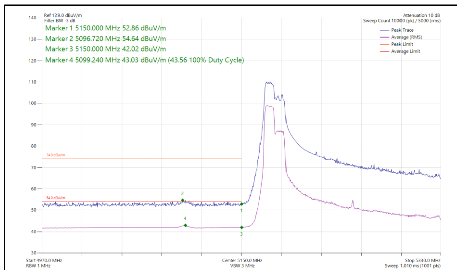
Figure 181 - 802.11ax HE160, RU 106-53P, SISO, Core 0 - 5250 MHz Band Edge Frequency 5150 MHz
