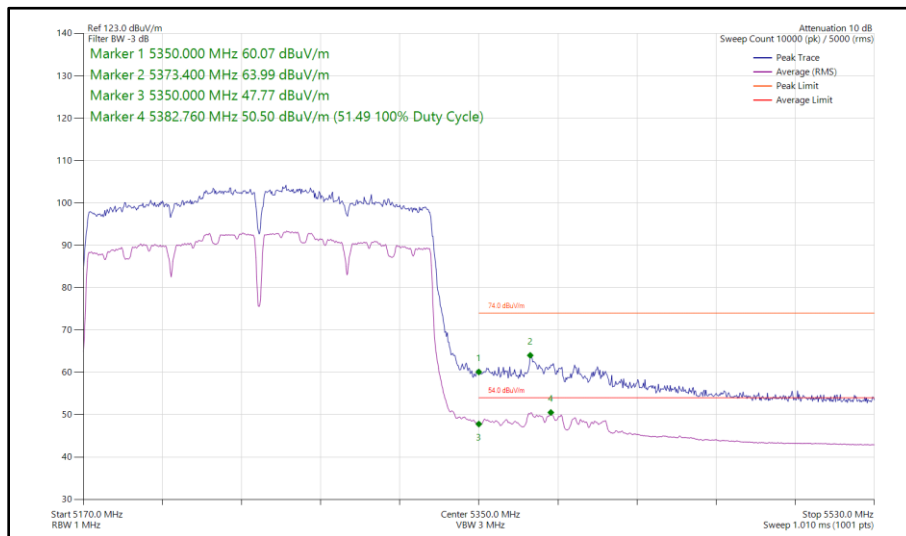
Figure 182 - 802.11ac VHT160, SISO, Core 0 - 5250 MHz Band Edge Frequency 5350 MHz
