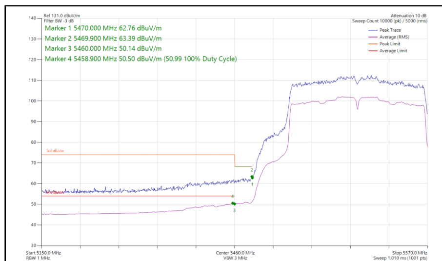
Figure 155 - 802.11ac VHT80, SISO, Core 1 - 5530 MHz Band Edge Frequency 5460 MHz
