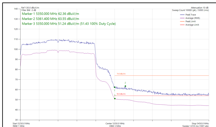
Figure 162 - 802.11ax HE80, SU, CDD, Core 0 - Core 1 - 5290 MHz Band Edge Frequency 5350 MHz
