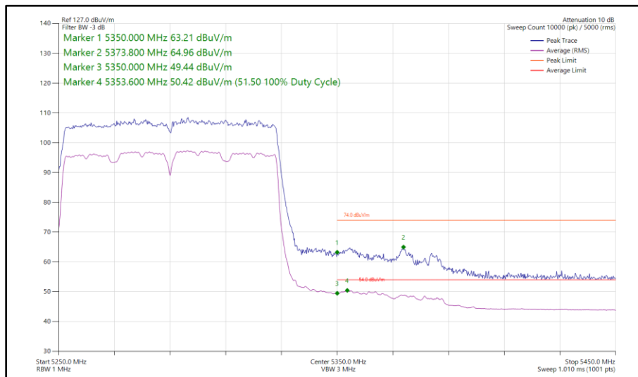
Figure 152 - 802.11ac VHT80, SISO, Core 1 - 5290 MHz Band Edge Frequency 5350 MHz
