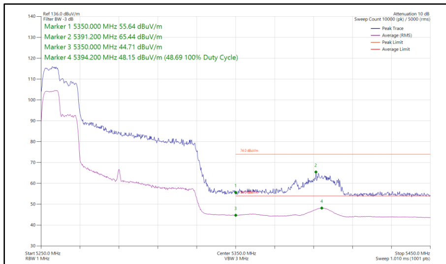
Figure 163 - 802.11ax HE80, RU 106-53, CDD, Core 0 - Core 1 - 5290 MHz Band Edge Frequency 5350 MHz
