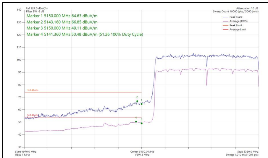
Figure 180 - 802.11ax HE160, SU, SISO, Core 0 - 5250 MHz Band Edge Frequency 5150 MHz
