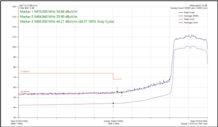
Figure 88 - 802.11ax HE40, SU, SISO, Core 0 - 5550 MHz Band Edge Frequency 5460 MHz
