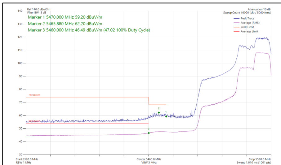
Figure 104 - 802.11ax HE40, RU 106-56, SISO, Core 1 - 5510 MHz Band Edge Frequency 5460 MHz
