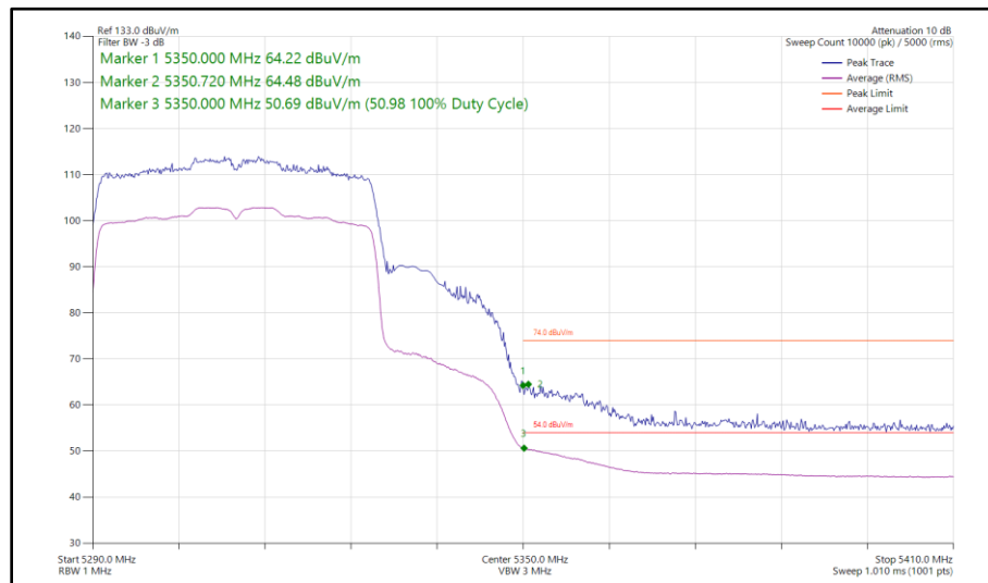
Figure 82 - 802.11ax HE40, SU, SISO, Core 0 - 5310 MHz Band Edge Frequency 5350 MHz
