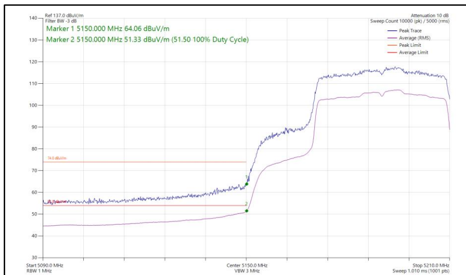
Figure 92 - 802.11ax HE40, SU, SISO, Core 1 - 5190 MHz Band Edge Frequency 5150 MHz
