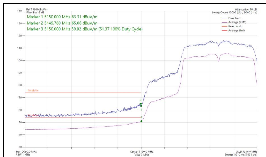
Figure 107 - 802.11n HT40, CDD, Core 0 - Core 1 - 5190 MHz Band Edge Frequency 5150 MHz
