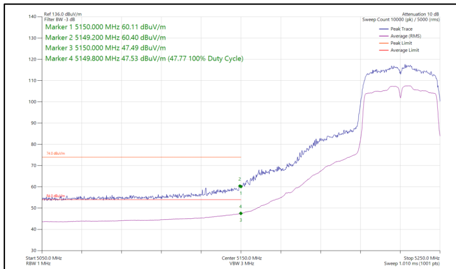
Figure 91 - 802.11n HT40, SISO, Core 1 - 5230 MHz Band Edge Frequency 5150 MHz
