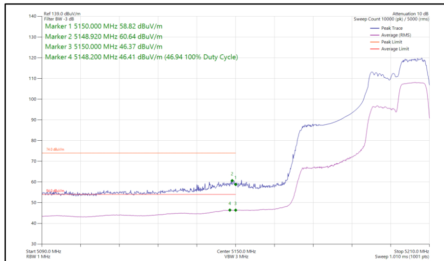
Figure 93 - 802.11ax HE40, RU 106-56, SISO, Core 1 - 5190 MHz Band Edge Frequency 5150 MHz
