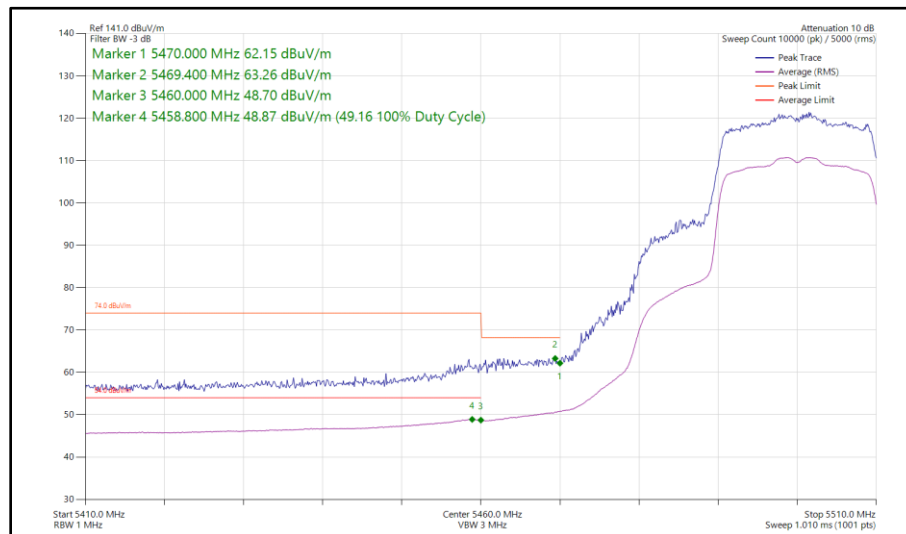
Figure 65 - 802.11ax HE20, SU, SDM, Core 0 - Core 1 - 5500 MHz Band Edge Frequency 5460 MHz
