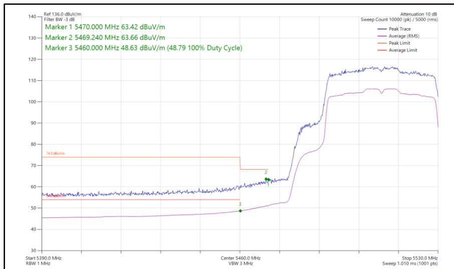
Figure 103 - 802.11ax HE40, SU, SISO, Core 1 - 5510 MHz Band Edge Frequency 5460 MHz
