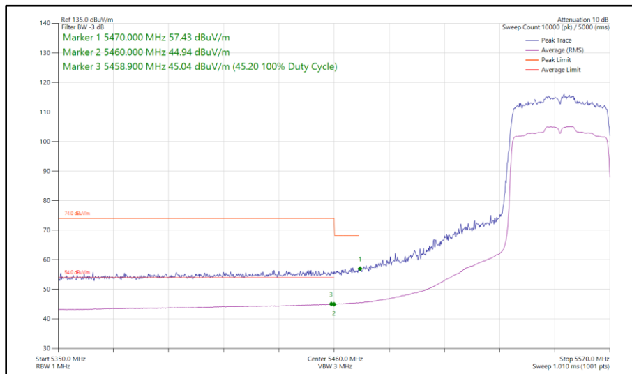
Figure 105 - 802.11ax HE40, SU, SISO, Core 1 - 5550 MHz Band Edge Frequency 5460 MHz
