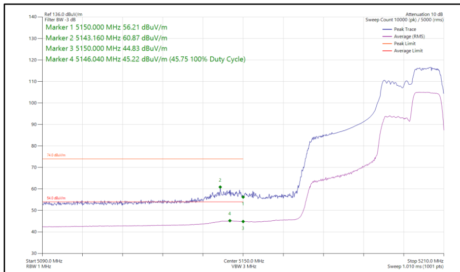
Figure 76 - 802.11ax HE40, RU 106-56, SISO, Core 0 - 5190 MHz Band Edge Frequency 5150 MHz
