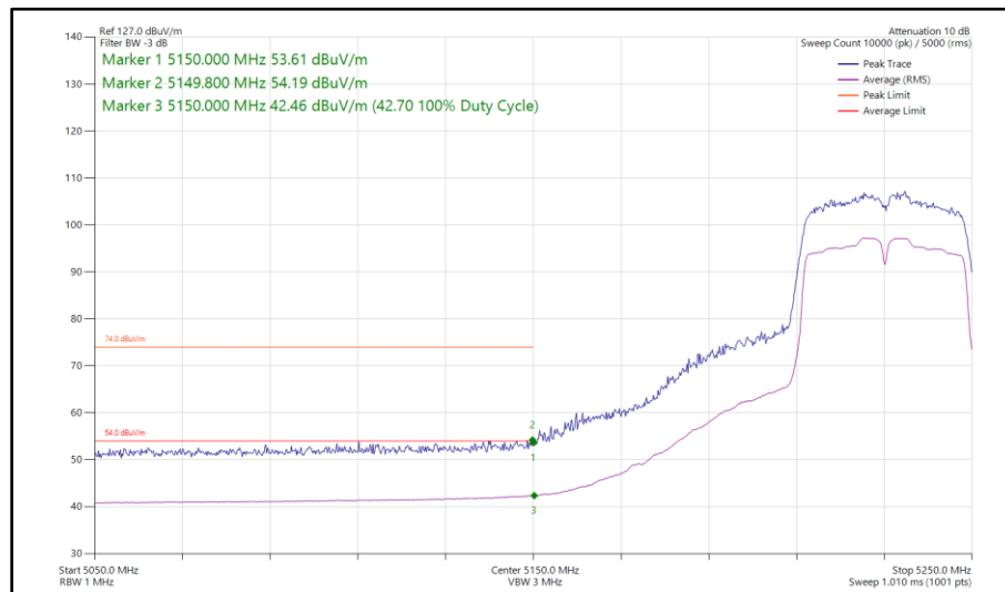
Figure 74 - 802.11n HT40, SISO, Core 0 - 5230 MHz Band Edge Frequency 5150 MHz
