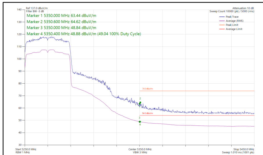
Figure 97 - 802.11ax HE40, SU, SISO, Core 1 - 5270 MHz Band Edge Frequency 5350 MHz
