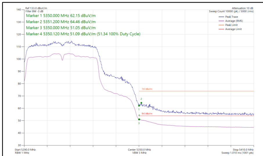
Figure 114 - 802.11n HT40, CDD, Core 0 - Core 1 - 5310 MHz Band Edge Frequency 5350 MHz
