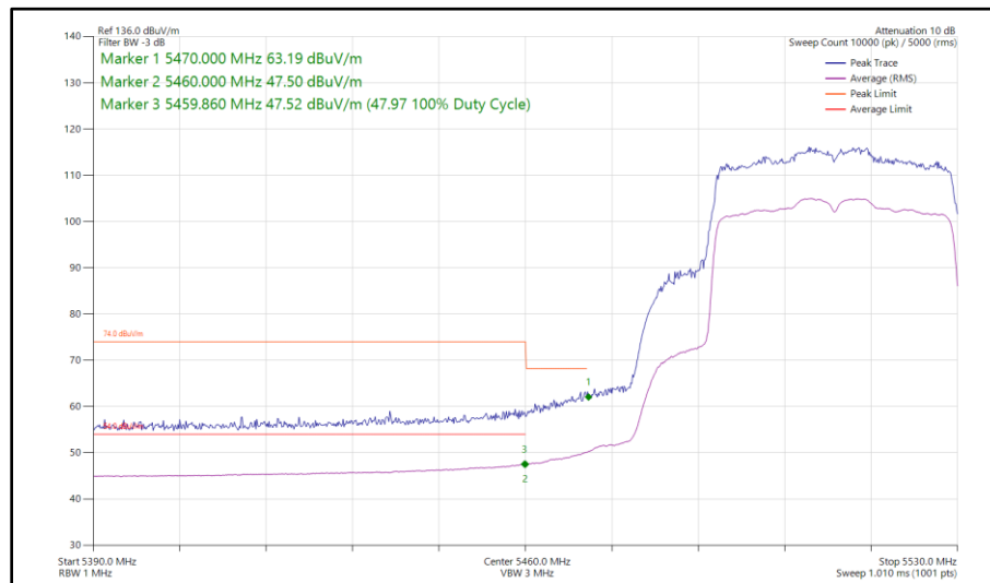
Figure 132 - 802.11ax HE40, SU, SDM, Core 0 - Core 1 - 5510 MHz Band Edge Frequency 5460 MHz
