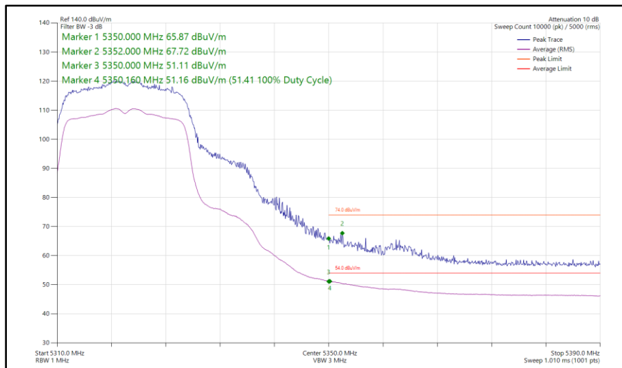
Figure 52 - 802.11n HT20, CDD, Core 0 - Core 1 - 5320 MHz Band Edge Frequency 5350 MHz
