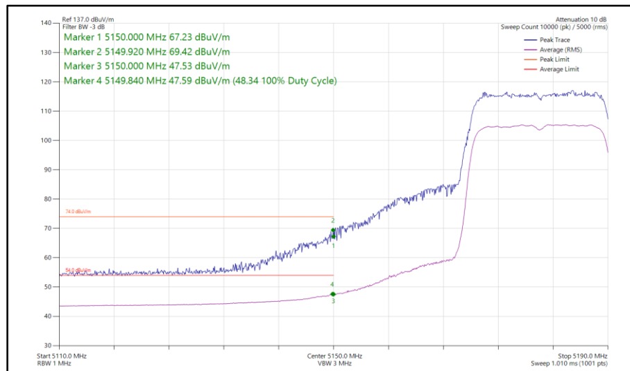
Figure 59 - 802.11ax HE20, SU, SDM, Core 0 - Core 1 - 5180 MHz Band Edge Frequency 5150 MHz
