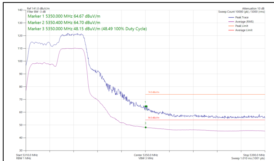
Figure 63 - 802.11ax HE20, RU 106-54, SDM, Core 0 - Core 1 - 5320 MHz Band Edge Frequency 5350 MHz
