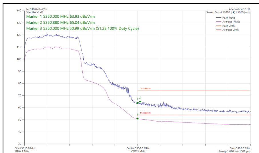
Figure 62 - 802.11ax HE20, SU, SDM, Core 0 - Core 1 - 5320 MHz Band Edge Frequency 5350 MHz
