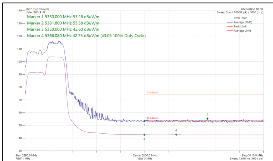
Figure 14 - 802.11ax HE20, RU 106-54, SISO, Core 0 - 5300 MHz Band Edge Frequency 5350 MHz
