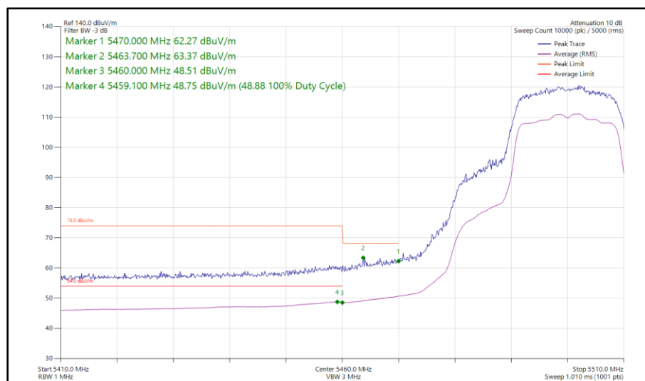
Figure 64 - 802.11n HT20, SDM, Core 0 - Core 1 - 5500 MHz Band Edge Frequency 5460 MHz
