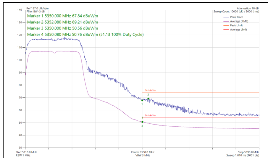
Figure 61 - 802.11n HT20, SDM, Core 0 - Core 1 - 5320 MHz Band Edge Frequency 5350 MHz
