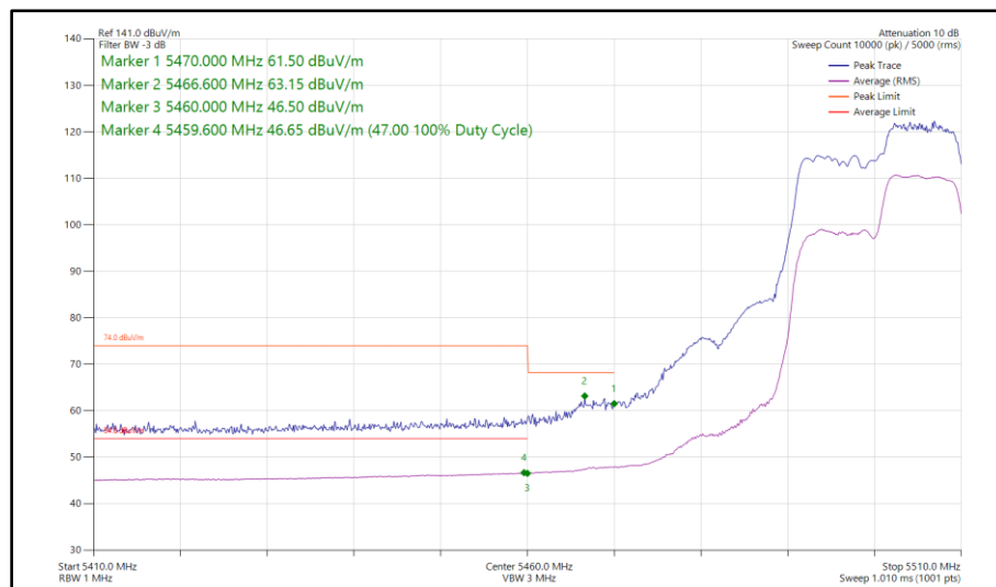
Figure 57 - 802.11ax HE20, RU 106-54, CDD, Core 0 - Core 1 - 5500 MHz Band Edge Frequency 5460 MHz
