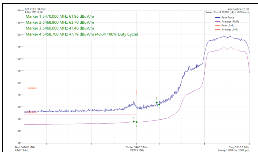
Figure 55 - 802.11n HT20, CDD, Core 0 - Core 1 - 5500 MHz Band Edge Frequency 5460 MHz
