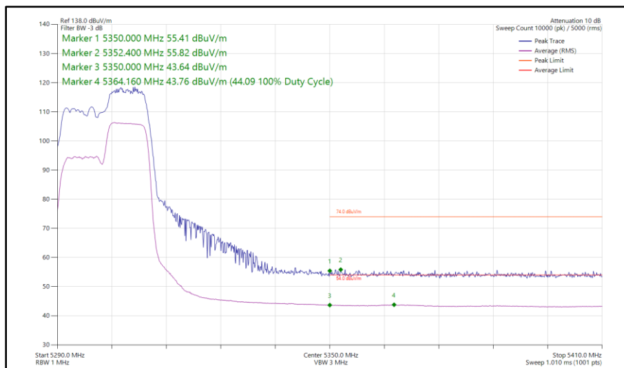
Figure 38 - 802.11ax HE20, RU 106-54, SISO, Core 1 - 5300 MHz Band Edge Frequency 5350 MHz
