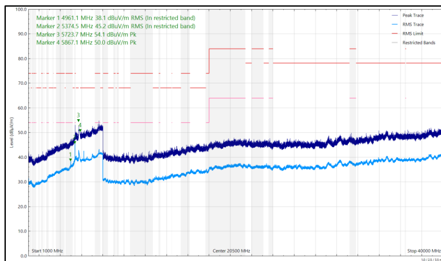
Figure 253 - 5788 MHz, HDR4, ePA, Core 0 + Core 1, 1 GHz to 40 GHz, Horizontal
