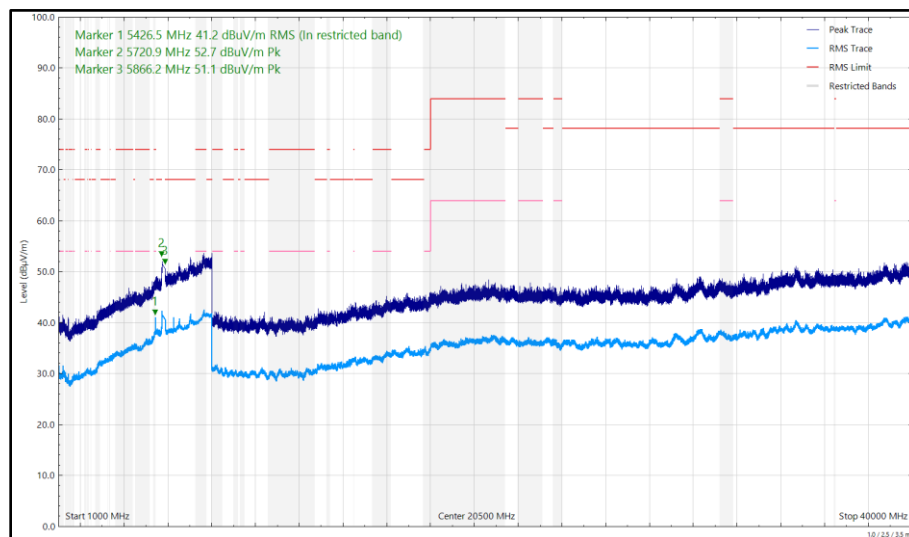
Figure 257 - 5844 MHz, HDR4, ePA, Core 0 + Core 1, 1 GHz to 40 GHz, Vertical
