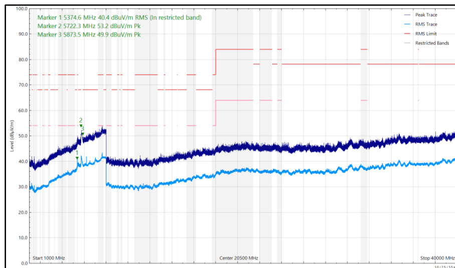
Figure 255 - 5788 MHz, HDR4, ePA, Core 0 + Core 1, 1 GHz to 40 GHz, Vertical
