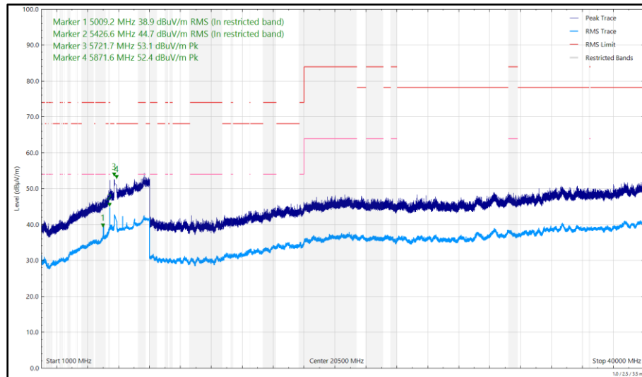
Figure 256 - 5844 MHz, HDR4, ePA, Core 0 + Core 1, 1 GHz to 40 GHz, Horizontal
