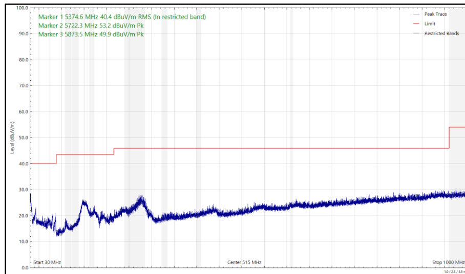
Figure 254 - 5788 MHz, HDR4, ePA, Core 0 + Core 1, 30 MHz to 1 GHz, Vertical (Peak)
