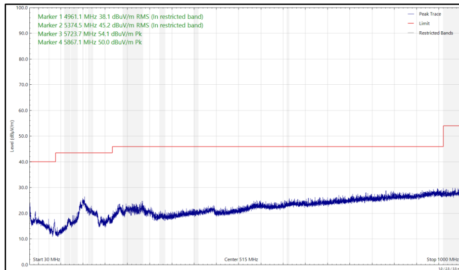
Figure 252 - 5788 MHz, HDR4, ePA, Core 0 + Core 1, 30 MHz to 1 GHz, Horizontal (Peak)
