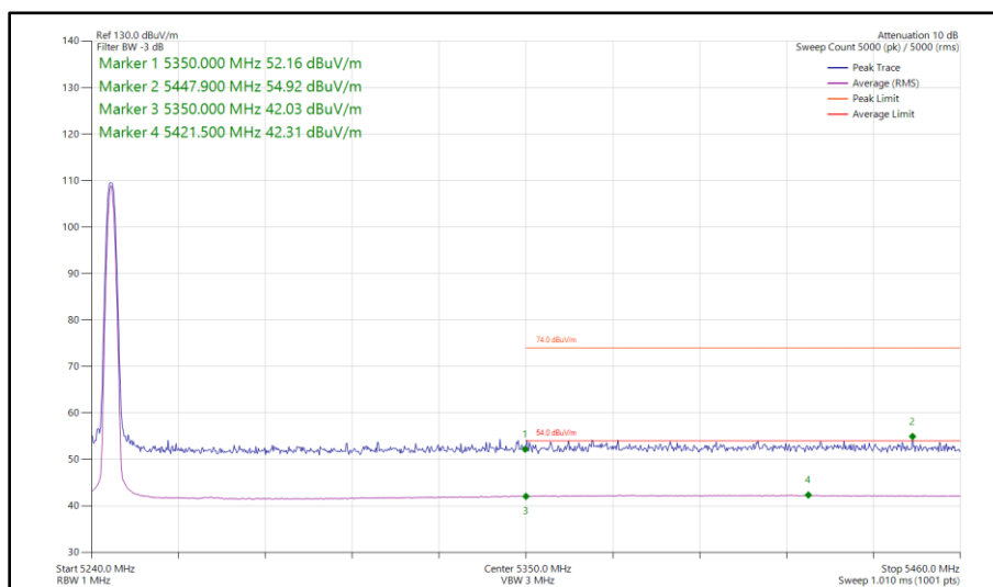
Figure 16 - Bluetooth DH5, MIMO, Core 0 - Core 1 - 5245 MHz Band Edge Frequency 5350 MHz
