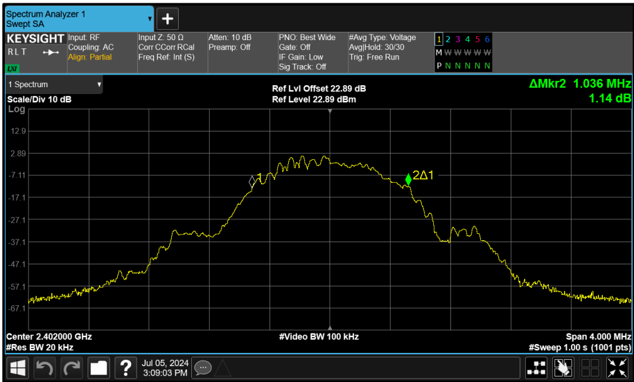
Figure 93 - Core 1 (B) 2402 MHz (CH37) 99% Bandwidth
