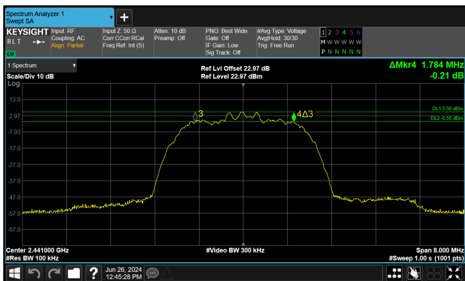
Figure 148 - Core 1 (B) 2441 MHz (CH39) 6 dB Bandwidth
