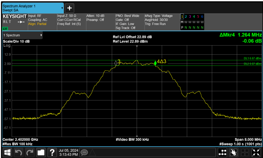
Figure 100 - Core 1 (B) 2402 MHz (CH37) 6 dB Bandwidth
