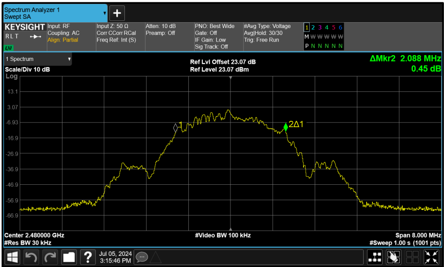
Figure 103 - Core 1 (B) 2480 MHz (CH39) 99% Bandwidth
