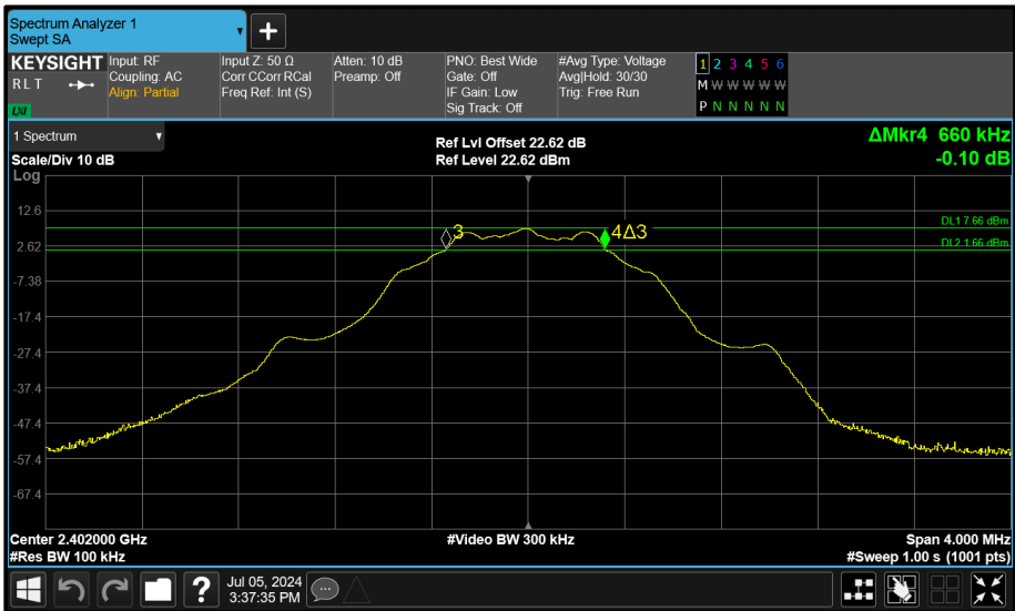
Figure 106 - Core 2 (C) 2402 MHz (CH37) 6 dB Bandwidth
