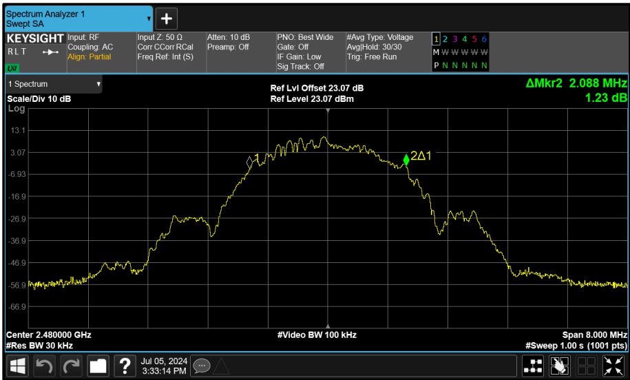
Figure 139 - Core 0 (A) 2480 MHz (CH39) 99% Bandwidth
