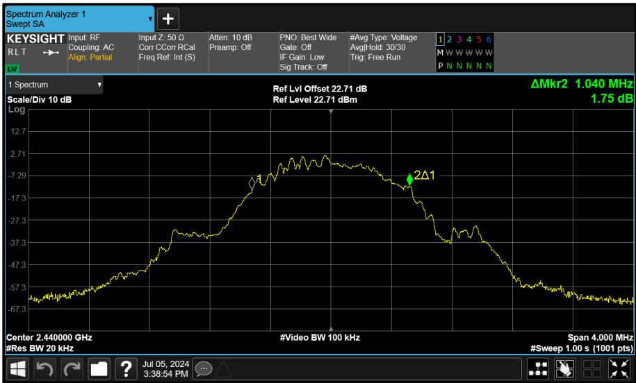
Figure 107 - Core 2 (C) 2440 MHz (CH17) 99% Bandwidth
