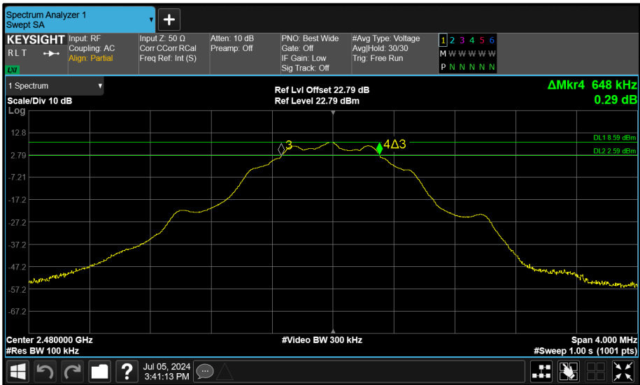
Figure 110 - Core 2 (C) 2480 MHz (CH39) 6 dB Bandwidth
