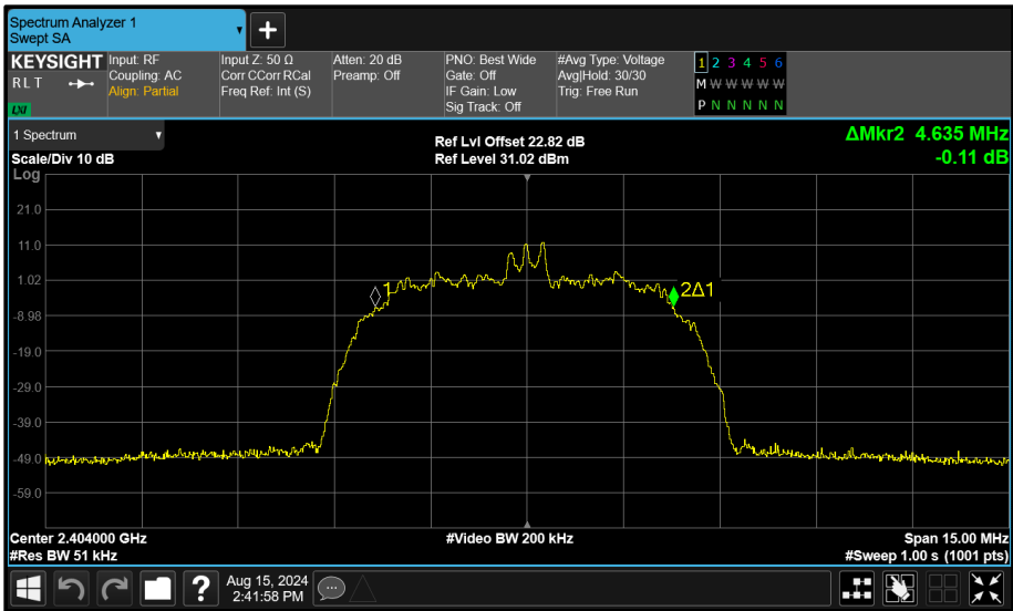
Figure 123 - Core 1 (B) 2404 MHz (CH2) 99% Bandwidth
