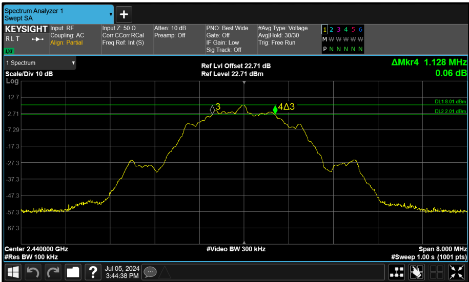
Figure 114 - Core 2 (C) 2440 MHz (CH17) 6 dB Bandwidth
