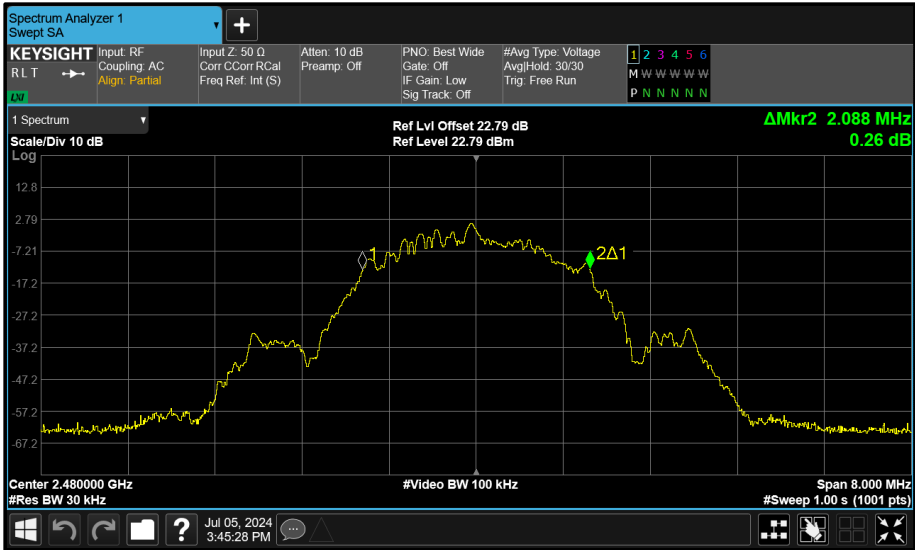
Figure 115 - Core 2 (C) 2480 MHz (CH39) 99% Bandwidth
