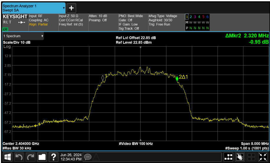
Figure 141 - Core 0 (A) 2404 MHz (CH2) 99% Bandwidth
