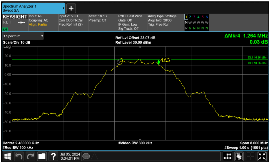
Figure 140 - Core 0 (A) 2480 MHz (CH39) 6 dB Bandwidth
