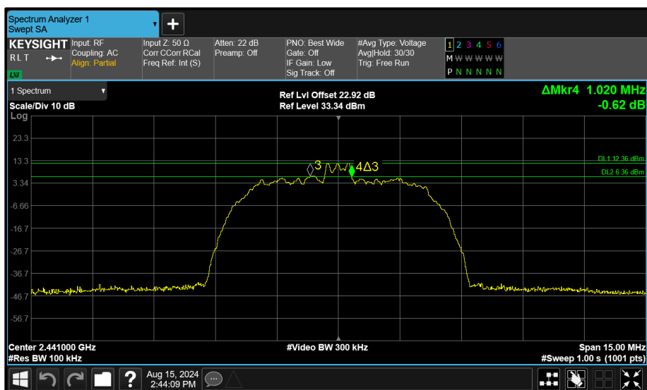
Figure 126 - Core 1 (B) 2441 MHz (CH39) 6 dB Bandwidth
