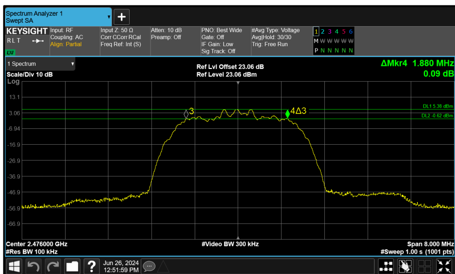
Figure 152 - Core 1 (B) 2476 MHz (CH74) 6 dB Bandwidth
