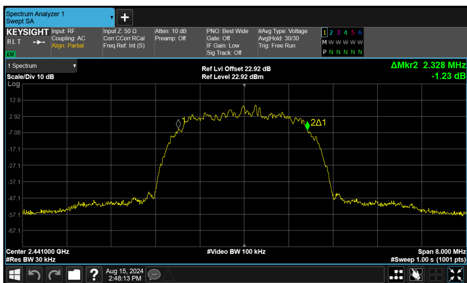
Figure 119 - Core 1 (B) 2441 MHz (CH39) 99% Bandwidth
