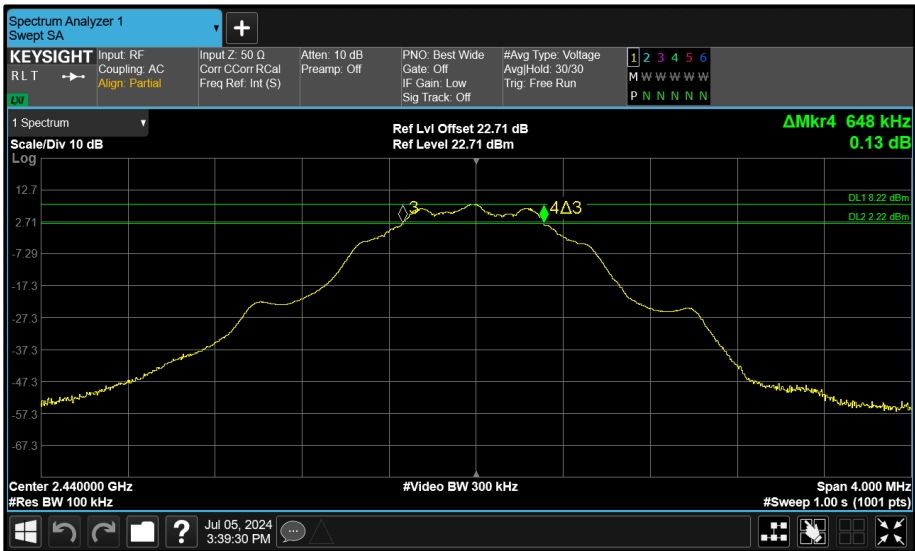
Figure 108 - Core 2 (C) 2440 MHz (CH17) 6 dB Bandwidth
