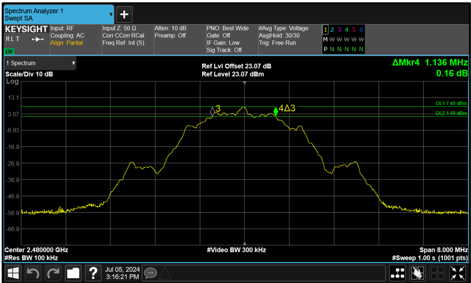
Figure 104 - Core 1 (B) 2480 MHz (CH39) 6 dB Bandwidth
