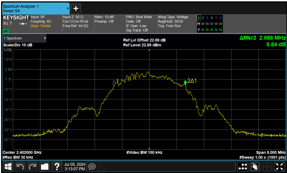
Figure 99 - Core 1 (B) 2402 MHz (CH37) 99% Bandwidth
