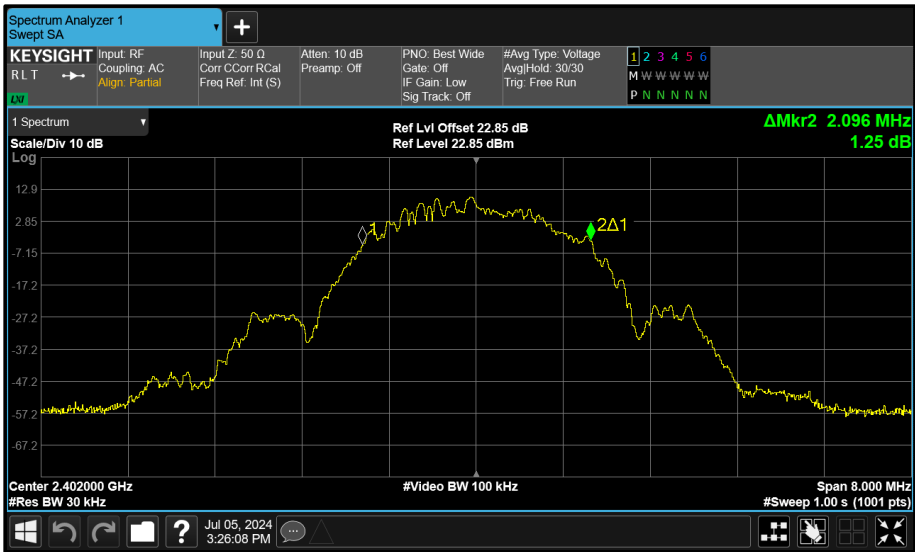
Figure 135 - Core 0 (A) 2402 MHz (CH37) 99% Bandwidth
