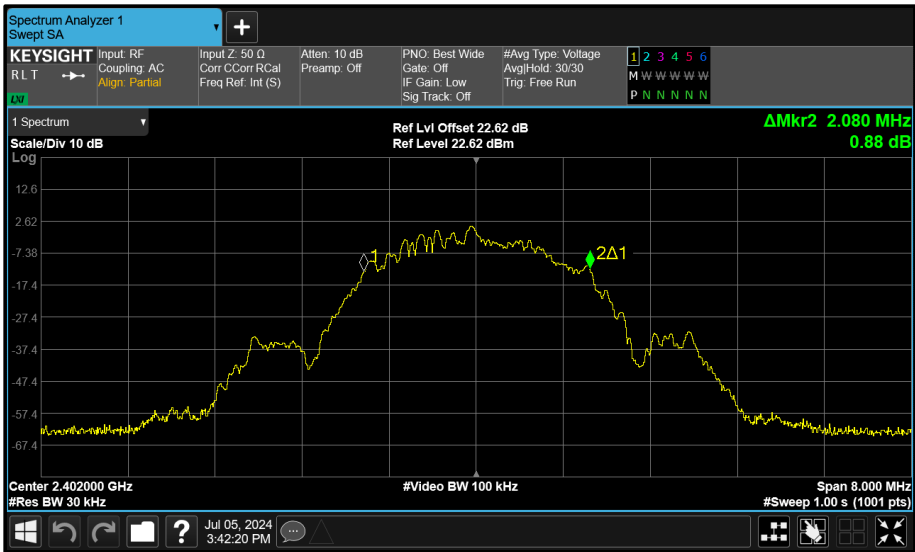
Figure 111 - Core 2 (C) 2402 MHz (CH37) 99% Bandwidth
