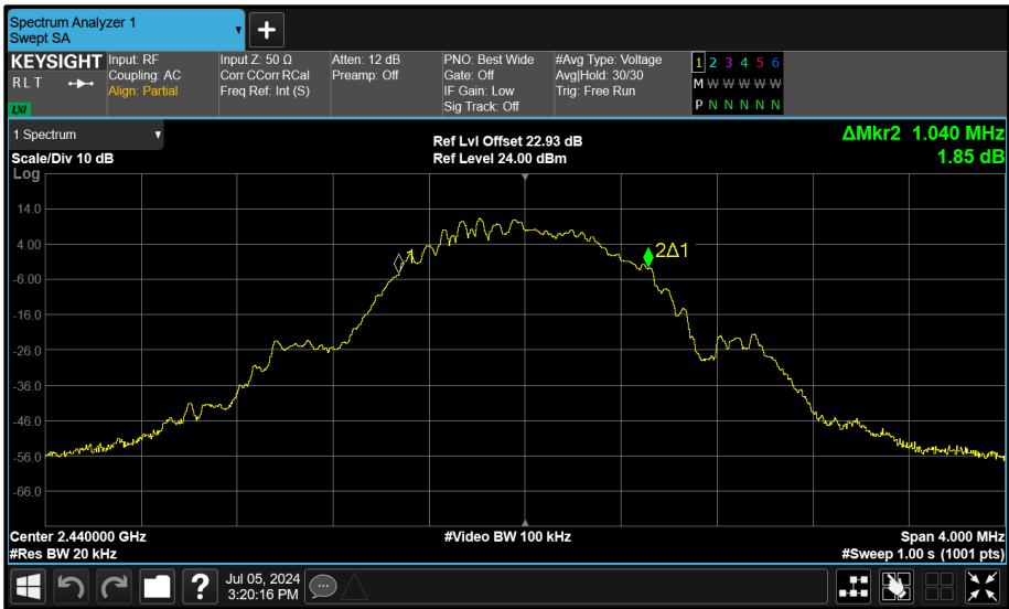
Figure 131 - Core 0 (A) 2440 MHz (CH17) 99% Bandwidth
