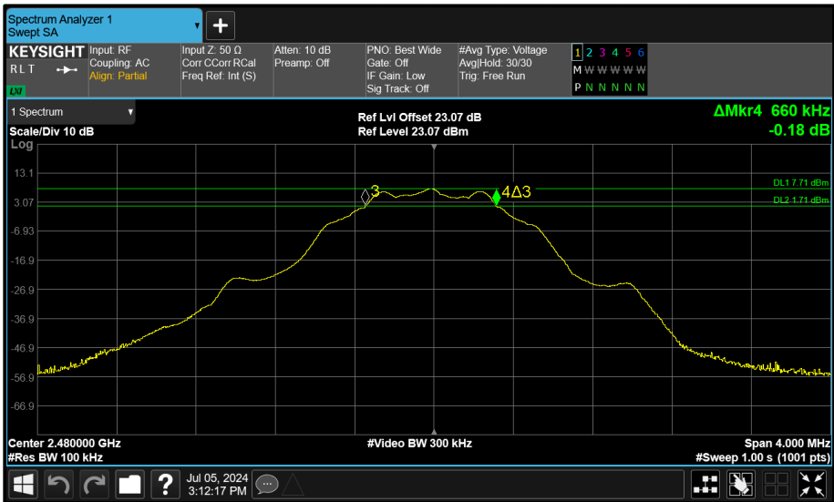
Figure 98 - Core 1 (B) 2480 MHz (CH39) 6 dB Bandwidth
