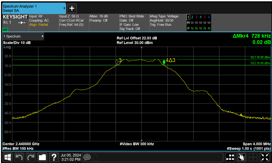
Figure 132 - Core 0 (A) 2440 MHz (CH17) 6 dB Bandwidth
