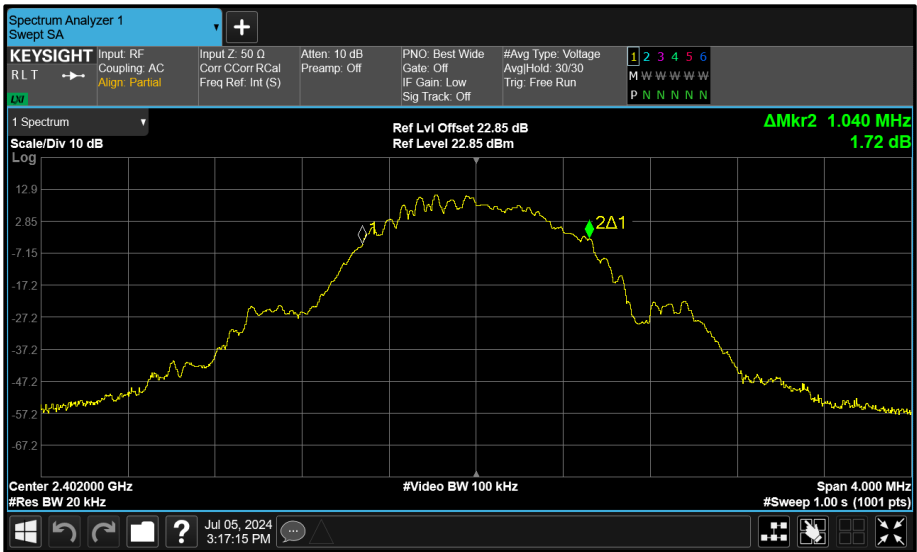
Figure 129 - Core 0 (A) 2402 MHz (CH37) 99% Bandwidth
