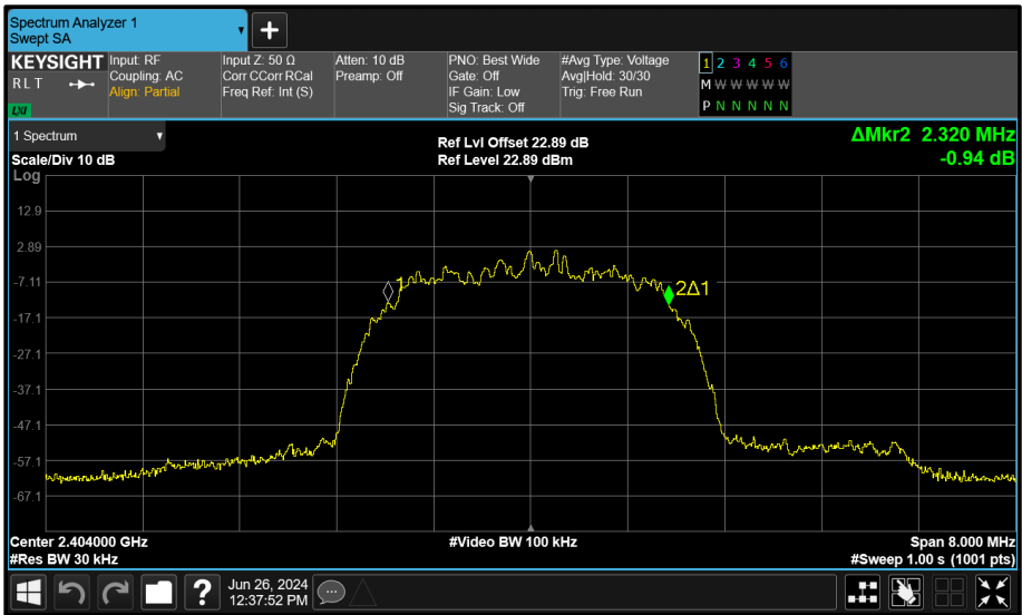
Figure 143 - Core 1 (B) 2404 MHz (CH2) 99% Bandwidth
