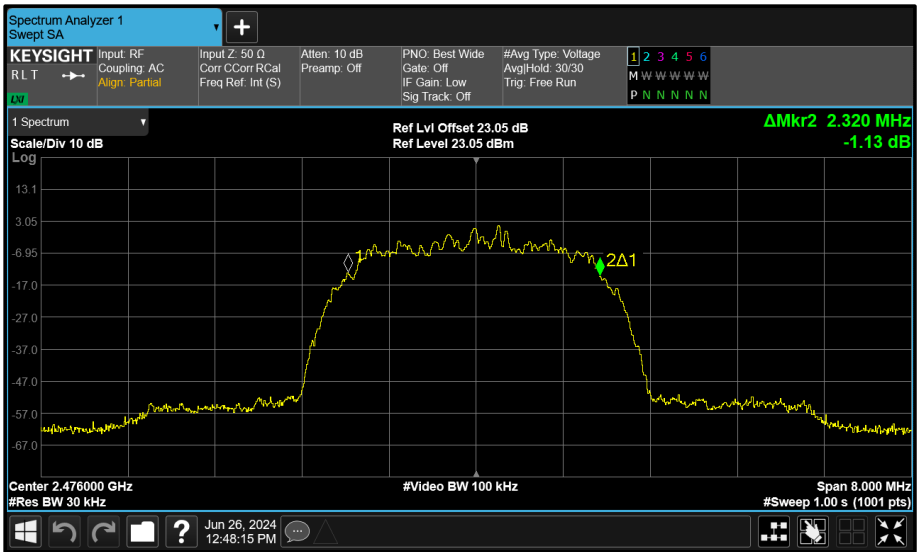
Figure 149 - Core 0 (A) 2476 MHz (CH74) 99% Bandwidth
