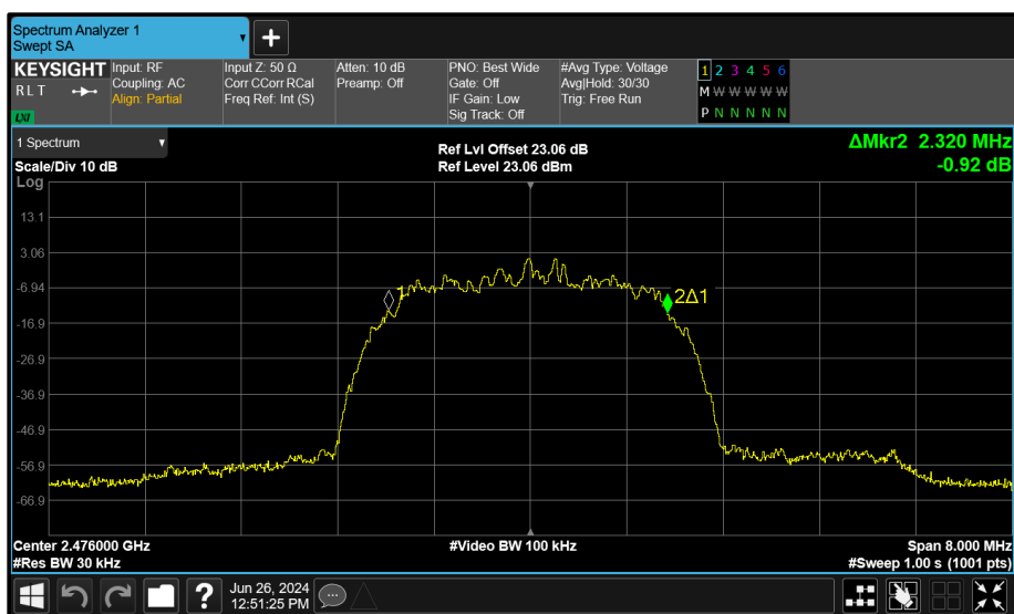
Figure 151 - Core 1 (B) 2476 MHz (CH74) 99% Bandwidth
