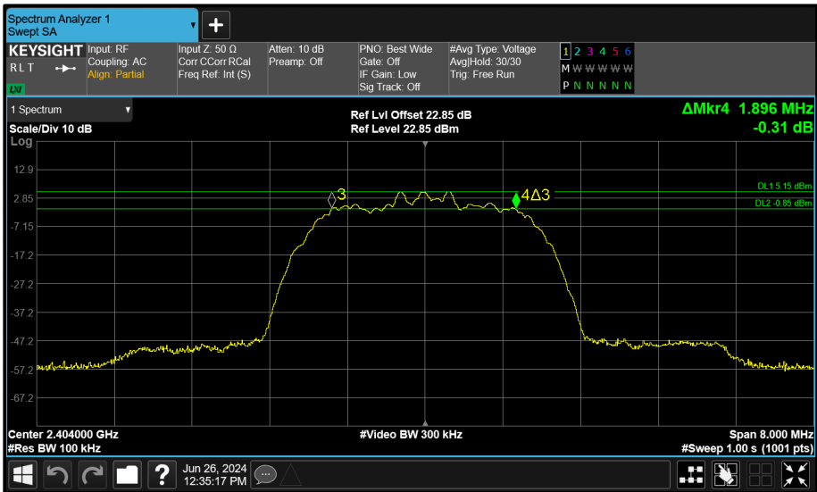
Figure 142 - Core 0 (A) 2404 MHz (CH2) 6 dB Bandwidth
