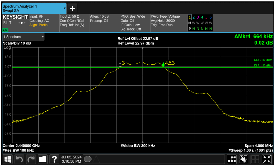
Figure 96 - Core 1 (B) 2440 MHz (CH17) 6 dB Bandwidth
