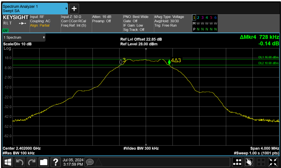
Figure 130 - Core 0 (A) 2402 MHz (CH37) 6 dB Bandwidth
