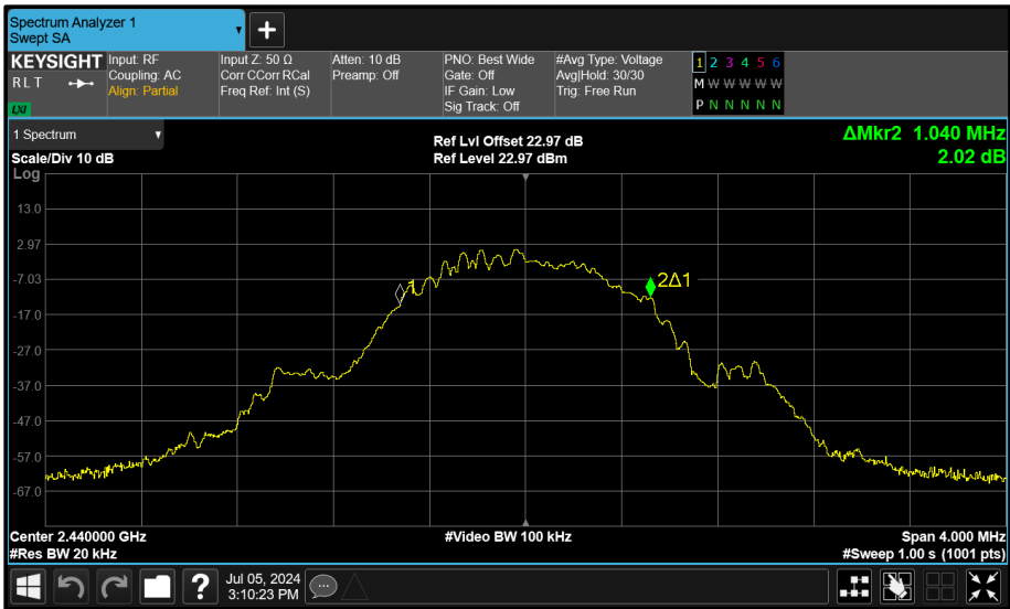
Figure 95 - Core 1 (B) 2440 MHz (CH17) 99% Bandwidth
