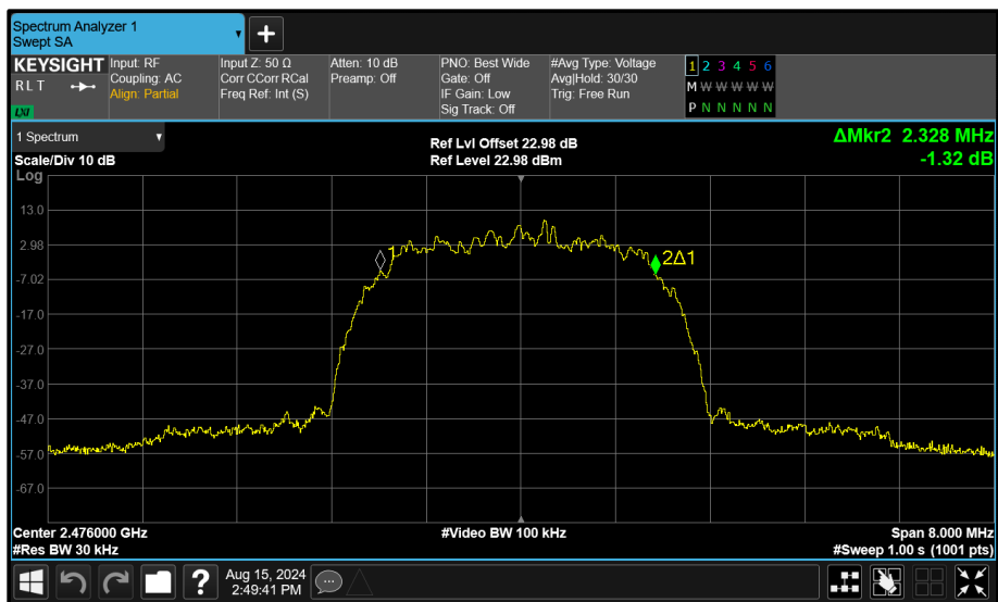
Figure 121 - Core 1 (B) 2476 MHz (CH74) 99% Bandwidth
