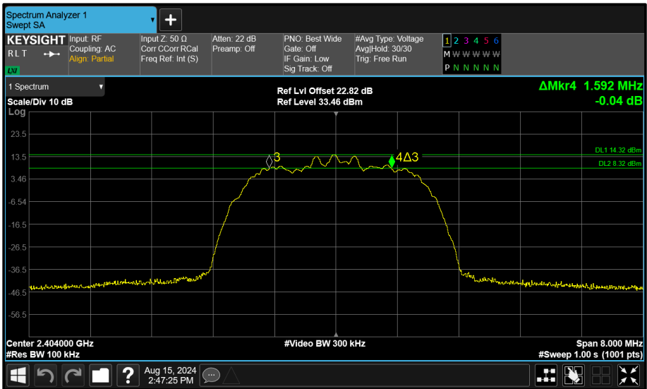
Figure 118 - Core 1 (B) 2404 MHz (CH2) 6 dB Bandwidth
