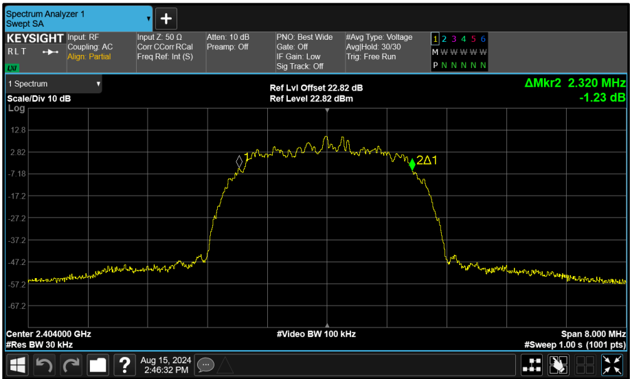
Figure 117 - Core 1 (B) 2404 MHz (CH2) 99% Bandwidth
