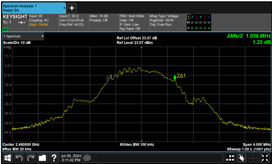
Figure 97 - Core 1 (B) 2480 MHz (CH39) 99% Bandwidth
