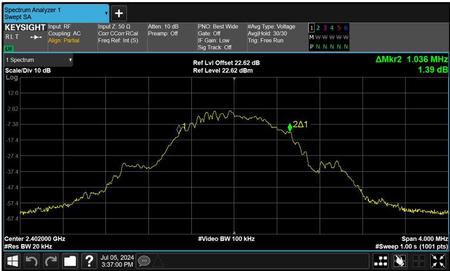
Figure 105 - Core 2 (C) 2402 MHz (CH37) 99% Bandwidth
