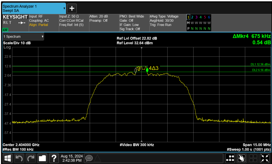
Figure 124 - Core 1 (B) 2404 MHz (CH2) 6 dB Bandwidth
