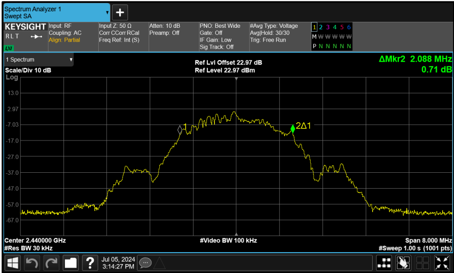
Figure 101 - Core 1 (B) 2440 MHz (CH17) 99% Bandwidth
