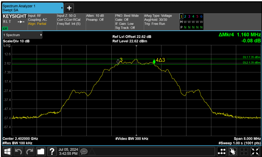
Figure 112 - Core 2 (C) 2402 MHz (CH37) 6 dB Bandwidth
