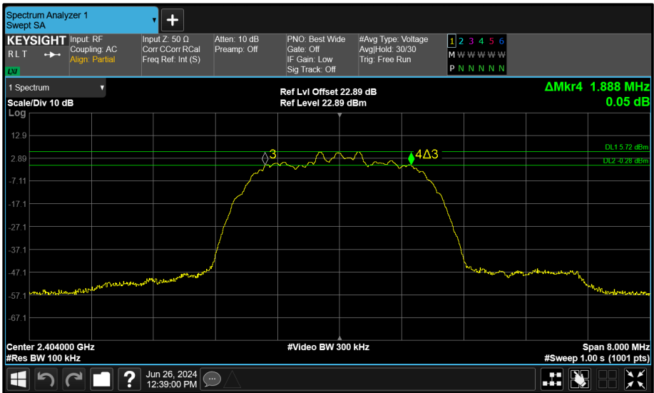
Figure 144 - Core 1 (B) 2404 MHz (CH2) 6 dB Bandwidth
