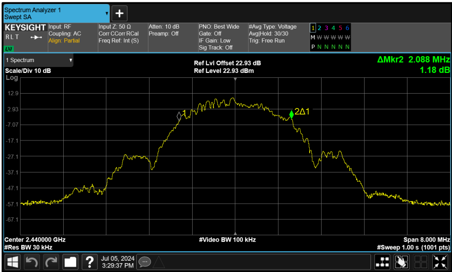
Figure 137 - Core 0 (A) 2440 MHz (CH17) 99% Bandwidth
