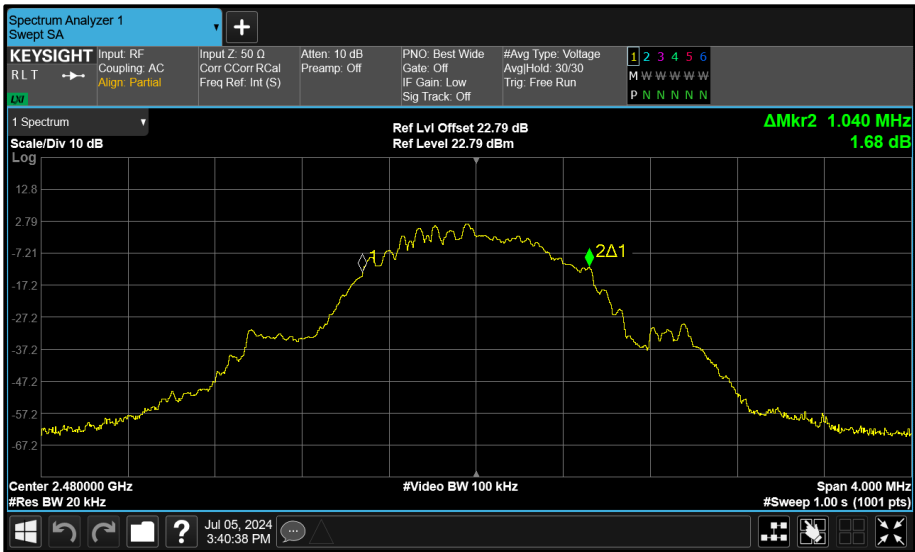
Figure 109 - Core 2 (C) 2480 MHz (CH39) 99% Bandwidth
