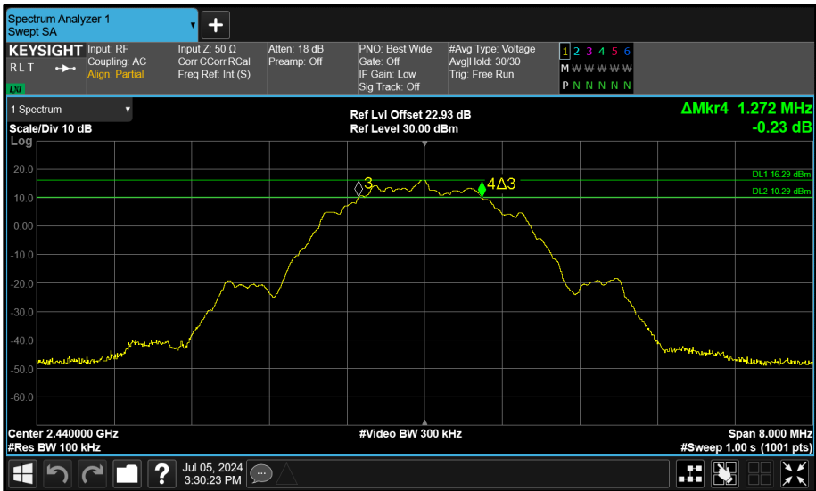
Figure 138 - Core 0 (A) 2440 MHz (CH17) 6 dB Bandwidth
