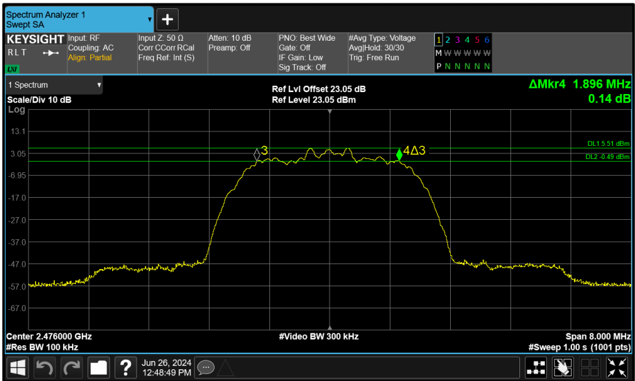
Figure 150 - Core 0 (A) 2476 MHz (CH74) 6 dB Bandwidth
