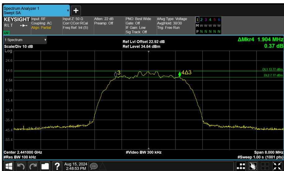
Figure 120 - Core 1 (B) 2441 MHz (CH39) 6 dB Bandwidth
