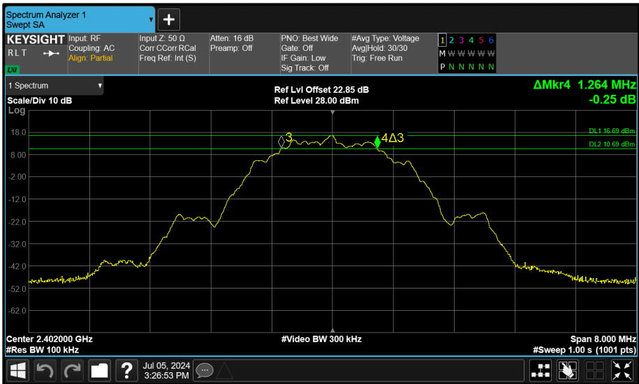
Figure 136 - Core 0 (A) 2402 MHz (CH37) 6 dB Bandwidth
