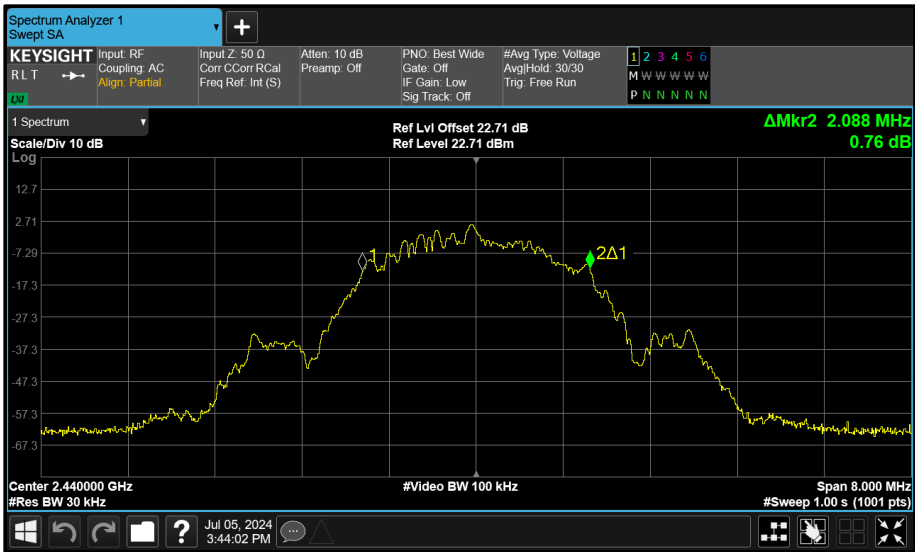
Figure 113 - Core 2 (C) 2440 MHz (CH17) 99% Bandwidth
