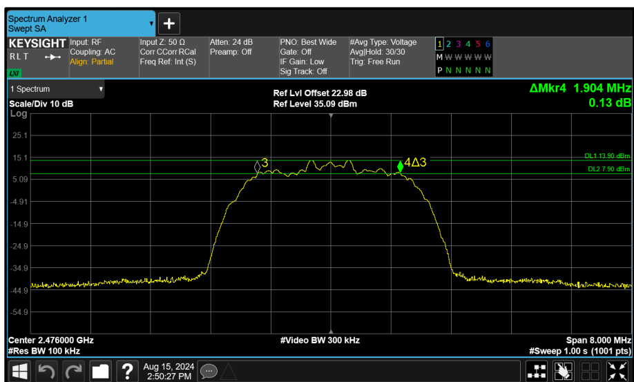
Figure 122 - Core 1 (B) 2476 MHz (CH74) 6 dB Bandwidth
