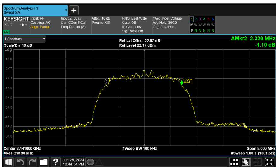
Figure 147 - Core 1 (B) 2441 MHz (CH39) 99% Bandwidth
