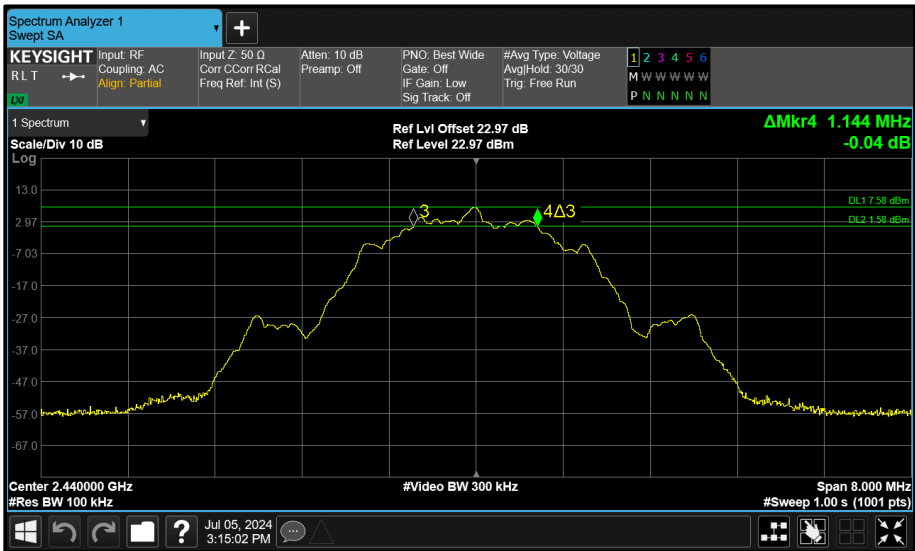
Figure 102 - Core 1 (B) 2440 MHz (CH17) 6 dB Bandwidth
