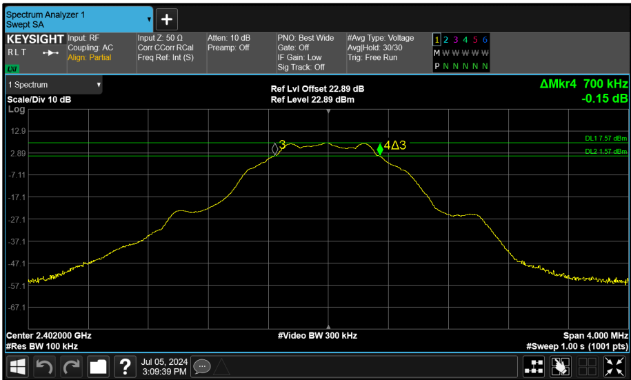
Figure 94 - Core 1 (B) 2402 MHz (CH37) 6 dB Bandwidth
