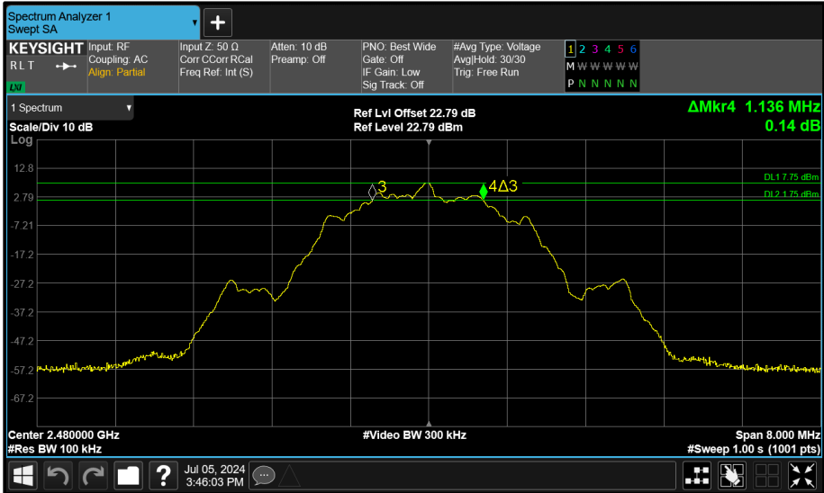
Figure 116 - Core 2 (C) 2480 MHz (CH39) 6 dB Bandwidth
