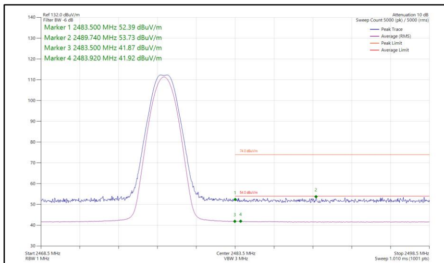
Figure 36 - Bluetooth LE1M, MIMO, Core 0 - Core 1 - 2478 MHz Band Edge Frequency 2483.5 MHz
