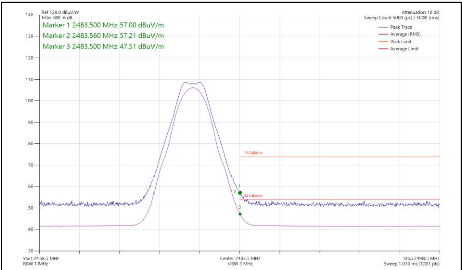
Figure 29 - Bluetooth LE2M, SISO, Core 2 - 2480 MHz Band Edge Frequency 2483.5 MHz
