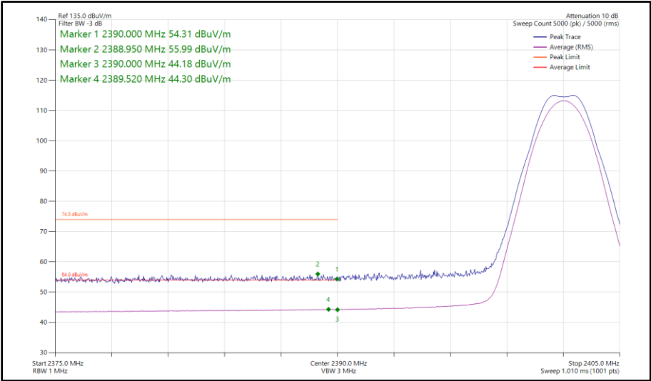
Figure 43 - Bluetooth LE2M, SISO, Core 0 - 2402 MHz Band Edge Frequency 2390 MHz
