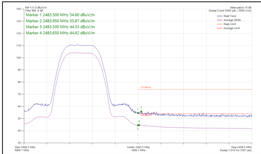
Figure 65 - Bluetooth HDR8, MIMO, Core 0 - Core 1 - 2476 MHz Band Edge Frequency 2483.5 MHz
