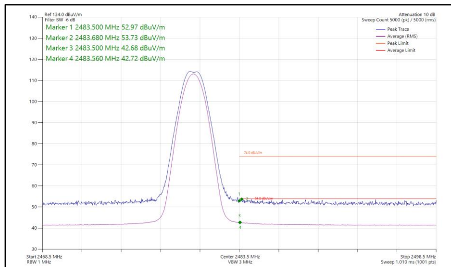
Figure 37 - Bluetooth LE1M, MIMO, Core 0 - Core 1 - 2480 MHz Band Edge Frequency 2483.5 MHz
