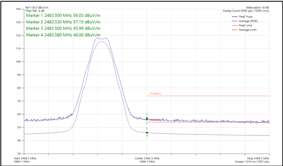
Figure 48 - Bluetooth LE2M, SISO, Core 0 - 2478 MHz Band Edge Frequency 2483.5 MHz
