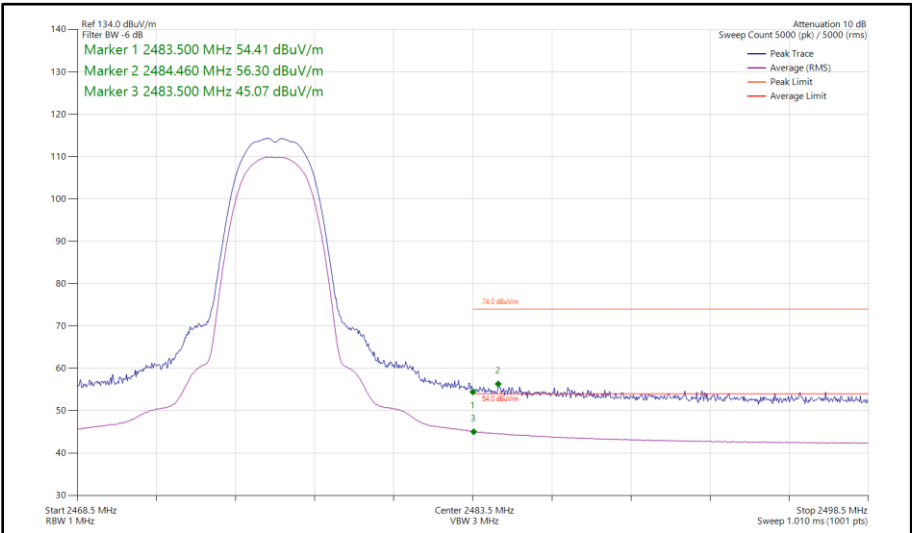
Figure 44 - Bluetooth HDR4, SISO, Core 0 - 2476 MHz Band Edge Frequency 2483.5 MHz
