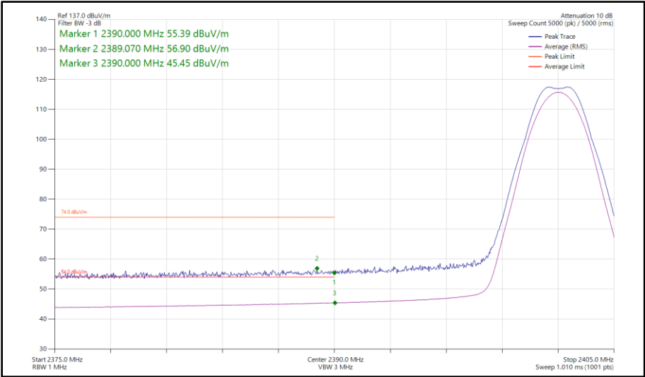
Figure 53 - Bluetooth LE2M, SISO, Core 1 - 2402 MHz Band Edge Frequency 2390 MHz
