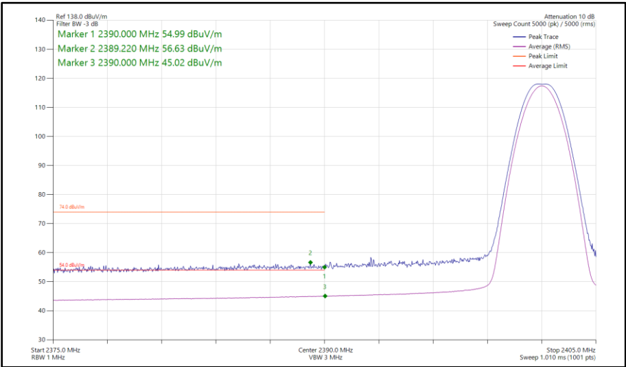
Figure 62 - Bluetooth LE1M, MIMO, Core 0 - Core 1 - 2402 MHz Band Edge Frequency 2390 MHz
