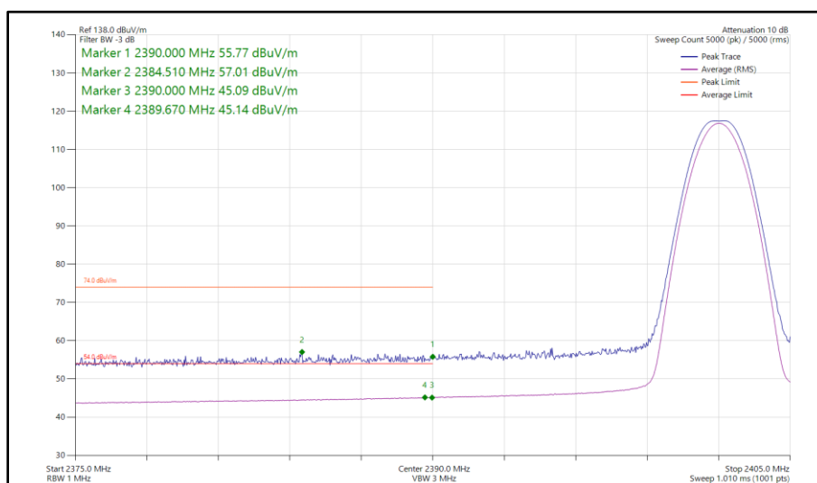
Figure 52 - Bluetooth LE1M, SISO, Core 1 - 2402 MHz Band Edge Frequency 2390 MHz
