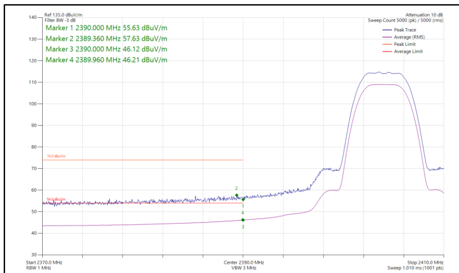
Figure 51 - Bluetooth HDR8, SISO, Core 1 - 2404 MHz Band Edge Frequency 2390 MHz
