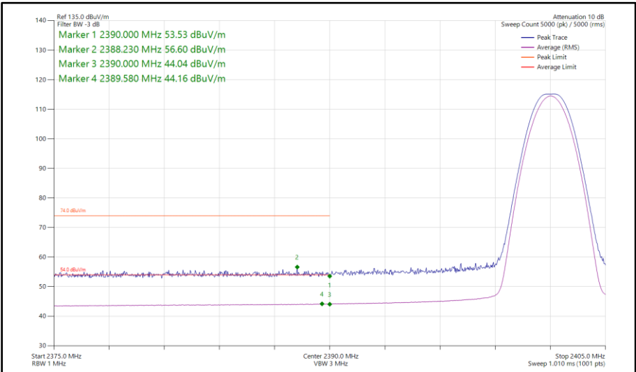
Figure 42 - Bluetooth LE1M, SISO, Core 0 - 2402 MHz Band Edge Frequency 2390 MHz
