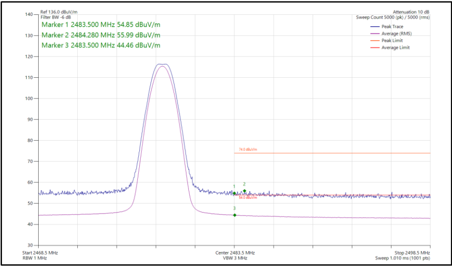
Figure 56 - Bluetooth LE1M, SISO, Core 1 - 2478 MHz Band Edge Frequency 2483.5 MHz
