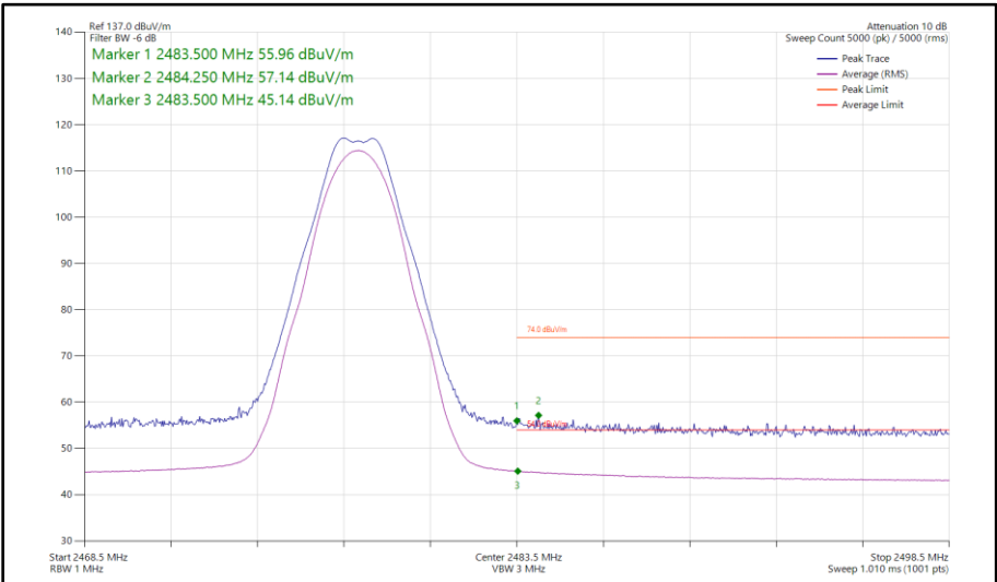
Figure 58 - Bluetooth LE2M, SISO, Core 1 - 2478 MHz Band Edge Frequency 2483.5 MHz
