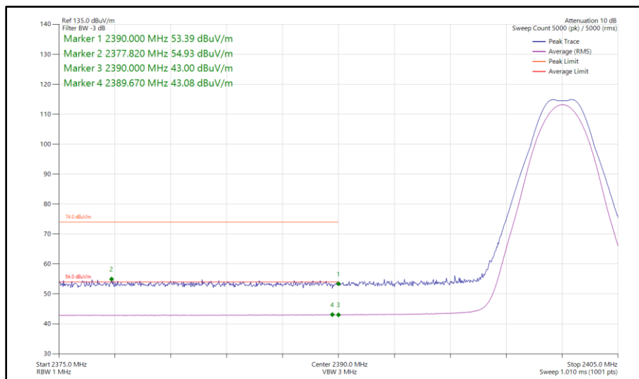
Figure 33 - Bluetooth LE2M, MIMO, Core 0 - Core 1 - 2402 MHz Band Edge Frequency 2390 MHz
