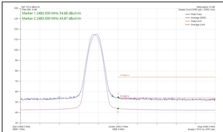
Figure 66 - Bluetooth LE1M, MIMO, Core 0 - Core 1 - 2480 MHz Band Edge Frequency 2483.5 MHz
