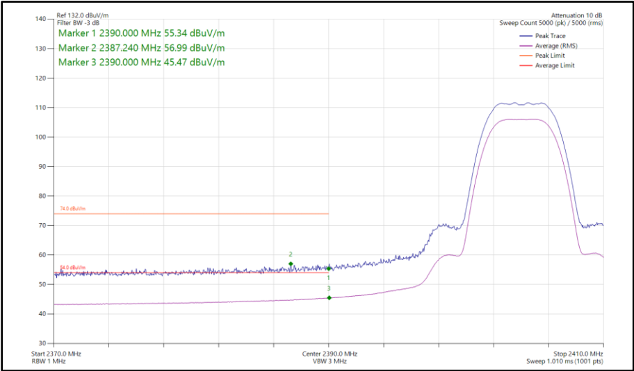
Figure 41 - Bluetooth HDR8, SISO, Core 0 - 2404 MHz Band Edge Frequency 2390 MHz
