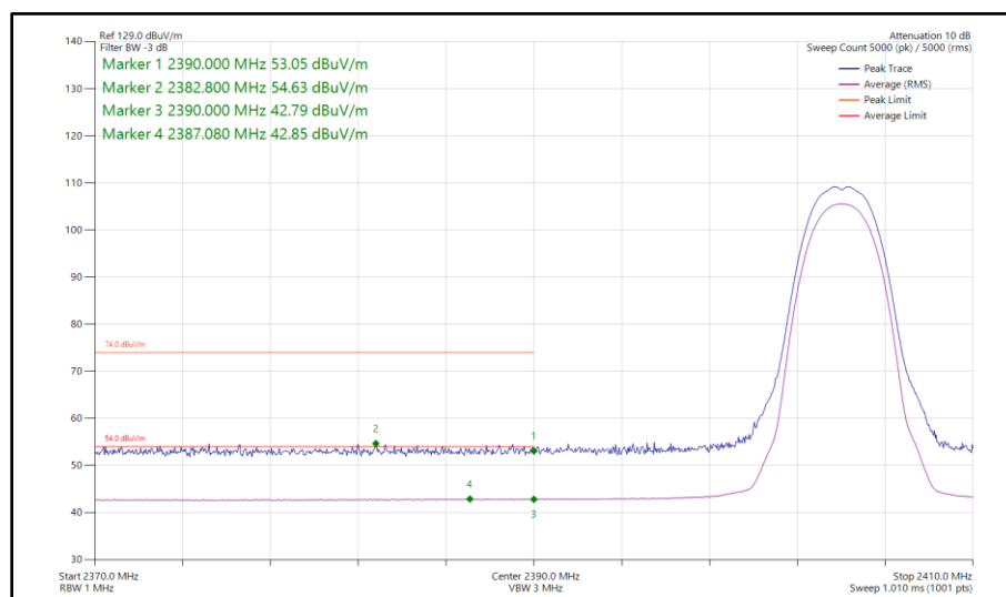
Figure 30 - Bluetooth HDR4, MIMO, Core 0 - Core 1 - 2404 MHz Band Edge Frequency 2390 MHz
