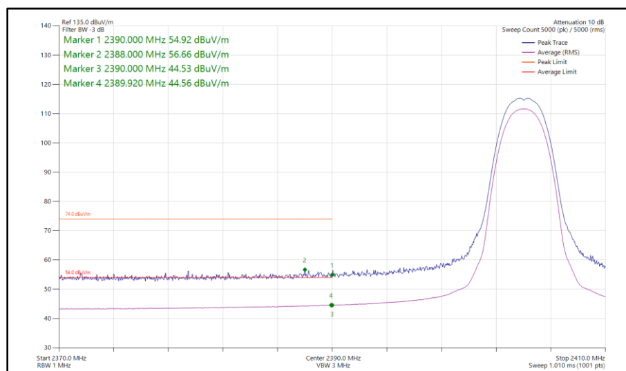
Figure 50 - Bluetooth HDR4, SISO, Core 1 - 2404 MHz Band Edge Frequency 2390 MHz
