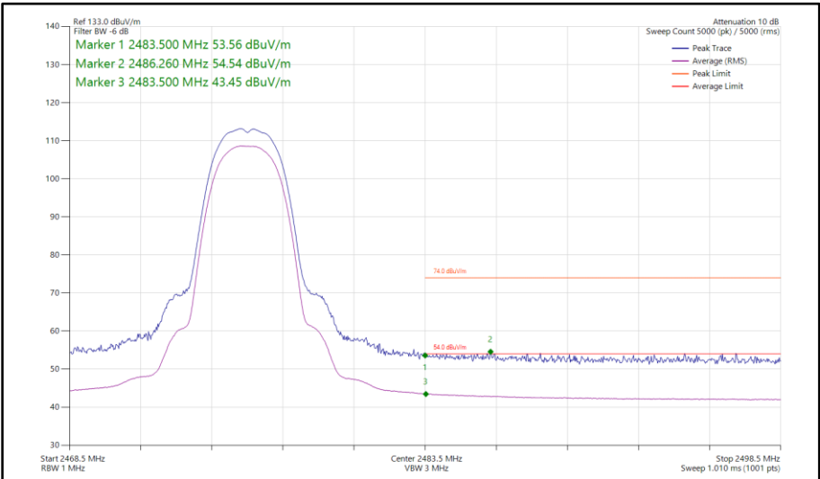
Figure 54 - Bluetooth HDR4, SISO, Core 1 - 2476 MHz Band Edge Frequency 2483.5 MHz
