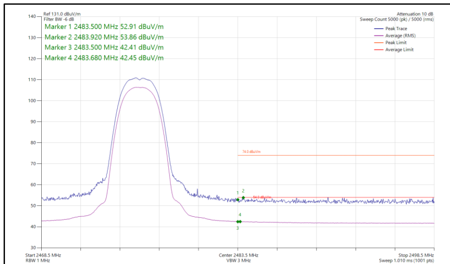
Figure 64 - Bluetooth HDR4, MIMO, Core 0 - Core 1 - 2476 MHz Band Edge Frequency 2483.5 MHz
