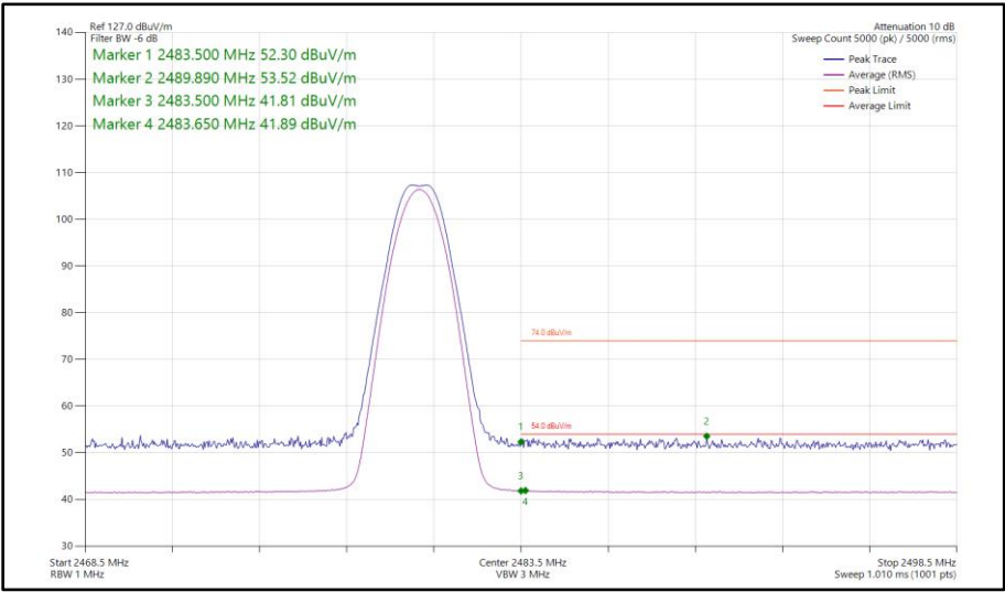
Figure 27 - Bluetooth LE1M, SISO, Core 2 - 2480 MHz Band Edge Frequency 2483.5 MHz
