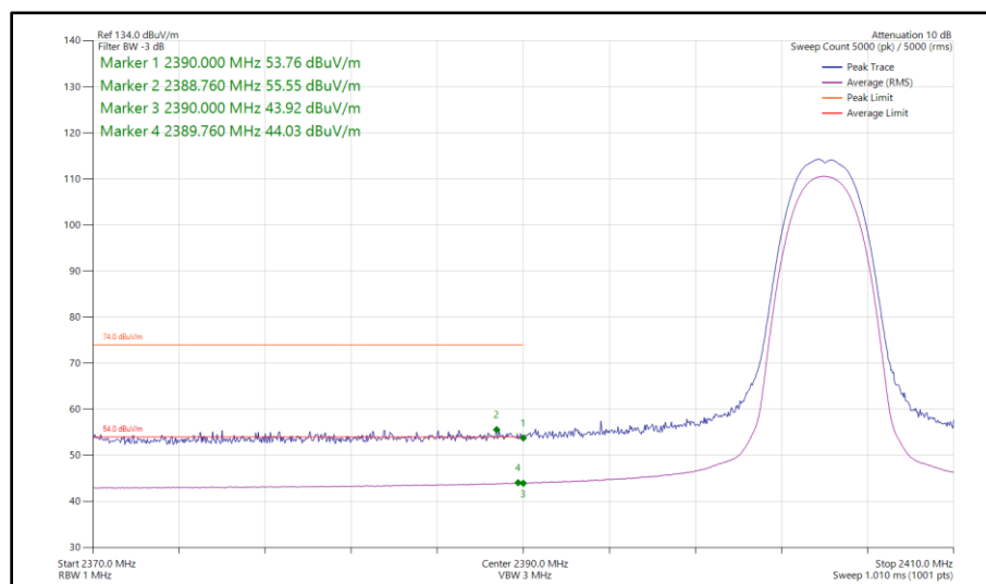
Figure 60 - Bluetooth HDR4, MIMO, Core 0 - Core 1 - 2404 MHz Band Edge Frequency 2390 MHz
