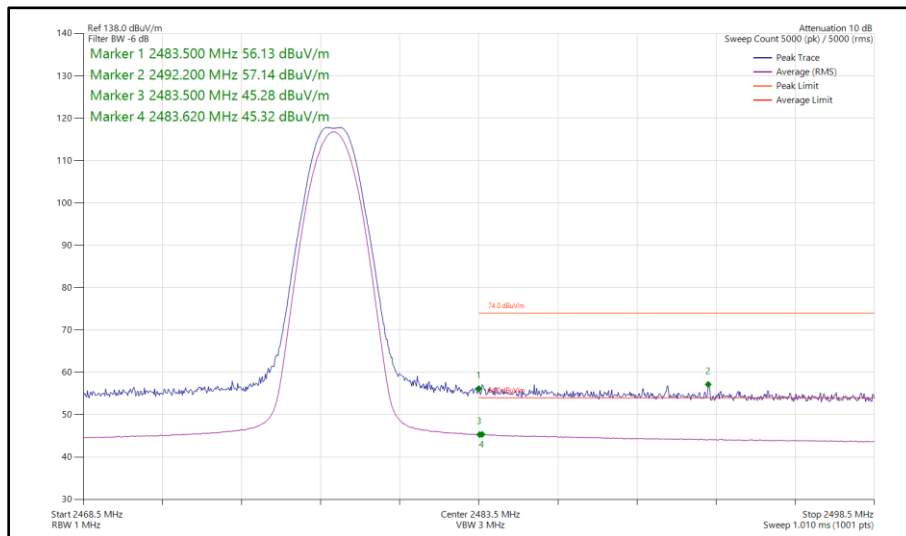
Figure 46 - Bluetooth LE1M, SISO, Core 0 - 2478 MHz Band Edge Frequency 2483.5 MHz
