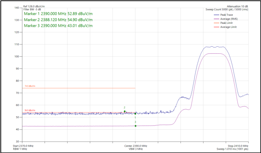
Figure 31 - Bluetooth HDR8, MIMO, Core 0 - Core 1 - 2404 MHz Band Edge Frequency 2390 MHz
