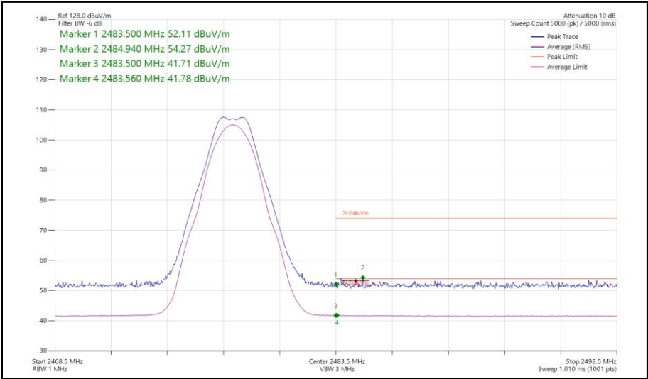
Figure 28 - Bluetooth LE2M, SISO, Core 2 - 2478 MHz Band Edge Frequency 2483.5 MHz
