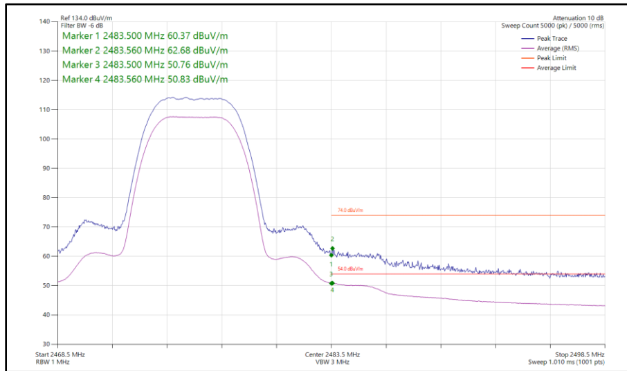
Figure 45 - Bluetooth HDR8, SISO, Core 0 - 2476 MHz Band Edge Frequency 2483.5 MHz
