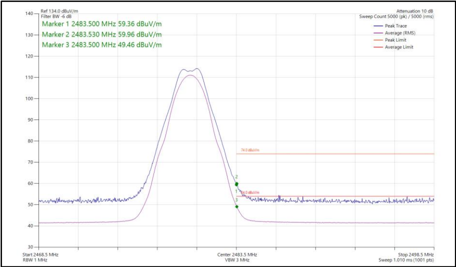
Figure 39 - Bluetooth LE2M, MIMO, Core 0 - Core 1 - 2480 MHz Band Edge Frequency 2483.5 MHz
