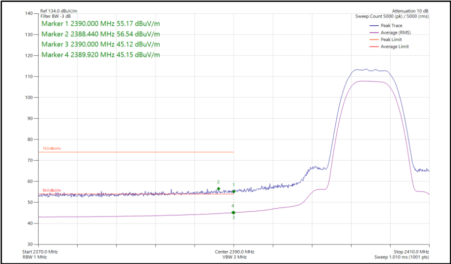
Figure 61 - Bluetooth HDR8, MIMO, Core 0 - Core 1 - 2404 MHz Band Edge Frequency 2390 MHz
