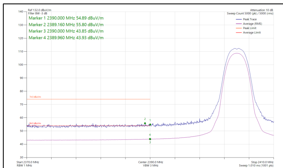
Figure 40 - Bluetooth HDR4, SISO, Core 0 - 2404 MHz Band Edge Frequency 2390 MHz
