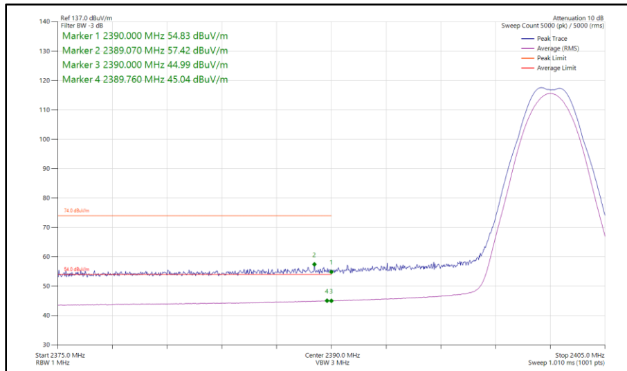
Figure 63 - Bluetooth LE2M, MIMO, Core 0 - Core 1 - 2402 MHz Band Edge Frequency 2390 MHz
