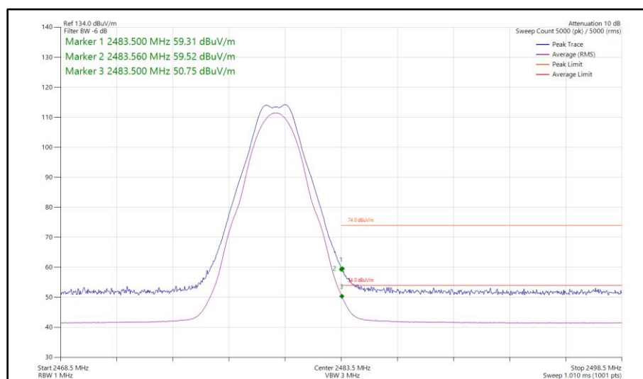
Figure 68 - Bluetooth LE2M, MIMO, Core 0 - Core 1 - 2480 MHz Band Edge Frequency 2483.5 MHz
