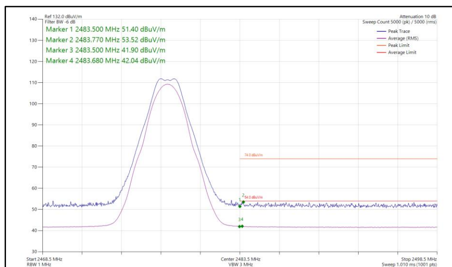
Figure 38 - Bluetooth LE2M, MIMO, Core 0 - Core 1 - 2478 MHz Band Edge Frequency 2483.5 MHz
