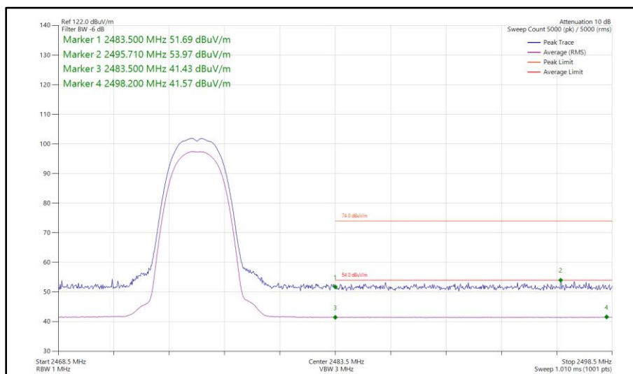
Figure 34 - Bluetooth HDR4, MIMO, Core 0 - Core 1 - 2476 MHz Band Edge Frequency 2483.5 MHz
