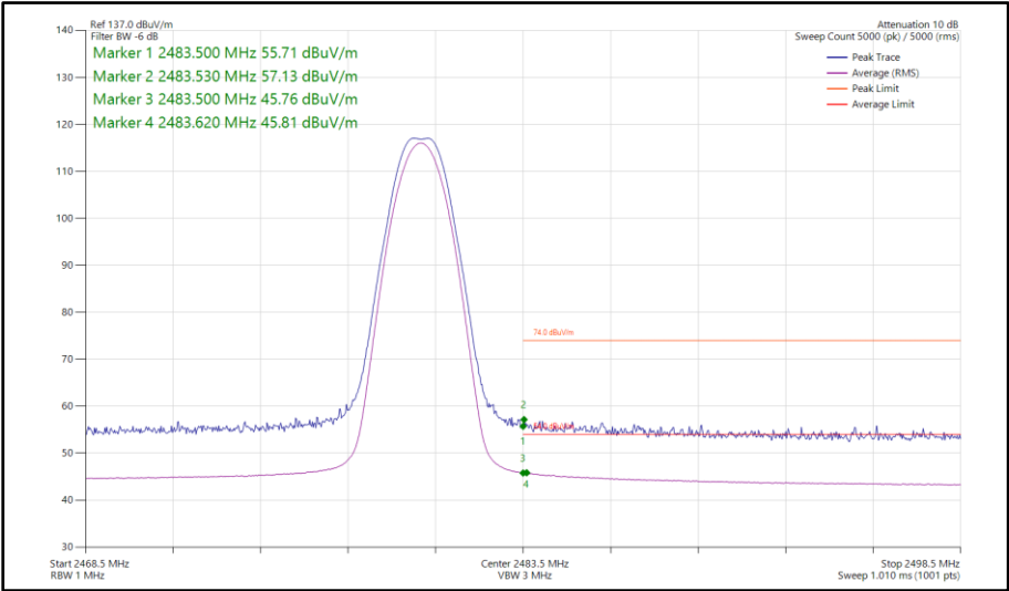
Figure 57 - Bluetooth LE1M, SISO, Core 1 - 2480 MHz Band Edge Frequency 2483.5 MHz
