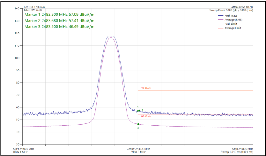
Figure 47 - Bluetooth LE1M, SISO, Core 0 - 2480 MHz Band Edge Frequency 2483.5 MHz
