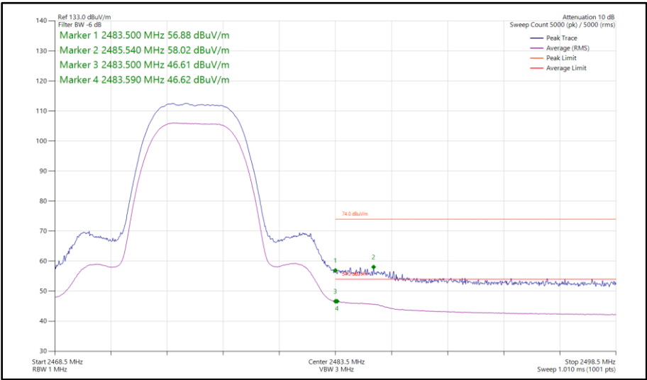
Figure 55 - Bluetooth HDR8, SISO, Core 1 - 2476 MHz Band Edge Frequency 2483.5 MHz
