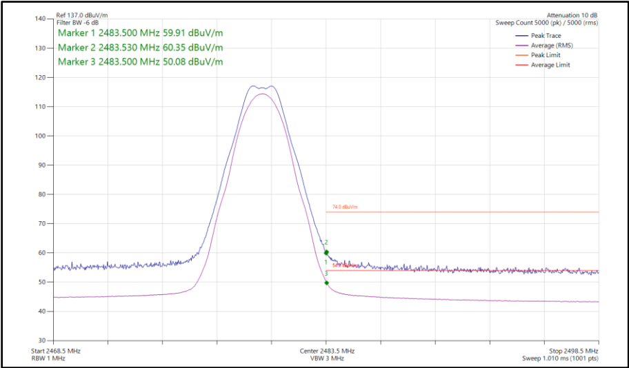
Figure 59 - Bluetooth LE2M, SISO, Core 1 - 2480 MHz Band Edge Frequency 2483.5 MHz
