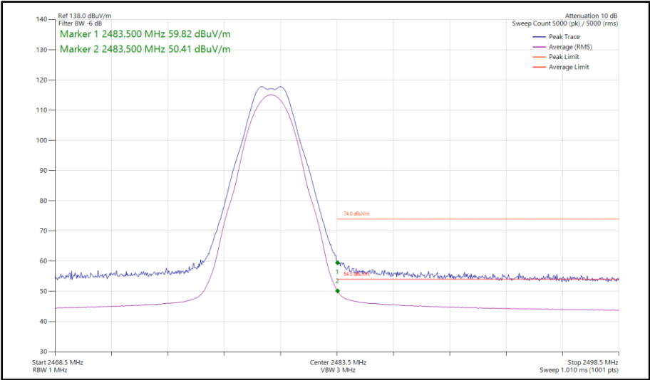
Figure 49 - Bluetooth LE2M, SISO, Core 0 - 2480 MHz Band Edge Frequency 2483.5 MHz
