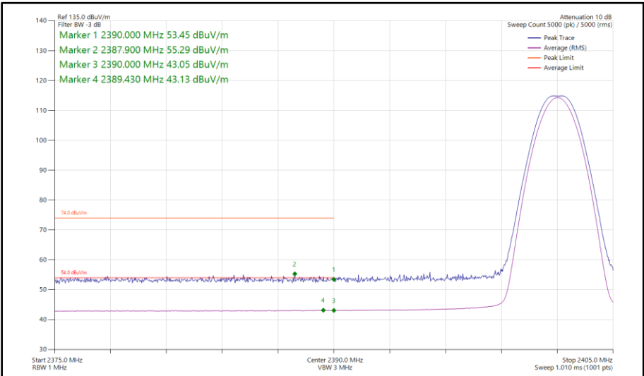
Figure 32 - Bluetooth LE1M, MIMO, Core 0 - Core 1 - 2402 MHz Band Edge Frequency 2390 MHz
