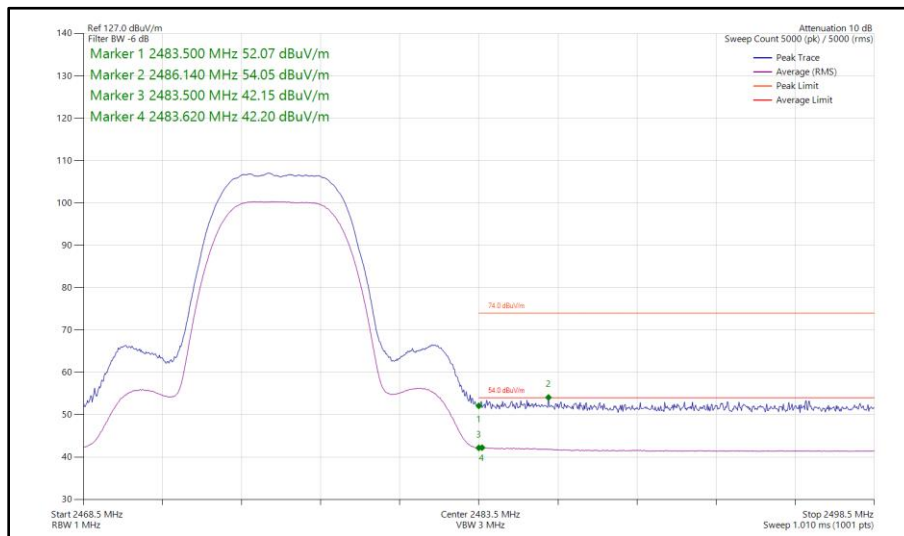
Figure 35 - Bluetooth HDR8, MIMO, Core 0 - Core 1 - 2476 MHz Band Edge Frequency 2483.5 MHz
