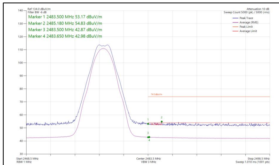
Figure 67 - Bluetooth LE2M, MIMO, Core 0 - Core 1 - 2478 MHz Band Edge Frequency 2483.5 MHz
