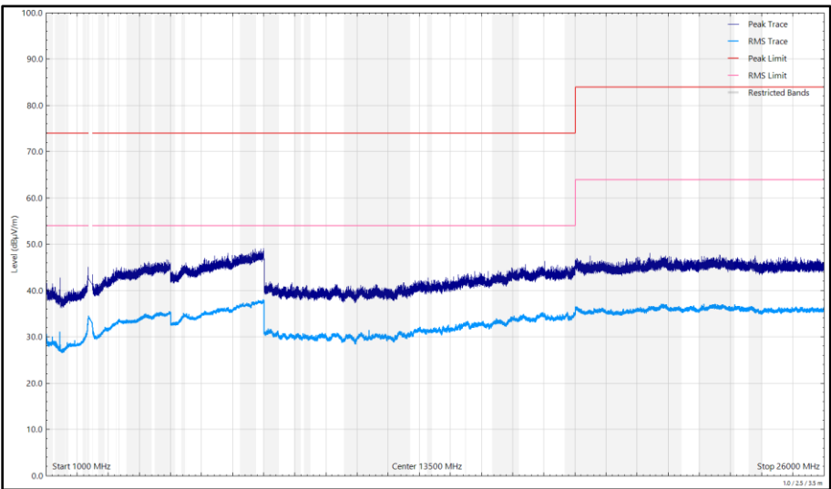
Figure 229 - 2412 MHz (CH1), HE20, RU26-0, CDD, Core 0 + Core 1, 1 GHz to 26 GHz, Vertical
