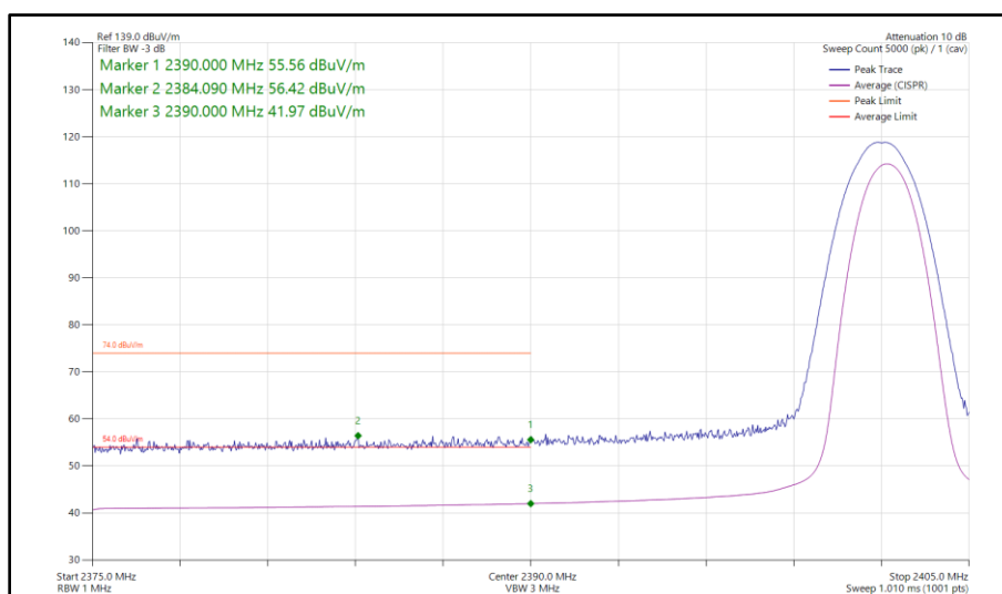
Figure 38 - Bluetooth 2-DH5, MIMO, Core 0 - Core 1 - 2402 MHz Band Edge Frequency 2390 MHz
