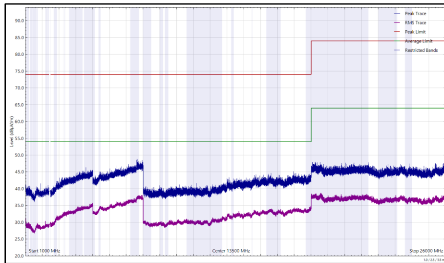
Figure 44 - 2441 MHz (CH39), DH5, iPA, Core 0, 1 GHz to 26 GHz, Horizontal
