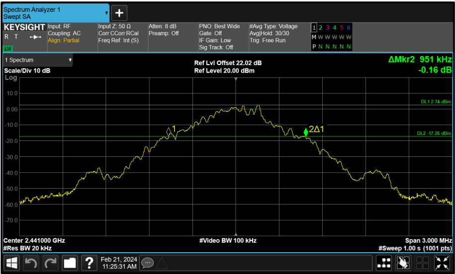
Figure 17 - Core 0 (A) 2441 MHz (CH39) 20 dB Bandwidth
