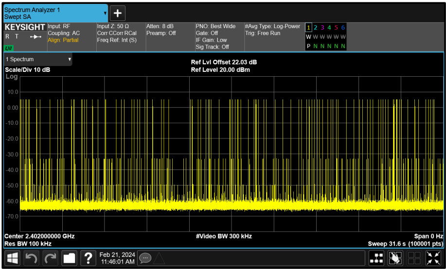
Figure 8 - \pi/4 DQPSK - 2402 MHz Accumulated Transmit Time
