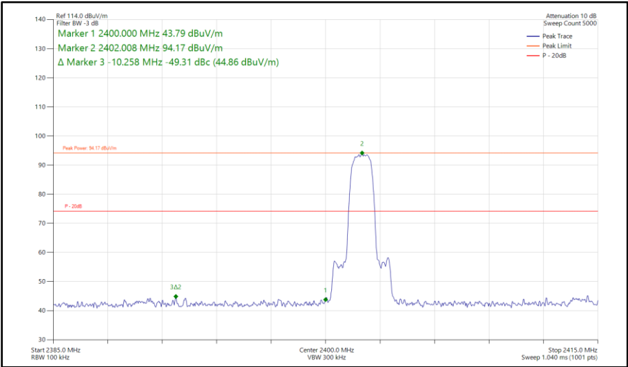
Figure 35 - Bluetooth 2-DH5, SISO, Core 0 - 2402 MHz Band Edge Frequency 2400 MHz
