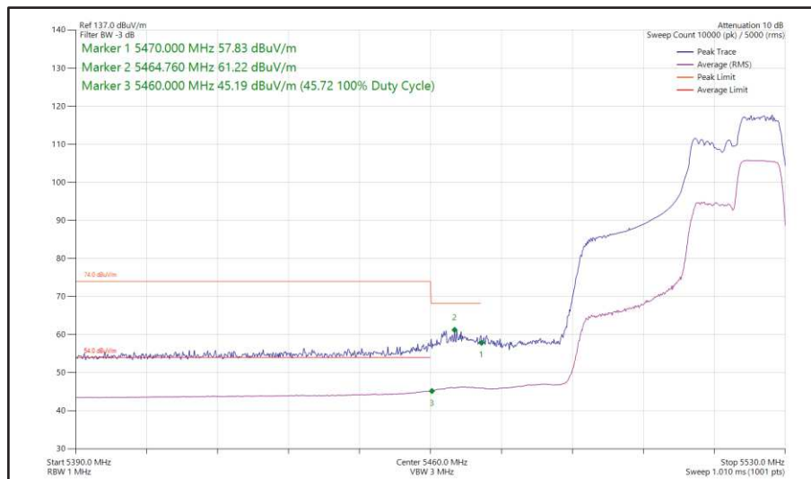
Figure 470 - 802.11ax HE40, RU 106-56, SISO, Core 1 - 5510 MHz Band Edge Frequency 5470 MHz
