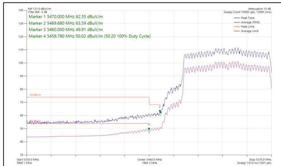
Figure 569 - 802.11ax HE80, SU, CDD, Core 0-1 - 5530 MHz Band Edge Frequency 5470 MHz
