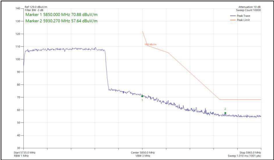
Figure 566 - 802.11ax HE80, SU, SISO, Core 1 - 5775 MHz Band Edge Frequency 5850 MHz
