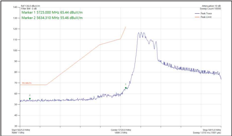
Figure 588 - 802.11ax HE80, RU 106-53, SDM, Core 0-1 - 5775 MHz Band Edge Frequency 5725 MHz
