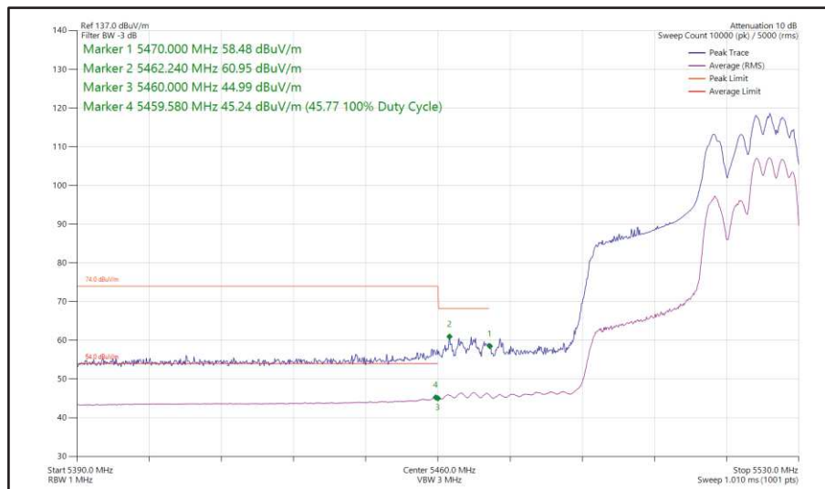
Figure 491 - 802.11ax HE40, RU 106-56, CDD, Core 0-1 - 5510 MHz Band Edge Frequency 5470 MHz
