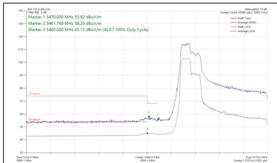
Figure 555 - 802.11ax HE80, RU 106-53, SISO, Core 1 - 5530 MHz Band Edge Frequency 5470 MHz
