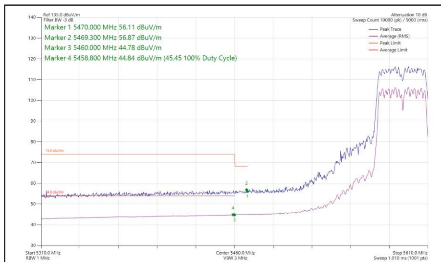
Figure 490 - 802.11n HT40, CDD, Core 0-1 - 5590 MHz Band Edge Frequency 5470 MHz
