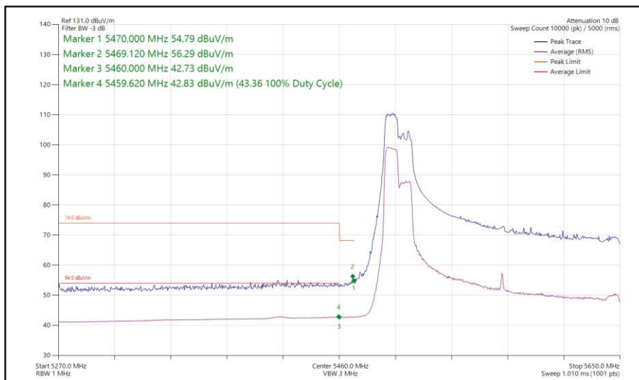
Figure 616- 802.11ax HE160, RU 106-53, SISO, Core 1 - 5570 MHz Band Edge Frequency 5470 MHz
