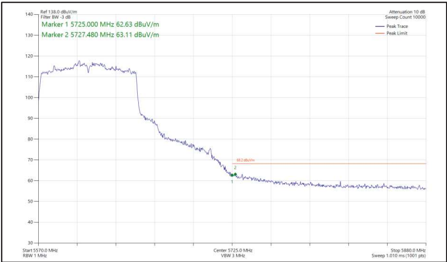
Figure 589 - 802.11ac VHT80, SDM, Core 0-1 - 5610 MHz Band Edge Frequency 5725 MHz
