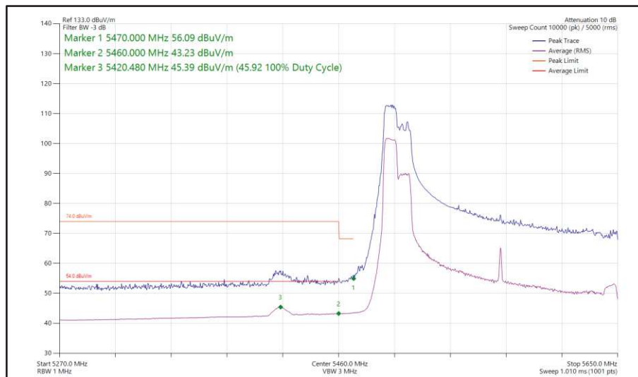
Figure 610- 802.11ax HE160, RU 106-53, SISO, Core 0 - 5570 MHz Band Edge Frequency 5470 MHz
