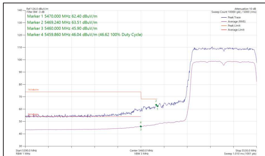
Figure 469 - 802.11ax HE40, SU, SISO, Core 1 - 5510 MHz Band Edge Frequency 5470 MHz
