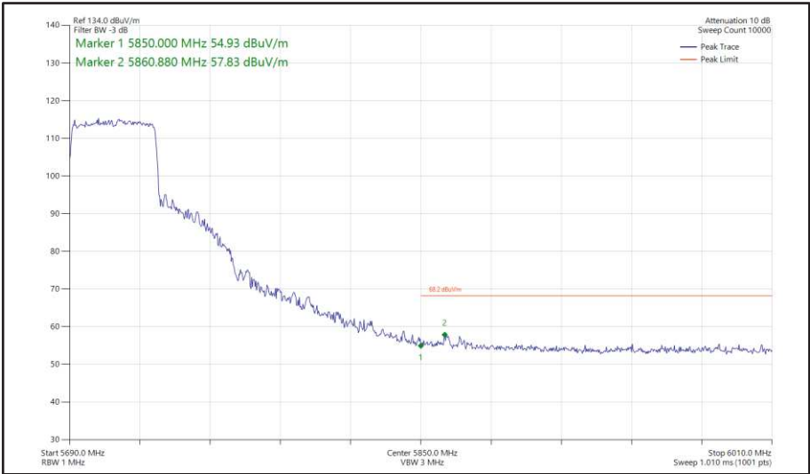
Figure 484 - 802.11ax HE40, SU, SISO, Core 1 - 5710 MHz Band Edge Frequency 5850 MHz
