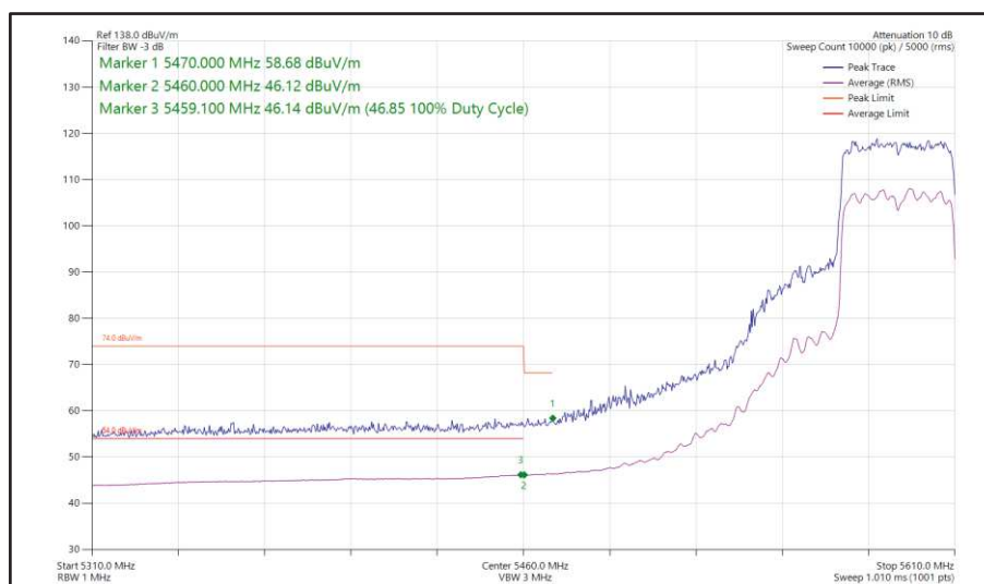
Figure 516 - 802.11ax HE40, SU, SDM, Core 0-1 - 5590 MHz Band Edge Frequency 5470 MHz
