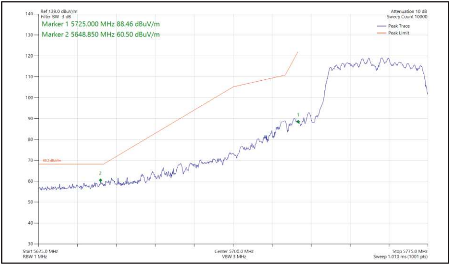
Figure 495 - 802.11n HT40, CDD, Core 0-1 - 5755 MHz Band Edge Frequency 5725 MHz
