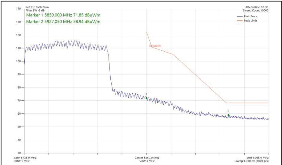
Figure 581 - 802.11ax HE80, SU, CDD, Core 0-1 - 5775 MHz Band Edge Frequency 5850 MHz
