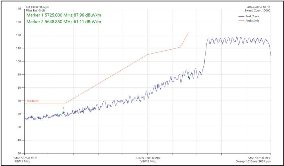
Figure 496 - 802.11ax HE40, SU, CDD, Core 0-1 - 5755 MHz Band Edge Frequency 5725 MHz
