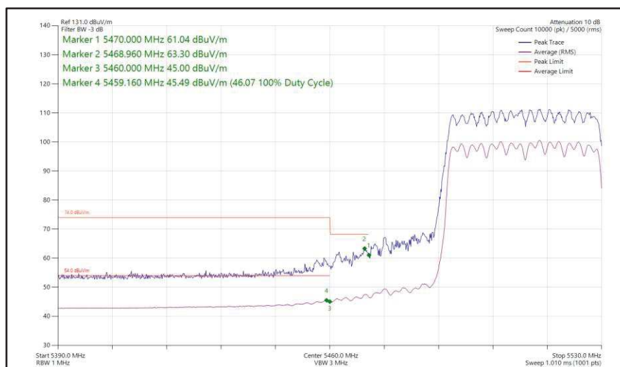
Figure 259 - 802.11ax HE40, SU, CDD, Core 0-1 - 5510 MHz Band Edge Frequency 5470 MHz
