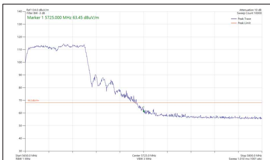
Figure 535 - 802.11ac VHT40, TxBF, Core 0 + Core 1 - 5670 MHz Band Edge Frequency 5725 MHz
