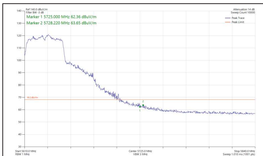
Figure 534 - 802.11ac VHT40, TxBF, Core 0 + Core 1 - 5630 MHz Band Edge Frequency 5725 MHz
