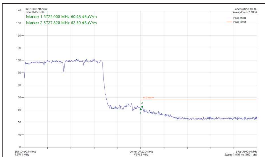
Figure 617 - 802.11ac VHT160, SISO, Core 1 - 5570 MHz Band Edge Frequency 5725 MHz
