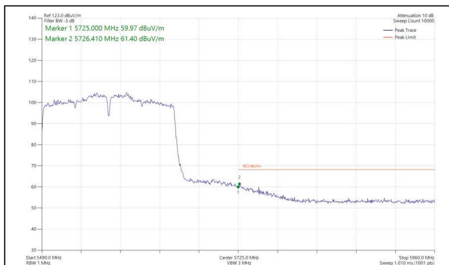
Figure 611- 802.11ac VHT160, SISO, Core 0 - 5570 MHz Band Edge Frequency 5725 MHz
