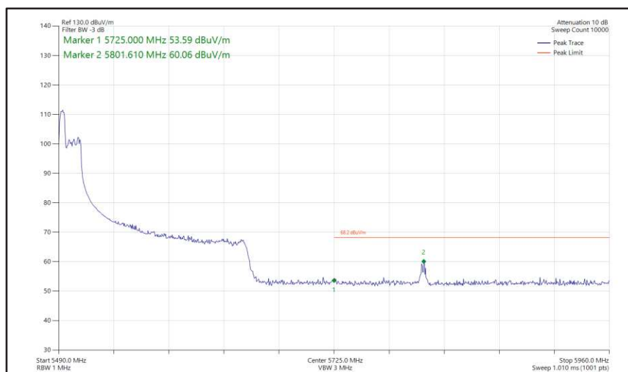
Figure 619- 802.11ax HE160, RU 52-37, SISO, Core 1 - 5570 MHz Band Edge Frequency 5725 MHz
