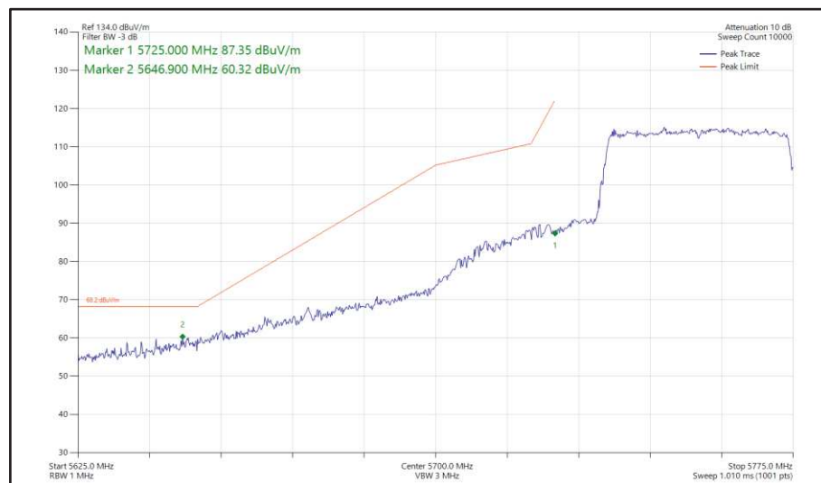
Figure 475 - 802.11ax HE40, SU, SISO, Core 1 - 5755 MHz Band Edge Frequency 5725 MHz
