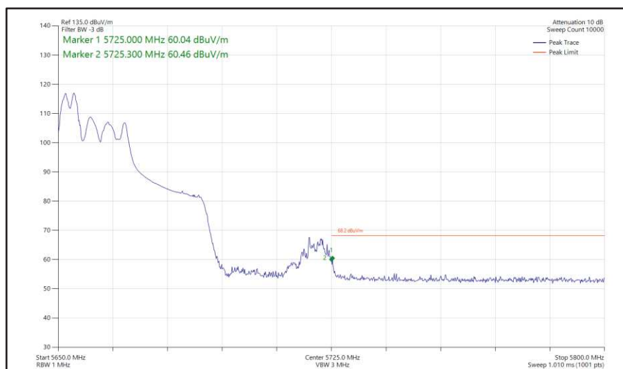
Figure 502 - 802.11ax HE40, RU 52-37, CDD, Core 0-1 - 5670 MHz Band Edge Frequency 5725 MHz
