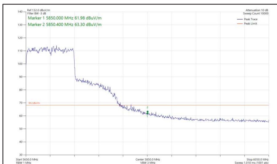
Figure 606 - 802.11ax HE80, SU, TxBF, Core 0 + Core 1 - 5690 MHz Band Edge Frequency 5850 MHz
