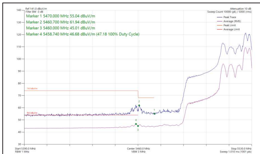
Figure 513 - 802.11ax HE40, RU 52-44, SDM, Core 0-1 - 5510 MHz Band Edge Frequency 5470 MHz
