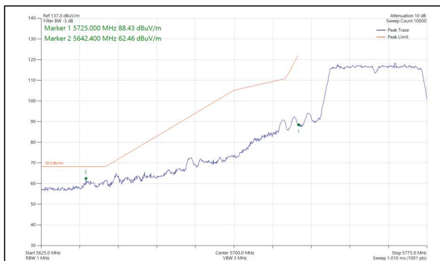
Figure 517 - 802.11n HT40, SDM, Core 0-1 - 5755 MHz Band Edge Frequency 5725 MHz
