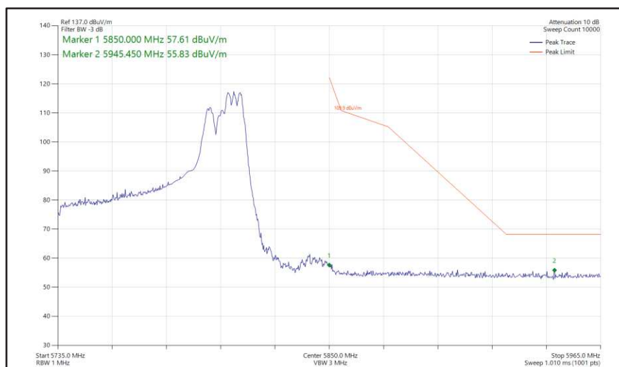
Figure 597 - 802.11ax HE80, RU 106-60, SDM, Core 0-1 - 5775 MHz Band Edge Frequency 5850 MHz
