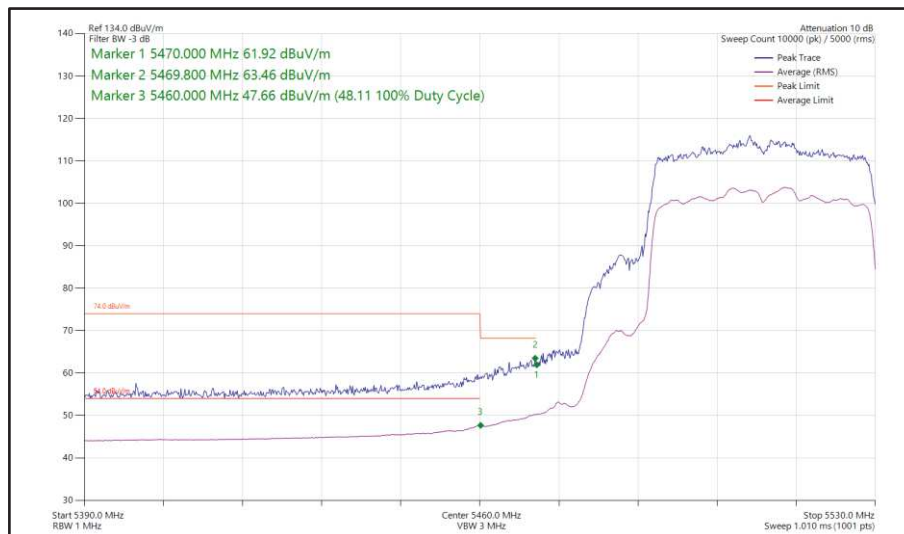
Figure 512 - 802.11ax HE40, SU, SDM, Core 0-1 - 5510 MHz Band Edge Frequency 5470 MHz
