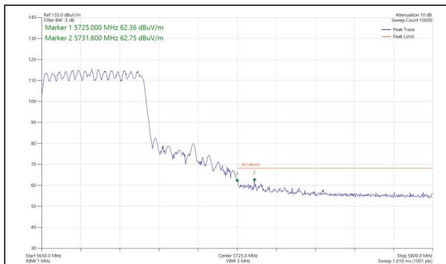
Figure 501 - 802.11ax HE40, SU, CDD, Core 0-1 - 5670 MHz Band Edge Frequency 5725 MHz
