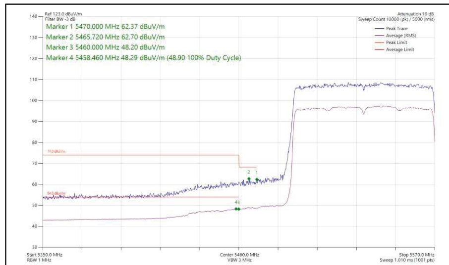
Figure 539 - 802.11ax HE80, SU, SISO, Core 0 - 5530 MHz Band Edge Frequency 5470 MHz
