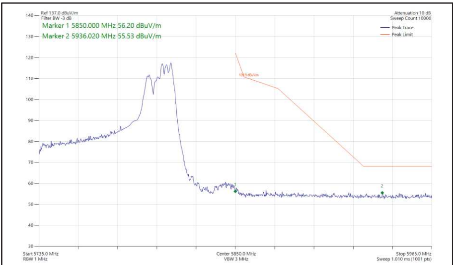
Figure 582 - 802.11ax HE80, RU 106-60, CDD, Core 0-1 - 5775 MHz Band Edge Frequency 5850 MHz
