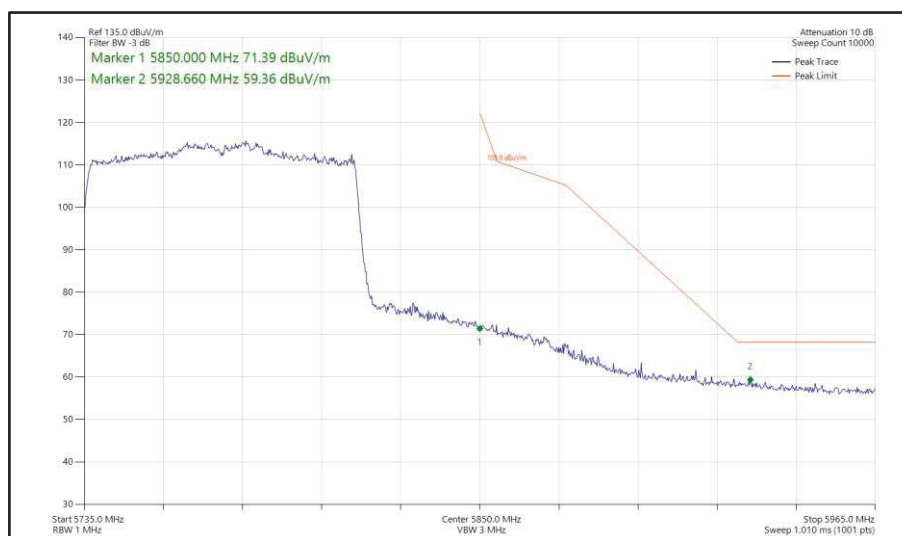
Figure 596 - 802.11ax HE80, SU, SDM, Core 0-1 - 5775 MHz Band Edge Frequency 5850 MHz
