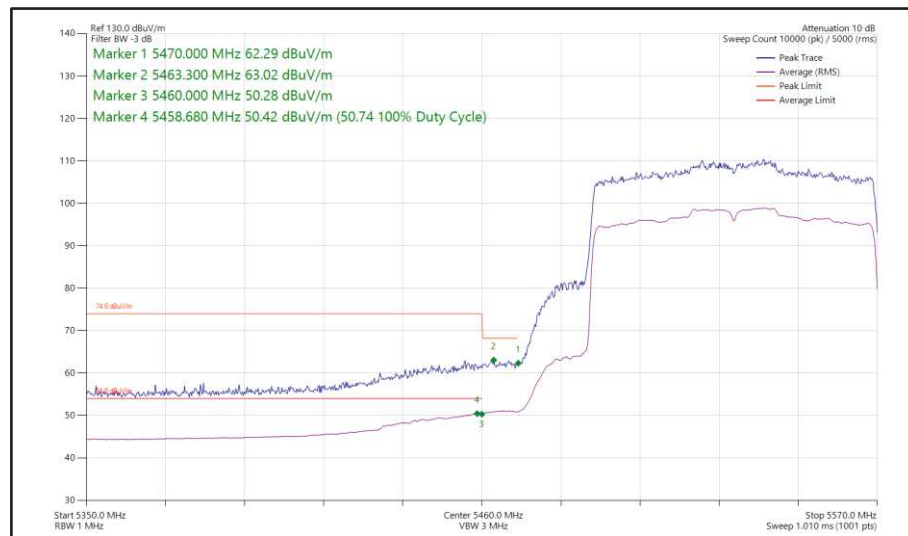
Figure 554 - 802.11ax HE80, SU, SISO, Core 1 - 5530 MHz Band Edge Frequency 5470 MHz
