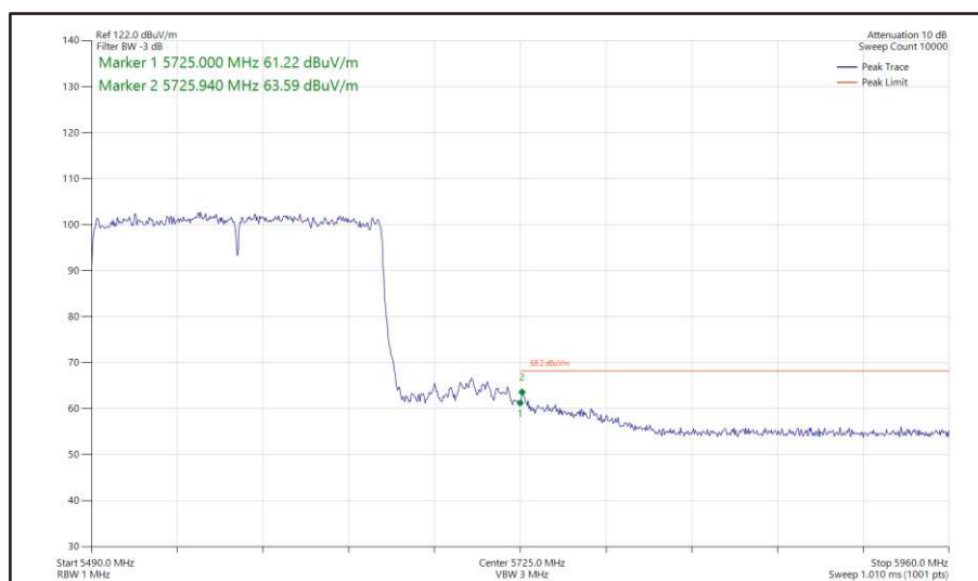
Figure 618- 802.11ax HE160, SU, SISO, Core 1 - 5570 MHz Band Edge Frequency 5725 MHz
