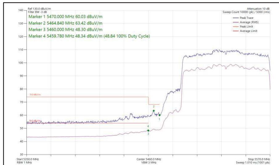
Figure 584 - 802.11ax HE80, SU, SDM, Core 0-1 - 5530 MHz Band Edge Frequency 5470 MHz
