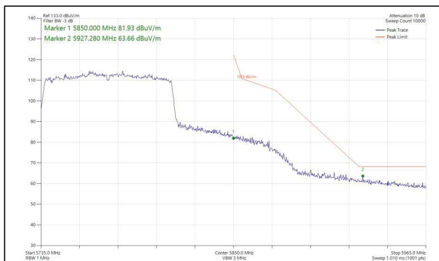
Figure 605 - 802.11ac VHT80, TxBF, Core 0 + Core 1 - 5775 MHz Band Edge Frequency 5850 MHz
