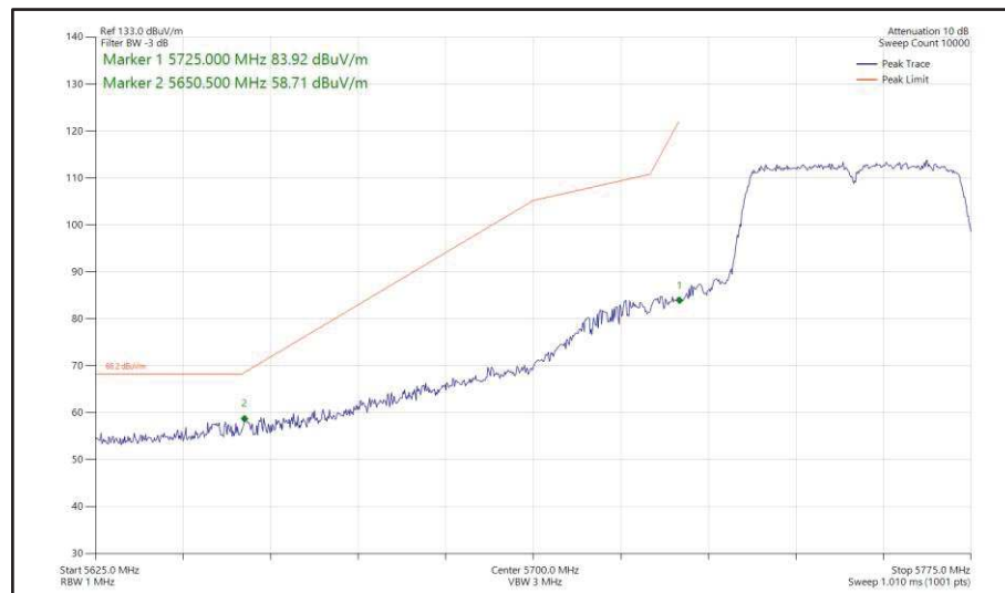
Figure 474 - 802.11n HT40, SISO, Core 1 - 5755 MHz Band Edge Frequency 5725 MHz
