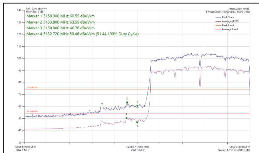
Figure 208 - 802.11ac VHT160, SISO, Core 0 - 5250 MHz Band Edge Frequency 5150 MHz
