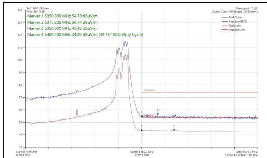
Figure 231 - 802.11ax HE160, RU 106-60S, CDD, Core 0-1 - 5250 MHz Band Edge Frequency 5350 MHz
