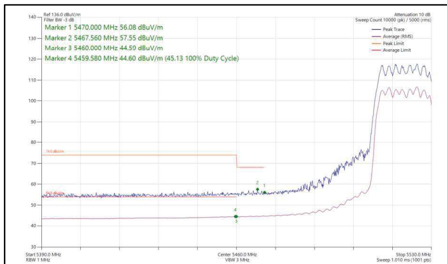
Figure 59 - 802.11ax HE20, SU, CDD, Core 0-1 - 5520 MHz Band Edge Trace Frequency 5460 MHz
