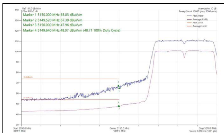
Figure 103 - 802.11n HT40, SISO, Core 1 - 5190 MHz Band Edge Frequency 5150 MHz
