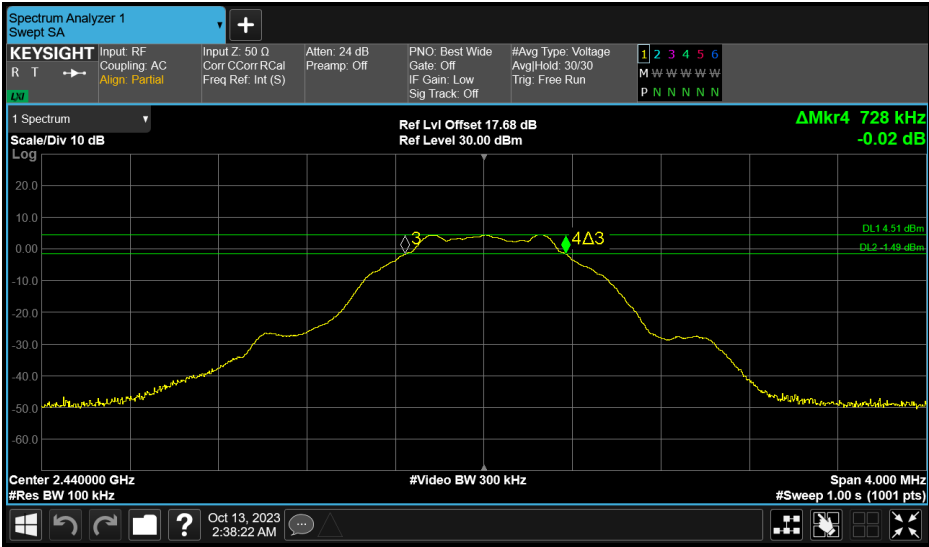
Middle Channel
