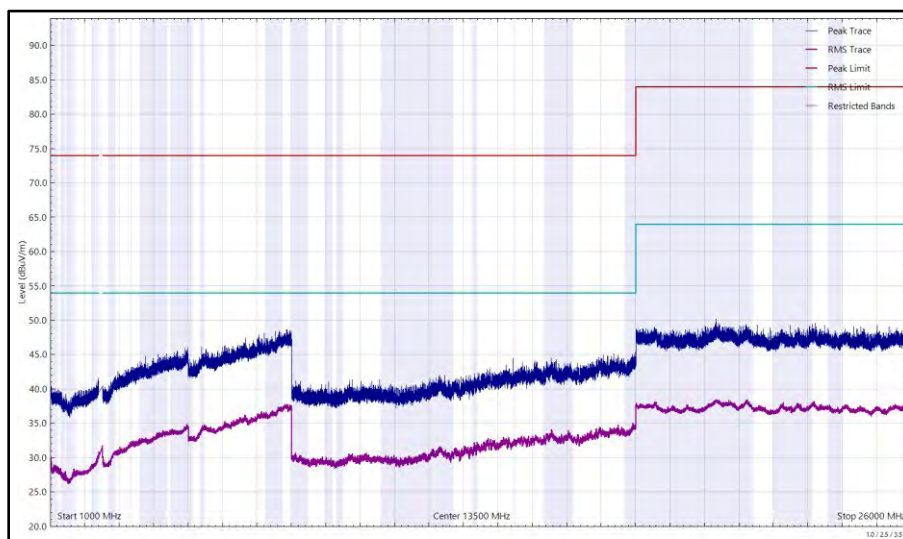
Figure 105 - 2472 MHz (CH13), 802.11b, Core 1, 1 GHz to 26 GHz, Horizontal
