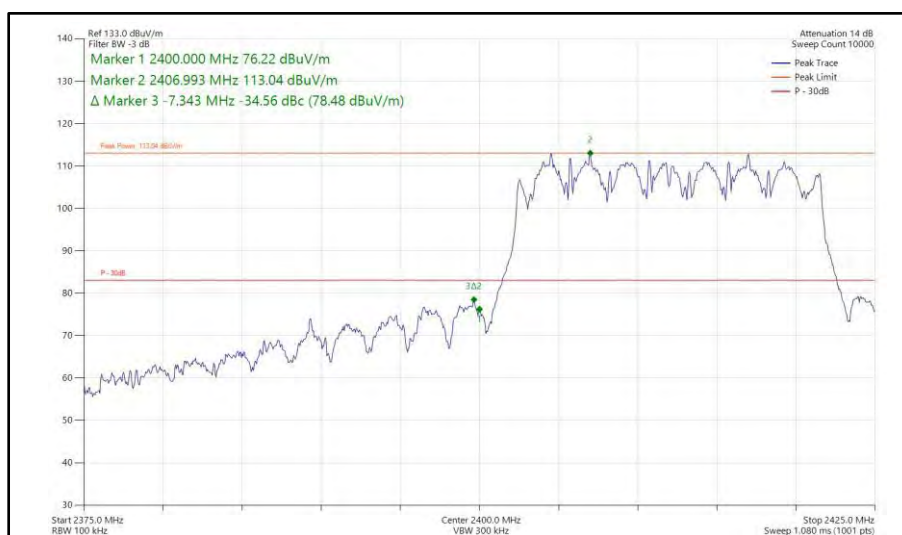
Figure 88 - 802.11ax HE20, SU, CDD, Core 0 + Core 1 - 2412 MHz Band Edge Frequency 2400 MHz
