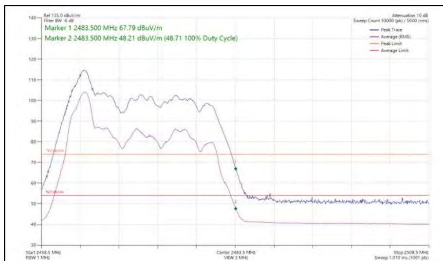
Figure 52 - 802.11ax HE20, RU 26-0, CDD, Core 0 + Core 1 - 2472 MHz Band Edge Frequency 2483.5 MHz
