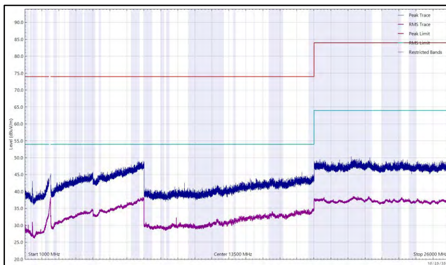
Figure 98 - 2472 MHz (CH13), 802.11b, Core 0, 1 GHz to 26 GHz, Vertical
