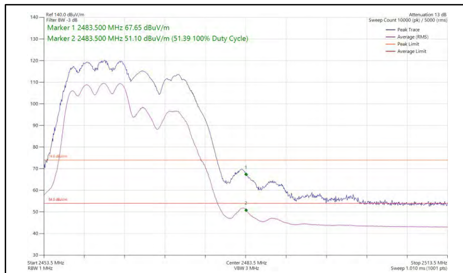
Figure 50 - 802.11ax HE20, RU 106-53, CDD, Core 0 + Core 1 - 2467 MHz Band Edge Frequency 2483.5 MHz
