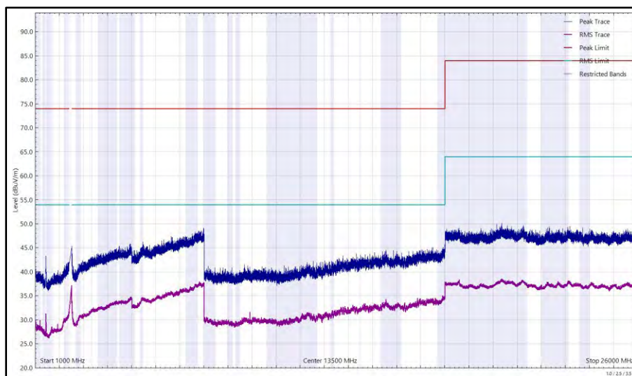
Figure 106 - 2472 MHz (CH13), 802.11b, Core 1, 1 GHz to 26 GHz, Vertical
