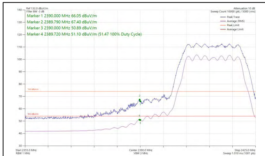
Figure 41 - 802.11n HT20, CDD, Core 0 + Core 1 - 2412 MHz Band Edge Frequency 2390 MHz
