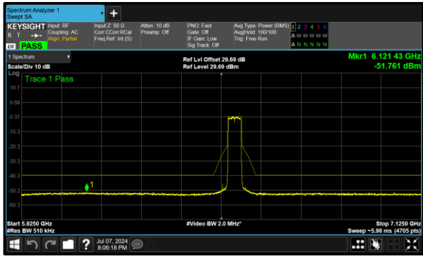
Figure 422 - A (Core 0) 6565 MHz (CH123)
