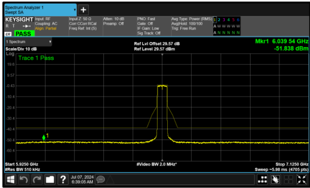
Figure 420 - A (Core 0) 6525 MHz (CH115)
