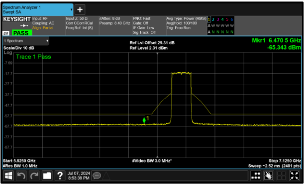
Figure 381 - B (Core 1) 6625 MHz (CH135)
