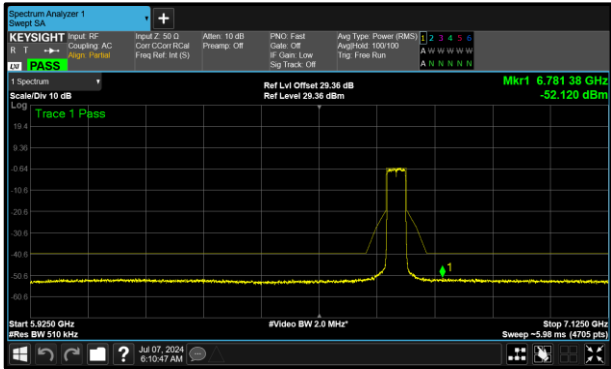
Figure 424 - A (Core 0) 6685 MHz (CH147)
