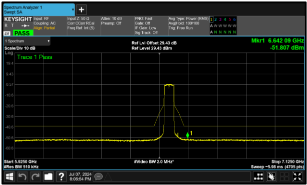
Figure 423 - B (Core 1) 6565 MHz (CH123)
