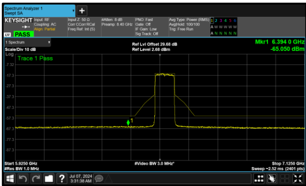
Figure 378 - A (Core 0) 6545 MHz (CH119)
