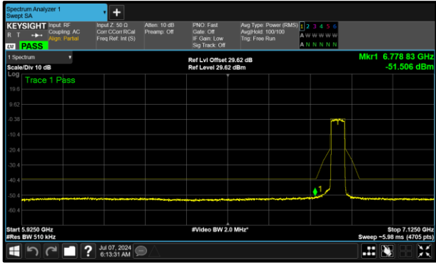
Figure 426 - A (Core 0) 6845 MHz (CH179)
