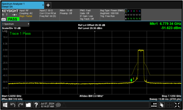
Figure 427 - B (Core 1) 6845 MHz (CH179)
