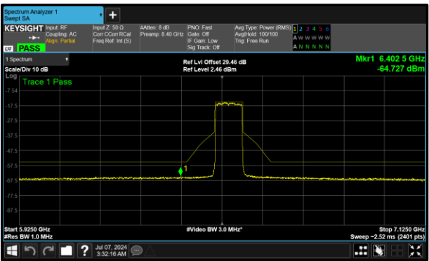
Figure 379 - B (Core 1) 6545 MHz (CH119)
