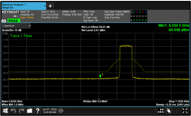
Figure 383 - B (Core 1) 6705 MHz (CH151)
