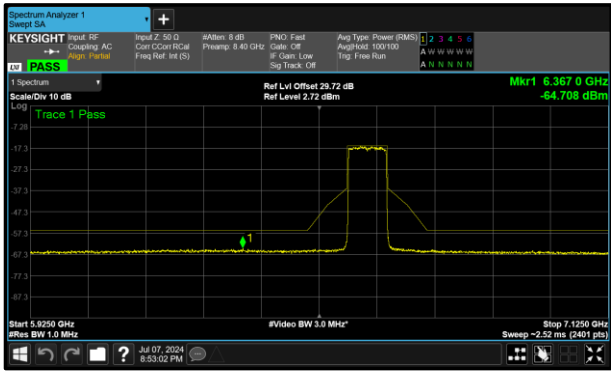
Figure 380 - A (Core 0) 6625 MHz (CH135)
