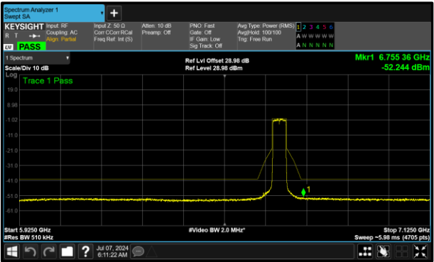
Figure 425 - B (Core 1) 6685 MHz (CH147)
