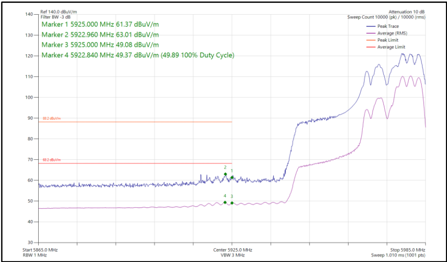
Figure 216 - 802.11ax HE40, SU, SDM, Core 0 - Core 1 - 5965 MHz Band Edge Frequency 5925 MHz
