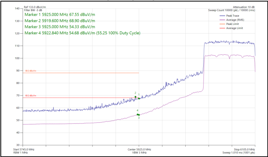
Figure 227 - 802.11ax HE80, RU 106-53, SISO, Core 0 - 5985 MHz Band Edge Frequency 5925 MHz
