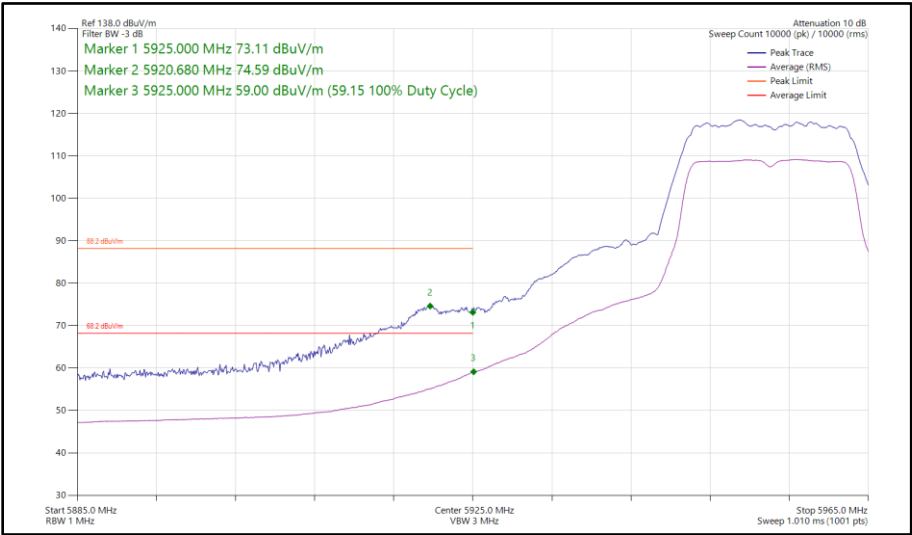
Figure 176 - 802.11a, SISO, Core 1 - 5955 MHz Band Edge Frequency 5925 MHz
