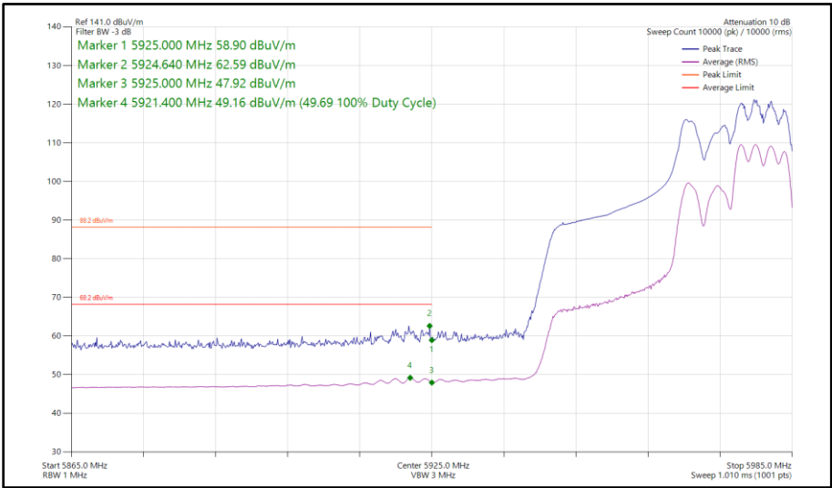
Figure 210 - 802.11ax HE40, SU, CDD, Core 0 - Core 1 - 5965 MHz Band Edge Frequency 5925 MHz
