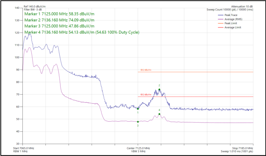
Figure 221 - 802.11ax HE40, RU 52-37, SDM, Core 0 - Core 1 - 7085 MHz Band Edge Frequency 7125 MHz
