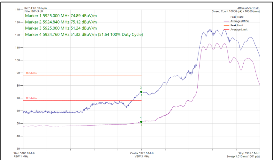
Figure 191 - 802.11ax HE20, RU 106-53, SDM, Core 0 - Core 1 - 5955 MHz Band Edge Frequency 5925 MHz
