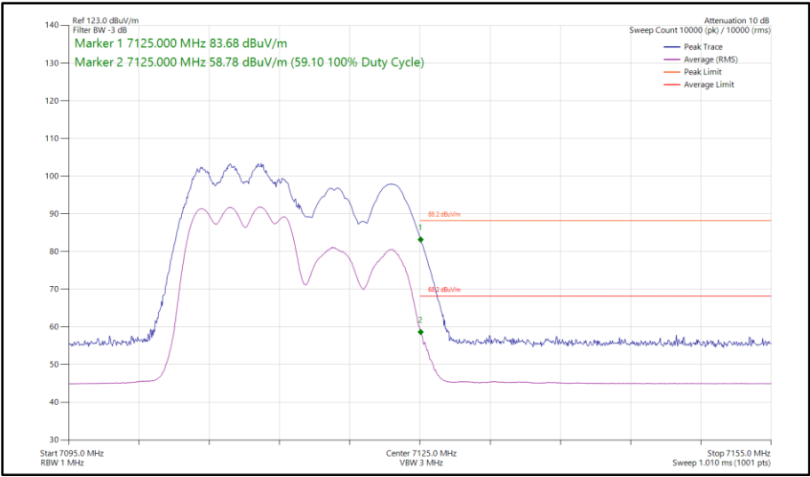
Figure 189 - 802.11ax HE20, RU 106-53, CDD, Core 0 - Core 1 - 7115 MHz Band Edge Frequency 7125 MHz
