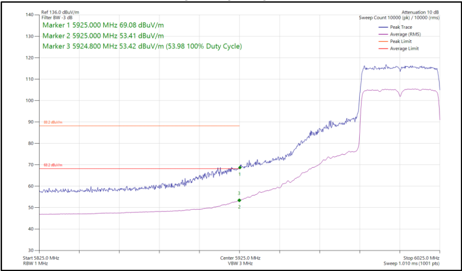
Figure 199 - 802.11ax HE40, RU 106-56, SISO, Core 0 - 5965 MHz Band Edge Frequency 5925 MHz
