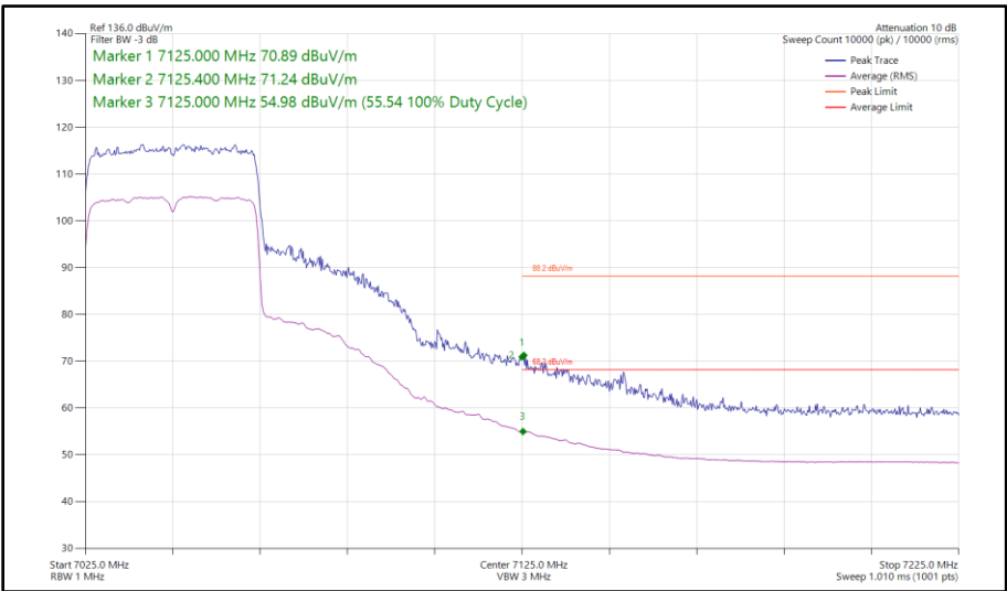
Figure 207 - 802.11ax HE40, SU, SISO, Core 1 - 7045 MHz Band Edge Frequency 7125 MHz
