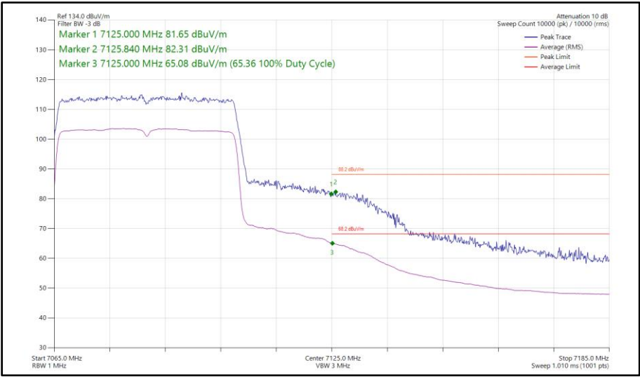
Figure 202 - 802.11ax HE40, SU, SISO, Core 0 - 7085 MHz Band Edge Frequency 7125 MHz
