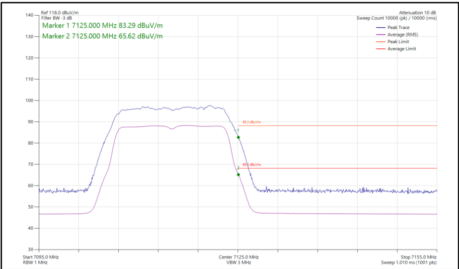
Figure 180 - 802.11a, SISO, Core 1 - 7115 MHz Band Edge Frequency 7125 MHz
