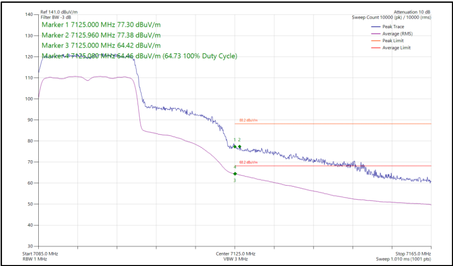
Figure 192 - 802.11ax HE20, SU, SDM, Core 0 - Core 1 - 7095 MHz Band Edge Frequency 7125 MHz
