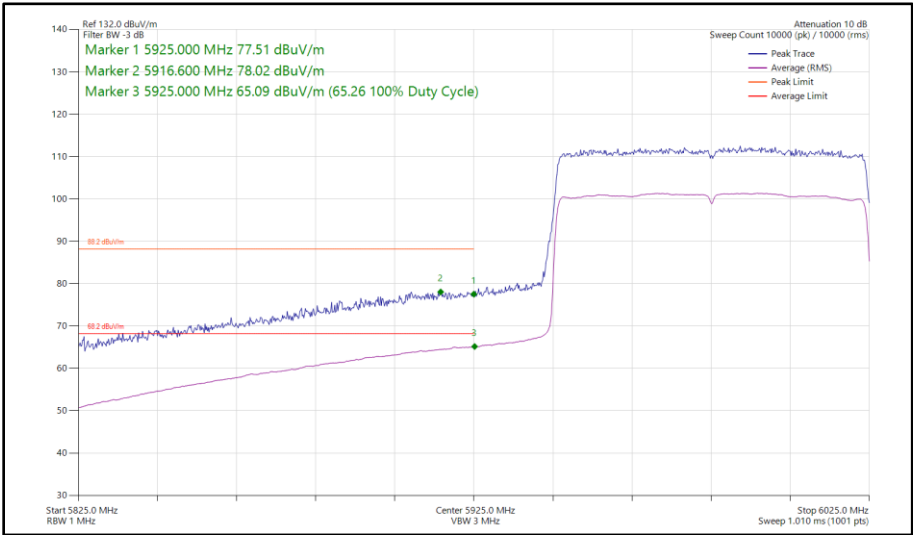
Figure 232 - 802.11ax HE80, SU, SISO, Core 1 - 5985 MHz Band Edge Frequency 5925 MHz
