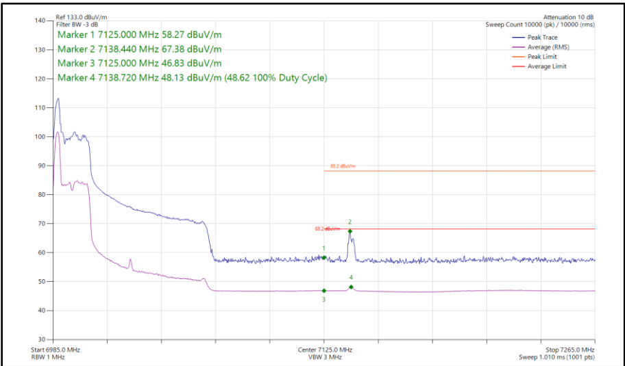
Figure 231 - 802.11ax HE80, RU 26-0, SISO, Core 0 - 7025 MHz Band Edge Frequency 7125 MHz
