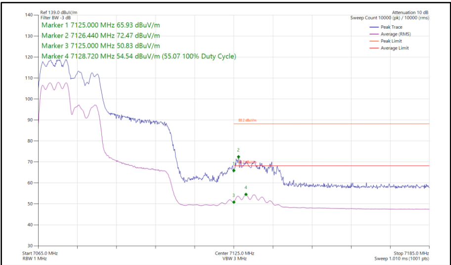
Figure 215 - 802.11ax HE40, RU 106-53, CDD, Core 0 - Core 1 - 7085 MHz Band Edge Frequency 7125 MHz
