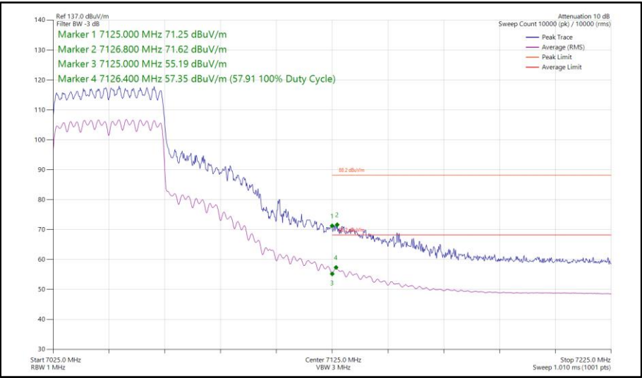
Figure 213 - 802.11ax HE40, SU, CDD, Core 0 - Core 1 - 7045 MHz Band Edge Frequency 7125 MHz
