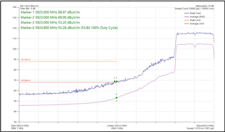
Figure 205 - 802.11ax HE40, RU 106-56, SISO, Core 1 - 5965 MHz Band Edge Frequency 5925 MHz
