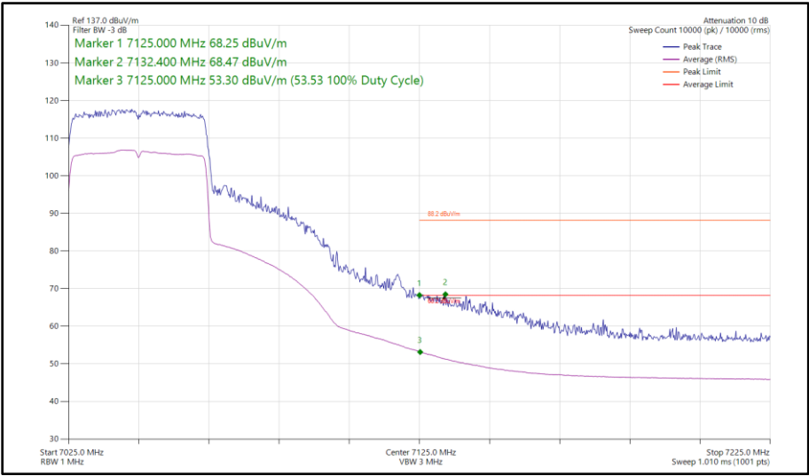
Figure 224 - 802.11ax HE40, SU, TxBF, Core 0 - Core 1 - 7045 MHz Band Edge Frequency 7125 MHz
