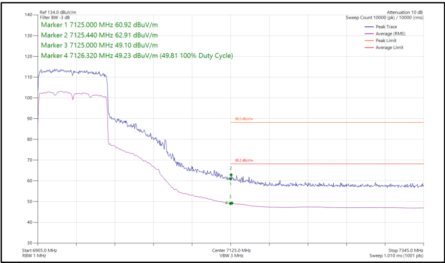
Figure 229 - 802.11ax HE80, SU, SISO, Core 0 - 6945 MHz Band Edge Frequency 7125 MHz
