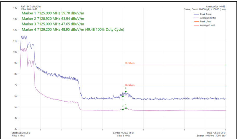
Figure 243 - 802.11ax HE80, RU 106-53, CDD, Core 0 - Core 1 - 7025 MHz Band Edge Frequency 7125 MHz
