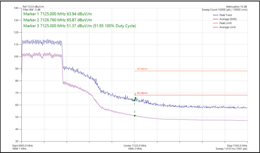
Figure 241 - 802.11ax HE80, SU, CDD, Core 0 - Core 1 - 6945 MHz Band Edge Frequency 7125 MHz
