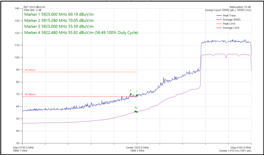
Figure 233 - 802.11ax HE80, RU 106-60, SISO, Core 1 - 5985 MHz Band Edge Frequency 5925 MHz
