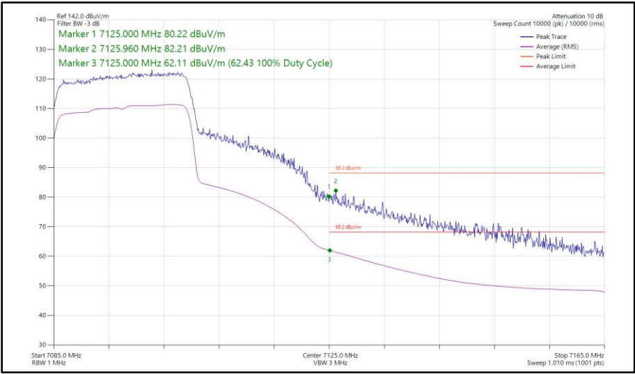
Figure 197 - 802.11ax HE20, SU, TxBF, Core 0 - Core 1 - 7095 MHz Band Edge Frequency 7125 MHz
