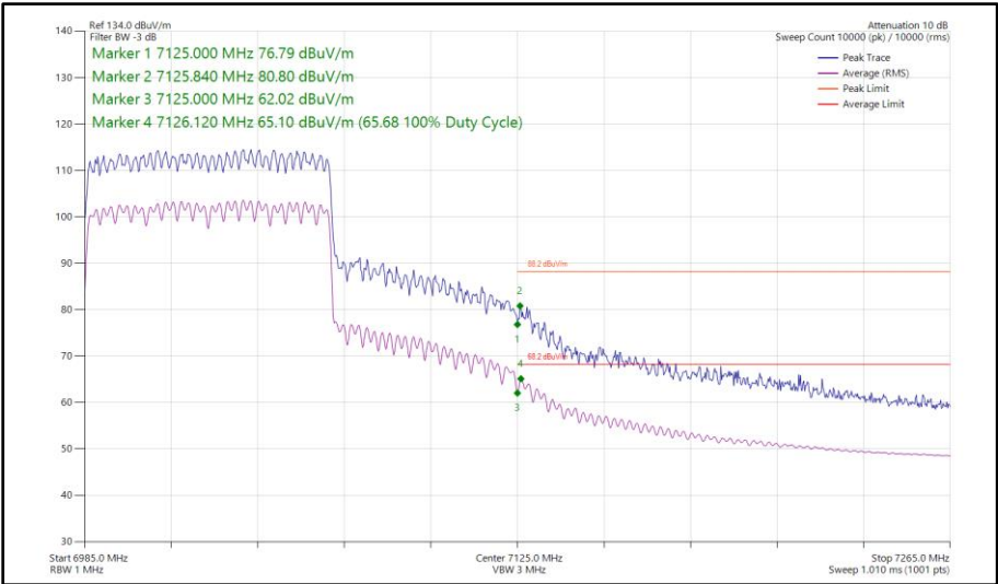
Figure 242 - 802.11ax HE80, SU, CDD, Core 0 - Core 1 - 7025 MHz Band Edge Frequency 7125 MHz
