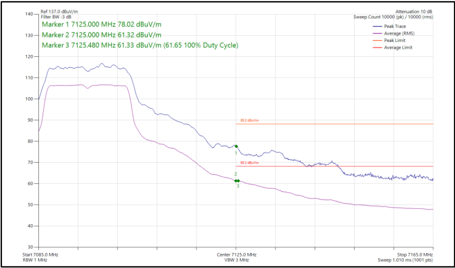
Figure 179 - 802.11a, SISO, Core 1 - 7095 MHz Band Edge Frequency 7125 MHz
