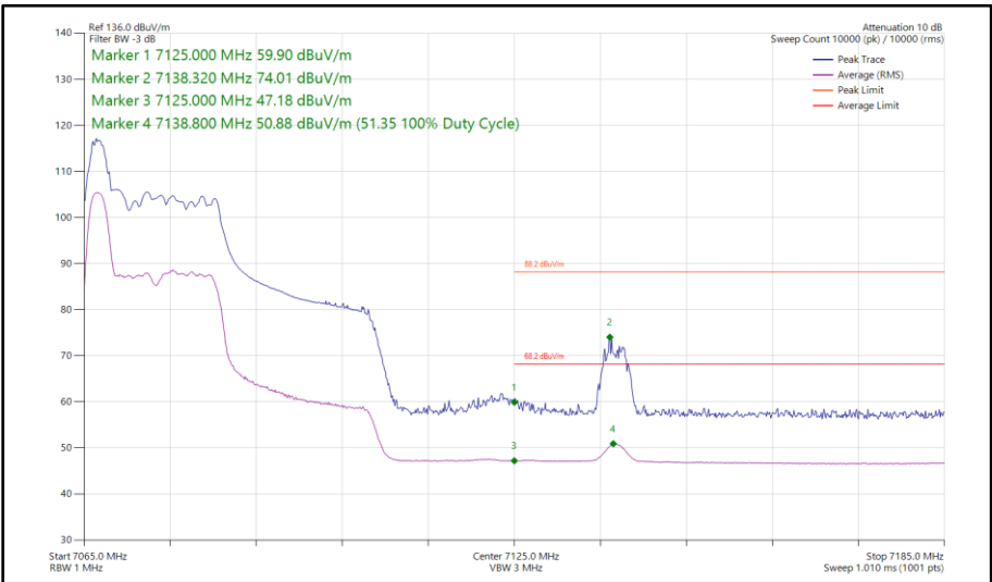
Figure 203 - 802.11ax HE40, RU 26-0, SISO, Core 0 - 7085 MHz Band Edge Frequency 7125 MHz
