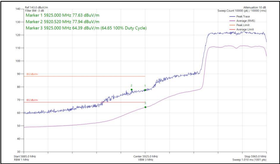
Figure 190 - 802.11ax HE20, SU, SDM, Core 0 - Core 1 - 5955 MHz Band Edge Frequency 5925 MHz
