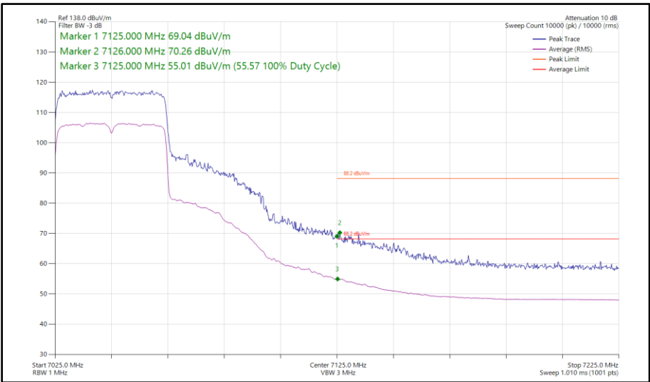
Figure 201 - 802.11ax HE40, SU, SISO, Core 0 - 7045 MHz Band Edge Frequency 7125 MHz
