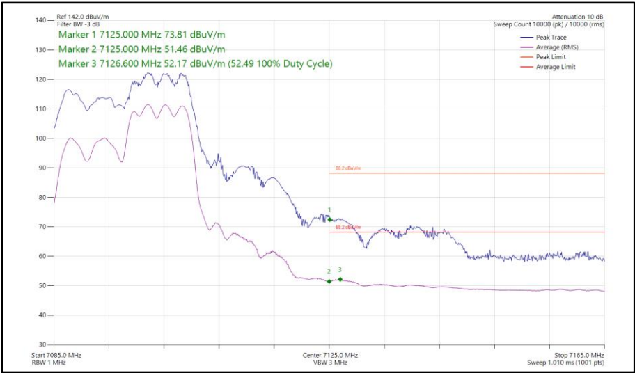
Figure 188 - 802.11ax HE20, RU 106-54, CDD, Core 0 - Core 1 - 7095 MHz Band Edge Frequency 7125 MHz
