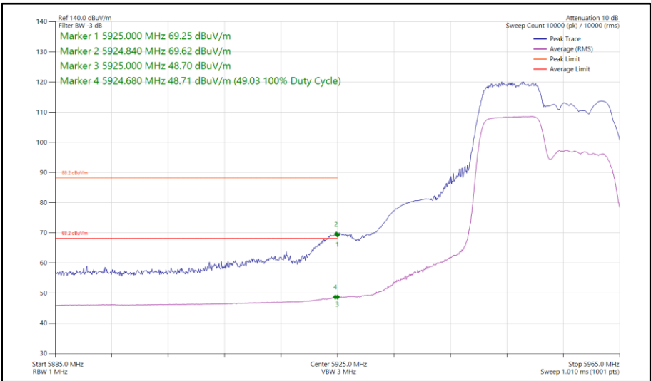
Figure 178 - 802.11ax HE20, RU 106-53, SISO, Core 1 - 5955 MHz Band Edge Frequency 5925 MHz
