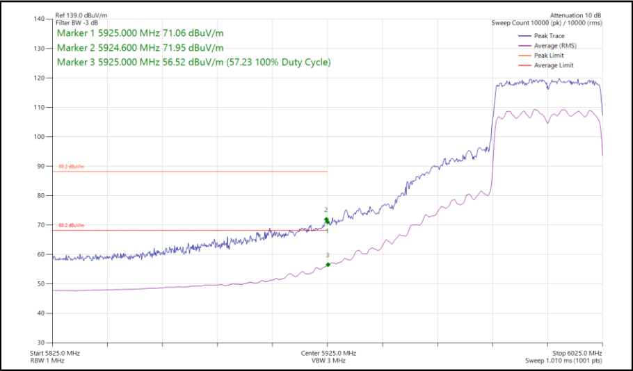
Figure 217 - 802.11ax HE40, RU 106-56, SDM, Core 0 - Core 1 - 5965 MHz Band Edge Frequency 5925 MHz
