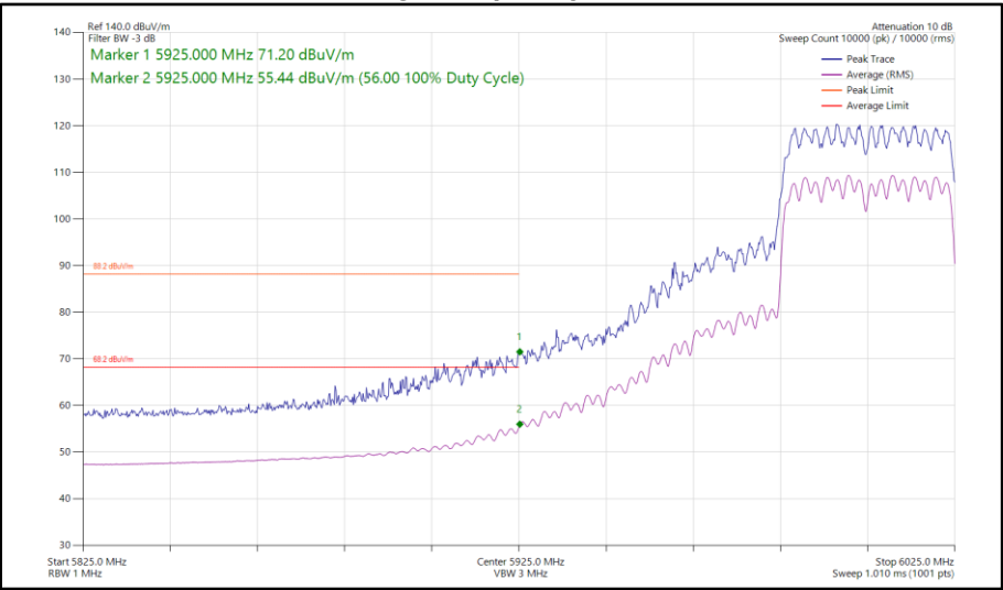
Figure 211 - 802.11ax HE40, RU 106-56, CDD, Core 0 - Core 1 - 5965 MHz Band Edge Frequency 5925 MHz
