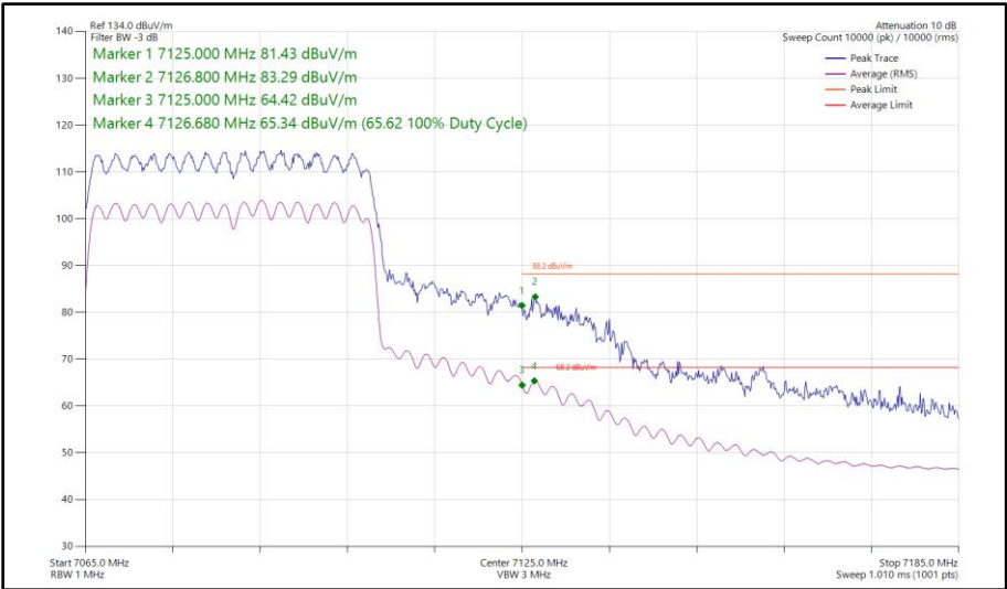
Figure 214 - 802.11ax HE40, SU, CDD, Core 0 - Core 1 - 7085 MHz Band Edge Frequency 7125 MHz
