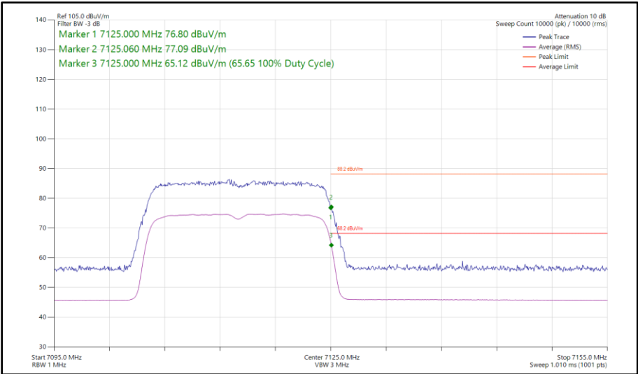
Figure 183 - 802.11ax HE20, SU, SISO, Core 1 - 7115 MHz Band Edge Frequency 7125 MHz
