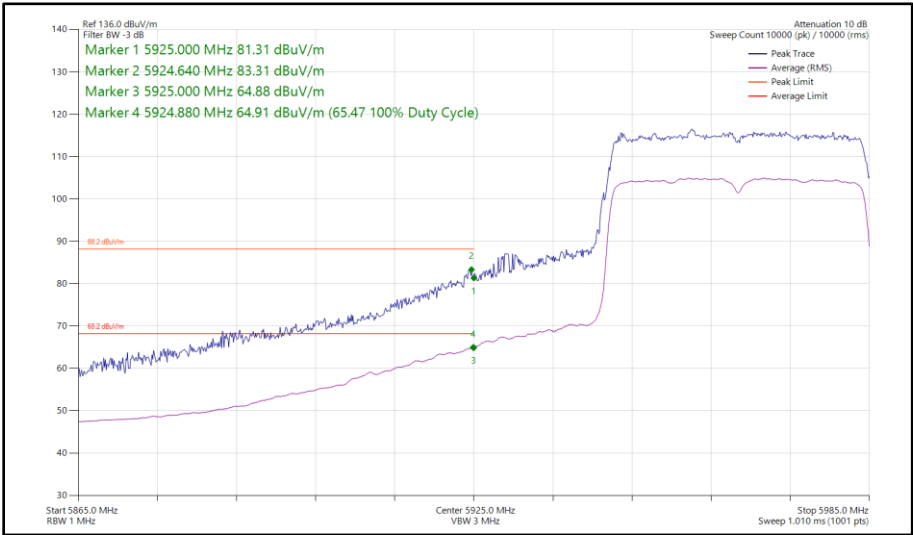
Figure 198 - 802.11ax HE40, SU, SISO, Core 0 - 5965 MHz Band Edge Frequency 5925 MHz
