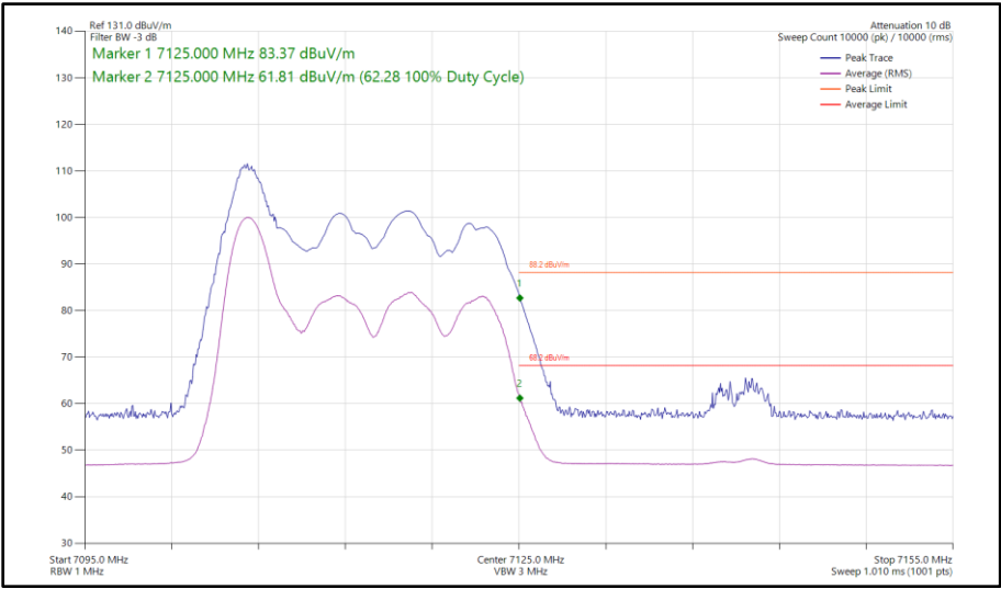
Figure 194 - 802.11ax HE20, RU 26-0, SDM, Core 0 - Core 1 - 7115 MHz Band Edge Frequency 7125 MHz
