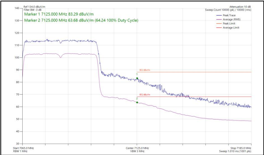
Figure 208 - 802.11ax HE40, SU, SISO, Core 1 - 7085 MHz Band Edge Frequency 7125 MHz
