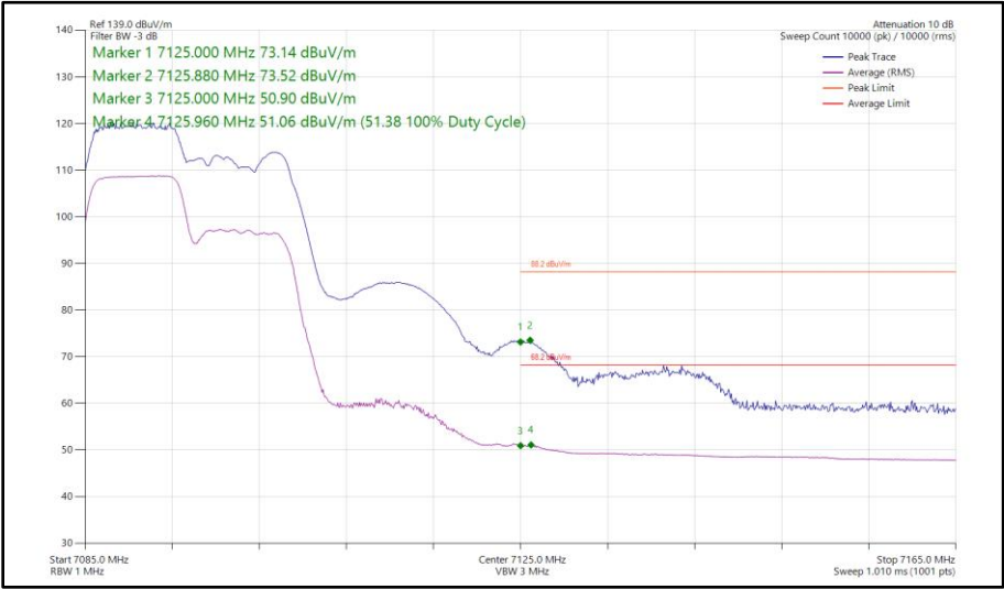
Figure 182 - 802.11ax HE20, RU 106-53, SISO, Core 1 - 7095 MHz Band Edge Frequency 7125 MHz
