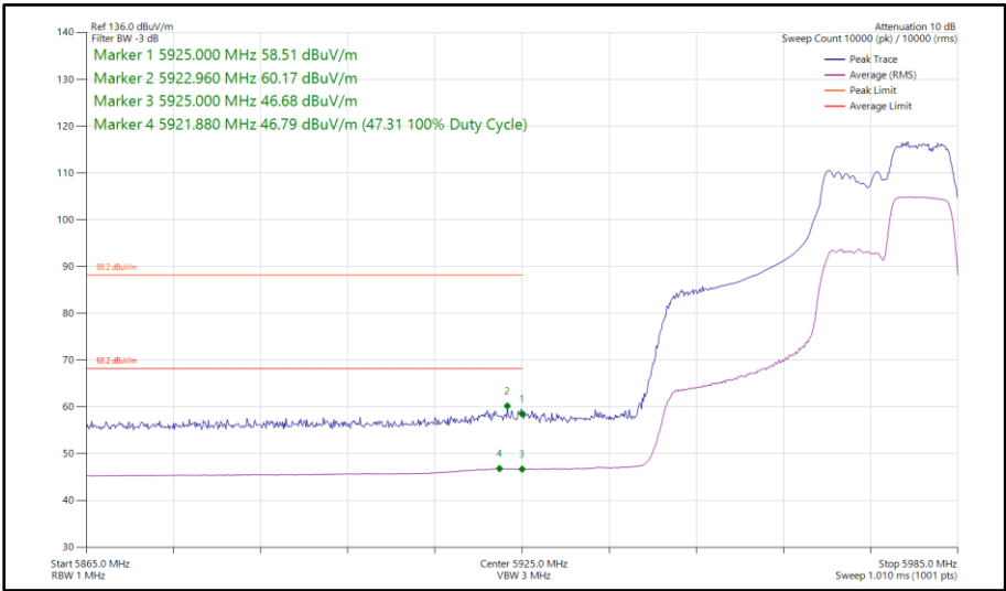
Figure 204 - 802.11ax HE40, SU, SISO, Core 1 - 5965 MHz Band Edge Frequency 5925 MHz
