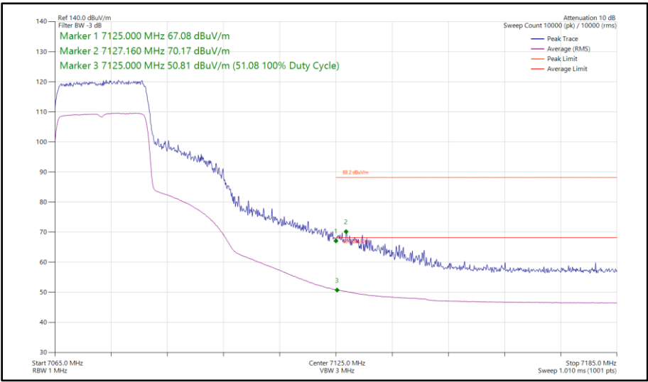
Figure 196 - 802.11ax HE20, SU, TxBF, Core 0 - Core 1 - 7075 MHz Band Edge Frequency 7125 MHz
