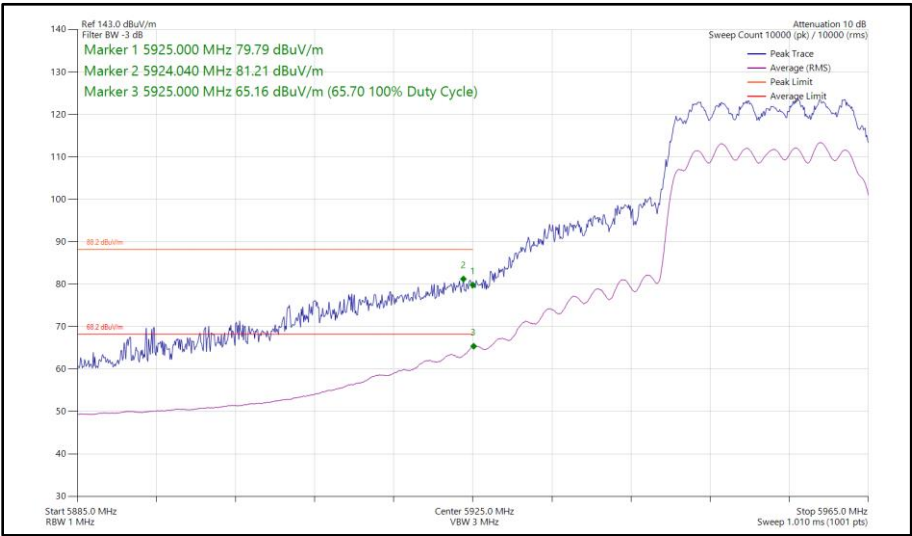
Figure 185 - 802.11ax HE20, SU, CDD, Core 0 - Core 1 - 5955 MHz Band Edge Frequency 5925 MHz
