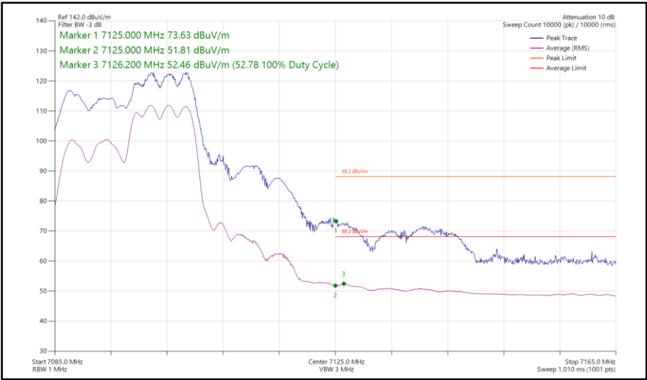
Figure 193 - 802.11ax HE20, RU 106-54, SDM, Core 0 - Core 1 - 7095 MHz Band Edge Frequency 7125 MHz
