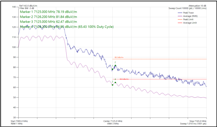
Figure 187 - 802.11ax HE20, SU, CDD, Core 0 - Core 1 - 7095 MHz Band Edge Frequency 7125 MHz
