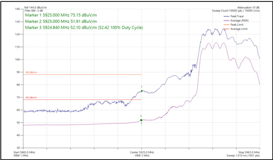
Figure 186 - 802.11ax HE20, RU 106-53, CDD, Core 0 - Core 1 - 5955 MHz Band Edge Frequency 5925 MHz
