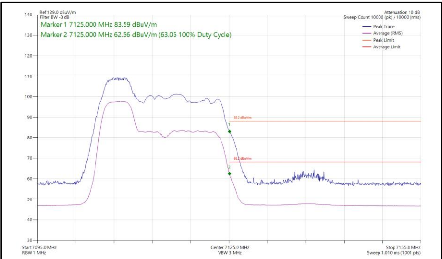
Figure 184 - 802.11ax HE20, RU 52-37, SISO, Core 1 - 7115 MHz Band Edge Frequency 7125 MHz
