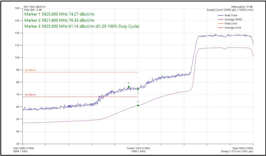
Figure 177 - 802.11ax HE20, SU, SISO, Core 1 - 5955 MHz Band Edge Frequency 5925 MHz
