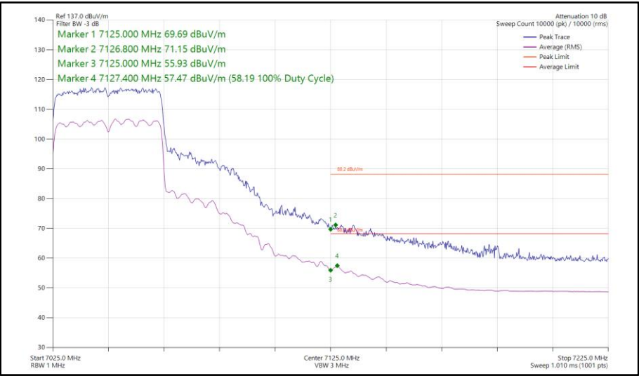
Figure 219 - 802.11ax HE40, SU, SDM, Core 0 - Core 1 - 7045 MHz Band Edge Frequency 7125 MHz
