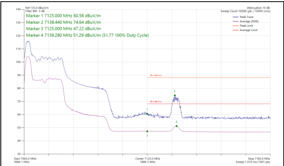
Figure 209 - 802.11ax HE40, RU 26-0, SISO, Core 1 - 7085 MHz Band Edge Frequency 7125 MHz
