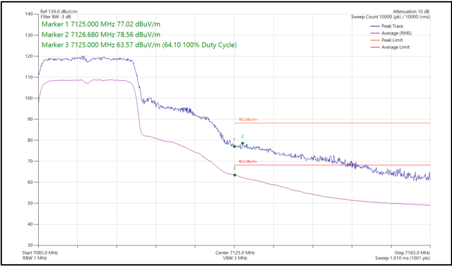
Figure 181 - 802.11ax HE20, SU, SISO, Core 1 - 7095 MHz Band Edge Frequency 7125 MHz
