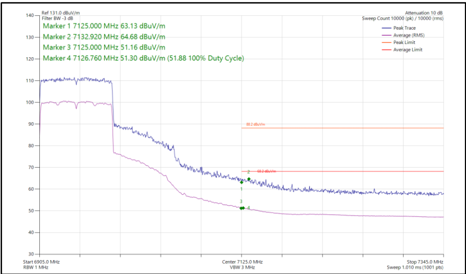
Figure 235 - 802.11ax HE80, SU, SISO, Core 1 - 6945 MHz Band Edge Frequency 7125 MHz
