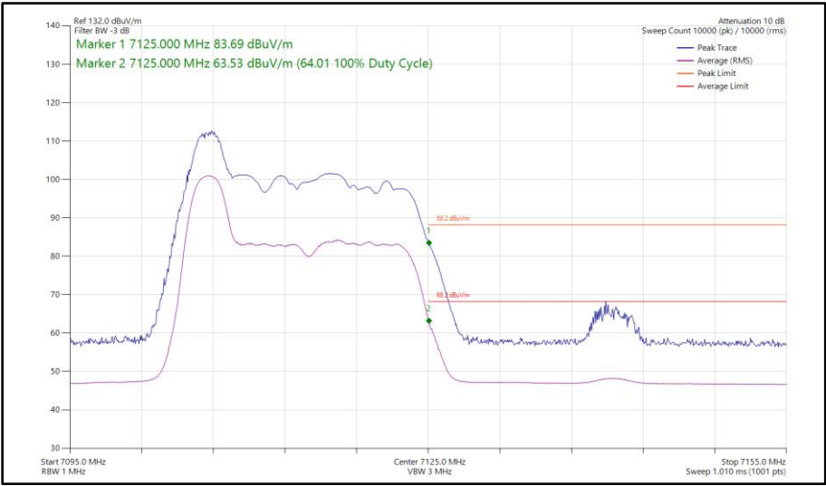
Figure 175 - 802.11ax HE20, RU 26-0, SISO, Core 0 - 7115 MHz Band Edge Frequency 7125 MHz
