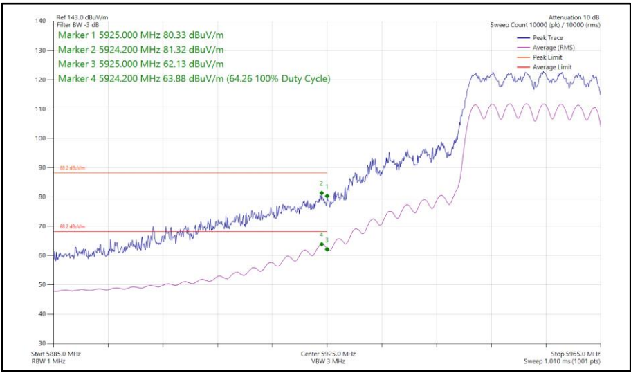
Figure 195 - 802.11ax HE20, SU, TxBF, Core 0 - Core 1 - 5955 MHz Band Edge Frequency 5925 MHz
