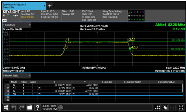
Figure 113 - 802.11ax HE80 SU LPI Minimum 26 dB EBW
