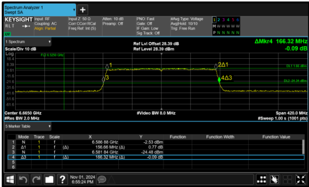
Figure 115 - 802.11ax HE160 SU LPI Minimum 26 dB EBW
