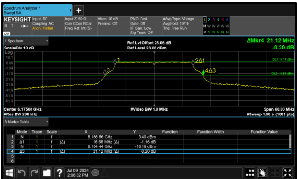
Figure 2 - 802.11a SP Maximum 26 dB EBW
