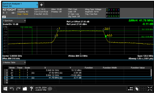
Figure 5 - 802.11ax HE40 SU SP Minimum 26 dB EBW
