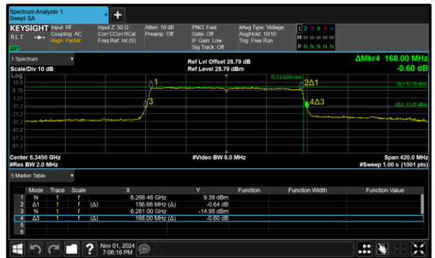
Figure 10 - 802.11ax HE160 SU SP Maximum 26 dB EBW
