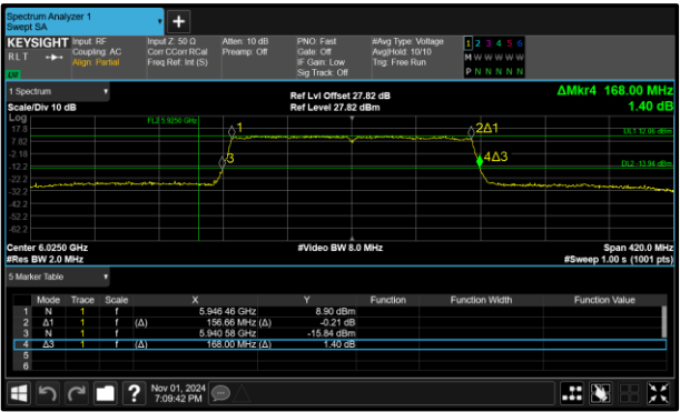
Figure 68 - 802.11ax HE160 SU SP Maximum 26 dB EBW
