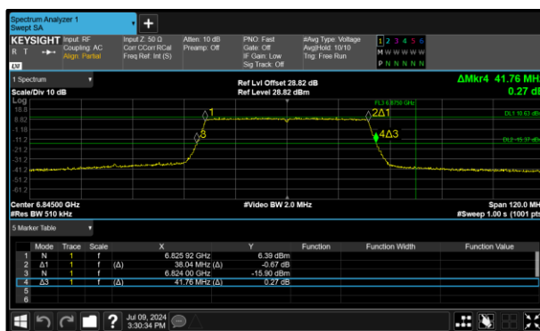
Figure 63 - 802.11ax HE40 SU SP Minimum 26 dB EBW
