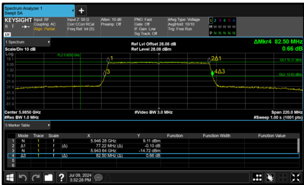
Figure 65 - 802.11ax HE80 SU SP Minimum 26 dB EBW
