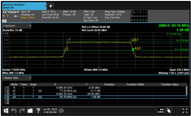
Figure 18 - 802.11ax HE80 SU LPI Maximum 26 dB EBW
