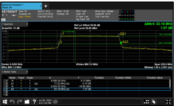
Figure 66 - 802.11ax HE80 SU SP Maximum 26 dB EBW
