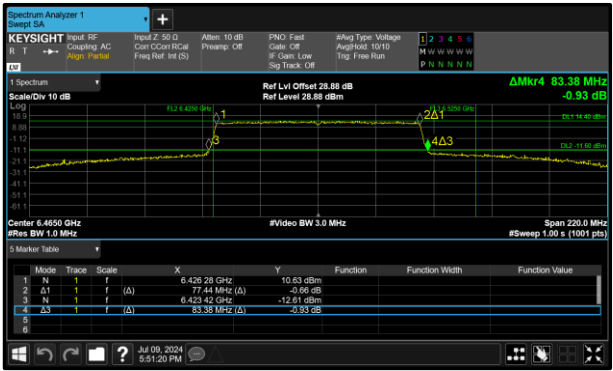
Figure 8 - 802.11ax HE80 SU SP Maximum 26 dB EBW
