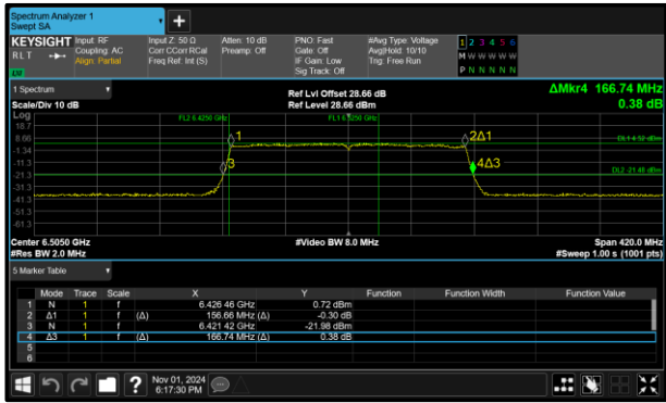
Figure 19 - 802.11ax HE160 SU LPI Minimum 26 dB EBW
