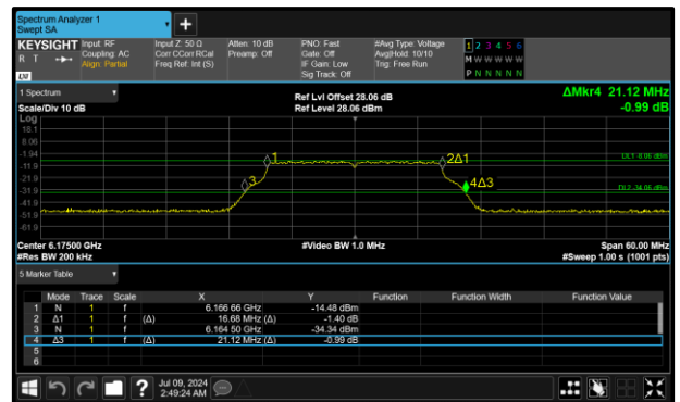
Figure 42 - 802.11a LPI Maximum 99% OBW
