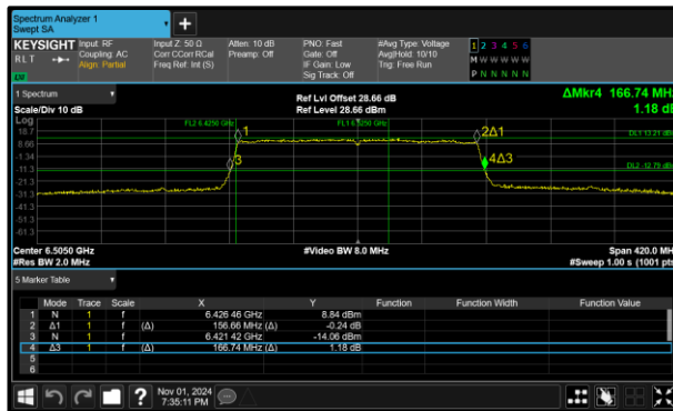
Figure 9 - 802.11ax HE160 SU SP Minimum 26 dB EBW
