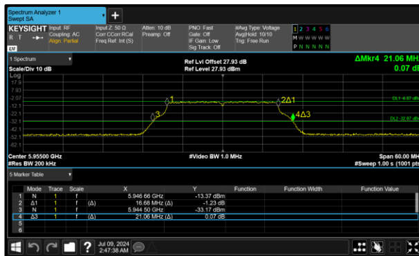
Figure 11 - 802.11a LPI Minimum 26 dB EBW
