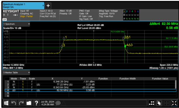
Figure 17 - 802.11ax HE80 SU LPI Minimum 26 dB EBW
