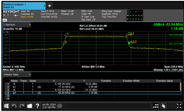
Figure 7 - 802.11ax HE80 SU SP Minimum 26 dB EBW
