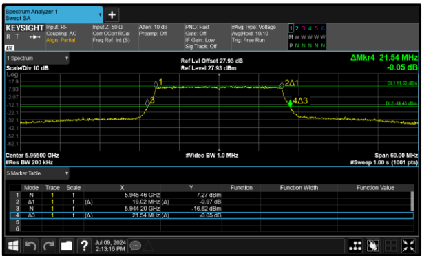
Figure 4 - 802.11ax HE20 SU SP Maximum 26 dB EBW
