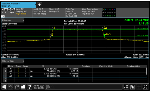
Figure 38 - 802.11ax HE80 SU SP Maximum 99% OBW
