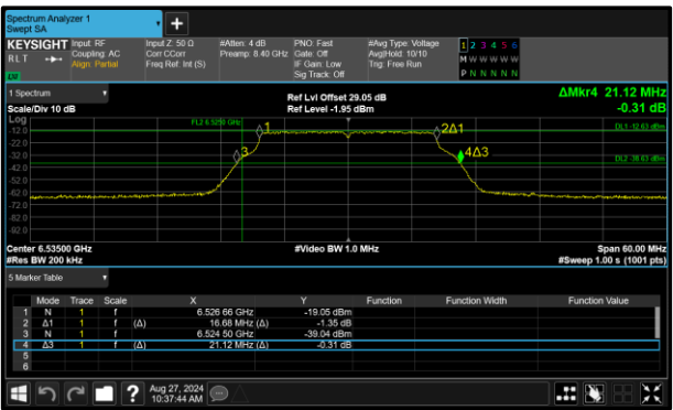
Figure 52 - 802.11a VLP Maximum 99% OBW
