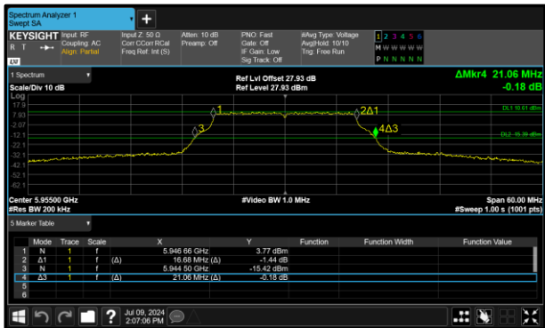
Figure 1 - 802.11a SP Minimum 26 dB EBW
