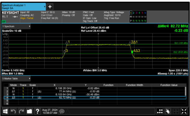
Figure 58 - 802.11ax HE80 SU VLP Maximum 99% OBW
