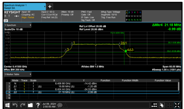
Figure 12 - 802.11a LPI Maximum 26 dB EBW
