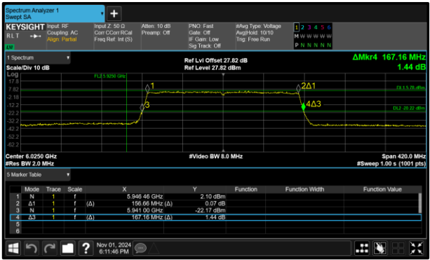
Figure 20 - 802.11ax HE160 SU LPI Maximum 26 dB EBW
