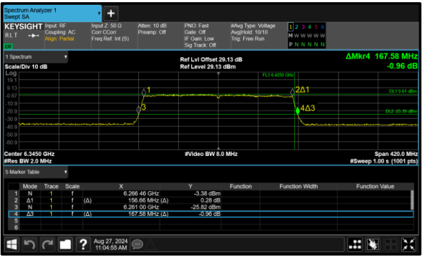
Figure 60 - 802.11ax HE160 SU VLP Maximum 99% OBW
