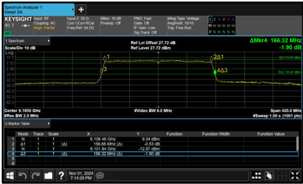
Figure 67 - 802.11ax HE160 SU SP Minimum 26 dB EBW
