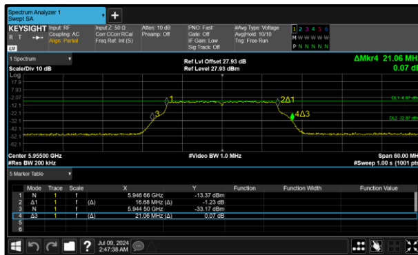
Figure 41 - 802.11a LPI Minimum 99% OBW
