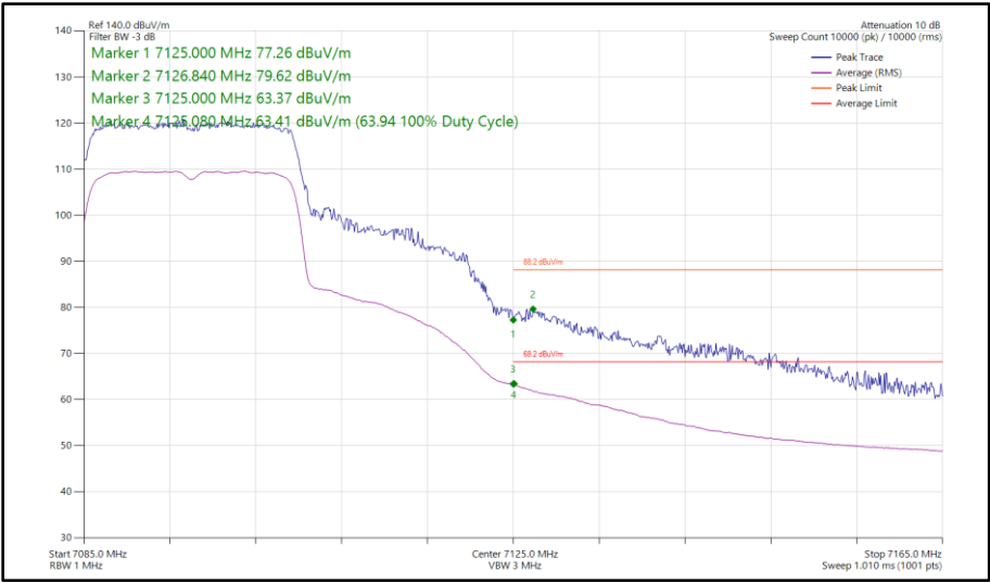
Figure 173 - 802.11ax HE20, SU, SISO, Core 0 - 7095 MHz Band Edge Frequency 7125 MHz
