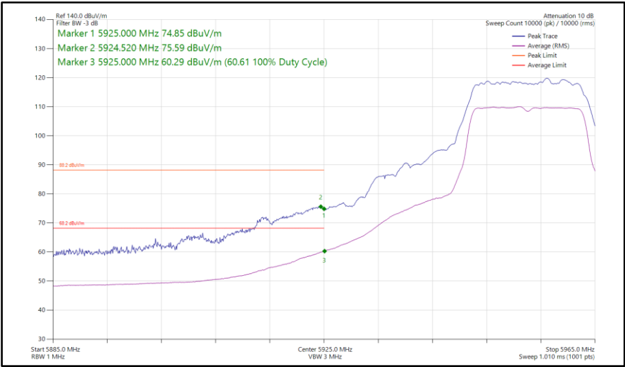
Figure 168 - 802.11a, SISO, Core 0 - 5955 MHz Band Edge Frequency 5925 MHz
