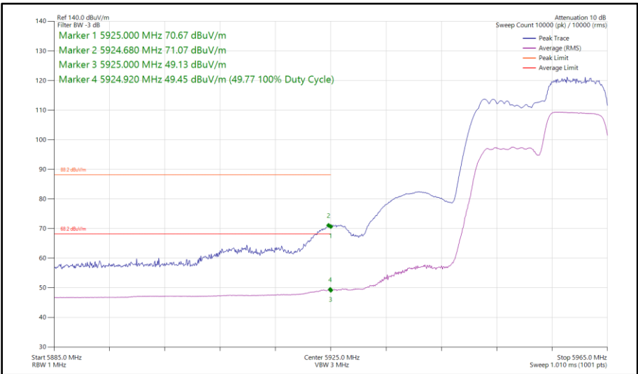
Figure 170 - 802.11ax HE20, RU 106-54, SISO, Core 0 - 5955 MHz Band Edge Frequency 5925 MHz
