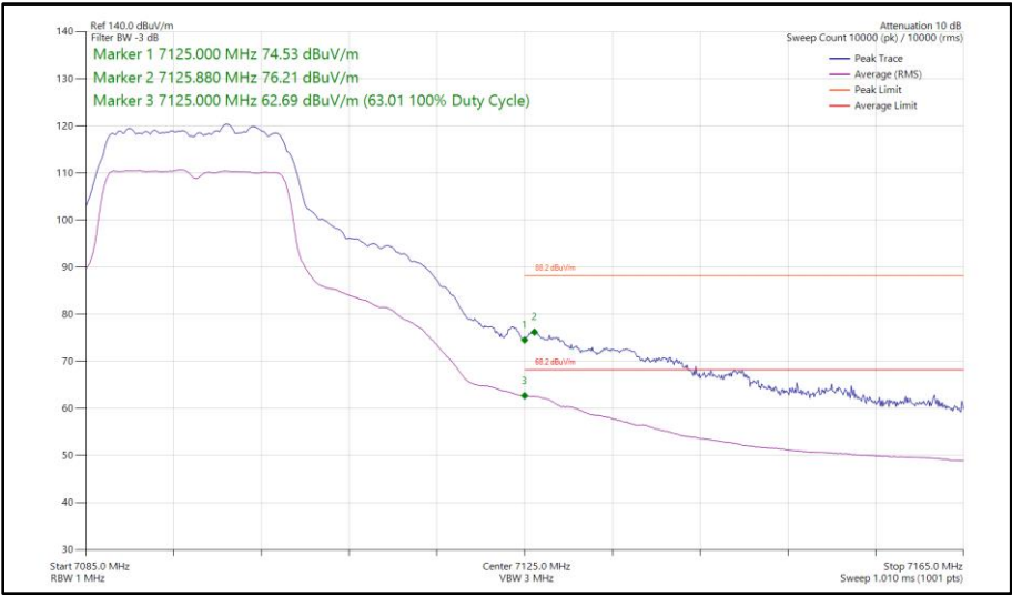
Figure 171 - 802.11a, SISO, Core 0 - 7095 MHz Band Edge Frequency 7125 MHz
