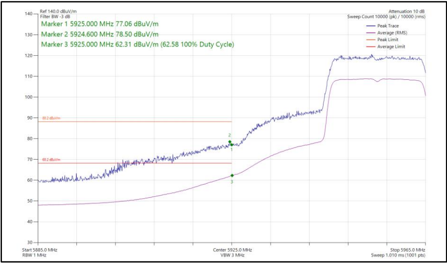
Figure 169 - 802.11ax HE20, SU, SISO, Core 0 - 5955 MHz Band Edge Frequency 5925 MHz
