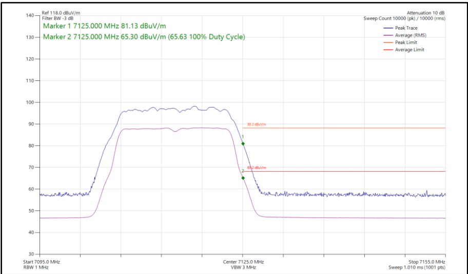
Figure 172 - 802.11a, SISO, Core 0 - 7115 MHz Band Edge Frequency 7125 MHz
