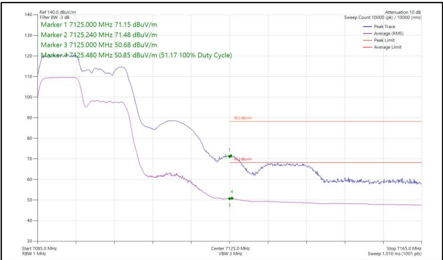
Figure 174 - 802.11ax HE20, RU 106-53, SISO, Core 0 - 7095 MHz Band Edge Frequency 7125 MHz
