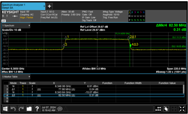
Figure 164 - 802.11ax HE80 SU SP Maximum 99% OBW
