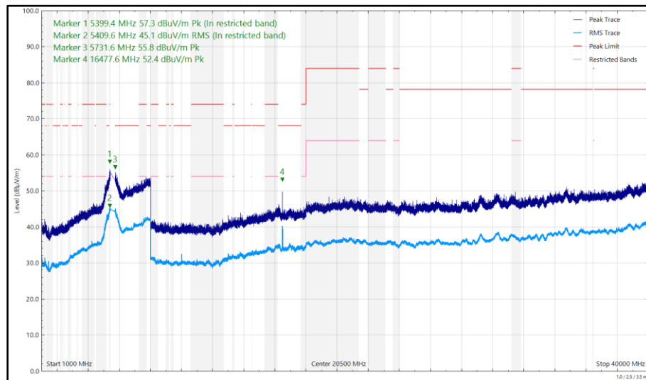
Figure 729 - U-NII-2C - 5500 MHz (CH100), HE20, RU52-37, CDD, Core 0 + Core 1, 1 GHz to 40 GHz, Vertical
