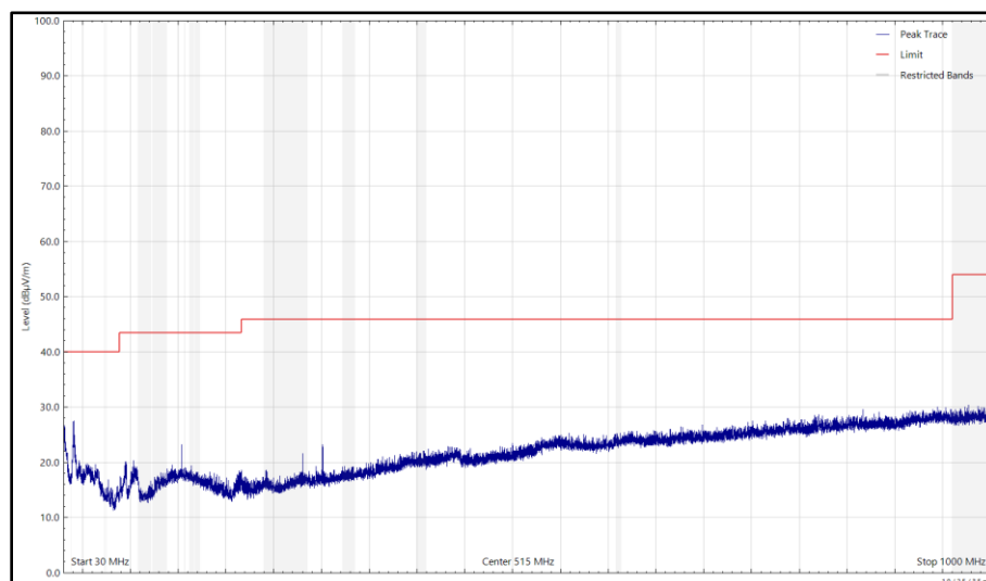
Figure 736 - U-NII-3 - 5825 MHz (CH165), HE20, RU26-0, CDD, Core 0 + Core 1, 30 MHz to 1 GHz, Vertical (Peak)
