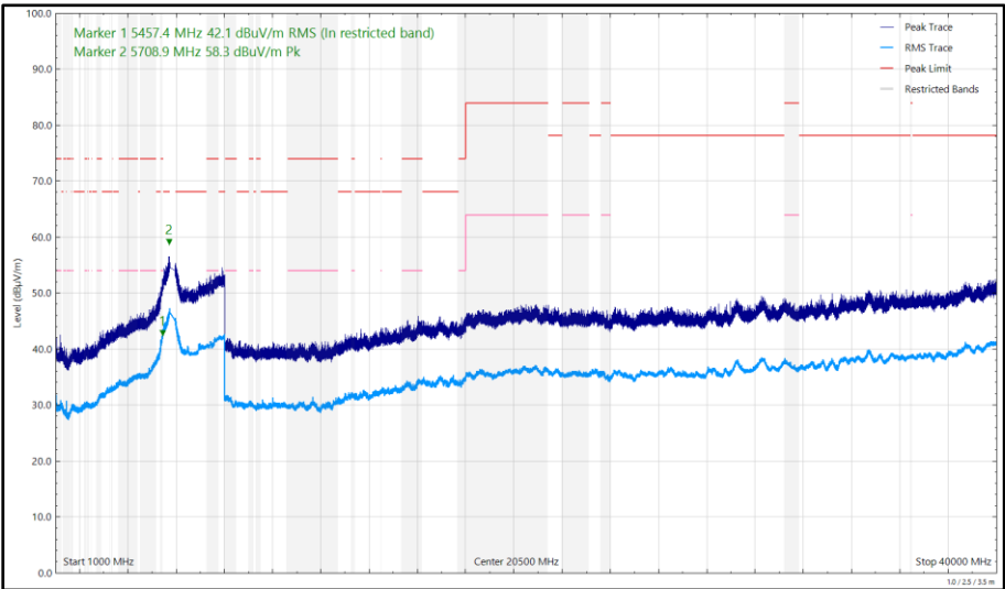
Figure 721 - U-NII-3 - 5825 MHz (CH165), HT20, CDD, Core 0 + Core 1, 1 GHz to 40 GHz, Vertical
