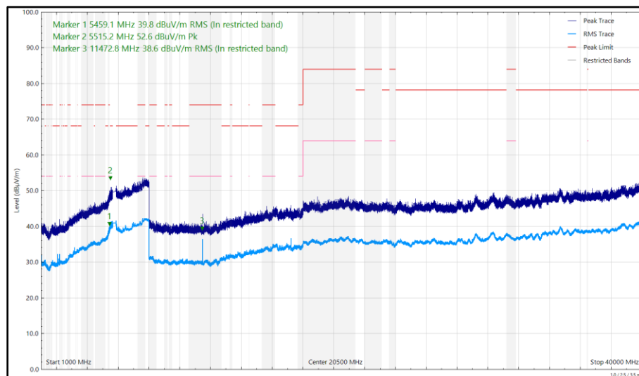
Figure 732 - U-NII-3 - 5745 MHz (CH149), HE20, RU26-0, CDD, Core 0 + Core 1, 1 GHz to 40 GHz, Horizontal
