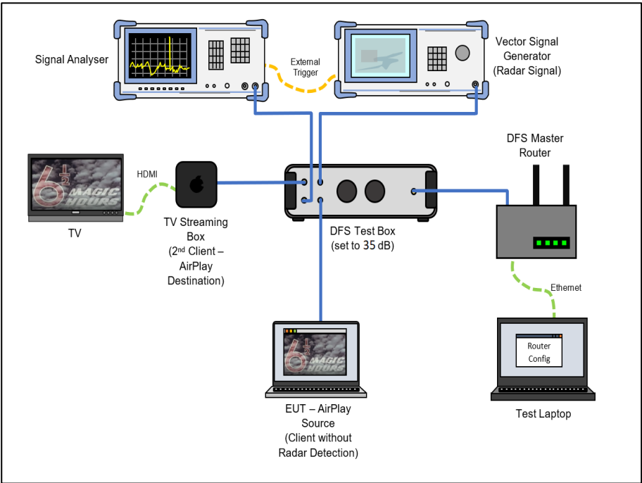
Figure 744- Test Equipment Setup Diagram for Client without Radar Detection with Injection at the Master
