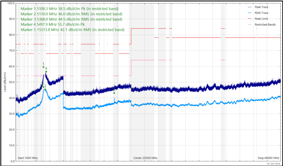
Figure 725 - U-NII-1 - 5180 MHz (CH36), HE20, RU26-0, CDD, Core 0 + Core 1, 1 GHz to 40 GHz, Vertical
