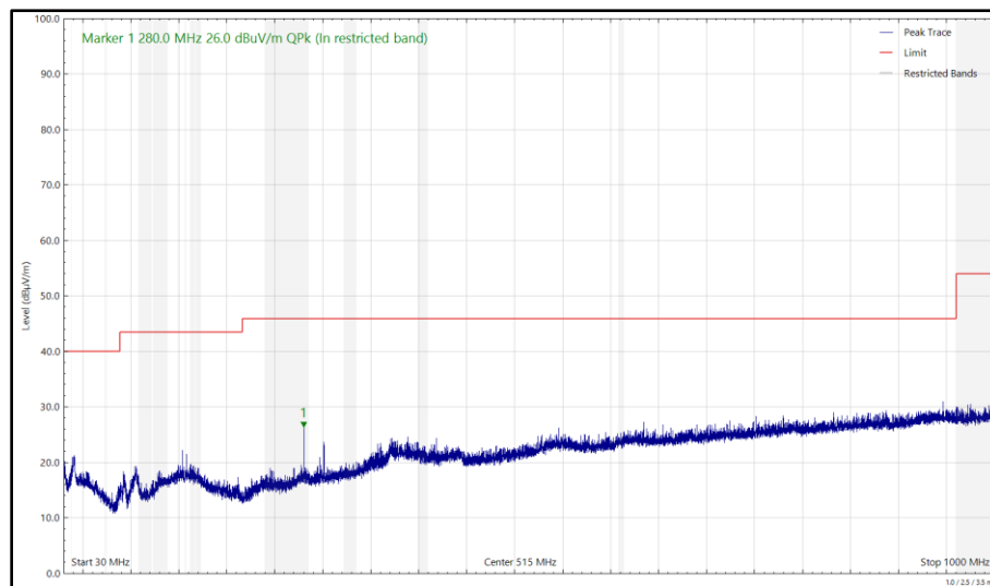
Figure 722 - U-NII-1 - 5180 MHz (CH36), HE20, RU26-0, CDD, Core 0 + Core 1, 30 MHz to 1 GHz, Horizontal (Peak)
