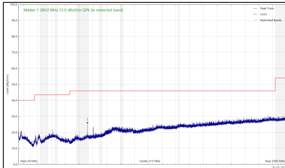
Figure 734 - U-NII-3 - 5825 MHz (CH165), HE20, RU26-0, CDD, Core 0 + Core 1, 30 MHz to 1 GHz, Horizontal (Peak)
