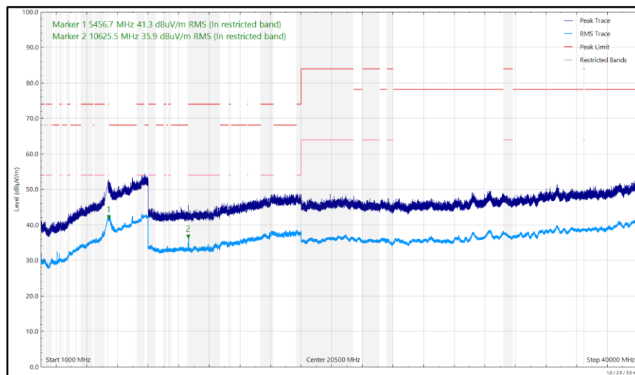
Figure 726 - U-NII-2A - 5320 MHz (CH64), HE20, RU52-37, CDD, Core 0 + Core 1, 1 GHz to 40 GHz, Horizontal
