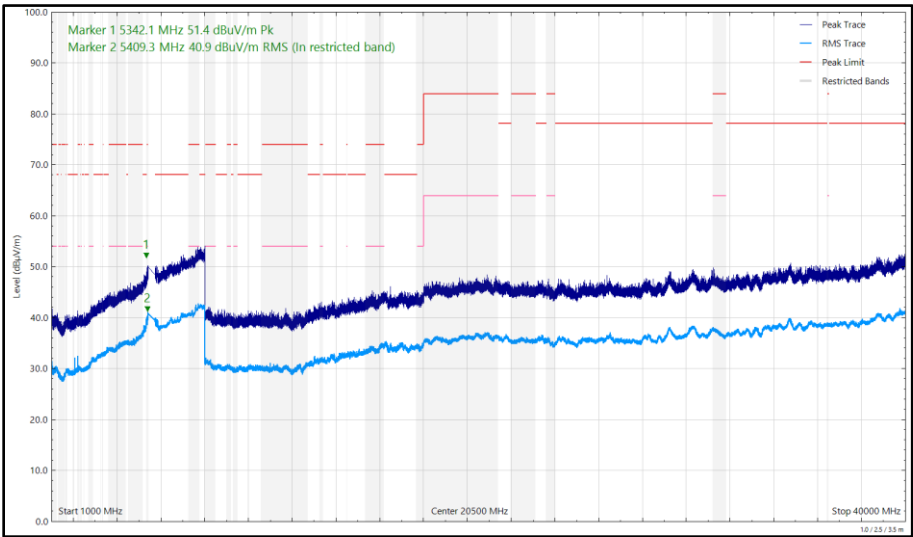
Figure 728 - U-NII-2C - 5500 MHz (CH100), HE20, RU52-37, CDD, Core 0 + Core 1, 1 GHz to 40 GHz, Horizontal
