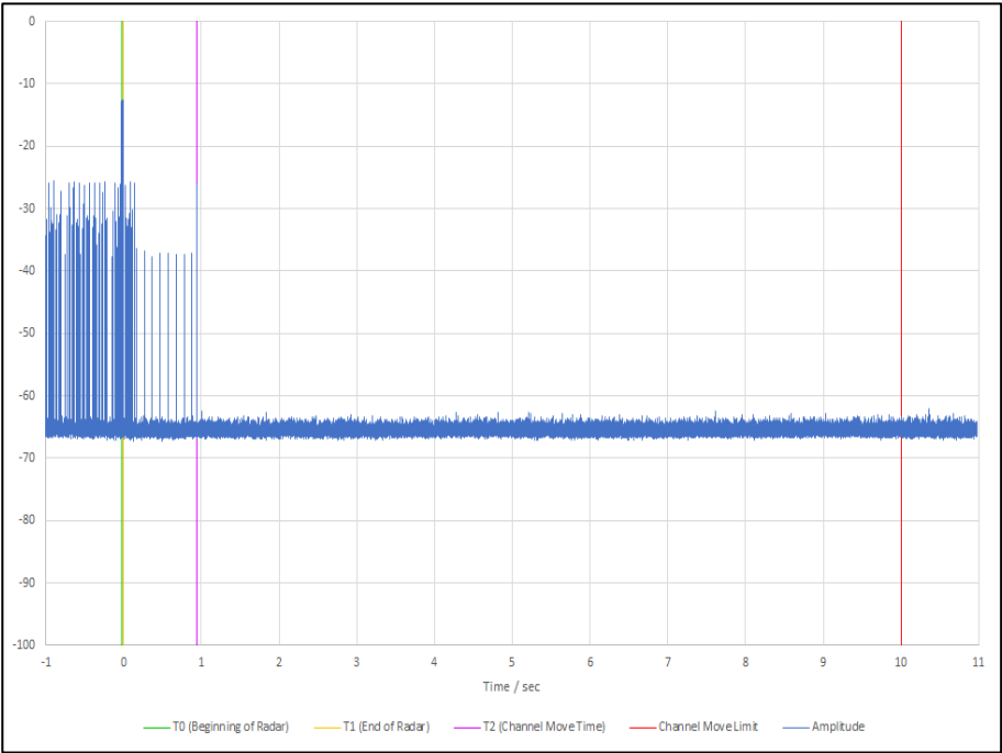
Figure 748 - First 12 s of Channel Shutdown Period
