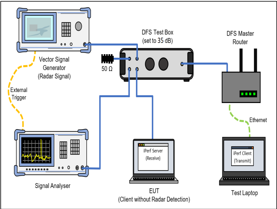
Figure 738- Test Equipment Setup Diagram for Client without Radar Detection with Injection at the Master
