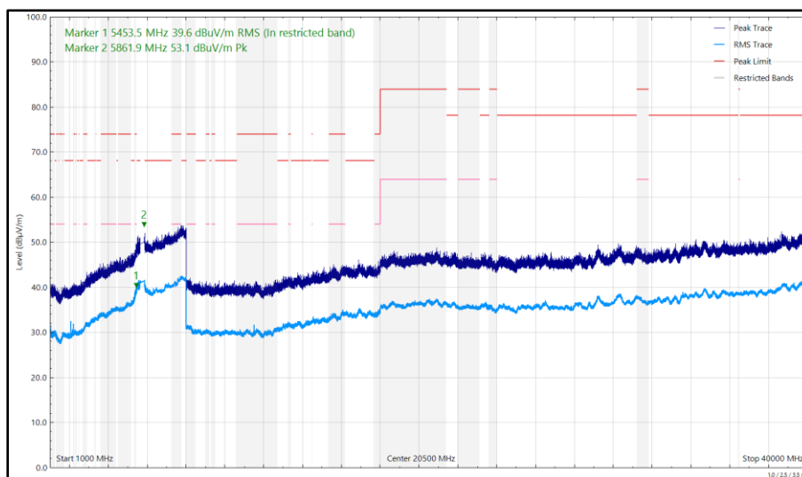
Figure 716 - U-NII-3 - 5745 MHz (CH149), HT20, CDD, Core 0 + Core 1, 1 GHz to 40 GHz, Horizontal
