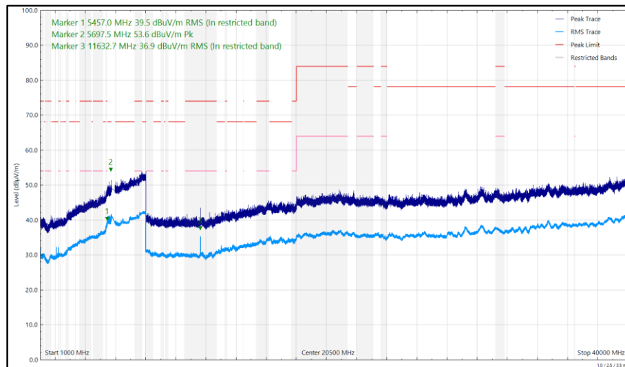
Figure 735 - U-NII-3 - 5825 MHz (CH165), HE20, RU26-0, CDD, Core 0 + Core 1, 1 GHz to 40 GHz, Horizontal
