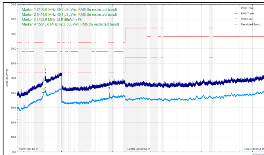
Figure 723 - U-NII-1 - 5180 MHz (CH36), HE20, RU26-0, CDD, Core 0 + Core 1, 1 GHz to 40 GHz, Horizontal
