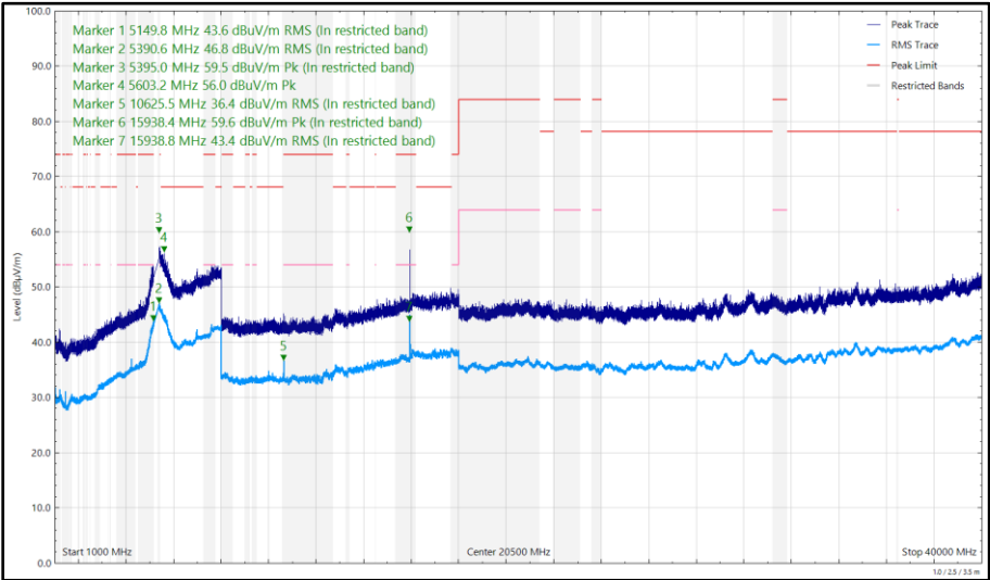
Figure 727 - U-NII-2A - 5320 MHz (CH64), HE20, RU52-37, CDD, Core 0 + Core 1, 1 GHz to 40 GHz, Vertical
