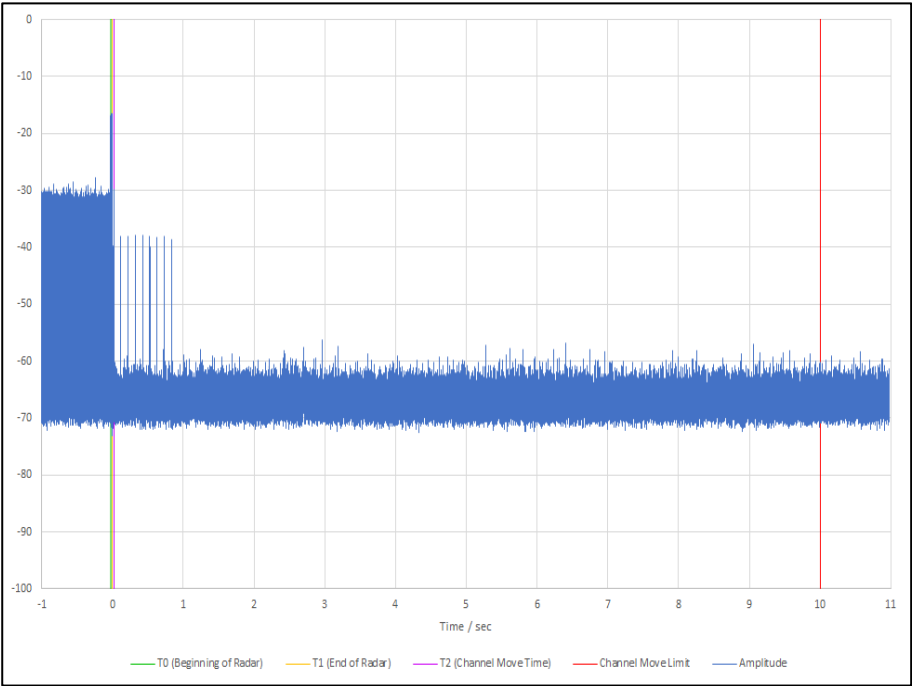
Figure 742 - First 12 s of Channel Shutdown Period
