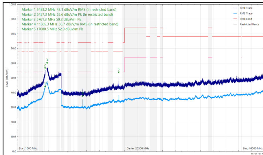
Figure 731 - U-NII-2C - 5700 MHz (CH140), HE20, RU52-37, CDD, Core 0 + Core 1, 1 GHz to 40 GHz, Vertical
