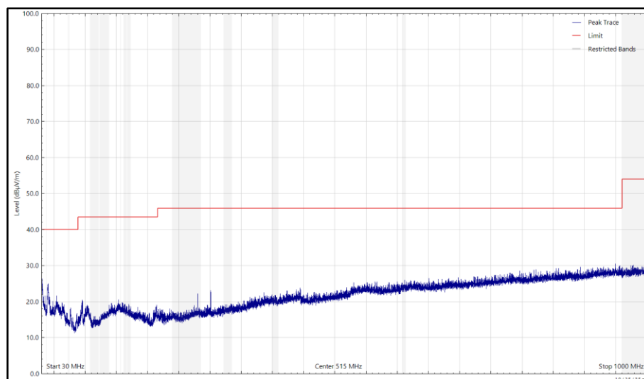
Figure 724 - U-NII-1 - 5180 MHz (CH36), HE20, RU26-0, CDD, Core 0 + Core 1, 30 MHz to 1 GHz, Vertical (Peak)
