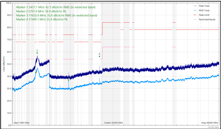
Figure 737 - U-NII-3 - 5825 MHz (CH165), HE20, RU26-0, CDD, Core 0 + Core 1, 1 GHz to 40 GHz, Vertical
