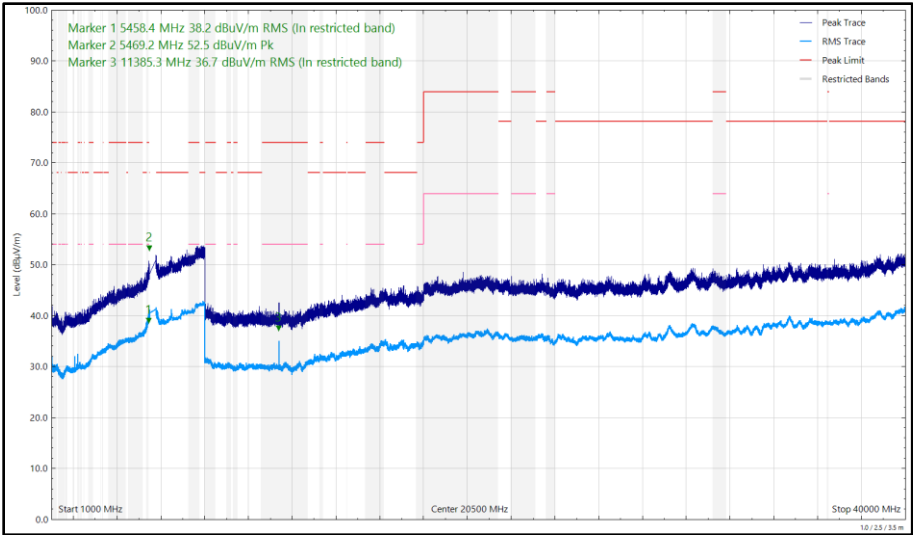
Figure 730 - U-NII-2C - 5700 MHz (CH140), HE20, RU52-37, CDD, Core 0 + Core 1, 1 GHz to 40 GHz, Horizontal
