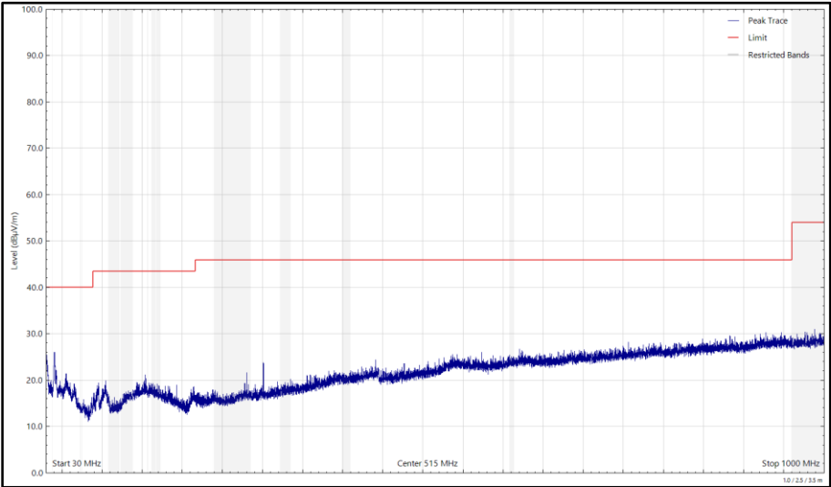
Figure 720 - U-NII-3 - 5825 MHz (CH165), HT20, CDD, Core 0 + Core 1, 30 MHz to 1 GHz, Vertical (Peak)
