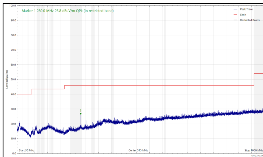
Figure 718 - U-NII-3 - 5825 MHz (CH165), HT20, CDD, Core 0 + Core 1, 30 MHz to 1 GHz, Horizontal (Peak)
