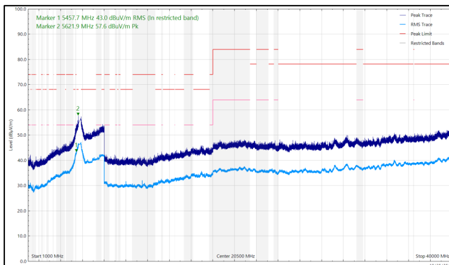
Figure 717 - U-NII-3 - 5745 MHz (CH149), HT20, CDD, Core 0 + Core 1, 1 GHz to 40 GHz, Vertical
