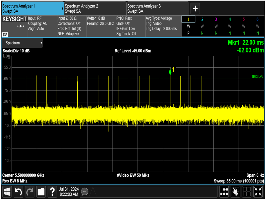
Figure 745 - Verification of Radar Type 0
