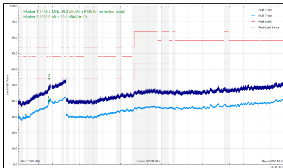
Figure 719 - U-NII-3 - 5825 MHz (CH165), HT20, CDD, Core 0 + Core 1, 1 GHz to 40 GHz, Horizontal
