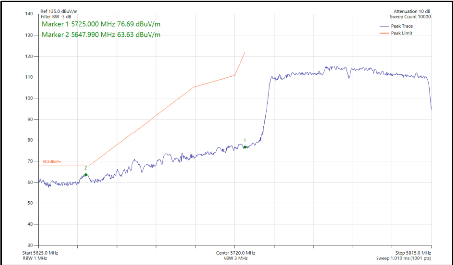
Figure 632 - 802.11ac VHT80, SDM, Core 0 - Core 1 - 5775 MHz Band Edge Frequency 5725 MHz
