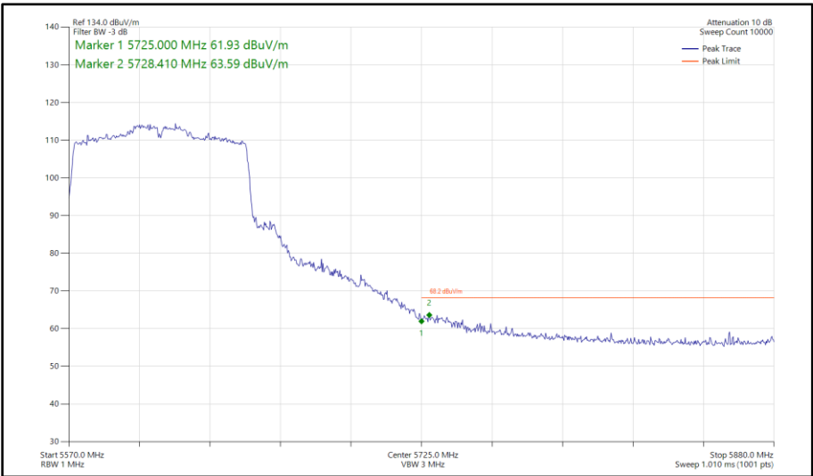
Figure 605 - 802.11ac VHT80, SISO, Core 1 - 5610 MHz Band Edge Frequency 5725 MHz
