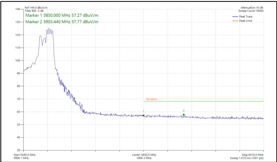
Figure 574 - 802.11ax HE40, RU 106-56, SDM, Core 0 - Core 1 - 5710 MHz Band Edge Frequency 5850 MHz
