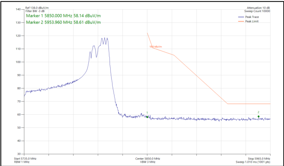
Figure 643 - 802.11ax HE80, RU 106-60, SDM, Core 0 - Core 1 - 5775 MHz Band Edge Frequency 5850 MHz
