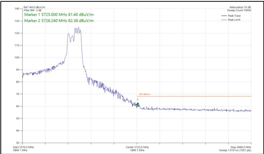
Figure 637 - 802.11ax HE80, RU 106-60, SDM, Core 0 - Core 1 - 5610 MHz Band Edge Frequency 5725 MHz
