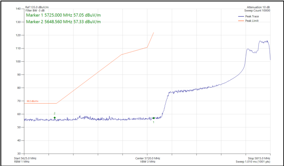
Figure 604 - 802.11ax HE80, RU 106-60, SISO, Core 1 - 5775 MHz Band Edge Frequency 5725 MHz
