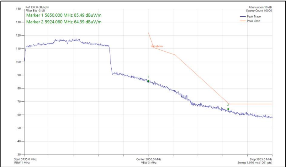
Figure 612 - 802.11ax HE80, SU, SISO, Core 1 - 5775 MHz Band Edge Frequency 5850 MHz
