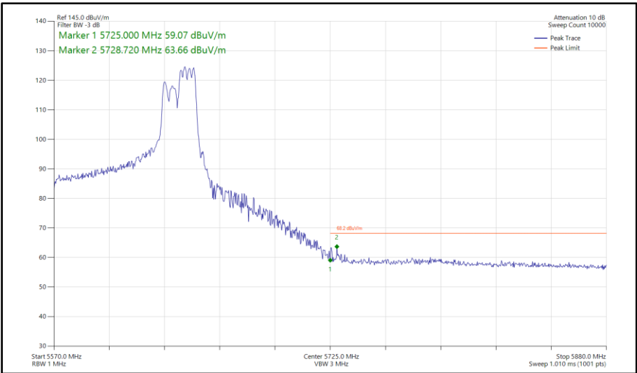
Figure 622 - 802.11ax HE80, RU 106-60, CDD, Core 0 - Core 1 - 5610 MHz Band Edge Frequency 5725 MHz
