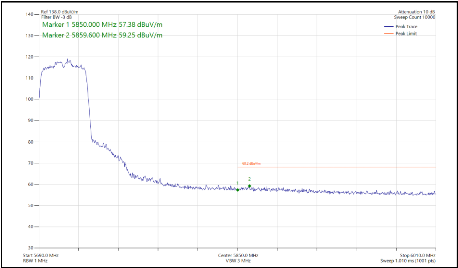
Figure 571 - 802.11n HT40, SDM, Core 0 - Core 1 - 5710 MHz Band Edge Frequency 5850 MHz
