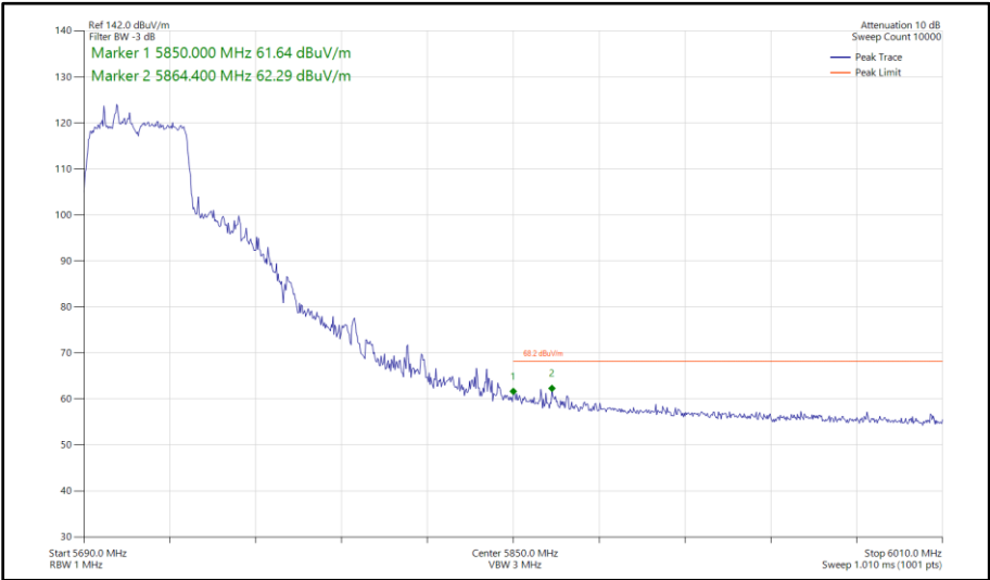
Figure 582 - 802.11ac VHT40, TxBF, Core 0 - Core 1 - 5710 MHz Band Edge Frequency 5850 MHz
