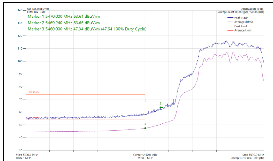
Figure 577 - 802.11ac VHT40, TxBF, Core 0 - Core 1 - 5510 MHz Band Edge Frequency 5470 MHz
