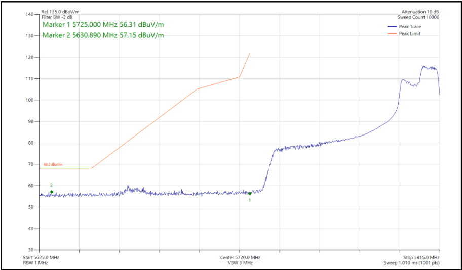
Figure 589 - 802.11ax HE80, RU 106-60, SISO, Core 0 - 5775 MHz Band Edge Frequency 5725 MHz
