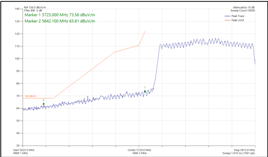
Figure 618 - 802.11ax HE80, SU, CDD, Core 0 - Core 1 - 5775 MHz Band Edge Frequency 5725 MHz
