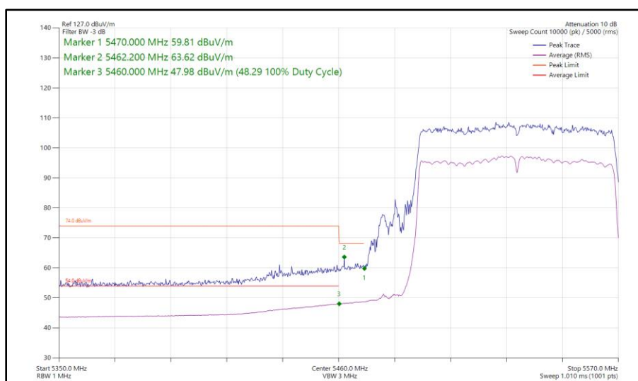
Figure 644 - 802.11ac VHT80, TxBF, Core 0 - Core 1 - 5530 MHz Band Edge Frequency 5470 MHz
