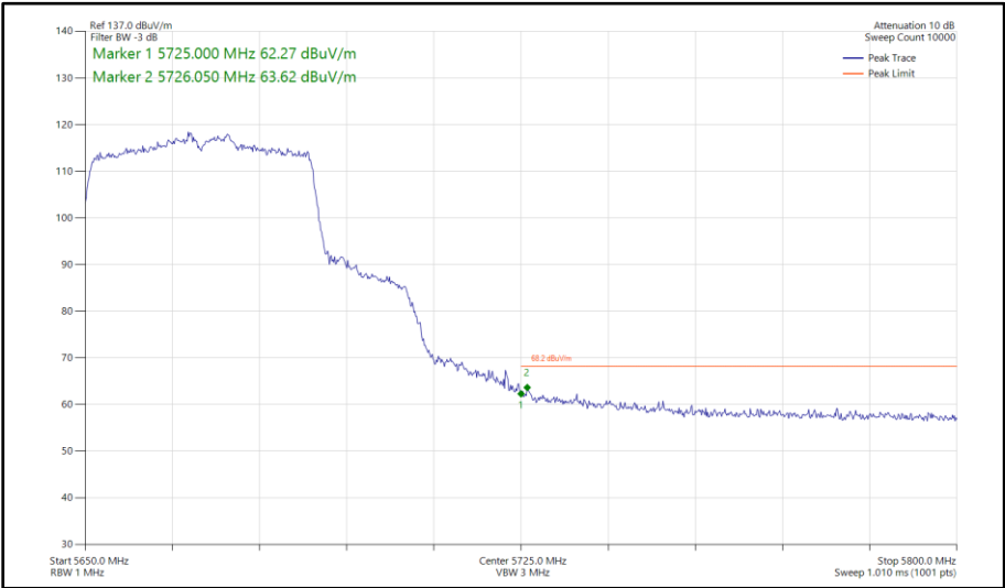
Figure 569 - 802.11ax HE40, SU, SDM, Core 0 - Core 1 - 5670 MHz Band Edge Frequency 5725 MHz
