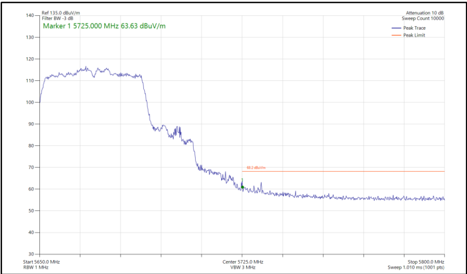
Figure 581 - 802.11ac VHT40, TxBF, Core 0 - Core 1 - 5670 MHz Band Edge Frequency 5725 MHz
