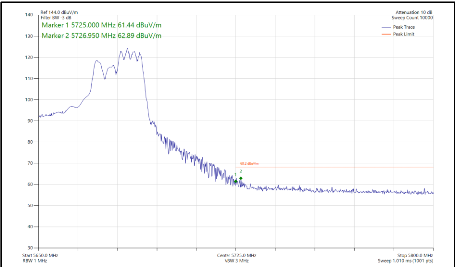
Figure 570 - 802.11ax HE40, RU 106-56, SDM, Core 0 - Core 1 - 5670 MHz Band Edge Frequency 5725 MHz
