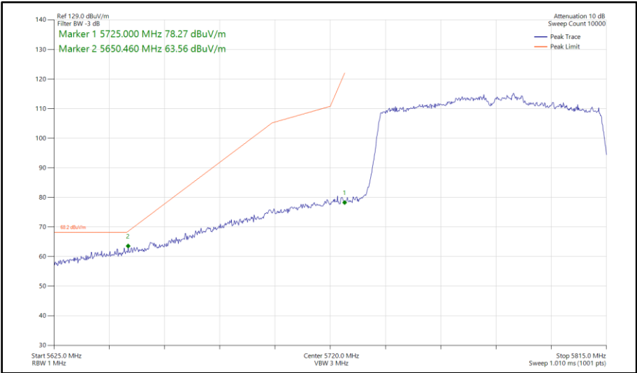
Figure 602 - 802.11ac VHT80, SISO, Core 1 - 5775 MHz Band Edge Frequency 5725 MHz
