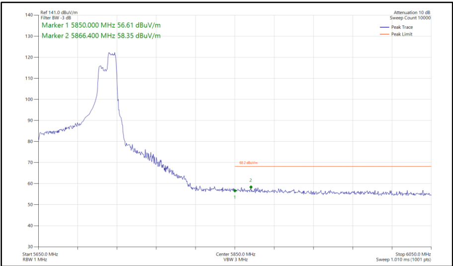
Figure 611 - 802.11ax HE80, RU 106-60, SISO, Core 1 - 5690 MHz Band Edge Frequency 5850 MHz
