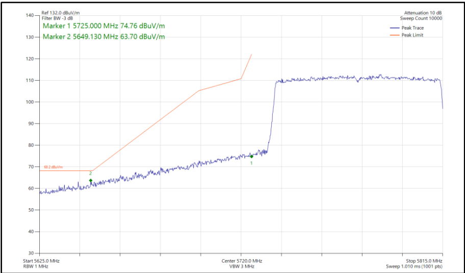
Figure 588 - 802.11ax HE80, SU, SISO, Core 0 - 5775 MHz Band Edge Frequency 5725 MHz
