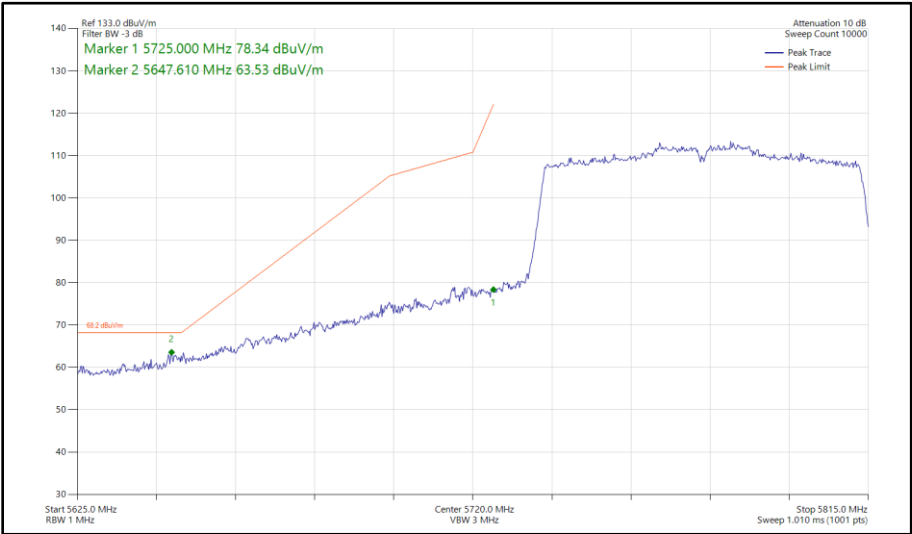
Figure 587 - 802.11ac VHT80, SISO, Core 0 - 5775 MHz Band Edge Frequency 5725 MHz
