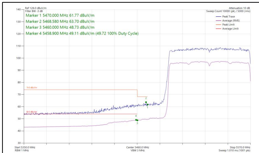
Figure 600 - 802.11ax HE80, SU, SISO, Core 1 - 5530 MHz Band Edge Frequency 5470 MHz
