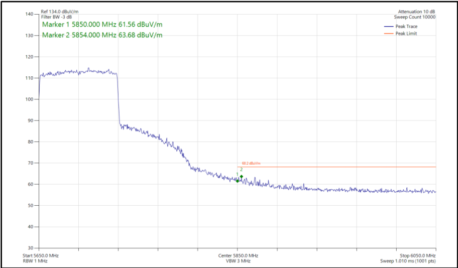
Figure 610 - 802.11ax HE80, SU, SISO, Core 1 - 5690 MHz Band Edge Frequency 5850 MHz
