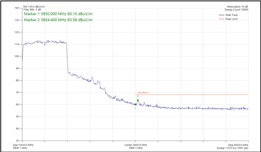
Figure 593 - 802.11ac VHT80, SISO, Core 0 - 5690 MHz Band Edge Frequency 5850 MHz
