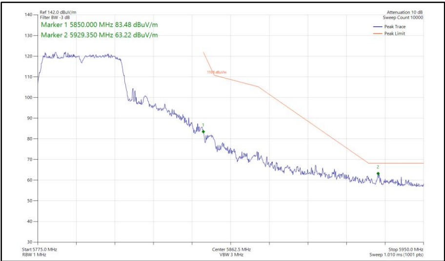
Figure 583 - 802.11ac VHT40, TxBF, Core 0 - Core 1 - 5795 MHz Band Edge Frequency 5850 MHz
