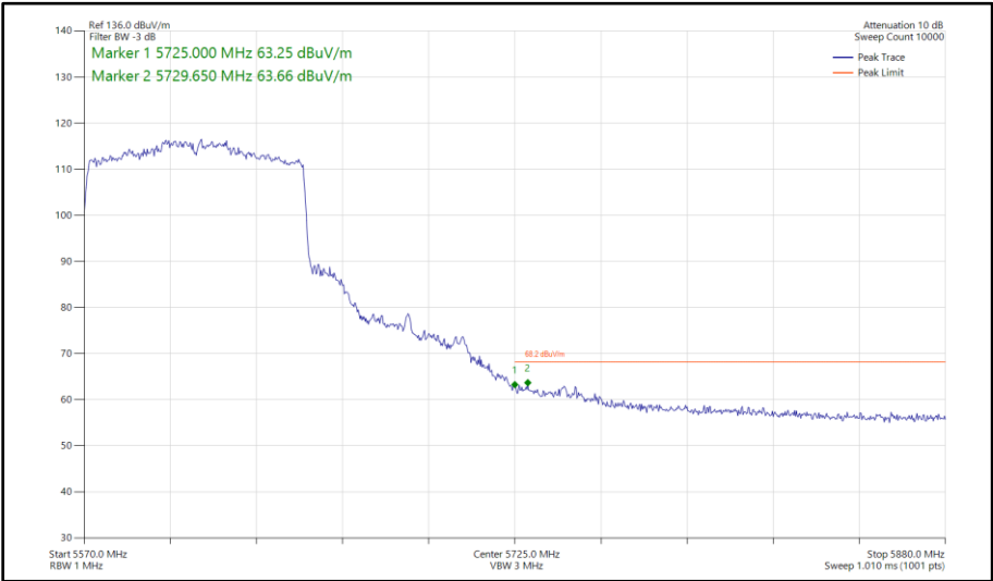
Figure 636 - 802.11ax HE80, SU, SDM, Core 0 - Core 1 - 5610 MHz Band Edge Frequency 5725 MHz
