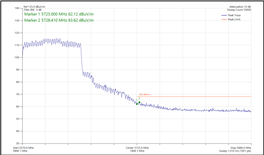
Figure 621 - 802.11ax HE80, SU, CDD, Core 0 - Core 1 - 5610 MHz Band Edge Frequency 5725 MHz
