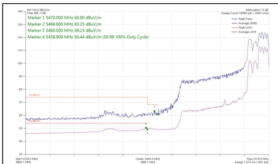
Figure 616 - 802.11ax HE80, RU 106-60, CDD, Core 0 - Core 1 - 5530 MHz Band Edge Frequency 5470 MHz
