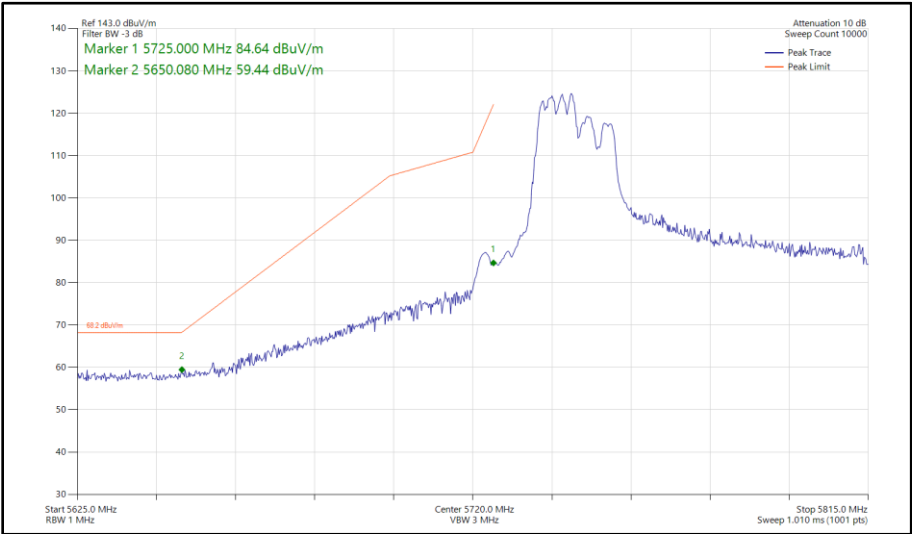
Figure 634 - 802.11ax HE80, RU 106-53, SDM, Core 0 - Core 1 - 5775 MHz Band Edge Frequency 5725 MHz
