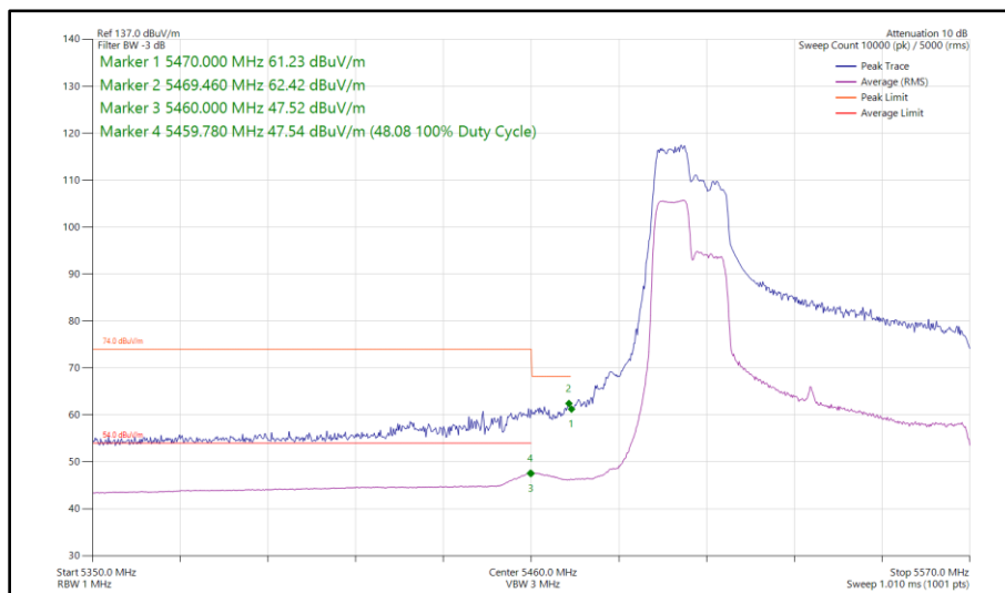
Figure 586 - 802.11ax HE80, RU 106-53, SISO, Core 0 - 5530 MHz Band Edge Frequency 5470 MHz
