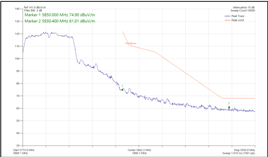
Figure 572 - 802.11n HT40, SDM, Core 0 - Core 1 - 5795 MHz Band Edge Frequency 5850 MHz
