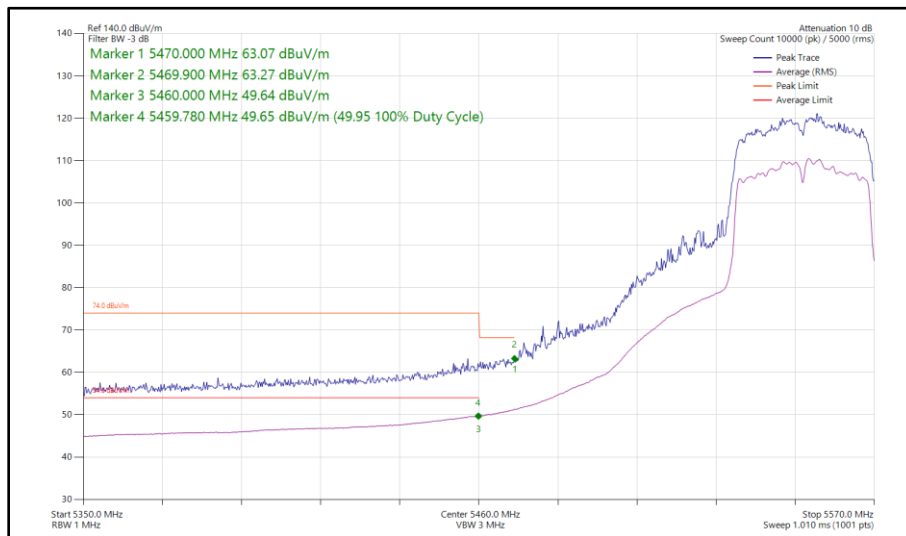
Figure 578 - 802.11ac VHT40, TxBF, Core 0 - Core 1 - 5550 MHz Band Edge Frequency 5470 MHz
