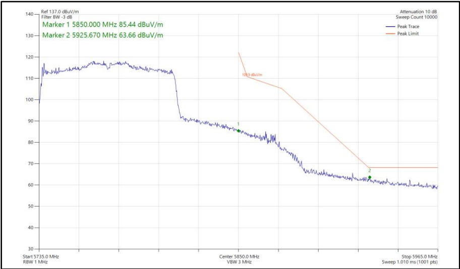
Figure 648 - 802.11ac VHT80, TxBF, Core 0 - Core 1 - 5775 MHz Band Edge Frequency 5850 MHz
