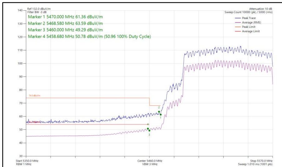
Figure 615 - 802.11ax HE80, SU, CDD, Core 0 - Core 1 - 5530 MHz Band Edge Frequency 5470 MHz
