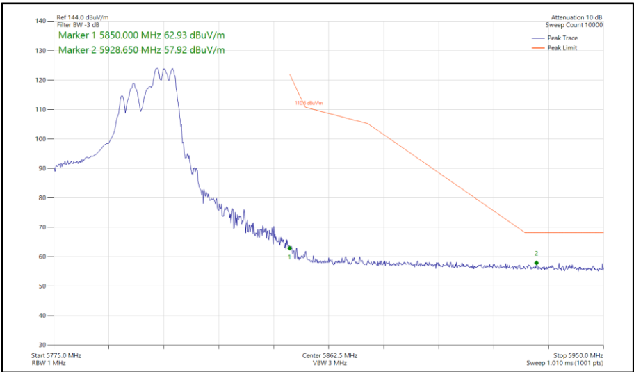
Figure 576 - 802.11ax HE40, RU 106-56, SDM, Core 0 - Core 1 - 5795 MHz Band Edge Frequency 5850 MHz
