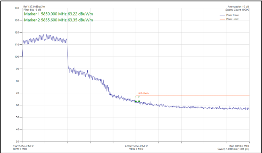
Figure 625 - 802.11ax HE80, SU, CDD, Core 0 - Core 1 - 5690 MHz Band Edge Frequency 5850 MHz
