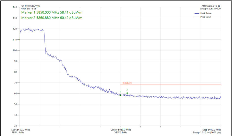
Figure 573 - 802.11ax HE40, SU, SDM, Core 0 - Core 1 - 5710 MHz Band Edge Frequency 5850 MHz
