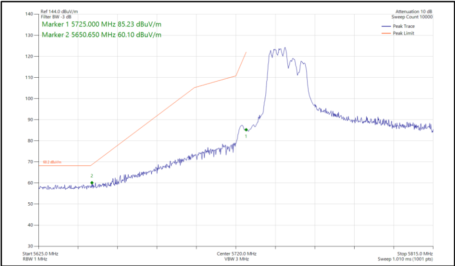
Figure 619 - 802.11ax HE80, RU 106-53, CDD, Core 0 - Core 1 - 5775 MHz Band Edge Frequency 5725 MHz
