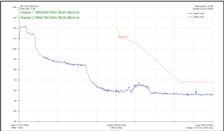
Figure 613 - 802.11ax HE80, RU 106-53, SISO, Core 1 - 5775 MHz Band Edge Frequency 5850 MHz
