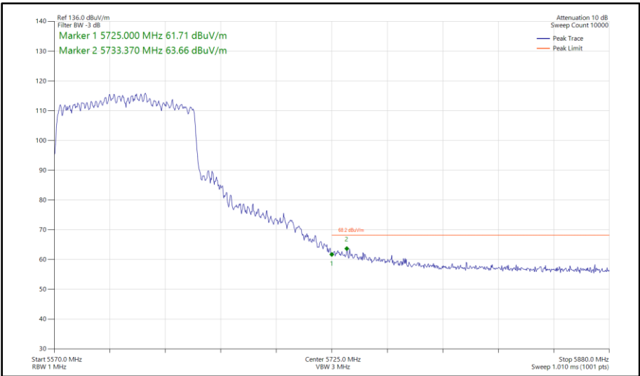
Figure 620 - 802.11ac VHT80, CDD, Core 0 - Core 1 - 5610 MHz Band Edge Frequency 5725 MHz
