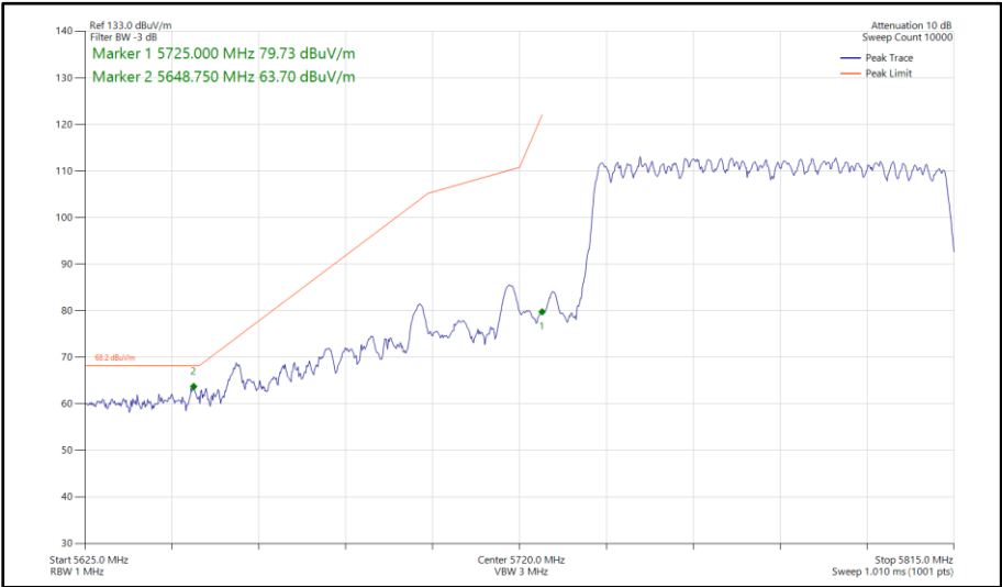
Figure 617 - 802.11ac VHT80, CDD, Core 0 - Core 1 - 5775 MHz Band Edge Frequency 5725 MHz
