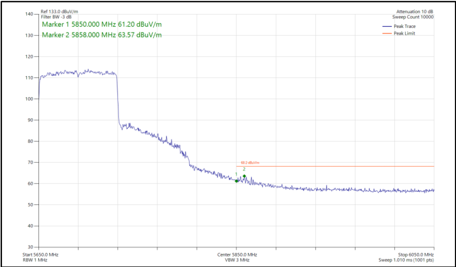
Figure 595 - 802.11ax HE80, SU, SISO, Core 0 - 5690 MHz Band Edge Frequency 5850 MHz
