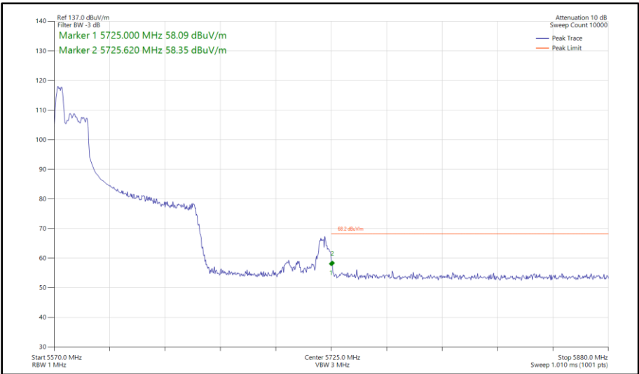
Figure 592 - 802.11ax HE80, RU 52-37, SISO, Core 0 - 5610 MHz Band Edge Frequency 5725 MHz
