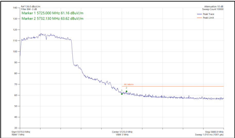
Figure 635 - 802.11ac VHT80, SDM, Core 0 - Core 1 - 5610 MHz Band Edge Frequency 5725 MHz
