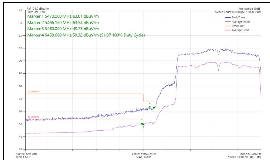
Figure 584 - 802.11ac VHT80, SISO, Core 0 - 5530 MHz Band Edge Frequency 5470 MHz
