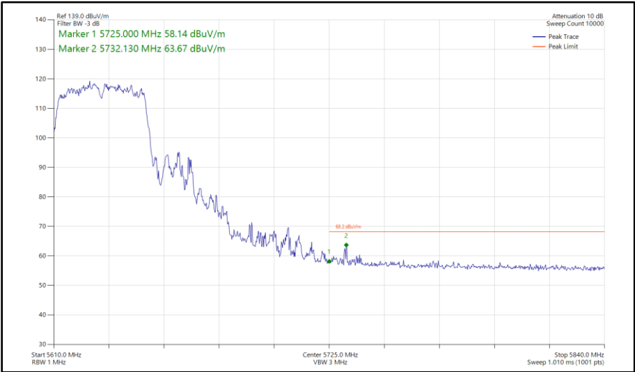
Figure 580 - 802.11ac VHT40, TxBF, Core 0 - Core 1 - 5630 MHz Band Edge Frequency 5725 MHz
