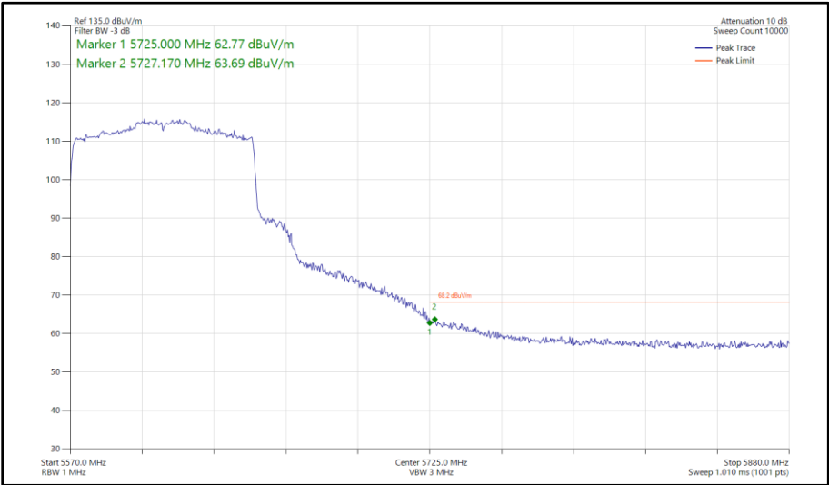
Figure 606 - 802.11ax HE80, SU, SISO, Core 1 - 5610 MHz Band Edge Frequency 5725 MHz
