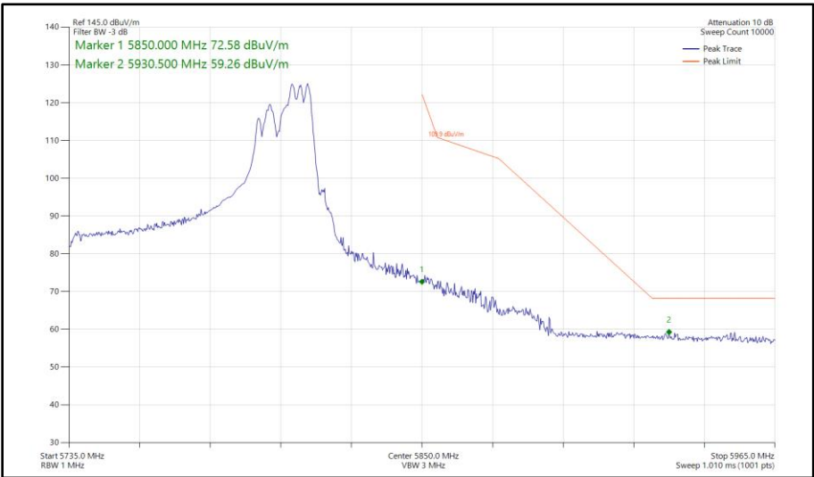
Figure 628 - 802.11ax HE80, RU 106-60, CDD, Core 0 - Core 1 - 5775 MHz Band Edge Frequency 5850 MHz
