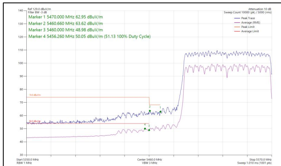
Figure 614 - 802.11ac VHT80, CDD, Core 0 - Core 1 - 5530 MHz Band Edge Frequency 5470 MHz
