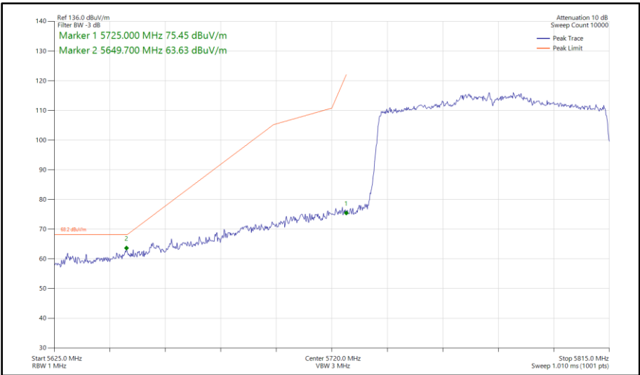
Figure 633 - 802.11ax HE80, SU, SDM, Core 0 - Core 1 - 5775 MHz Band Edge Frequency 5725 MHz
