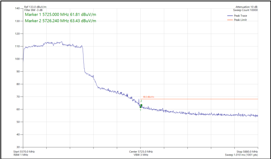
Figure 591 - 802.11ax HE80, SU, SISO, Core 0 - 5610 MHz Band Edge Frequency 5725 MHz
