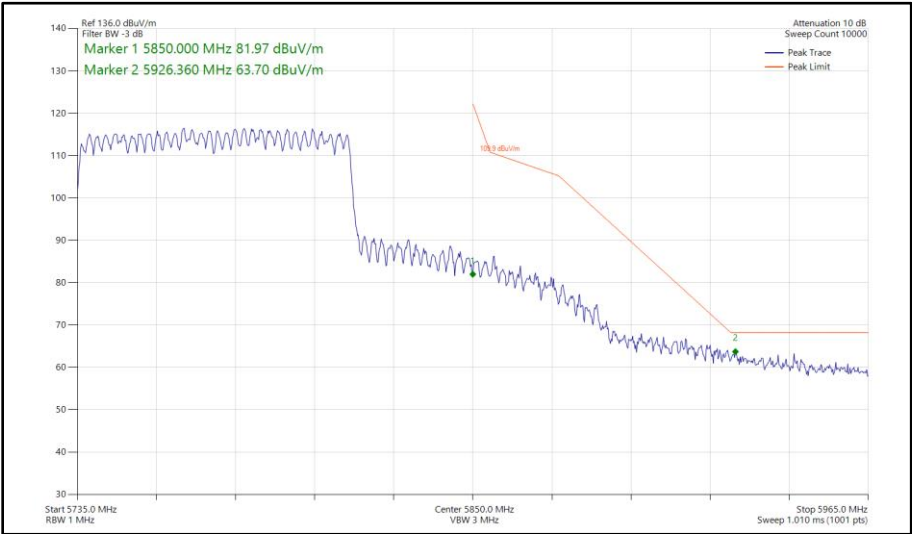
Figure 627 - 802.11ax HE80, SU, CDD, Core 0 - Core 1 - 5775 MHz Band Edge Frequency 5850 MHz
