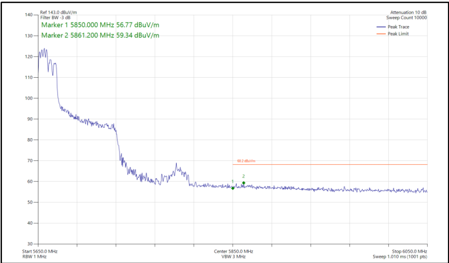
Figure 626 - 802.11ax HE80, RU 106-53, CDD, Core 0 - Core 1 - 5690 MHz Band Edge Frequency 5850 MHz
