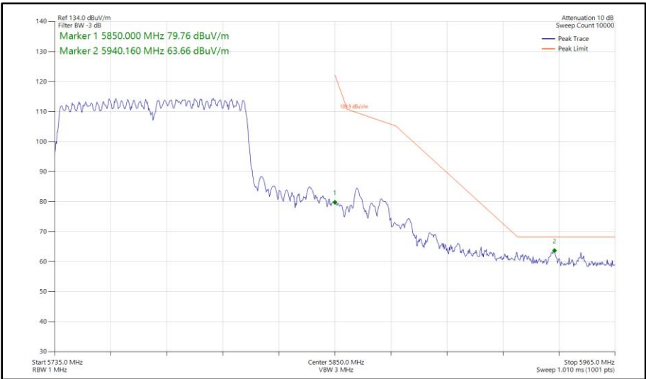
Figure 624 - 802.11ac VHT80, CDD, Core 0 - Core 1 - 5775 MHz Band Edge Frequency 5850 MHz
