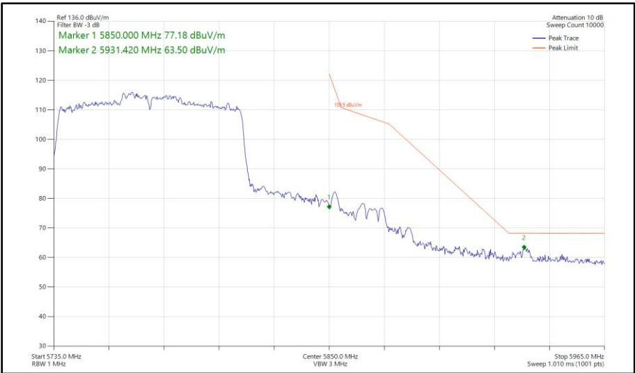
Figure 639 - 802.11ac VHT80, SDM, Core 0 - Core 1 - 5775 MHz Band Edge Frequency 5850 MHz
