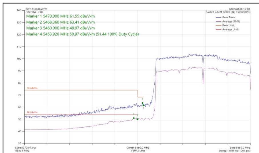
Figure 650 - 802.11ax HE160, SU, SISO, Core 0 - 5570 MHz Band Edge Frequency 5470 MHz
