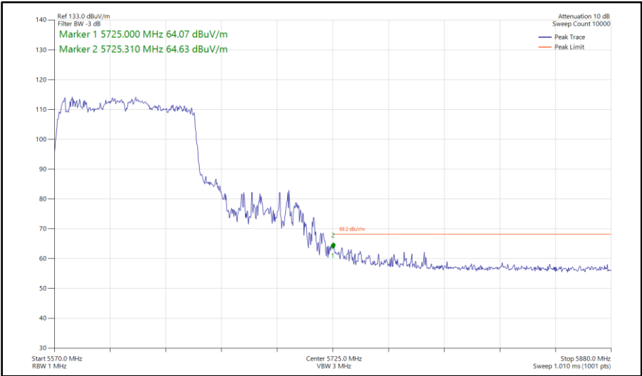
Figure 646 - 802.11ac VHT80, TxBF, Core 0 - Core 1 - 5610 MHz Band Edge Frequency 5725 MHz
