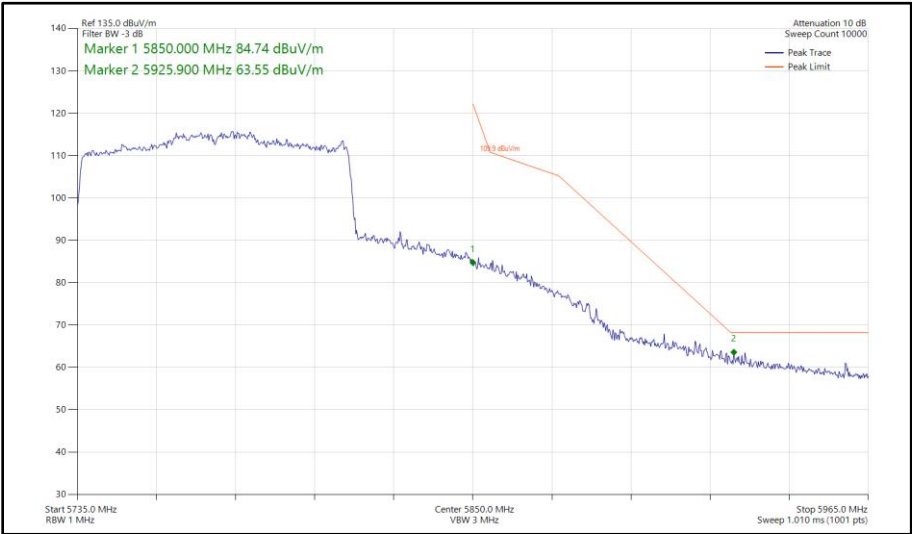
Figure 597 - 802.11ax HE80, SU, SISO, Core 0 - 5775 MHz Band Edge Frequency 5850 MHz
