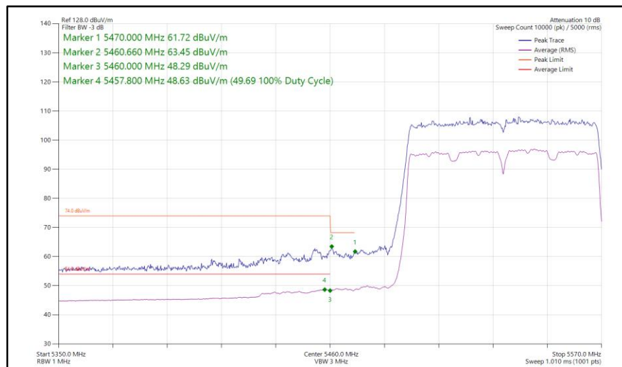
Figure 599 - 802.11ac VHT80, SISO, Core 1 - 5530 MHz Band Edge Frequency 5470 MHz
