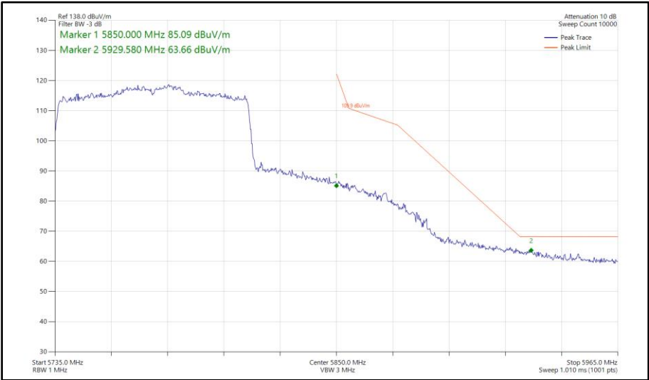
Figure 642 - 802.11ax HE80, SU, SDM, Core 0 - Core 1 - 5775 MHz Band Edge Frequency 5850 MHz
