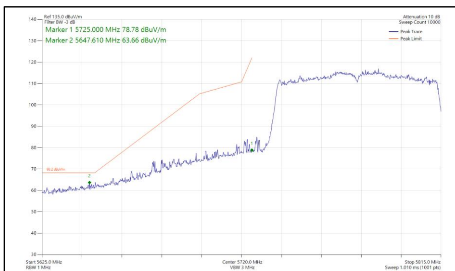
Figure 645 - 802.11ac VHT80, TxBF, Core 0 - Core 1 - 5775 MHz Band Edge Frequency 5725 MHz
