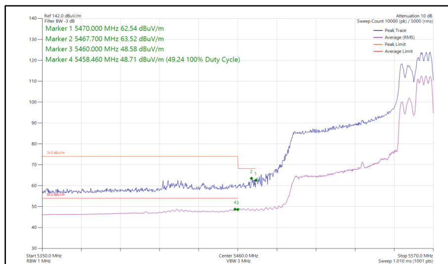
Figure 631 - 802.11ax HE80, RU 106-60, SDM, Core 0 - Core 1 - 5530 MHz Band Edge Frequency 5470 MHz
