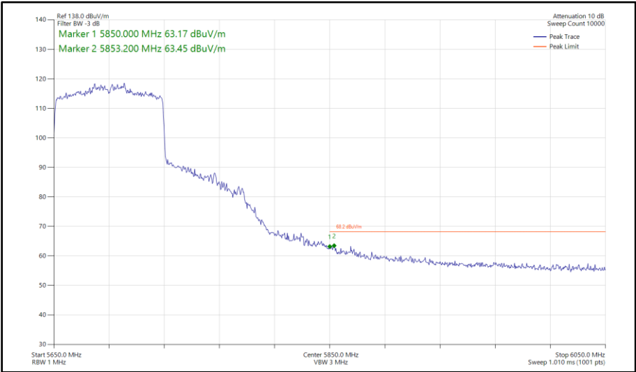
Figure 640 - 802.11ax HE80, SU, SDM, Core 0 - Core 1 - 5690 MHz Band Edge Frequency 5850 MHz
