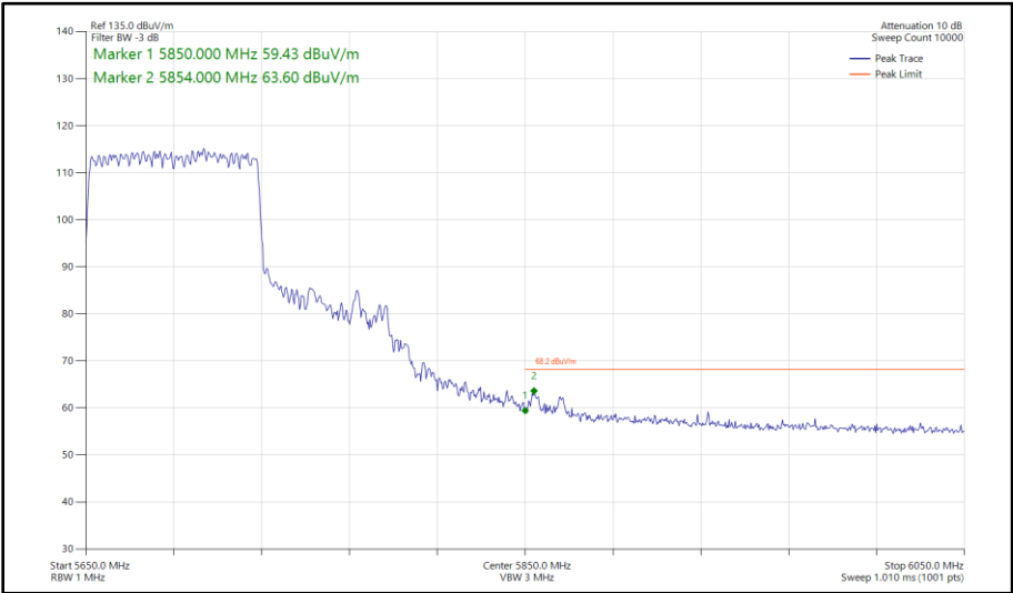
Figure 623 - 802.11ac VHT80, CDD, Core 0 - Core 1 - 5690 MHz Band Edge Frequency 5850 MHz
