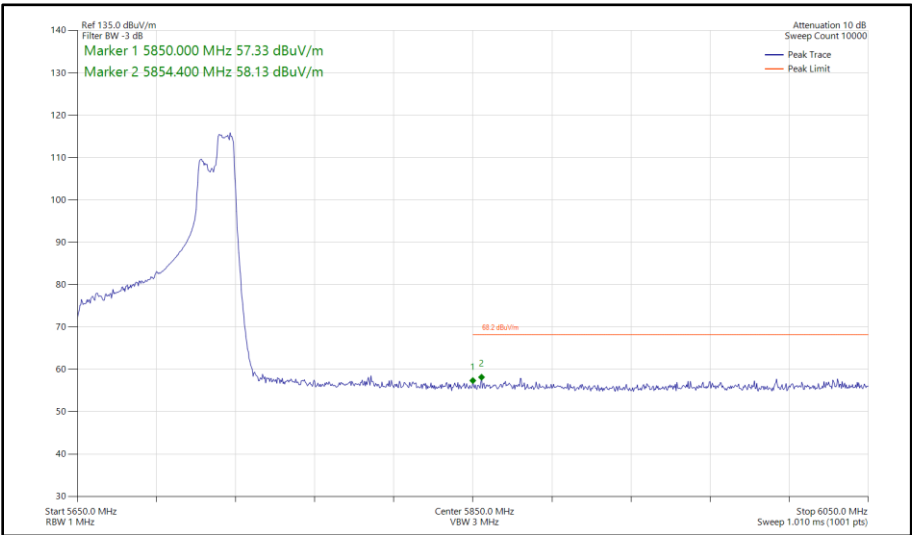
Figure 596 - 802.11ax HE80, RU 106-60, SISO, Core 0 - 5690 MHz Band Edge Frequency 5850 MHz
