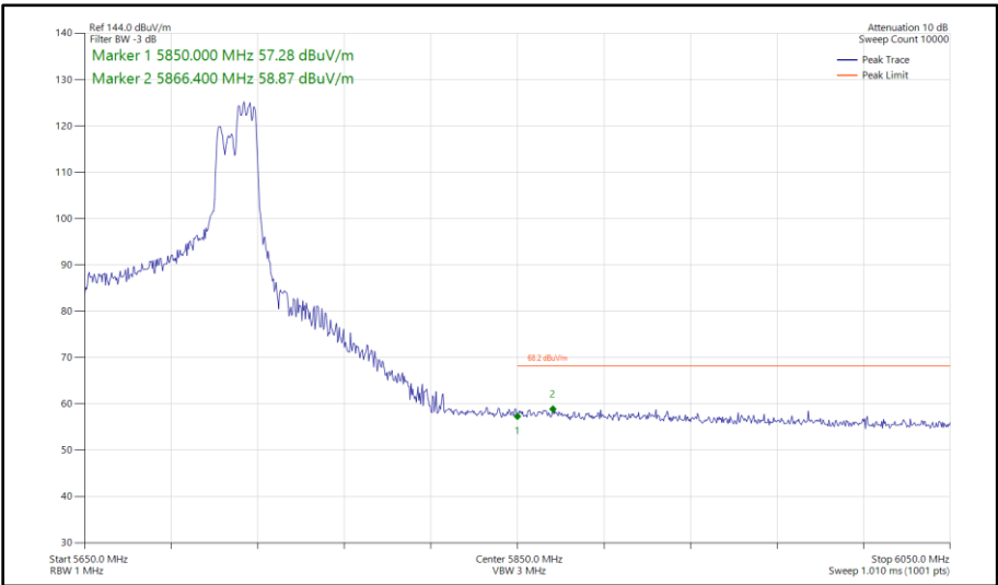
Figure 641 - 802.11ax HE80, RU 106-60, SDM, Core 0 - Core 1 - 5690 MHz Band Edge Frequency 5850 MHz
