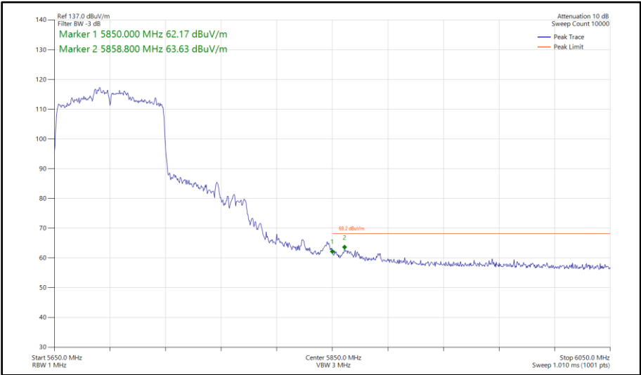
Figure 638 - 802.11ac VHT80, SDM, Core 0 - Core 1 - 5690 MHz Band Edge Frequency 5850 MHz
