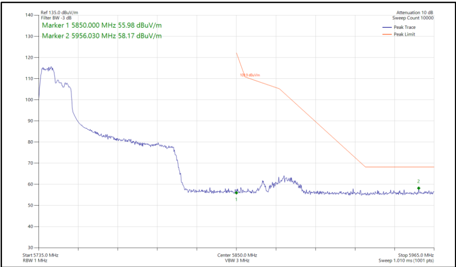
Figure 598 - 802.11ax HE80, RU 106-53, SISO, Core 0 - 5775 MHz Band Edge Frequency 5850 MHz
