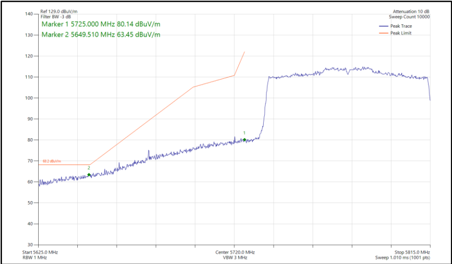
Figure 603 - 802.11ax HE80, SU, SISO, Core 1 - 5775 MHz Band Edge Frequency 5725 MHz
