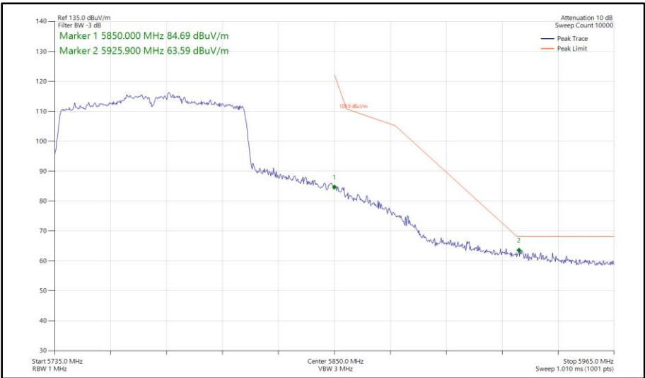
Figure 594 - 802.11ac VHT80, SISO, Core 0 - 5775 MHz Band Edge Frequency 5850 MHz
