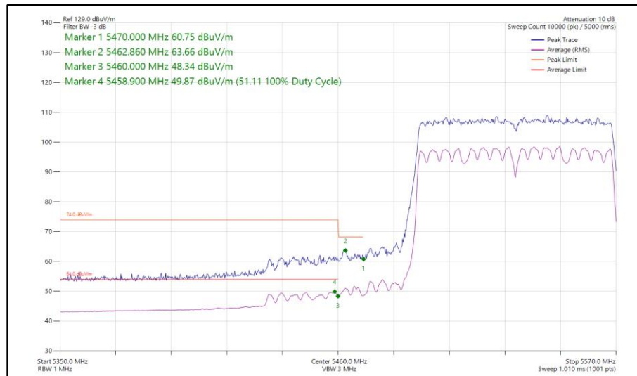
Figure 629 - 802.11ac VHT80, SDM, Core 0 - Core 1 - 5530 MHz Band Edge Frequency 5470 MHz
