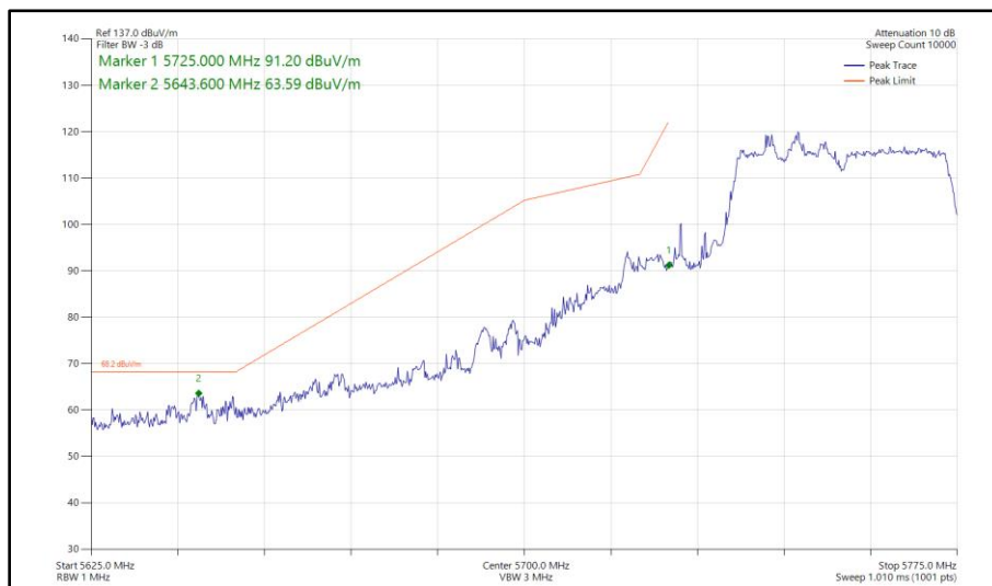
Figure 579 - 802.11ac VHT40, TxBF, Core 0 - Core 1 - 5755 MHz Band Edge Frequency 5725 MHz
