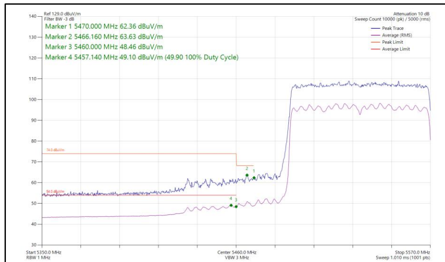
Figure 630 - 802.11ax HE80, SU, SDM, Core 0 - Core 1 - 5530 MHz Band Edge Frequency 5470 MHz
