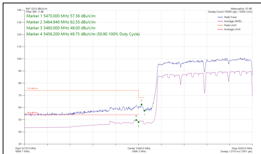
Figure 649 - 802.11ac VHT160, SISO, Core 0 - 5570 MHz Band Edge Frequency 5470 MHz
