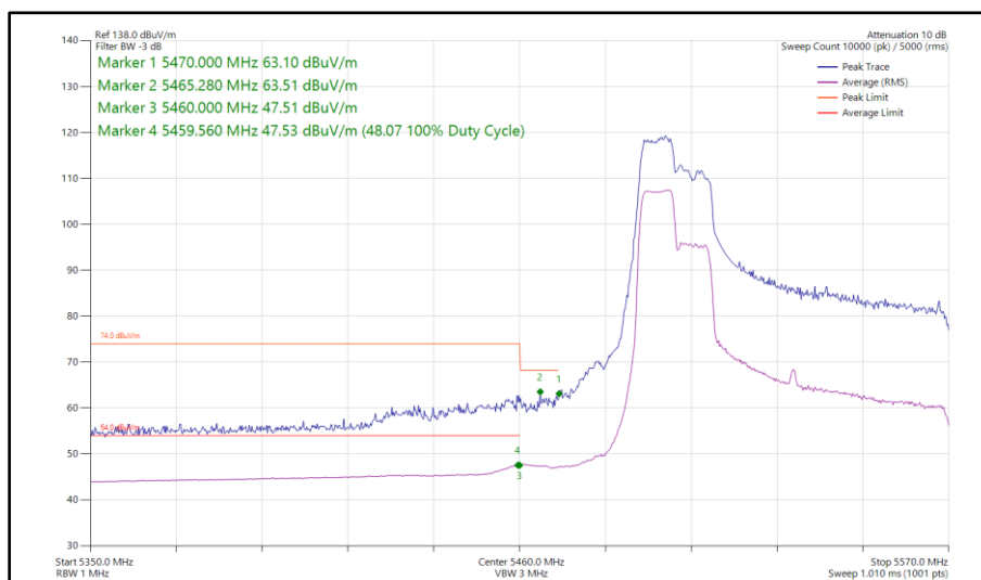
Figure 601 - 802.11ax HE80, RU 106-53, SISO, Core 1 - 5530 MHz Band Edge Frequency 5470 MHz
