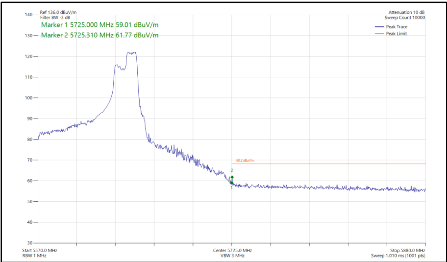
Figure 607 - 802.11ax HE80, RU 106-60, SISO, Core 1 - 5610 MHz Band Edge Frequency 5725 MHz
