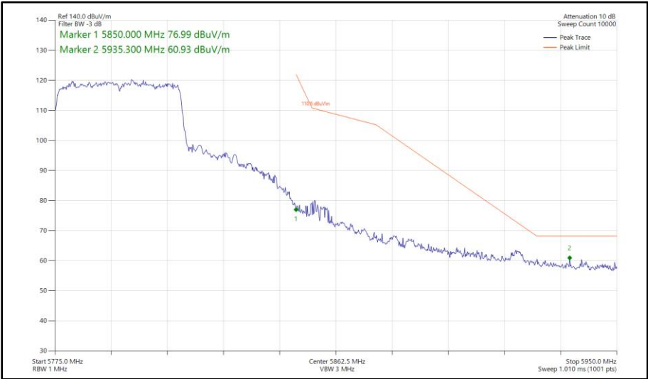
Figure 575 - 802.11ax HE40, SU, SDM, Core 0 - Core 1 - 5795 MHz Band Edge Frequency 5850 MHz
