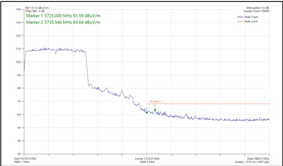
Figure 590 - 802.11ac VHT80, SISO, Core 0 - 5610 MHz Band Edge Frequency 5725 MHz
