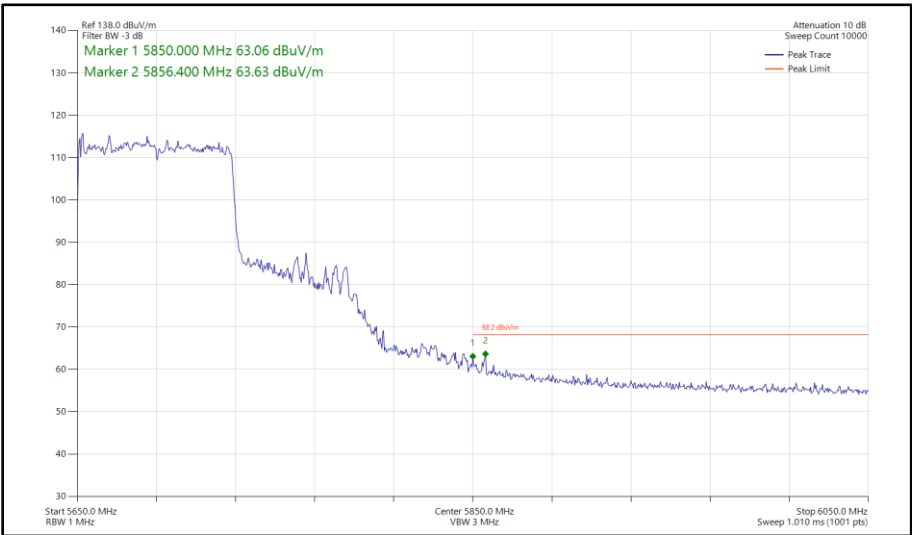
Figure 647 - 802.11ac VHT80, TxBF, Core 0 - Core 1 - 5690 MHz Band Edge Frequency 5850 MHz
