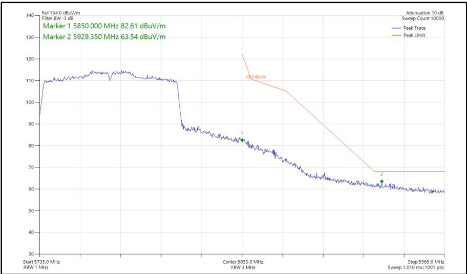
Figure 609 - 802.11ac VHT80, SISO, Core 1 - 5775 MHz Band Edge Frequency 5850 MHz
