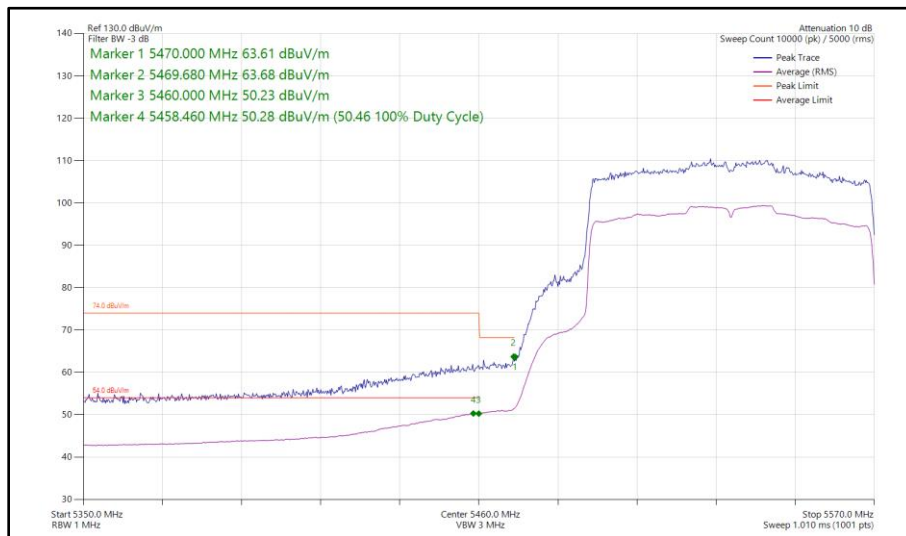
Figure 585 - 802.11ax HE80, SU, SISO, Core 0 - 5530 MHz Band Edge Frequency 5470 MHz
