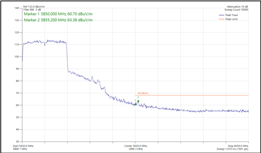
Figure 608 - 802.11ac VHT80, SISO, Core 1 - 5690 MHz Band Edge Frequency 5850 MHz
