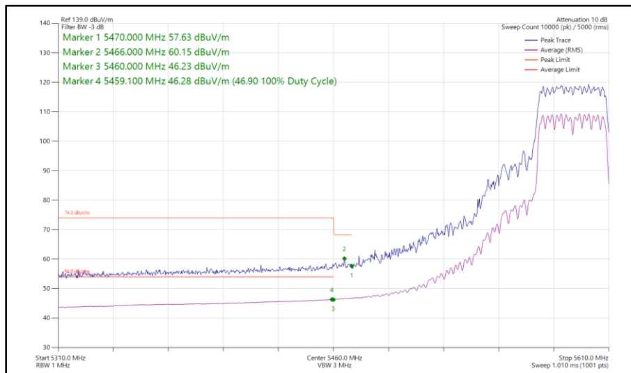
Figure 534 - 802.11n HT40, CDD, Core 0 - Core 1 - 5590 MHz Band Edge Frequency 5470 MHz
