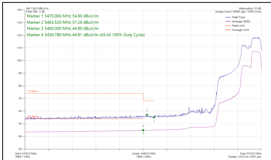
Figure 495 - 802.11ax HE40, RU 106-56, SISO, Core 0 - 5550 MHz Band Edge Frequency 5470 MHz
