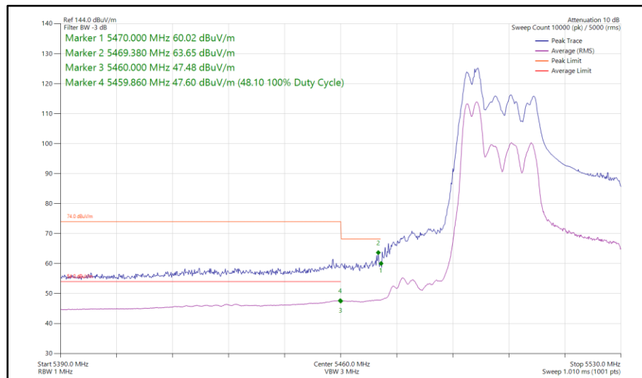
Figure 536 - 802.11ax HE40, RU 52-37, CDD, Core 0 - Core 1 - 5510 MHz Band Edge Frequency 5470 MHz
