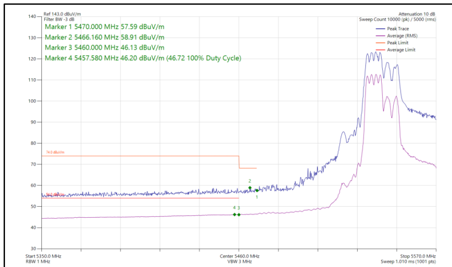
Figure 538 - 802.11ax HE40, RU 106-53, CDD, Core 0 - Core 1 - 5550 MHz Band Edge Frequency 5470 MHz
