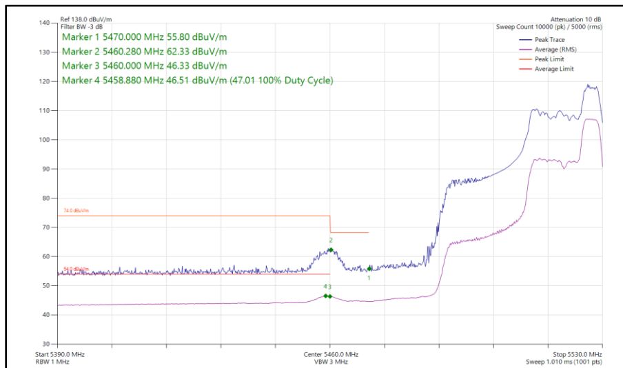
Figure 493 - 802.11ax HE40, RU 52-44, SISO, Core 0 - 5510 MHz Band Edge Frequency 5470 MHz
