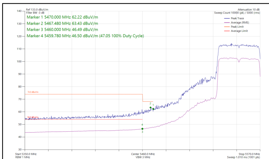
Figure 494 - 802.11ax HE40, SU, SISO, Core 0 - 5550 MHz Band Edge Frequency 5470 MHz
