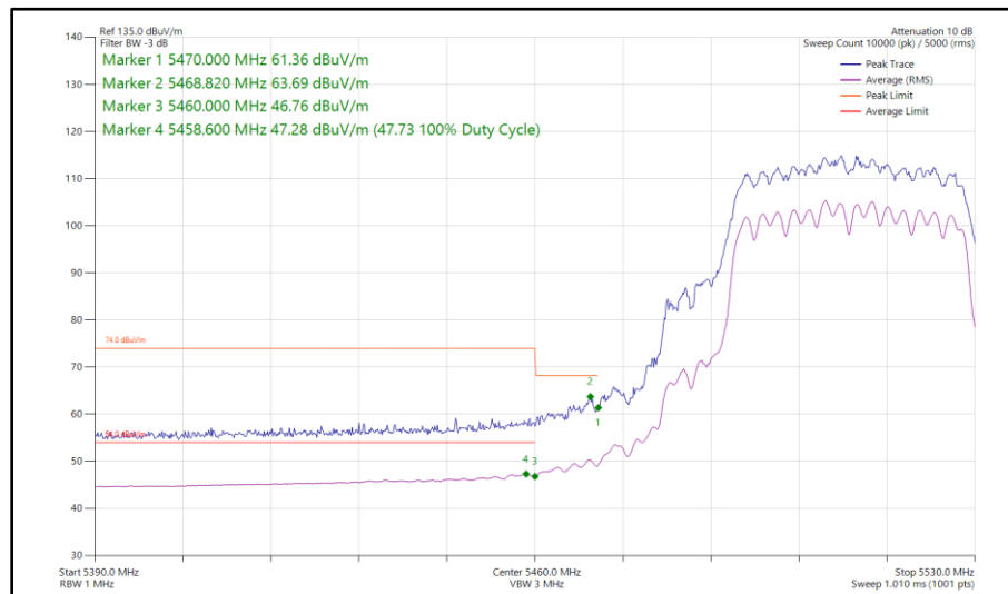
Figure 532 - 802.11n HT40, CDD, Core 0 - Core 1 - 5510 MHz Band Edge Frequency 5470 MHz
