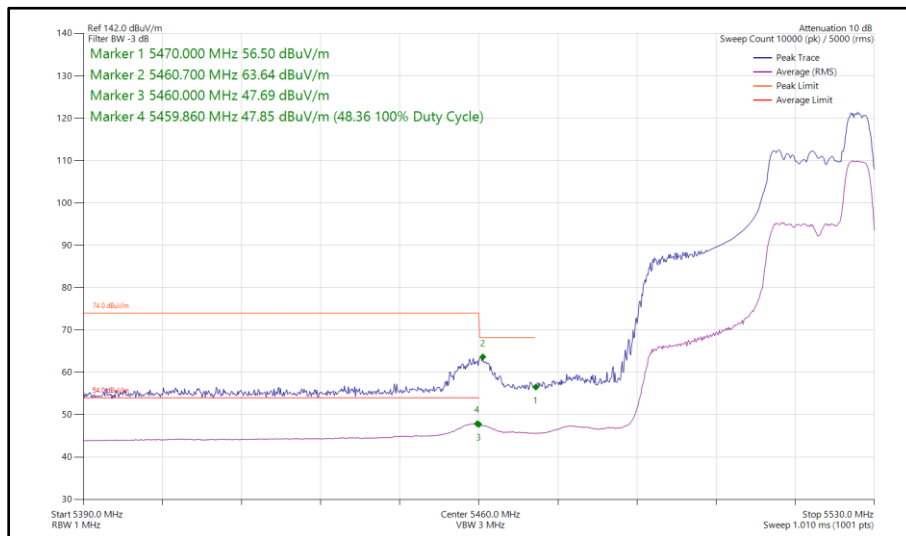
Figure 514 - 802.11ax HE40, RU 52-44, SISO, Core 1 - 5510 MHz Band Edge Frequency 5470 MHz
