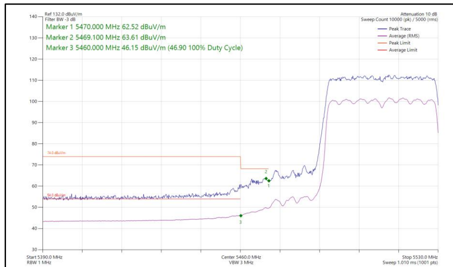
Figure 557 - 802.11ax HE40, SU, SDM, Core 0 - Core 1 - 5510 MHz Band Edge Frequency 5470 MHz
