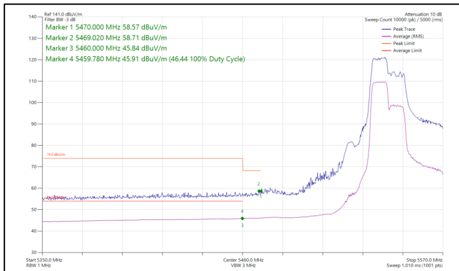
Figure 516 - 802.11ax HE40, RU 106-53, SISO, Core 1 - 5550 MHz Band Edge Frequency 5470 MHz
