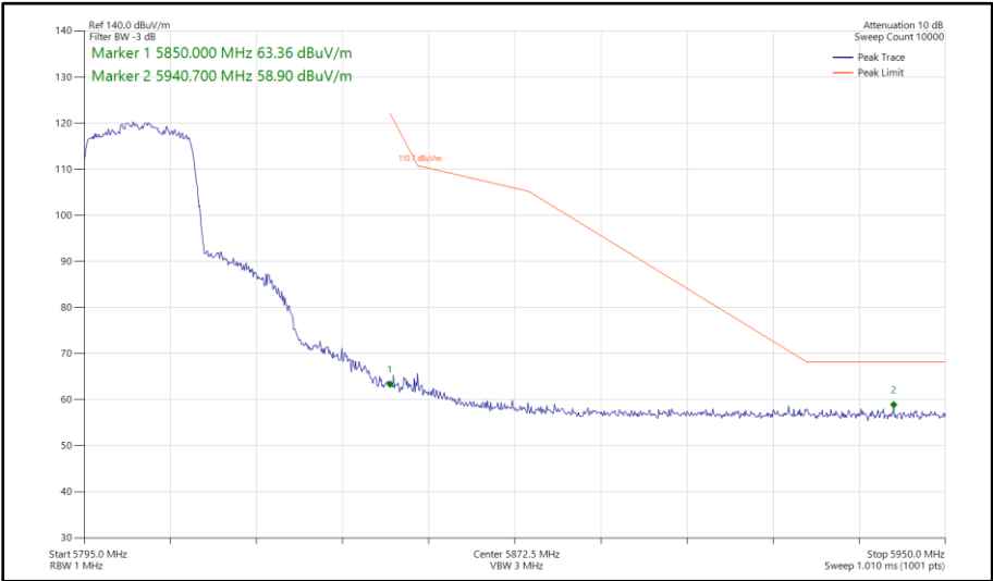
Figure 423 - 802.11ax HE20, SU, SISO, Core 1 - 5805 MHz Band Edge Frequency 5850 MHz
