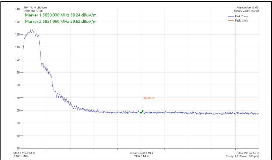
Figure 447 - 802.11n HT20, CDD, Core 0 - Core 1 - 5720 MHz Band Edge Frequency 5850 MHz
