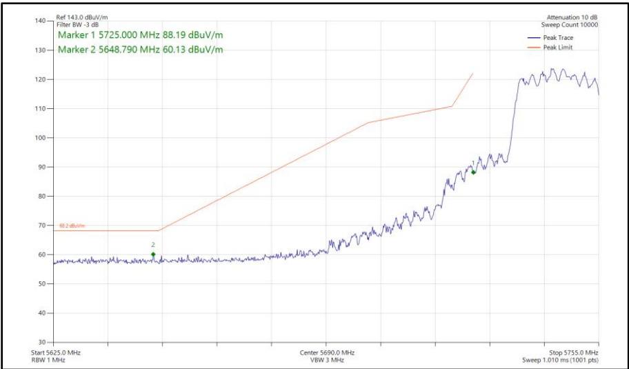
Figure 435 - 802.11ax HE20, SU, CDD, Core 0 - Core 1 - 5745 MHz Band Edge Frequency 5725 MHz
