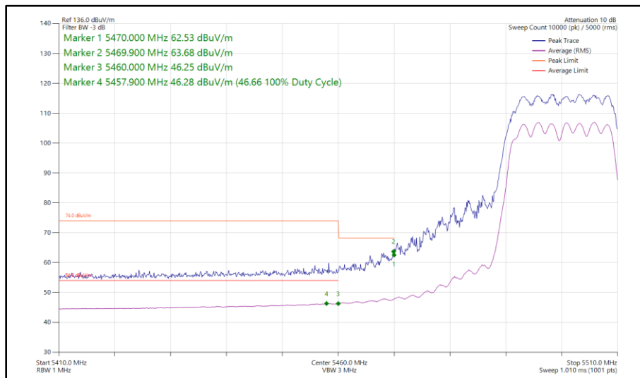
Figure 426 - 802.11n HT20, CDD, Core 0 - Core 1 - 5500 MHz Band Edge Frequency 5470 MHz
