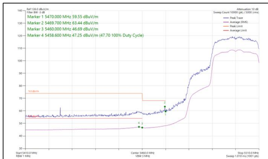
Figure 481 - 802.11ac VHT20, TxBF, Core 0 - Core 1 - 5500 MHz Band Edge Frequency 5470 MHz
