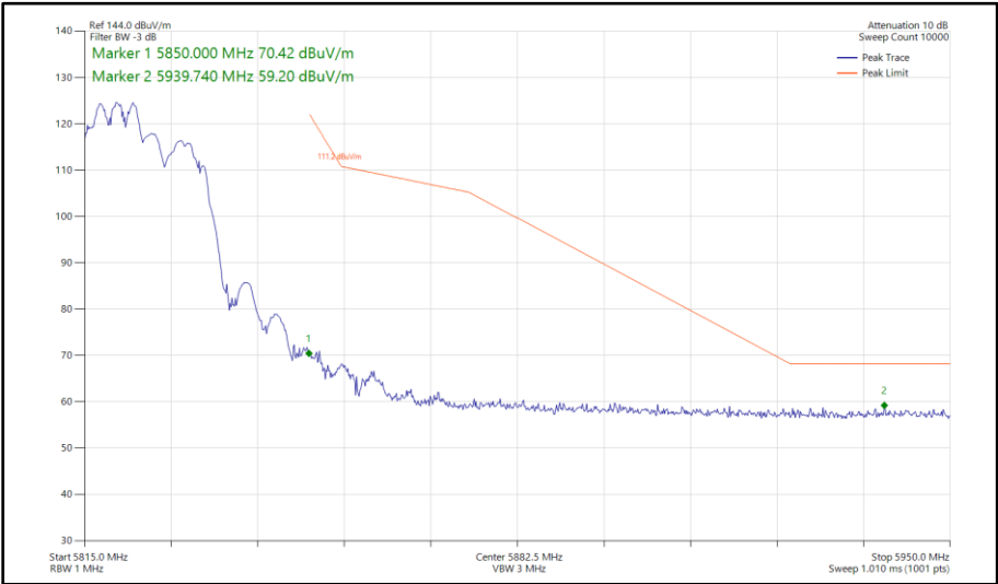
Figure 480 - 802.11ax HE20, RU 106-53, SDM, Core 0 - Core 1 - 5825 MHz Band Edge Frequency 5850 MHz
