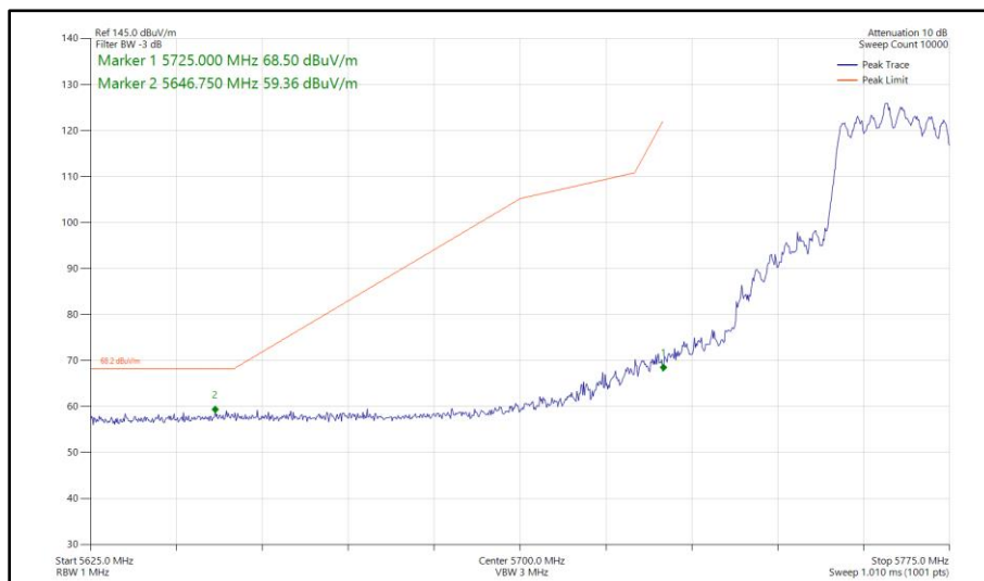
Figure 437 - 802.11ax HE20, SU, CDD, Core 0 - Core 1 - 5765 MHz Band Edge Frequency 5725 MHz
