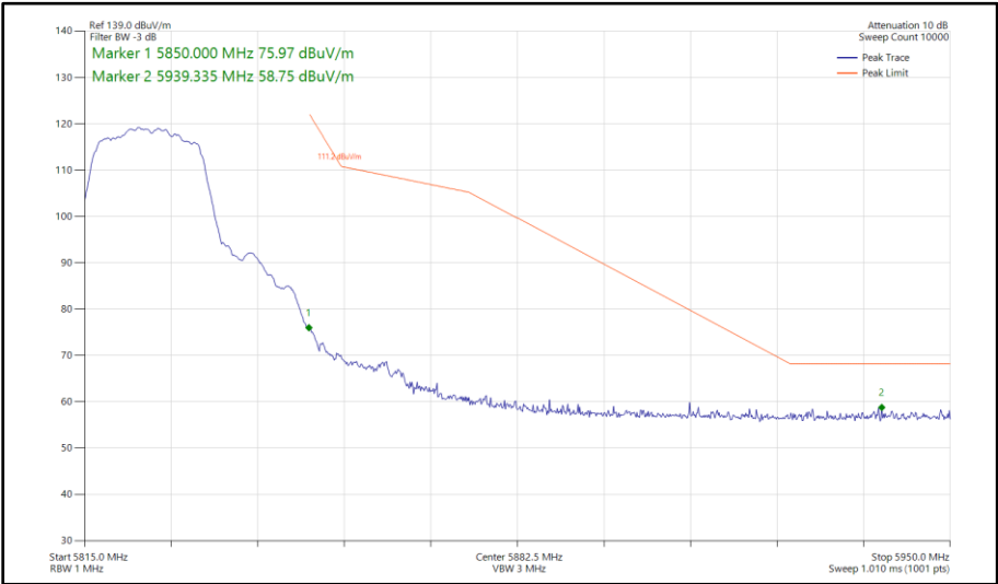
Figure 417 - 802.11a, SISO, Core 1 - 5825 MHz Band Edge Frequency 5850 MHz
