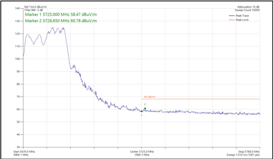
Figure 444 - 802.11ax HE20, RU 106-54, CDD, Core 0 - Core 1 - 5680 MHz Band Edge Frequency 5725 MHz
