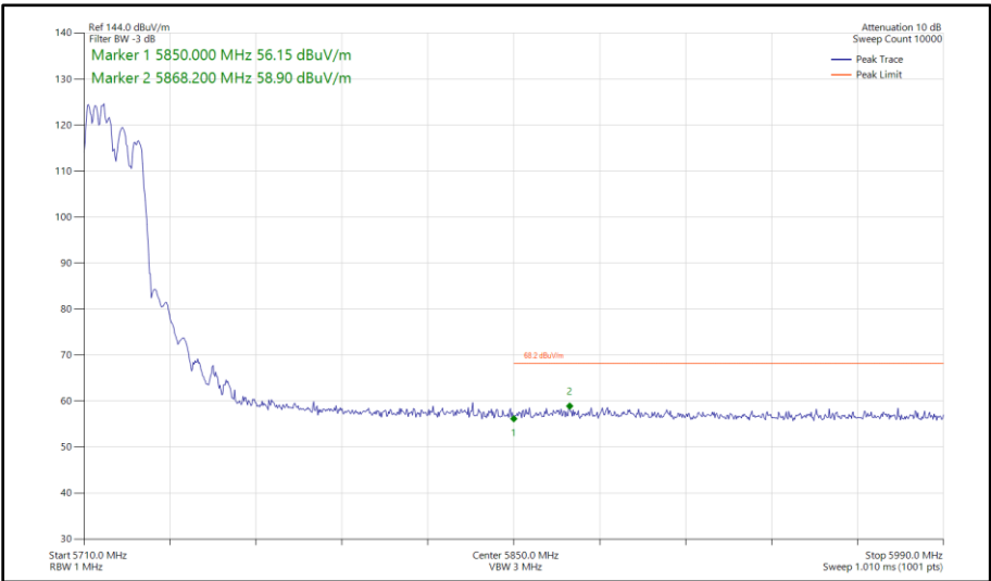
Figure 451 - 802.11ax HE20, RU 106-53, CDD, Core 0 - Core 1 - 5720 MHz Band Edge Frequency 5850 MHz
