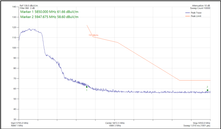
Figure 419 - 802.11n HT20, SISO, Core 1 - 5805 MHz Band Edge Frequency 5850 MHz
