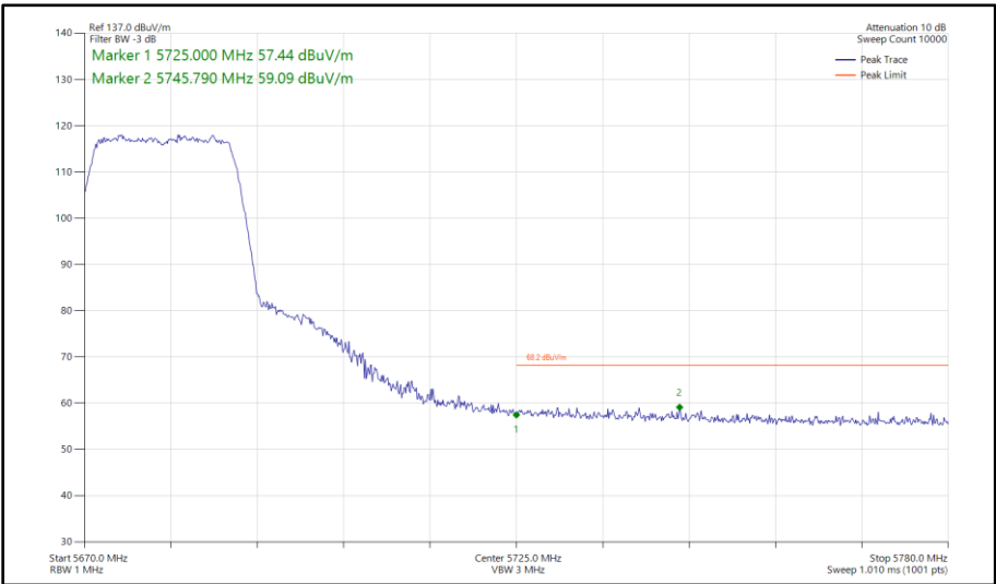
Figure 466 - 802.11n HT20, SDM, Core 0 - Core 1 - 5680 MHz Band Edge Frequency 5725 MHz
