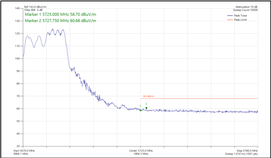
Figure 471 - 802.11ax HE20, RU 106-54, SDM, Core 0 - Core 1 - 5680 MHz Band Edge Frequency 5725 MHz
