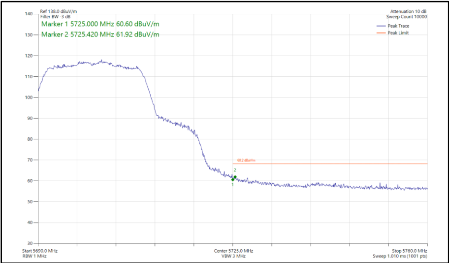
Figure 467 - 802.11n HT20, SDM, Core 0 - Core 1 - 5700 MHz Band Edge Frequency 5725 MHz
