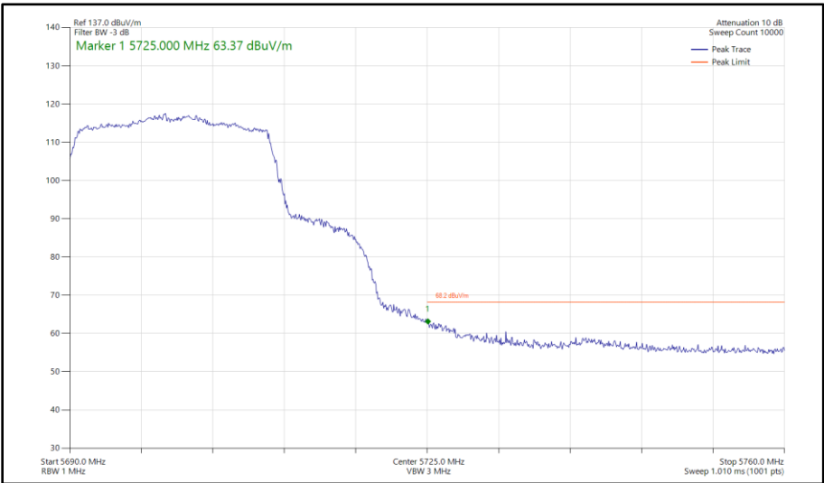
Figure 472 - 802.11ax HE20, SU, SDM, Core 0 - Core 1 - 5700 MHz Band Edge Frequency 5725 MHz
