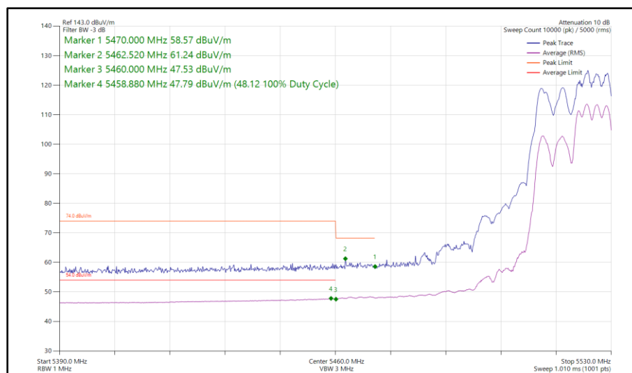
Figure 431 - 802.11ax HE20, RU 106-54, CDD, Core 0 - Core 1 - 5520 MHz Band Edge Frequency 5470 MHz
