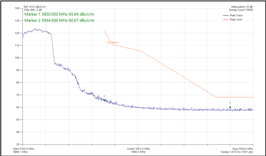
Figure 478 - 802.11ax HE20, SU, SDM, Core 0 - Core 1 - 5805 MHz Band Edge Frequency 5850 MHz
