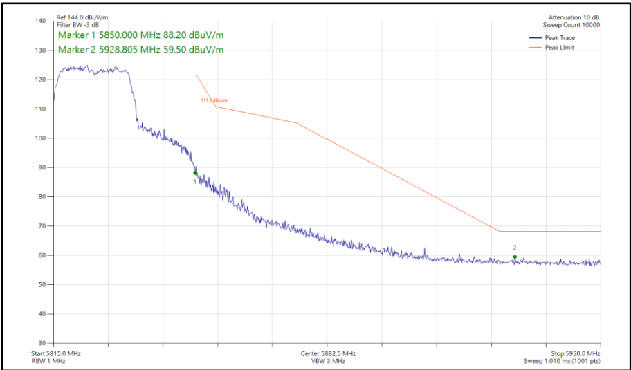
Figure 489 - 802.11ac VHT20, TxBF, Core 0 - Core 1 - 5825 MHz Band Edge Frequency 5850 MHz
