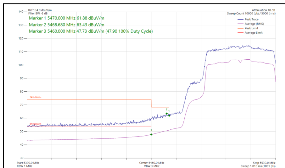
Figure 492 - 802.11ax HE40, SU, SISO, Core 0 - 5510 MHz Band Edge Frequency 5470 MHz
