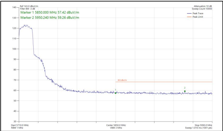
Figure 476 - 802.11ax HE20, SU, SDM, Core 0 - Core 1 - 5720 MHz Band Edge Frequency 5850 MHz
