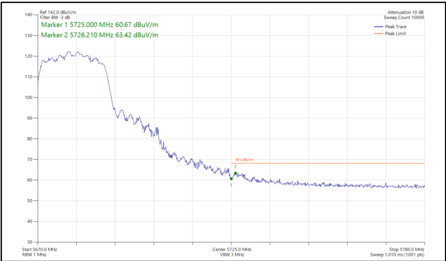
Figure 439 - 802.11n HT20, CDD, Core 0 - Core 1 - 5680 MHz Band Edge Frequency 5725 MHz
