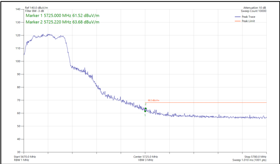
Figure 485 - 802.11ac VHT20, TxBF, Core 0 - Core 1 - 5680 MHz Band Edge Frequency 5725 MHz
