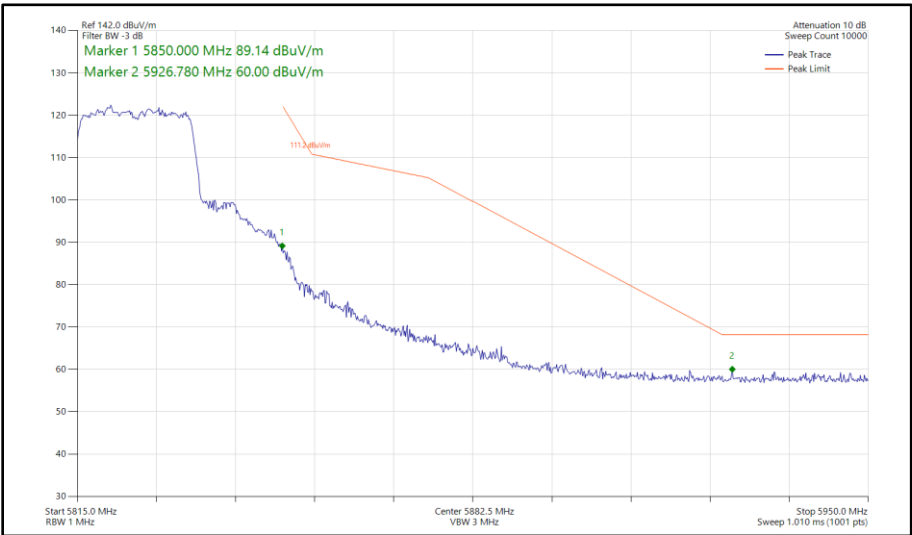
Figure 479 - 802.11ax HE20, SU, SDM, Core 0 - Core 1 - 5825 MHz Band Edge Frequency 5850 MHz
