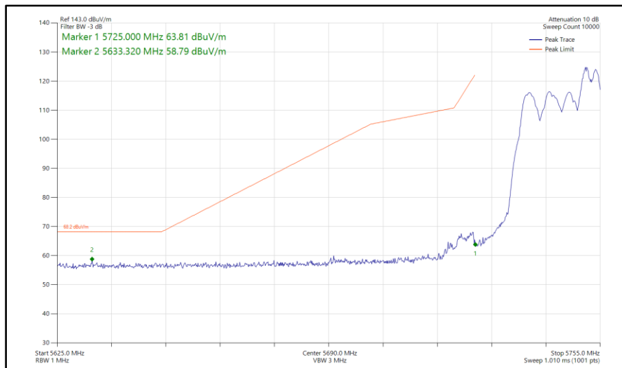
Figure 436 - 802.11ax HE20, RU 52-40, CDD, Core 0 - Core 1 - 5745 MHz Band Edge Frequency 5725 MHz
