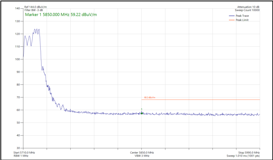
Figure 477 - 802.11ax HE20, RU 106-54, SDM, Core 0 - Core 1 - 5720 MHz Band Edge Frequency 5850 MHz
