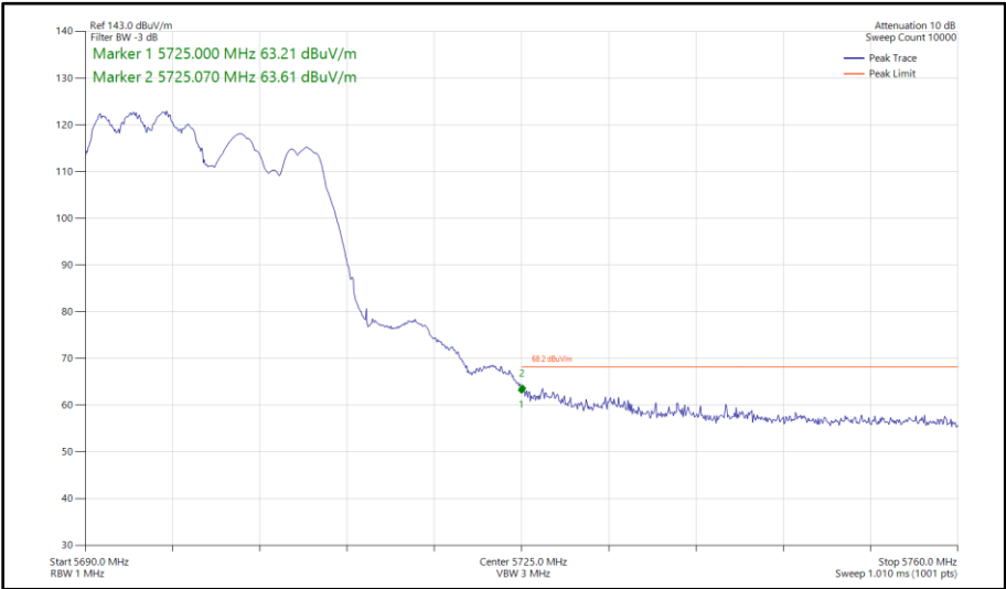
Figure 473 - 802.11ax HE20, RU 106-53, SDM, Core 0 - Core 1 - 5700 MHz Band Edge Frequency 5725 MHz
