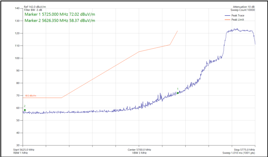
Figure 484 - 802.11ac VHT20, TxBF, Core 0 - Core 1 - 5765 MHz Band Edge Frequency 5725 MHz
