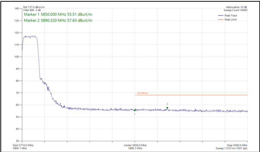
Figure 474 - 802.11n HT20, SDM, Core 0 - Core 1 - 5720 MHz Band Edge Frequency 5850 MHz
