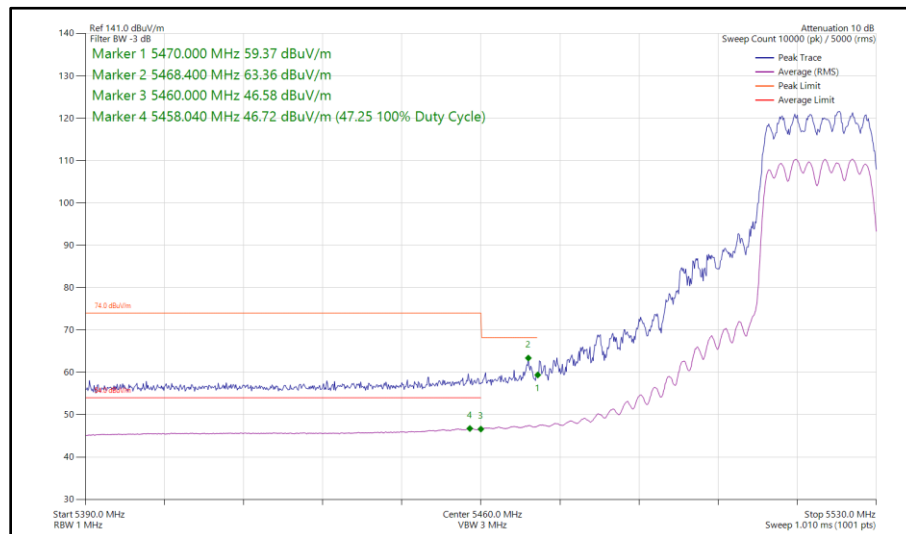
Figure 430 - 802.11ax HE20, SU, CDD, Core 0 - Core 1 - 5520 MHz Band Edge Frequency 5470 MHz
