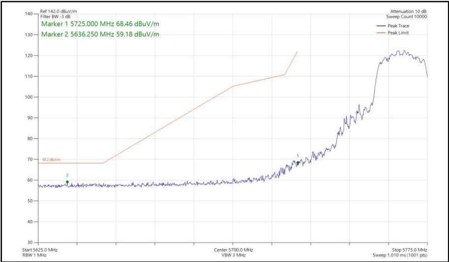
Figure 434 - 802.11n HT20, CDD, Core 0 - Core 1 - 5765 MHz Band Edge Frequency 5725 MHz
