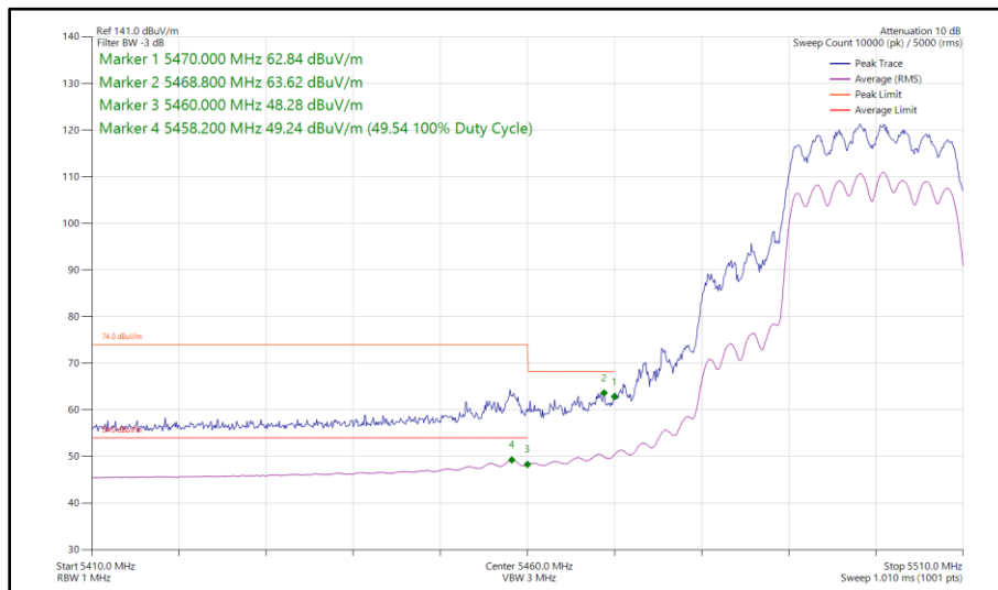
Figure 428 - 802.11ax HE20, SU, CDD, Core 0 - Core 1 - 5500 MHz Band Edge Frequency 5470 MHz
