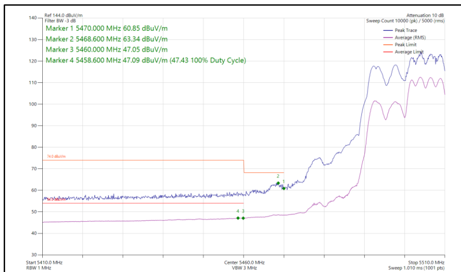
Figure 429 - 802.11ax HE20, RU 106-54, CDD, Core 0 - Core 1 - 5500 MHz Band Edge Frequency 5470 MHz
