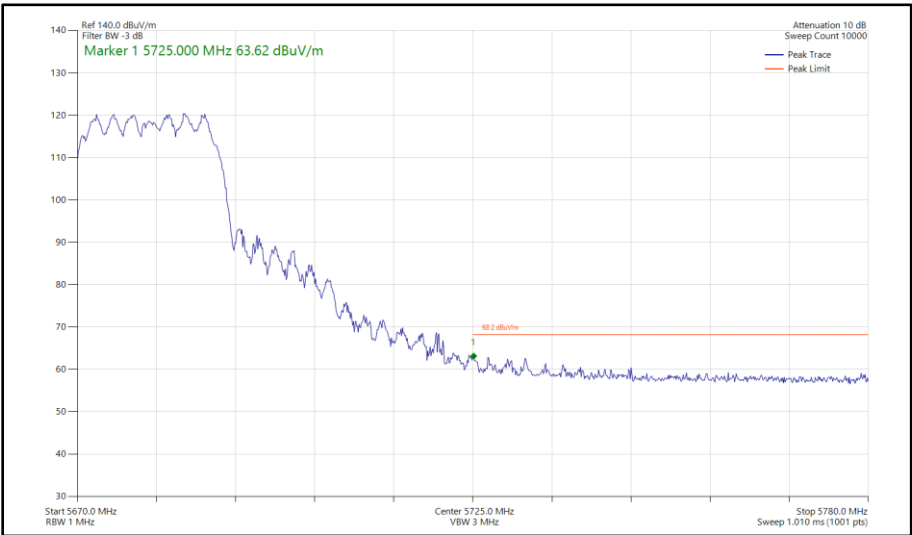
Figure 443 - 802.11ax HE20, SU, CDD, Core 0 - Core 1 - 5680 MHz Band Edge Frequency 5725 MHz
