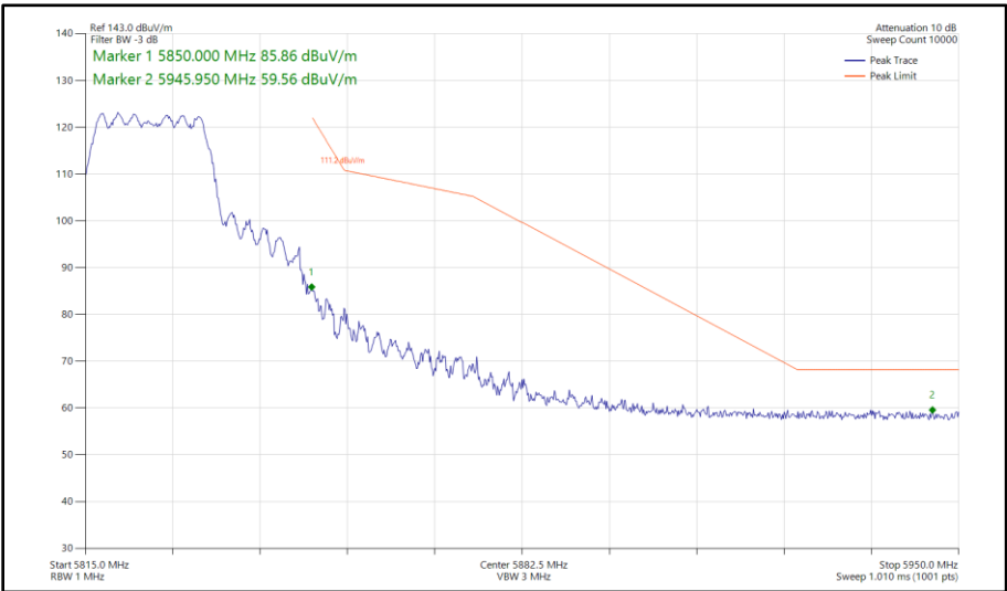
Figure 449 - 802.11n HT20, CDD, Core 0 - Core 1 - 5825 MHz Band Edge Frequency 5850 MHz
