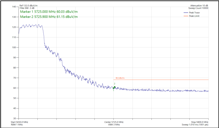
Figure 438 - 802.11n HT20, CDD, Core 0 - Core 1 - 5660 MHz Band Edge Frequency 5725 MHz
