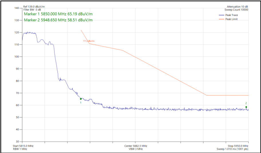
Figure 425 - 802.11ax HE20, RU 106-53, SISO, Core 1 - 5825 MHz Band Edge Frequency 5850 MHz
