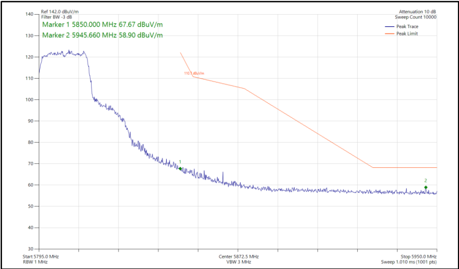
Figure 488 - 802.11ac VHT20, TxBF, Core 0 - Core 1 - 5805 MHz Band Edge Frequency 5850 MHz
