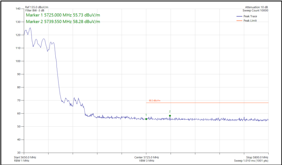
Figure 469 - 802.11ax HE20, RU 52-37, SDM, Core 0 - Core 1 - 5660 MHz Band Edge Frequency 5725 MHz
