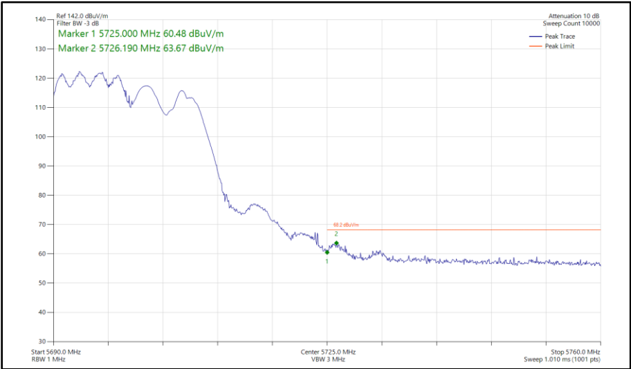
Figure 446 - 802.11ax HE20, RU 106-53, CDD, Core 0 - Core 1 - 5700 MHz Band Edge Frequency 5725 MHz
