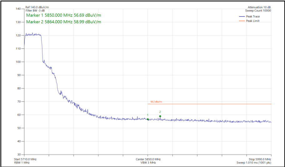
Figure 421 - 802.11ax HE20, SU, SISO, Core 1 - 5720 MHz Band Edge Frequency 5850 MHz
