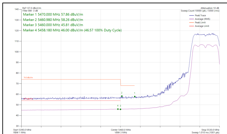
Figure 456 - 802.11n HT20, SDM, Core 0 - Core 1 - 5520 MHz Band Edge Frequency 5470 MHz
