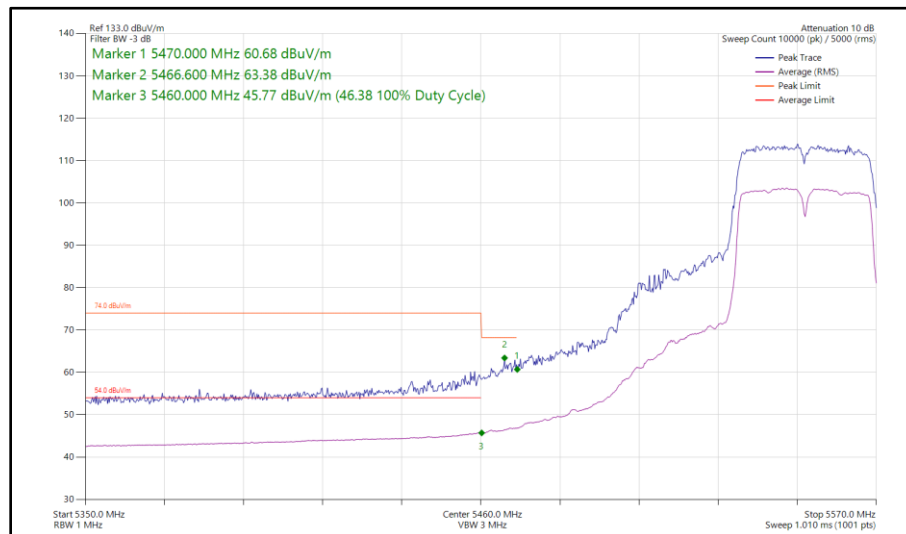
Figure 491 - 802.11n HT40, SISO, Core 0 - 5550 MHz Band Edge Frequency 5470 MHz
