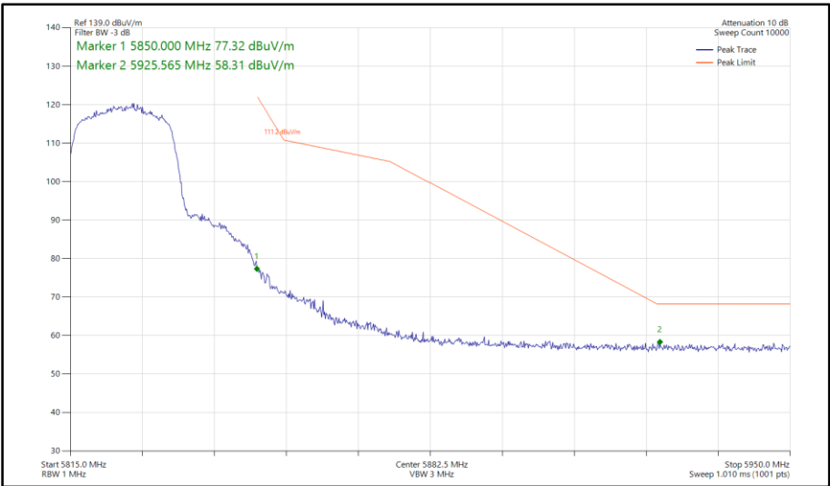
Figure 420 - 802.11n HT20, SISO, Core 1 - 5825 MHz Band Edge Frequency 5850 MHz
