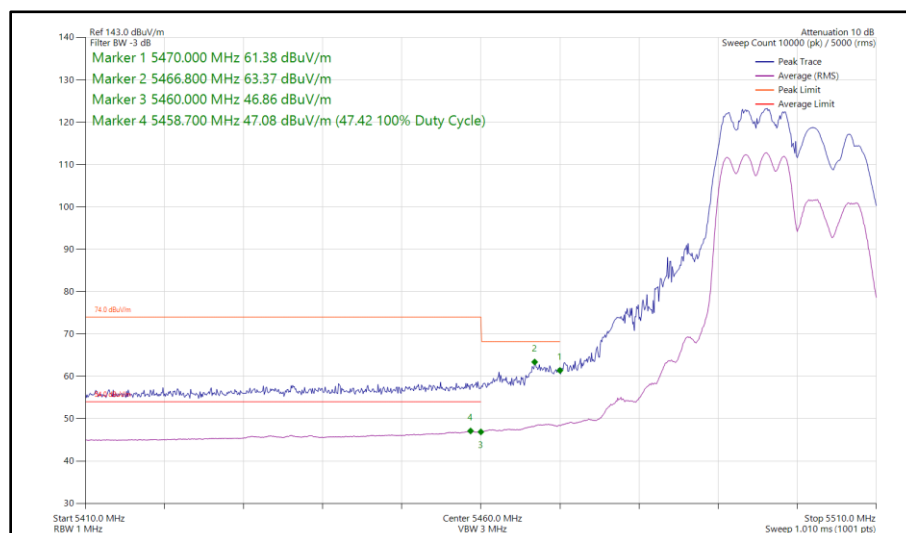
Figure 458 - 802.11ax HE20, RU 106-53, SDM, Core 0 - Core 1 - 5500 MHz Band Edge Frequency 5470 MHz
