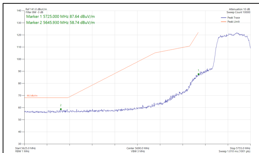
Figure 483 - 802.11ac VHT20, TxBF, Core 0 - Core 1 - 5745 MHz Band Edge Frequency 5725 MHz
