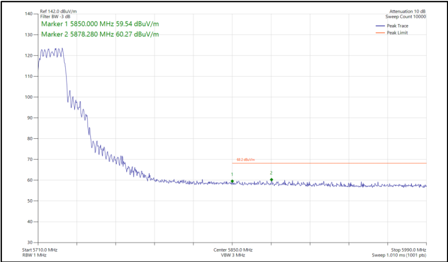
Figure 450 - 802.11ax HE20, SU, CDD, Core 0 - Core 1 - 5720 MHz Band Edge Frequency 5850 MHz
