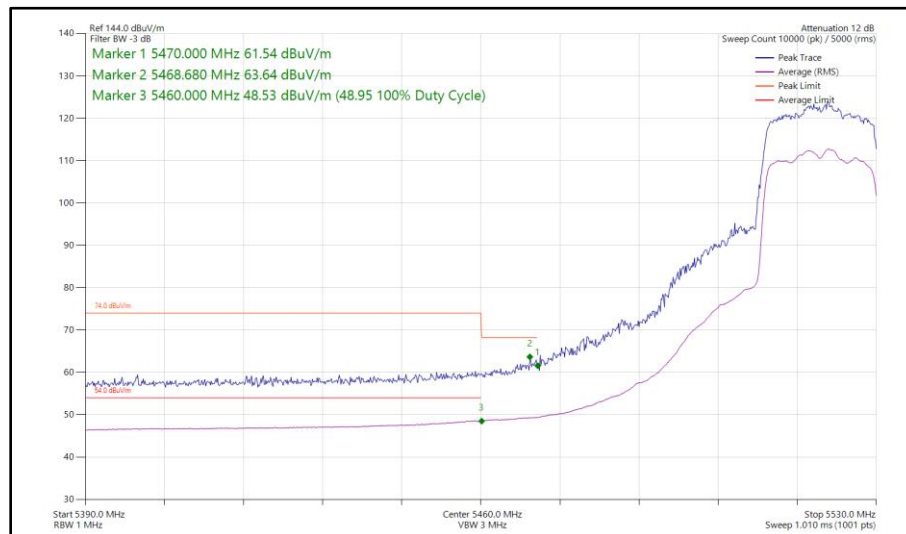
Figure 459 - 802.11ax HE20, SU, SDM, Core 0 - Core 1 - 5520 MHz Band Edge Frequency 5470 MHz
