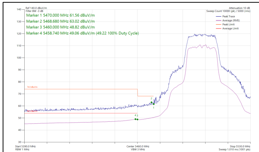
Figure 482 - 802.11ac VHT20, TxBF, Core 0 - Core 1 - 5520 MHz Band Edge Frequency 5470 MHz
