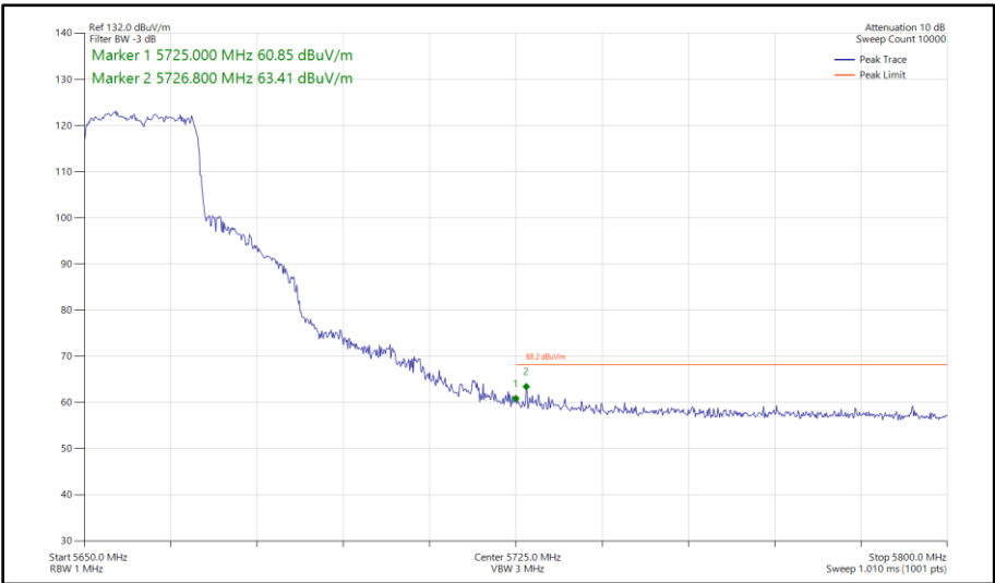
Figure 468 - 802.11ax HE20, SU, SDM, Core 0 - Core 1 - 5660 MHz Band Edge Frequency 5725 MHz
