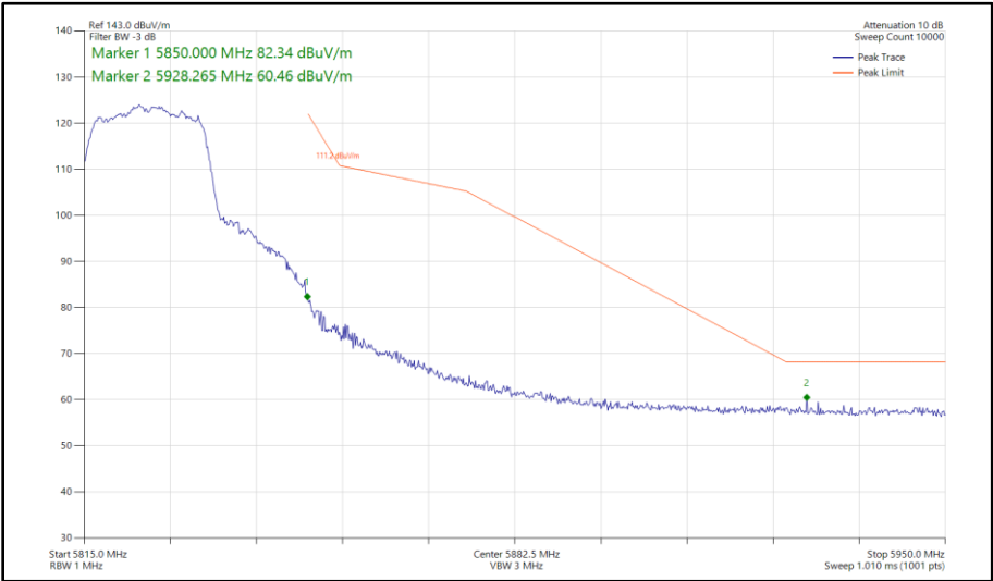
Figure 475 - 802.11n HT20, SDM, Core 0 - Core 1 - 5825 MHz Band Edge Frequency 5850 MHz
