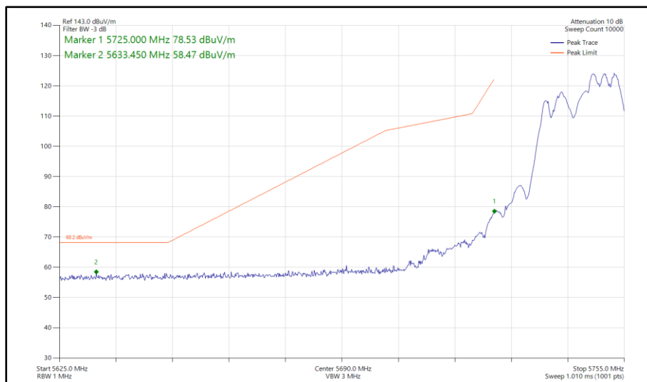
Figure 464 - 802.11ax HE20, RU 106-54, SDM, Core 0 - Core 1 - 5745 MHz Band Edge Frequency 5725 MHz
