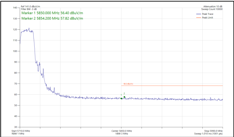
Figure 487 - 802.11ac VHT20, TxBF, Core 0 - Core 1 - 5720 MHz Band Edge Frequency 5850 MHz
