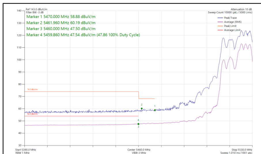
Figure 460 - 802.11ax HE20, RU 106-54, SDM, Core 0 - Core 1 - 5520 MHz Band Edge Frequency 5470 MHz
