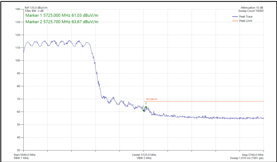
Figure 445 - 802.11ax HE20, SU, CDD, Core 0 - Core 1 - 5700 MHz Band Edge Frequency 5725 MHz
