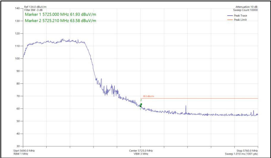
Figure 486 - 802.11ac VHT20, TxBF, Core 0 - Core 1 - 5700 MHz Band Edge Frequency 5725 MHz
