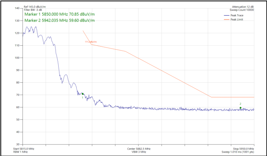
Figure 454 - 802.11ax HE20, RU 106-53, CDD, Core 0 - Core 1 - 5825 MHz Band Edge Frequency 5850 MHz
