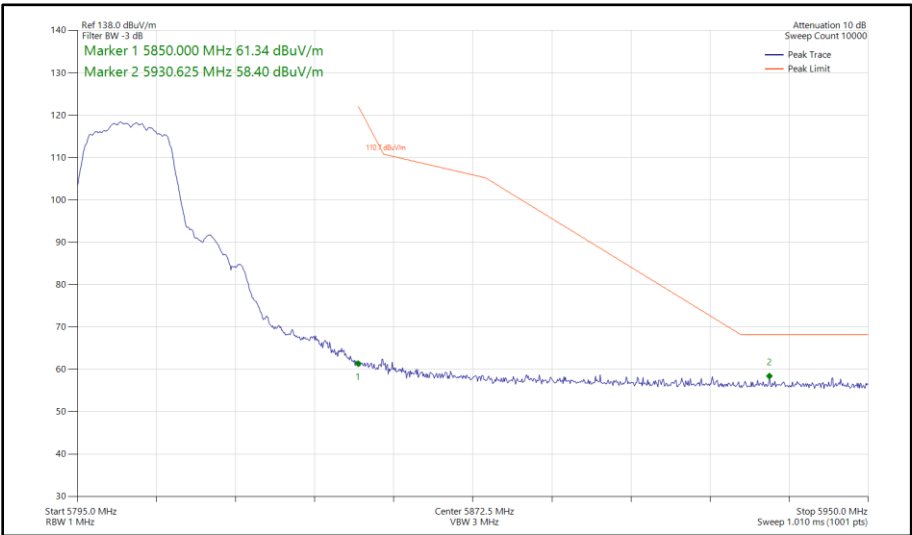
Figure 416 - 802.11a, SISO, Core 1 - 5805 MHz Band Edge Frequency 5850 MHz
