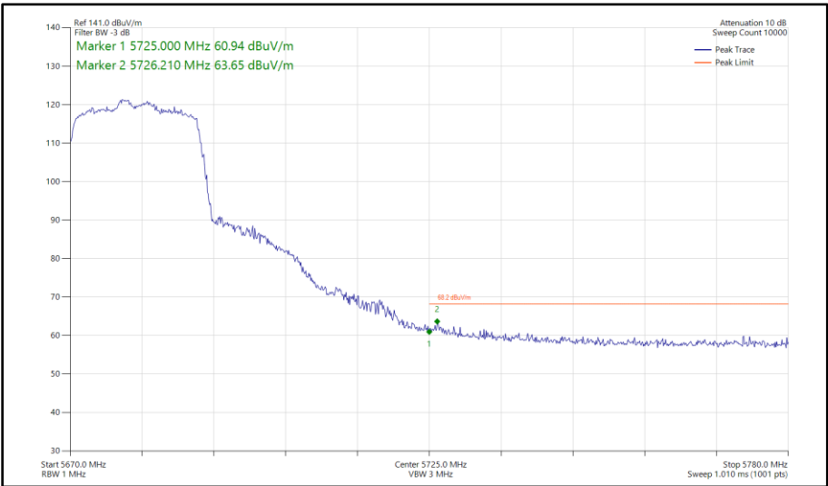
Figure 470 - 802.11ax HE20, SU, SDM, Core 0 - Core 1 - 5680 MHz Band Edge Frequency 5725 MHz
