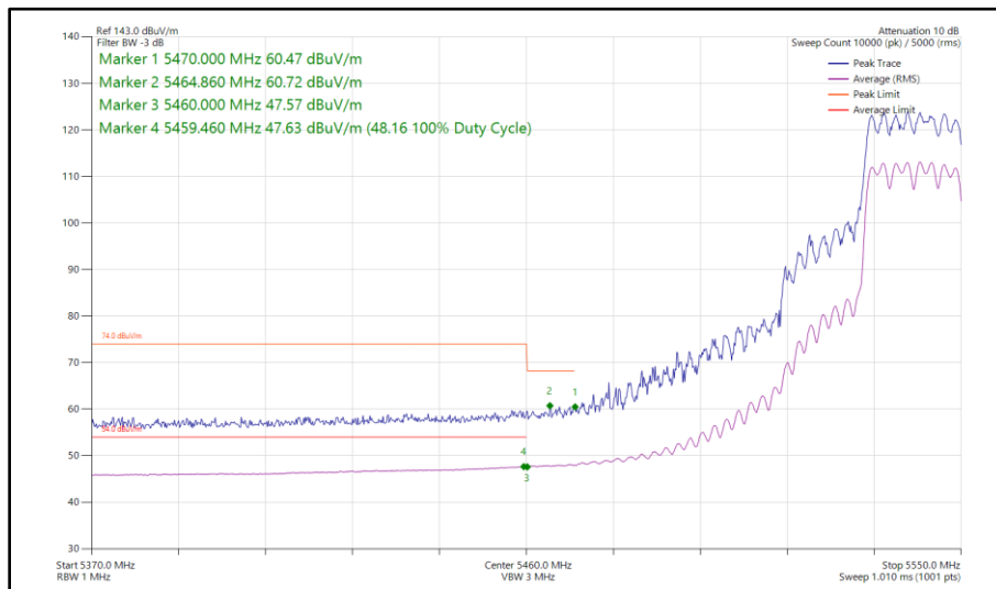
Figure 432 - 802.11ax HE20, SU, CDD, Core 0 - Core 1 - 5540 MHz Band Edge Frequency 5470 MHz
