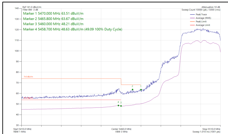
Figure 457 - 802.11ax HE20, SU, SDM, Core 0 - Core 1 - 5500 MHz Band Edge Frequency 5470 MHz
