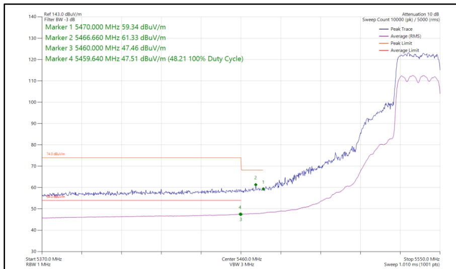
Figure 461 - 802.11ax HE20, SU, SDM, Core 0 - Core 1 - 5540 MHz Band Edge Frequency 5470 MHz
