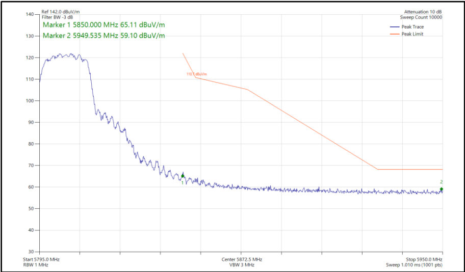
Figure 448 - 802.11n HT20, CDD, Core 0 - Core 1 - 5805 MHz Band Edge Frequency 5850 MHz
