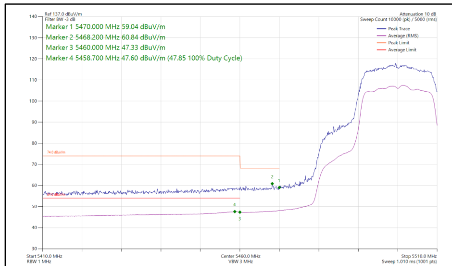
Figure 455 - 802.11n HT20, SDM, Core 0 - Core 1 - 5500 MHz Band Edge Frequency 5470 MHz
