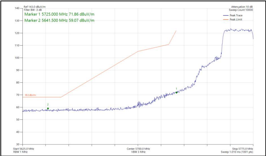
Figure 465 - 802.11ax HE20, SU, SDM, Core 0 - Core 1 - 5765 MHz Band Edge Frequency 5725 MHz
