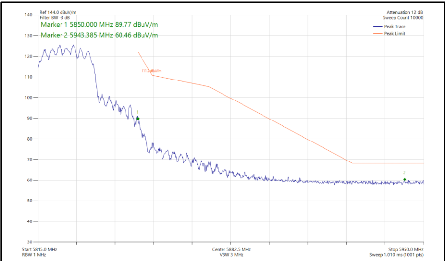
Figure 453 - 802.11ax HE20, SU, CDD, Core 0 - Core 1 - 5825 MHz Band Edge Frequency 5850 MHz
