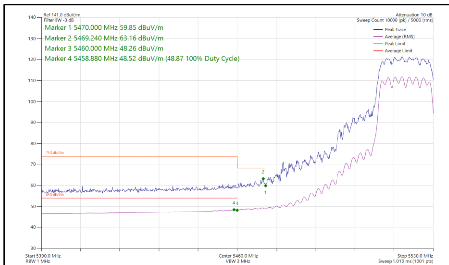
Figure 427 - 802.11n HT20, CDD, Core 0 - Core 1 - 5520 MHz Band Edge Frequency 5470 MHz
