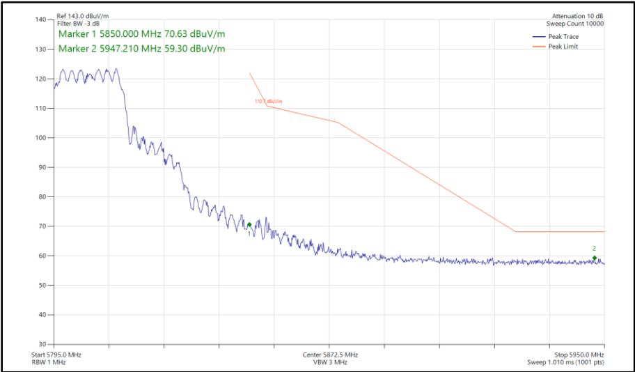
Figure 452 - 802.11ax HE20, SU, CDD, Core 0 - Core 1 - 5805 MHz Band Edge Frequency 5850 MHz
