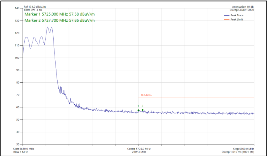
Figure 442 - 802.11ax HE20, RU 52-40, CDD, Core 0 - Core 1 - 5660 MHz Band Edge Frequency 5725 MHz
