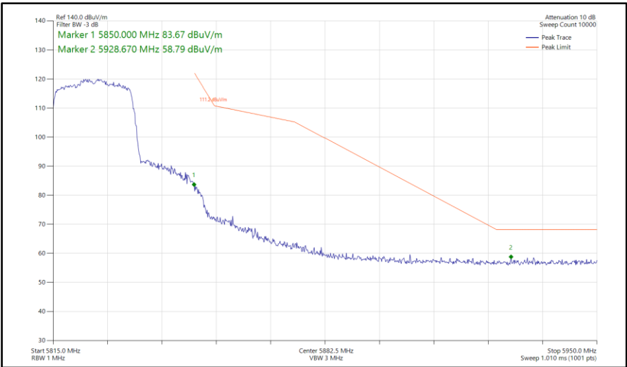
Figure 424 - 802.11ax HE20, SU, SISO, Core 1 - 5825 MHz Band Edge Frequency 5850 MHz
