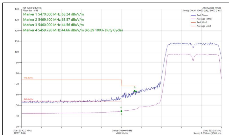
Figure 490 - 802.11n HT40, SISO, Core 0 - 5510 MHz Band Edge Frequency 5470 MHz
