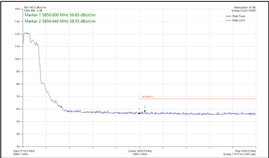
Figure 422 - 802.11ax HE20, RU 106-53, SISO, Core 1 - 5720 MHz Band Edge Frequency 5850 MHz
