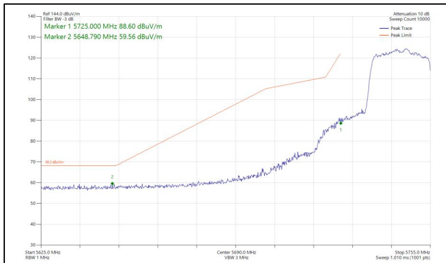
Figure 463 - 802.11ax HE20, SU, SDM, Core 0 - Core 1 - 5745 MHz Band Edge Frequency 5725 MHz
