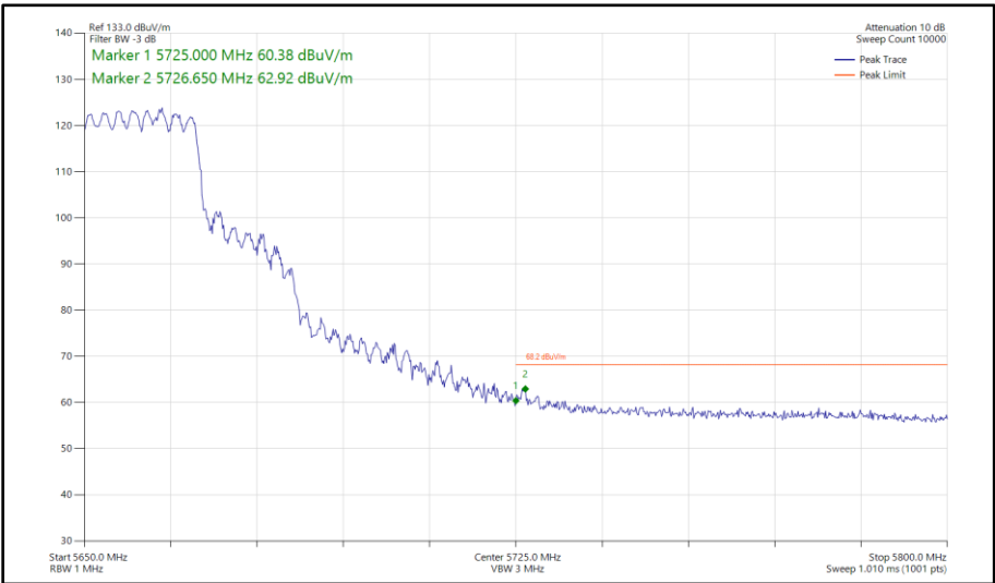
Figure 441 - 802.11ax HE20, SU, CDD, Core 0 - Core 1 - 5660 MHz Band Edge Frequency 5725 MHz
