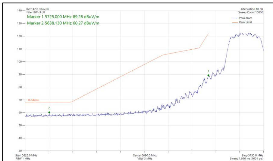
Figure 433 - 802.11n HT20, CDD, Core 0 - Core 1 - 5745 MHz Band Edge Frequency 5725 MHz
