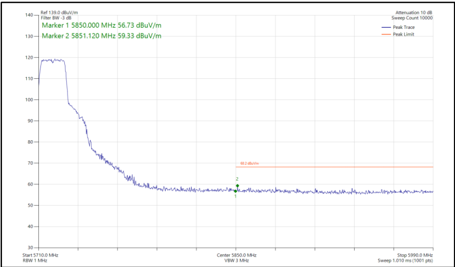
Figure 418 - 802.11n HT20, SISO, Core 1 - 5720 MHz Band Edge Frequency 5850 MHz
