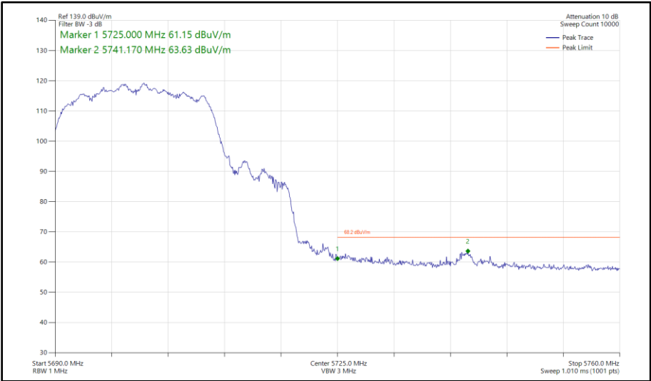
Figure 440 - 802.11n HT20, CDD, Core 0 - Core 1 - 5700 MHz Band Edge Frequency 5725 MHz
