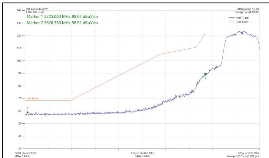
Figure 462 - 802.11n HT20, SDM, Core 0 - Core 1 - 5745 MHz Band Edge Frequency 5725 MHz
