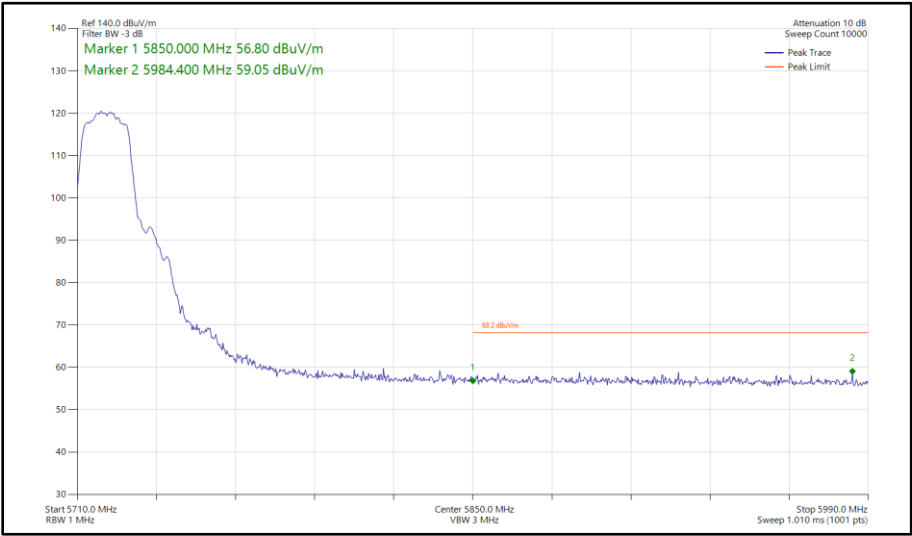
Figure 415 - 802.11a, SISO, Core 1 - 5720 MHz Band Edge Frequency 5850 MHz
