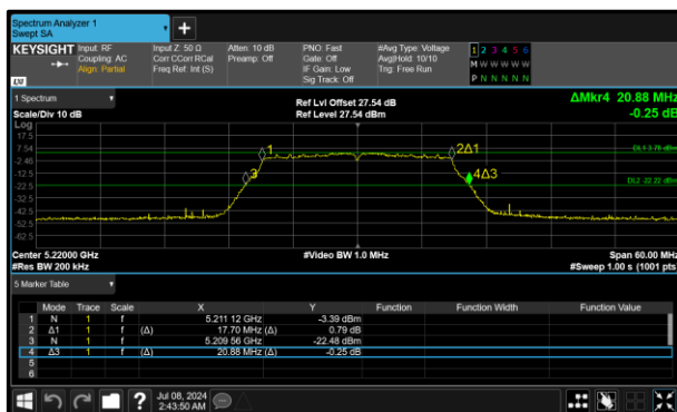
Figure 346 - 802.11ac VHT20 Minimum 99% OBW
