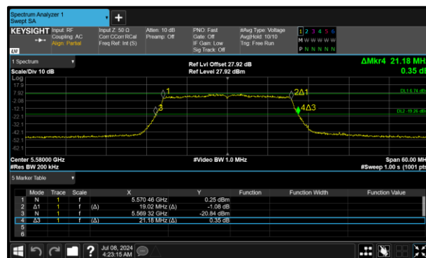
Figure 347 - 802.11ac VHT20 Maximum 99% OBW
