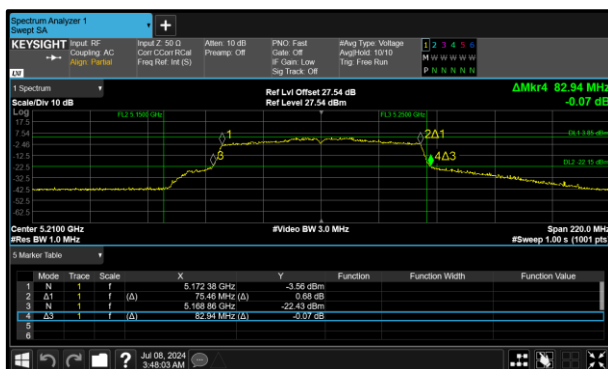
Figure 350 - 802.11ac VHT80 Minimum 99% OBW
