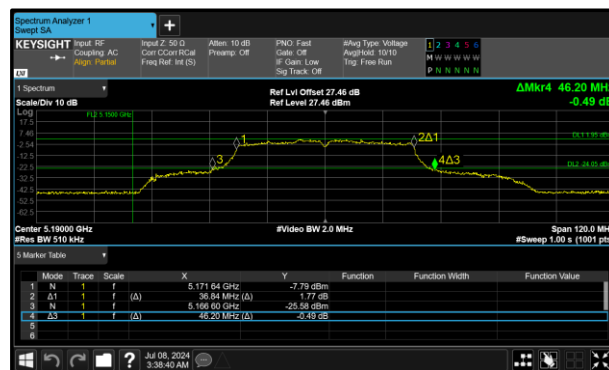
Figure 349 - 802.11ac VHT40 Maximum 99% OBW
