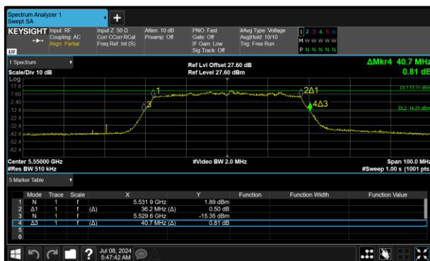
Figure 348 - 802.11ac VHT40 Minimum 99% OBW
