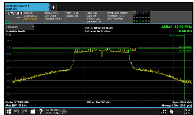
Figure 287 - 802.11n HT40 Maximum 6 dB EBW
