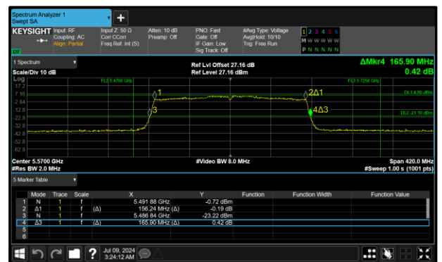
Figure 311 - 802.11ax HE160 SU Maximum 99% OBW
