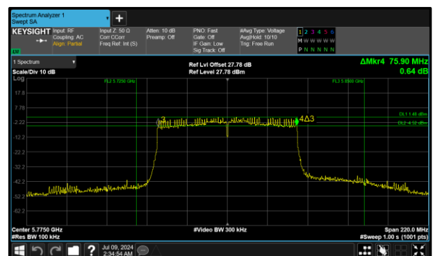
Figure 289 - 802.11ac VHT80 Maximum 6 dB EBW
