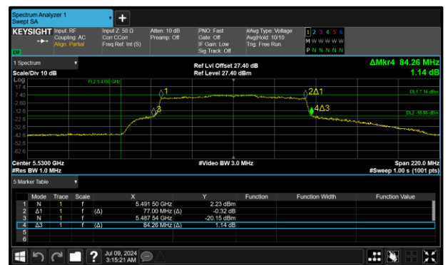
Figure 309 - 802.11ax HE80 SU Maximum 99% OBW
