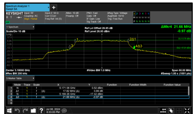
Figure 269 - 802.11n HT20 Maximum 99% OBW
