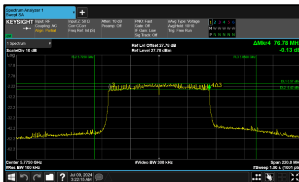
Figure 294 - 802.11ax HE80 SU Minimum 6 dB EBW
