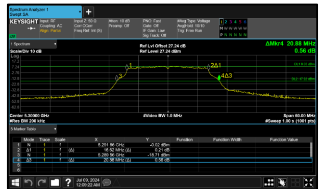
Figure 267 - 802.11a Maximum 99% OBW
