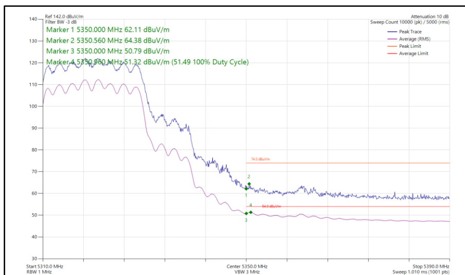
Figure 61 - 802.11ax HE20, SU, CDD, Core 0 - Core 1 - 5320 MHz Band Edge Frequency 5350 MHz
