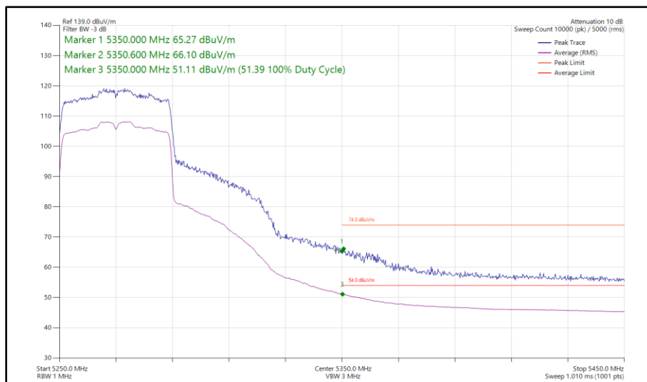
Figure 119 - 802.11ax HE40, SU, SISO, Core 1 - 5270 MHz Band Edge Frequency 5350 MHz
