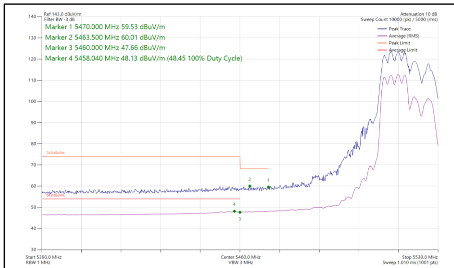
Figure 85 - 802.11ax HE20, RU 106-53, SDM, Core 0 - Core 1 - 5520 MHz Band Edge Frequency 5460 MHz
