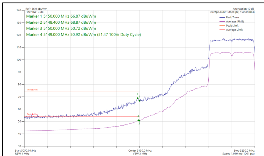
Figure 115 - 802.11ax HE40, SU, SISO, Core 1 - 5230 MHz Band Edge Frequency 5150 MHz
