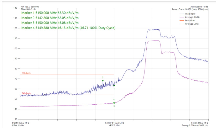
Figure 114 - 802.11ax HE40, RU 106-53, SISO, Core 1 - 5190 MHz Band Edge Frequency 5150 MHz
