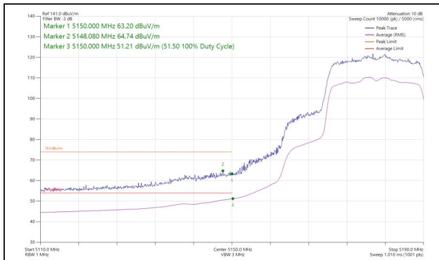
Figure 71 - 802.11ax HE20, SU, SDM, Core 0 - Core 1 - 5180 MHz Band Edge Frequency 5150 MHz
