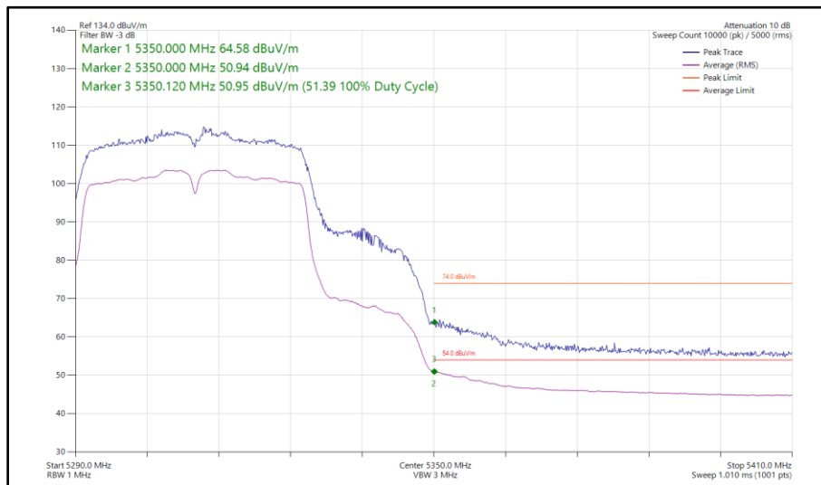
Figure 118 - 802.11n HT40, SISO, Core 1 - 5310 MHz Band Edge Frequency 5350 MHz
