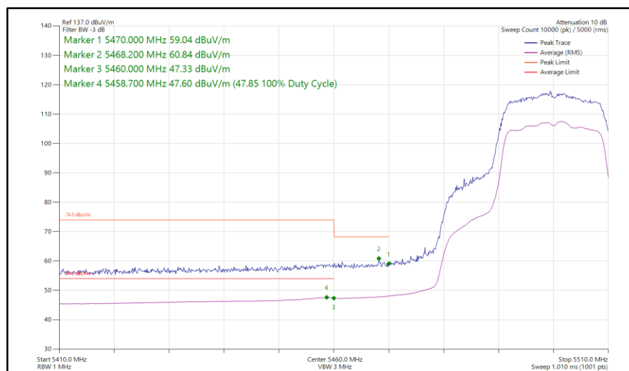
Figure 80 - 802.11n HT20, SDM, Core 0 - Core 1 - 5500 MHz Band Edge Frequency 5460 MHz
