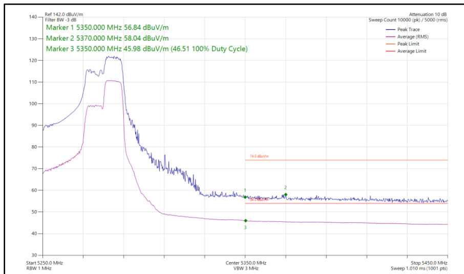
Figure 102 - 802.11ax HE40, RU 106-56, SISO, Core 0 - 5270 MHz Band Edge Frequency 5350 MHz
