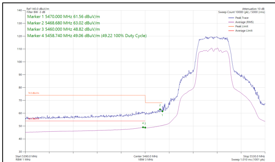
Figure 92 - 802.11ac VHT20, TxBF, Core 0 - Core 1 - 5520 MHz Band Edge Frequency 5460 MHz
