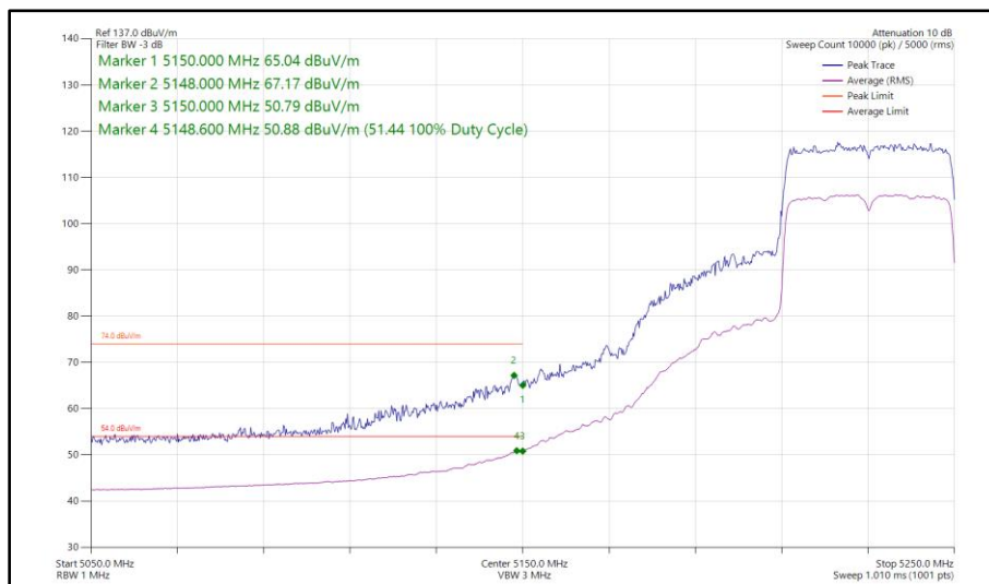
Figure 97 - 802.11ax HE40, SU, SISO, Core 0 - 5230 MHz Band Edge Frequency 5150 MHz
