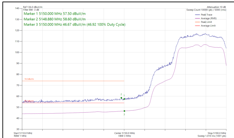
Figure 70 - 802.11n HT20, SDM, Core 0 - Core 1 - 5180 MHz Band Edge Frequency 5150 MHz
