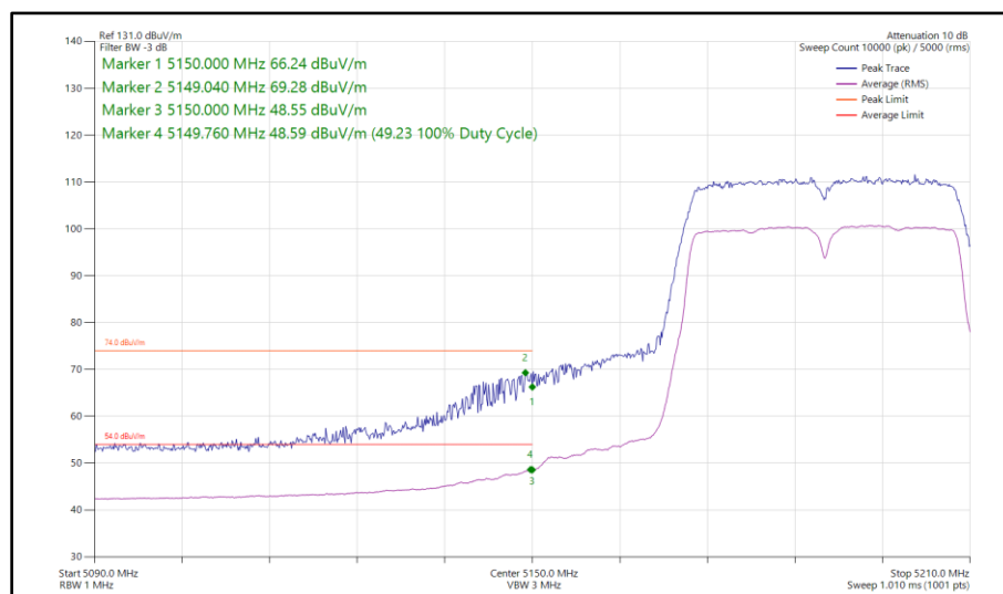
Figure 93 - 802.11n HT40, SISO, Core 0 - 5190 MHz Band Edge Frequency 5150 MHz
