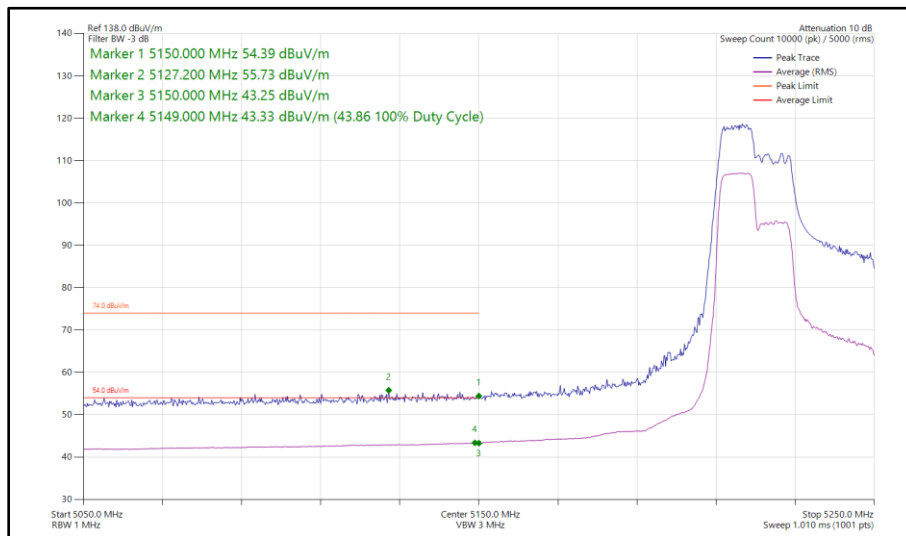
Figure 116 - 802.11ax HE40, RU 106-53, SISO, Core 1 - 5230 MHz Band Edge Frequency 5150 MHz
