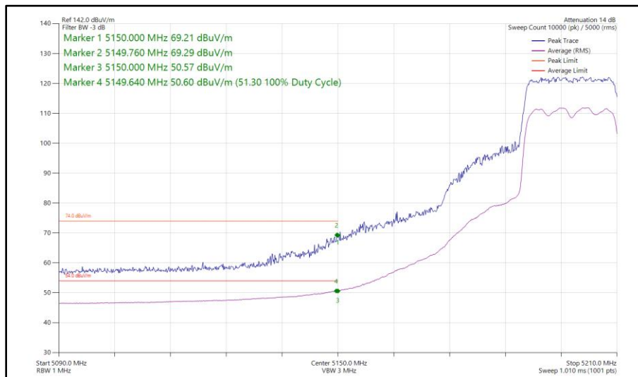
Figure 73 - 802.11ax HE20, SU, SDM, Core 0 - Core 1 - 5200 MHz Band Edge Frequency 5150 MHz
