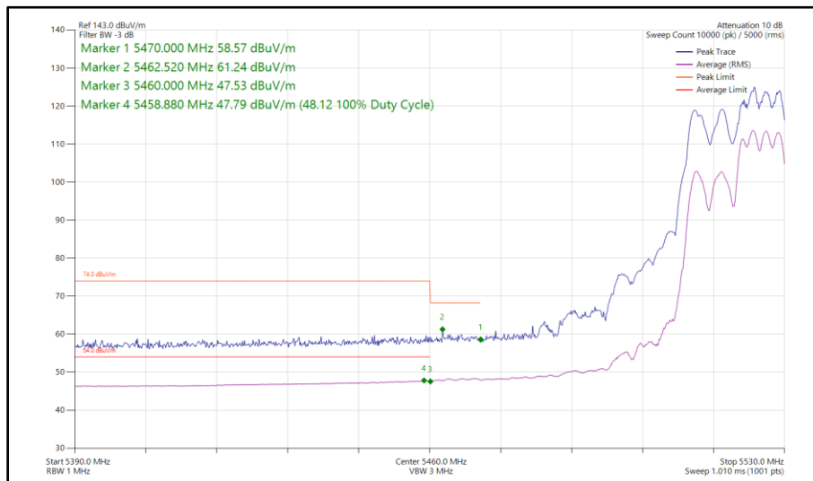
Figure 68 - 802.11ax HE20, RU 106-54, CDD, Core 0 - Core 1 - 5520 MHz Band Edge Frequency 5460 MHz
