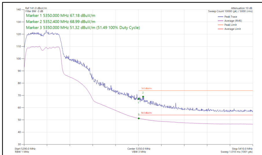
Figure 89 - 802.11ac VHT20, TxBF, Core 0 - Core 1 - 5300 MHz Band Edge Frequency 5350 MHz
