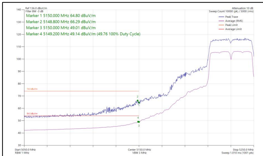
Figure 112 - 802.11n HT40, SISO, Core 1 - 5230 MHz Band Edge Frequency 5150 MHz
