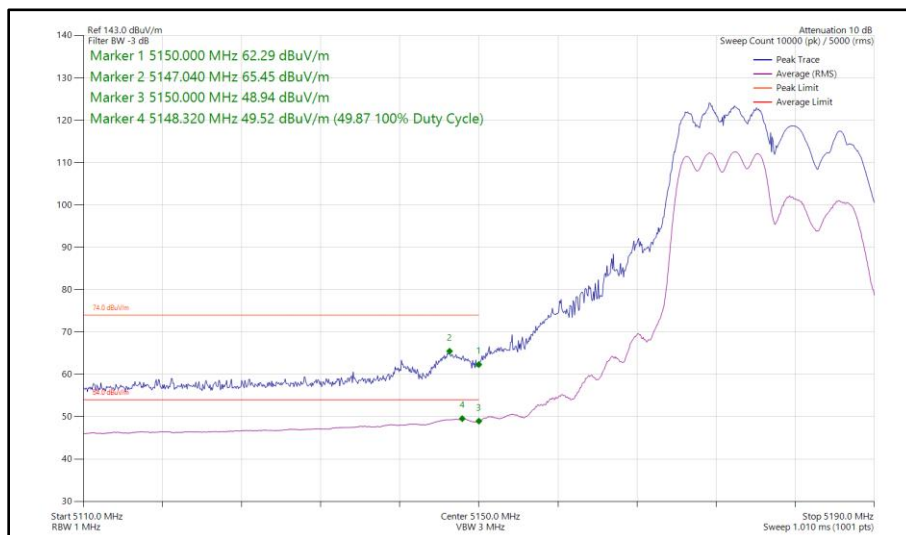
Figure 72 - 802.11ax HE20, RU 106-53, SDM, Core 0 - Core 1 - 5180 MHz Band Edge Frequency 5150 MHz
