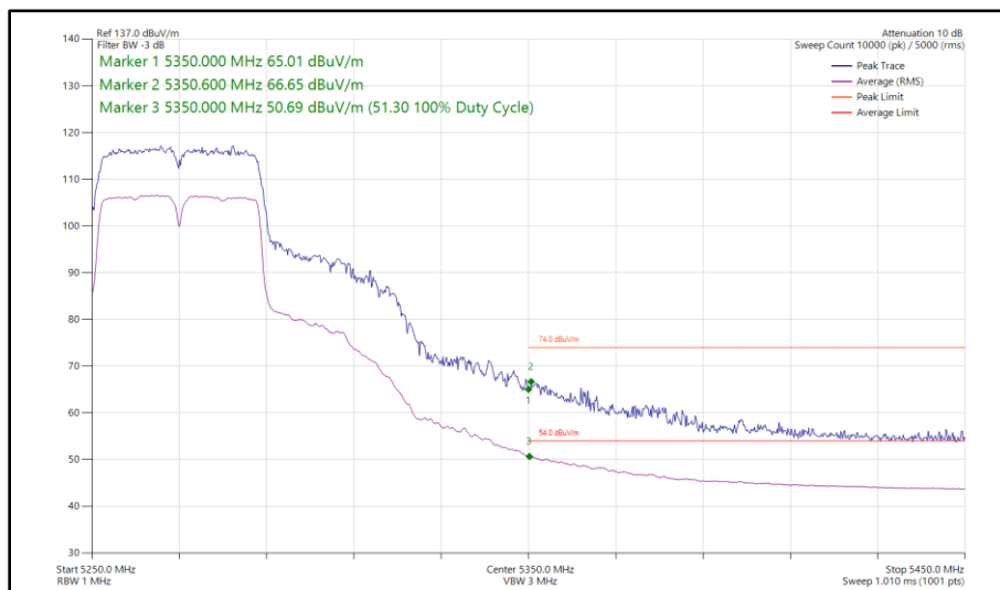
Figure 99 - 802.11n HT40, SISO, Core 0 - 5270 MHz Band Edge Frequency 5350 MHz
