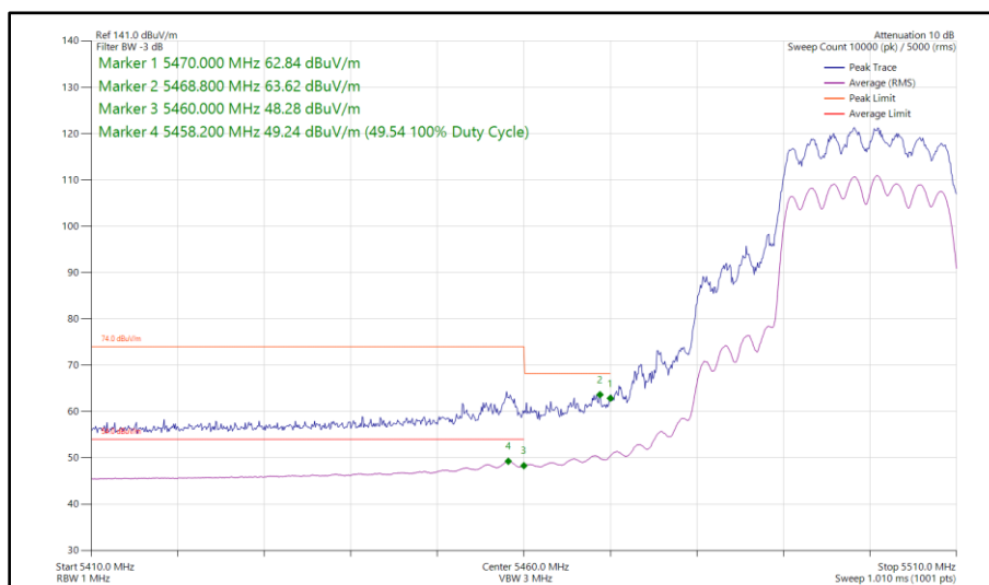
Figure 65 - 802.11ax HE20, SU, CDD, Core 0 - Core 1 - 5500 MHz Band Edge Frequency 5460 MHz
