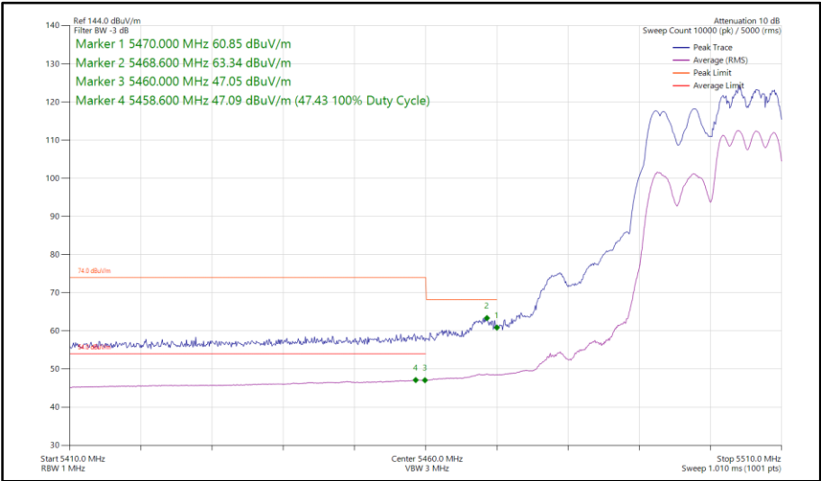
Figure 66 - 802.11ax HE20, RU 106-54, CDD, Core 0 - Core 1 - 5500 MHz Band Edge Frequency 5460 MHz
