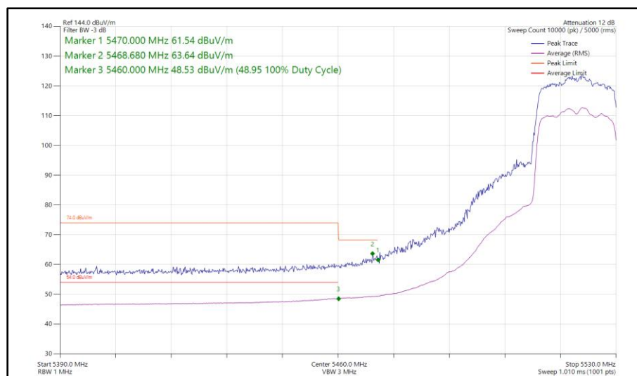
Figure 84 - 802.11ax HE20, SU, SDM, Core 0 - Core 1 - 5520 MHz Band Edge Frequency 5460 MHz
