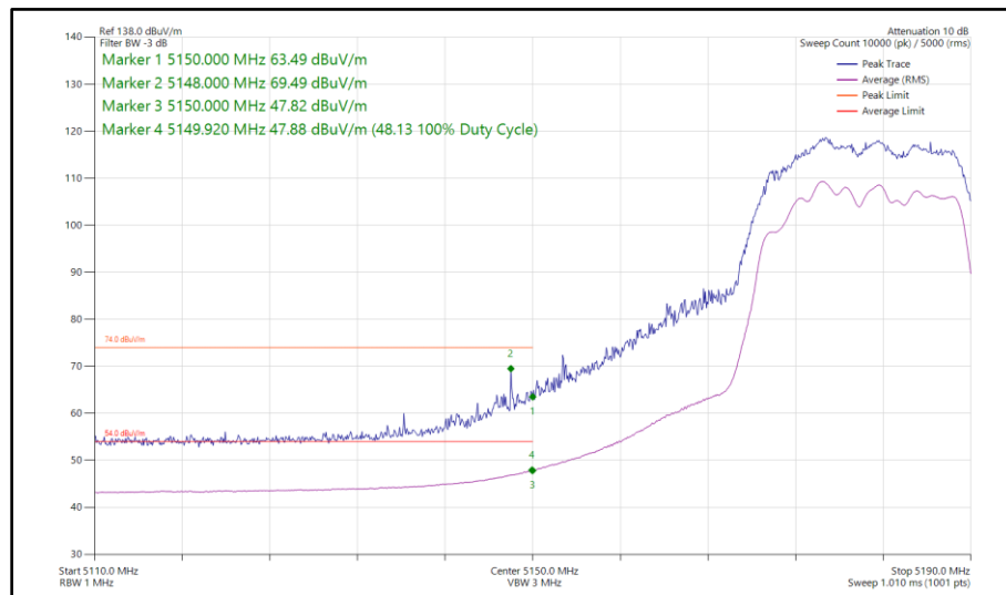
Figure 87 - 802.11ac VHT20, TxBF, Core 0 - Core 1 - 5180 MHz Band Edge Frequency 5150 MHz
