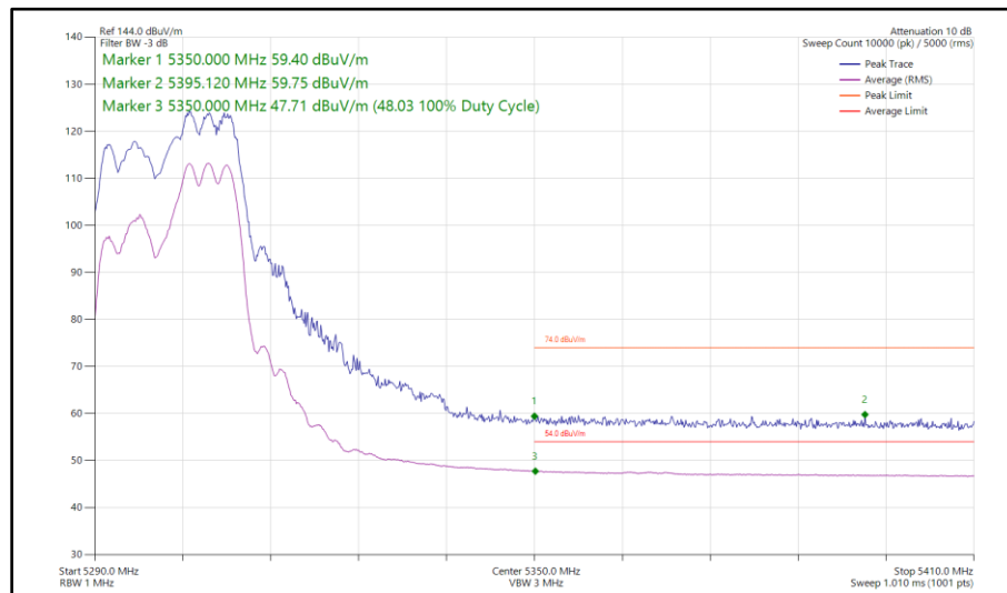
Figure 77 - 802.11ax HE20, RU 106-54, SDM, Core 0 - Core 1 - 5300 MHz Band Edge Frequency 5350 MHz
