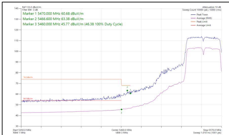
Figure 106 - 802.11n HT40, SISO, Core 0 - 5550 MHz Band Edge Frequency 5460 MHz
