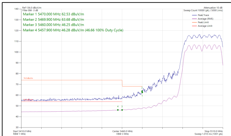
Figure 63 - 802.11n HT20, CDD, Core 0 - Core 1 - 5500 MHz Band Edge Frequency 5460 MHz
