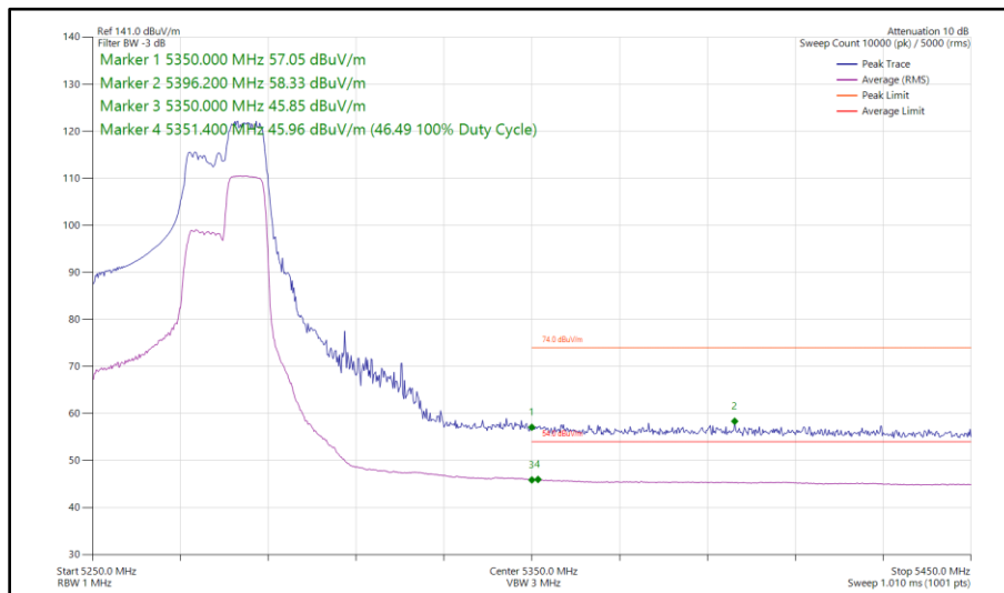
Figure 120 - 802.11ax HE40, RU 106-56, SISO, Core 1 - 5270 MHz Band Edge Frequency 5350 MHz
