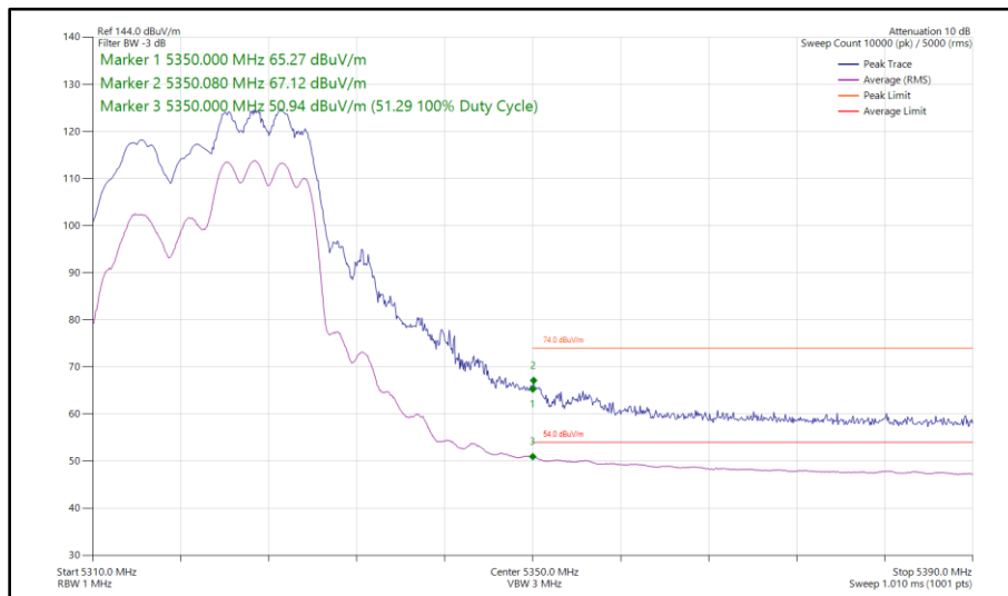
Figure 62 - 802.11ax HE20, RU 106-54, CDD, Core 0 - Core 1 - 5320 MHz Band Edge Frequency 5350 MHz
