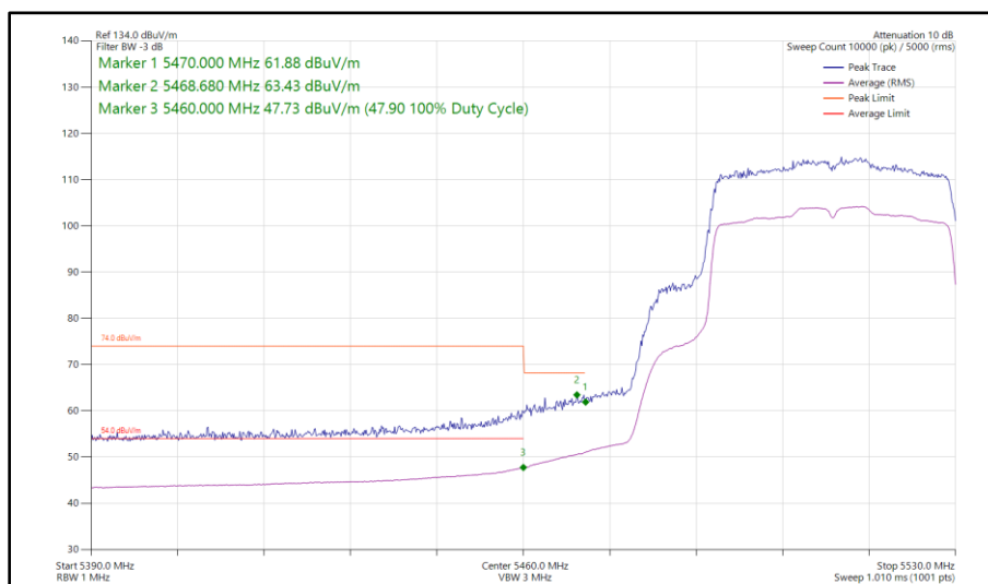
Figure 107 - 802.11ax HE40, SU, SISO, Core 0 - 5510 MHz Band Edge Frequency 5460 MHz
