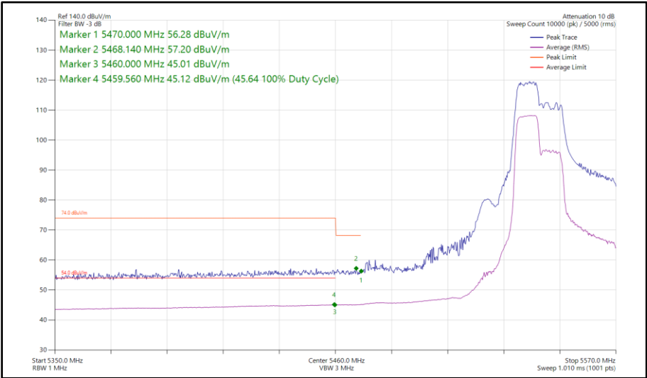
Figure 110 - 802.11ax HE40, RU 106-53, SISO, Core 0 - 5550 MHz Band Edge Frequency 5460 MHz
