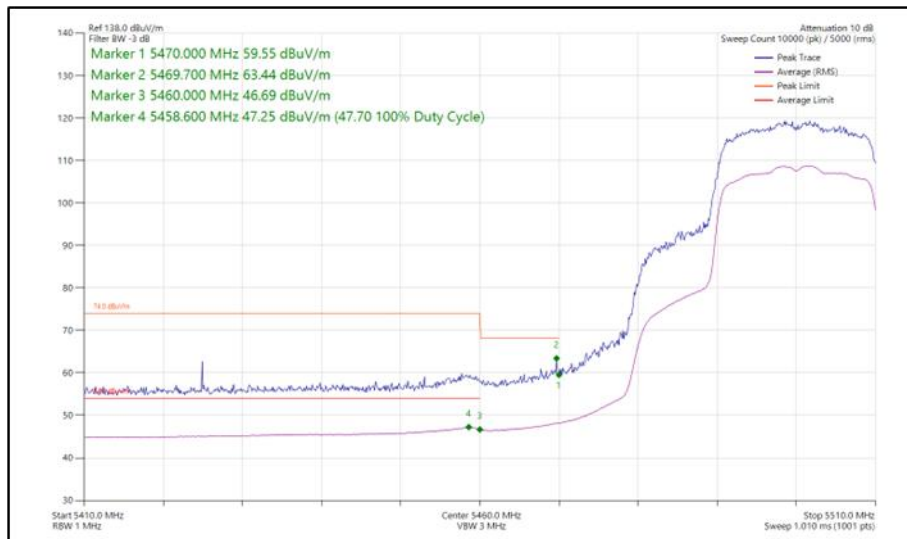
Figure 91 - 802.11ac VHT20, TxBF, Core 0 - Core 1 - 5500 MHz Band Edge Frequency 5460 MHz
