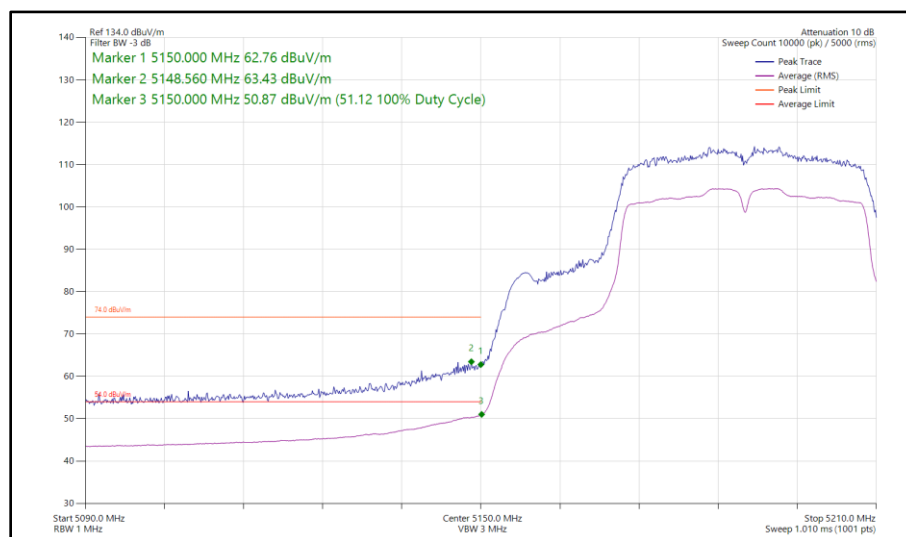
Figure 111 - 802.11n HT40, SISO, Core 1 - 5190 MHz Band Edge Frequency 5150 MHz
