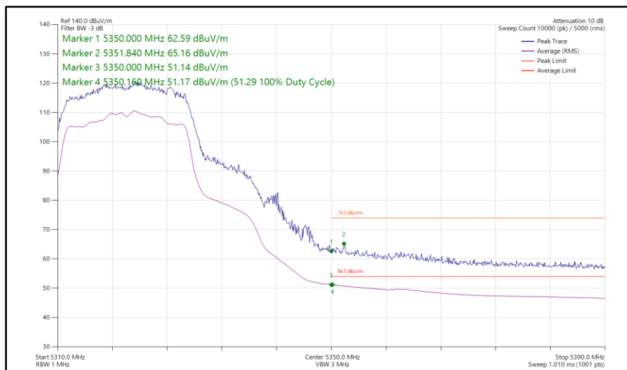
Figure 90 - 802.11ac VHT20, TxBF, Core 0 - Core 1 - 5320 MHz Band Edge Frequency 5350 MHz
