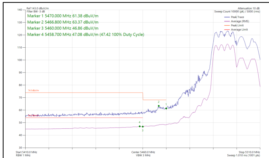
Figure 83 - 802.11ax HE20, RU 106-53, SDM, Core 0 - Core 1 - 5500 MHz Band Edge Frequency 5460 MHz
