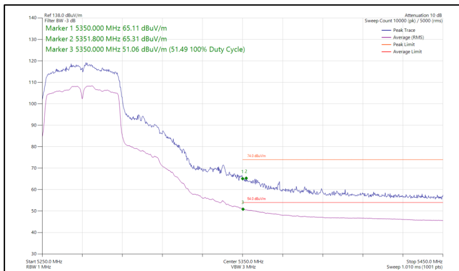
Figure 117 - 802.11n HT40, SISO, Core 1 - 5270 MHz Band Edge Frequency 5350 MHz
