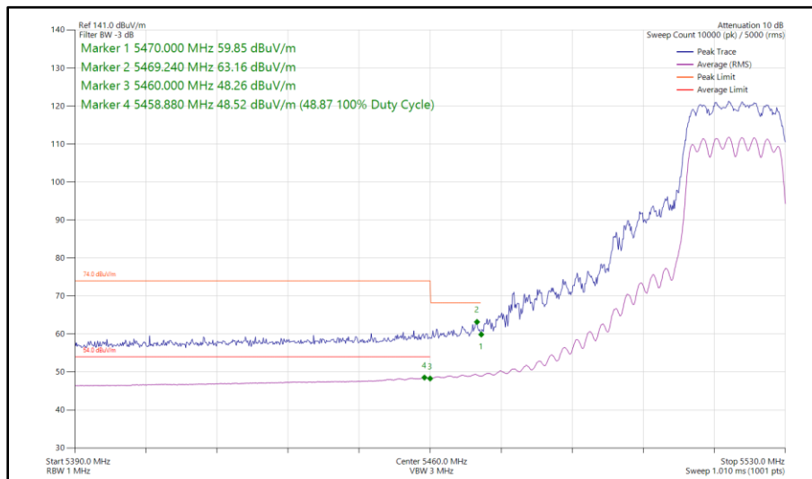
Figure 64 - 802.11n HT20, CDD, Core 0 - Core 1 - 5520 MHz Band Edge Frequency 5460 MHz
