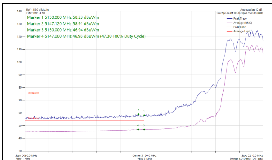
Figure 74 - 802.11ax HE20, RU 106-54, SDM, Core 0 - Core 1 - 5200 MHz Band Edge Frequency 5150 MHz
