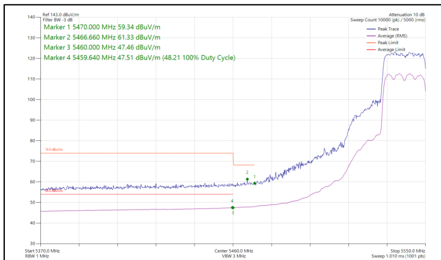
Figure 86 - 802.11ax HE20, SU, SDM, Core 0 - Core 1 - 5540 MHz Band Edge Frequency 5460 MHz
