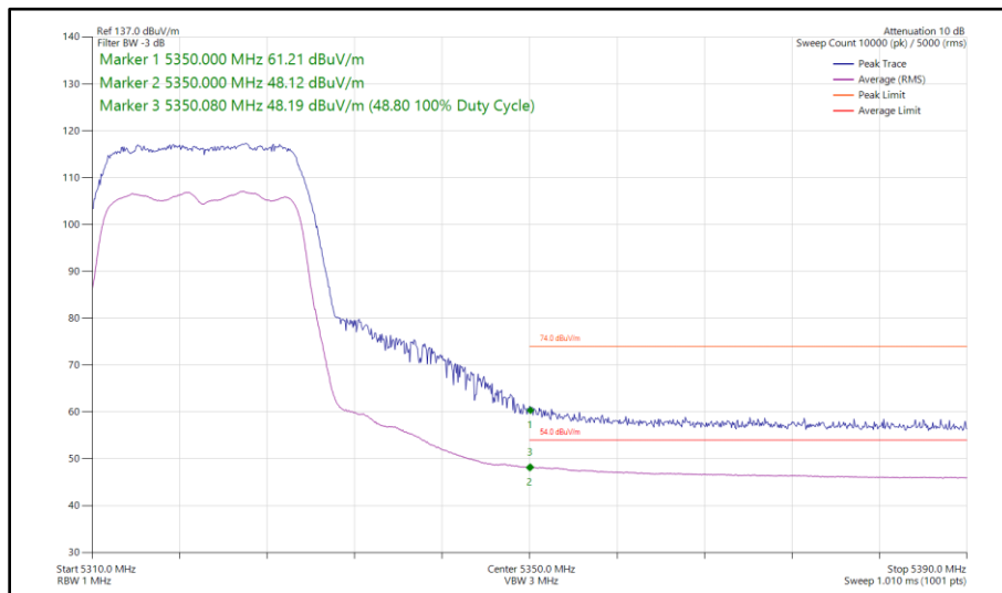
Figure 75 - 802.11n HT20, SDM, Core 0 - Core 1 - 5320 MHz Band Edge Frequency 5350 MHz
