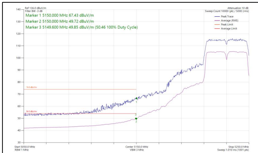
Figure 94 - 802.11n HT40, SISO, Core 0 - 5230 MHz Band Edge Frequency 5150 MHz
