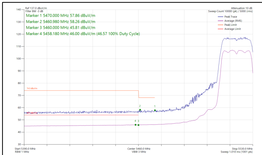
Figure 81 - 802.11n HT20, SDM, Core 0 - Core 1 - 5520 MHz Band Edge Frequency 5460 MHz
