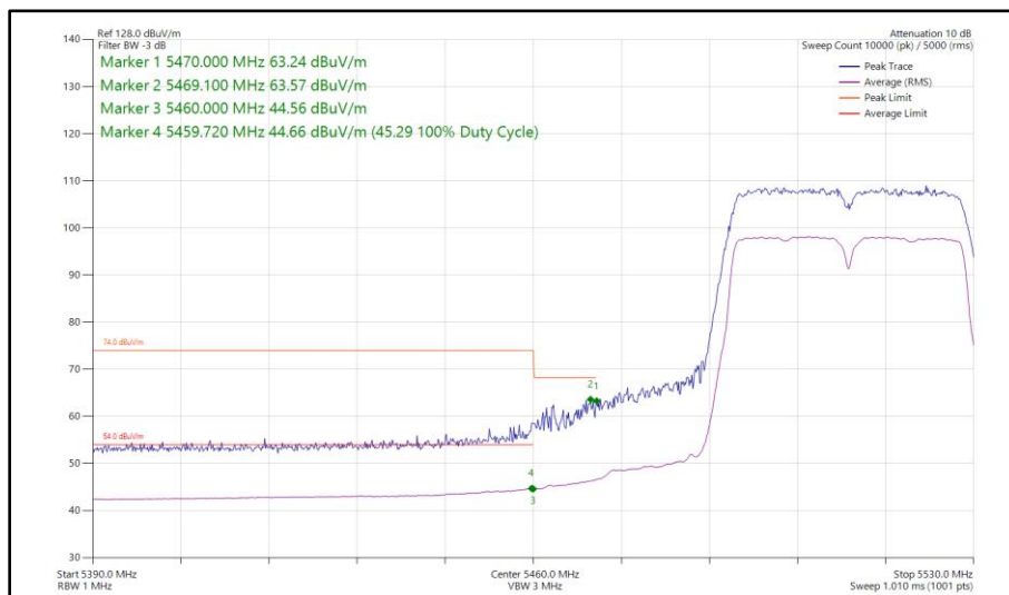
Figure 105 - 802.11n HT40, SISO, Core 0 - 5510 MHz Band Edge Frequency 5460 MHz
