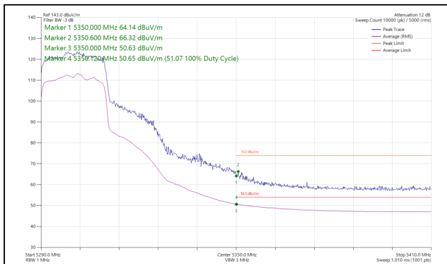
Figure 76 - 802.11ax HE20, SU, SDM, Core 0 - Core 1 - 5300 MHz Band Edge Frequency 5350 MHz
