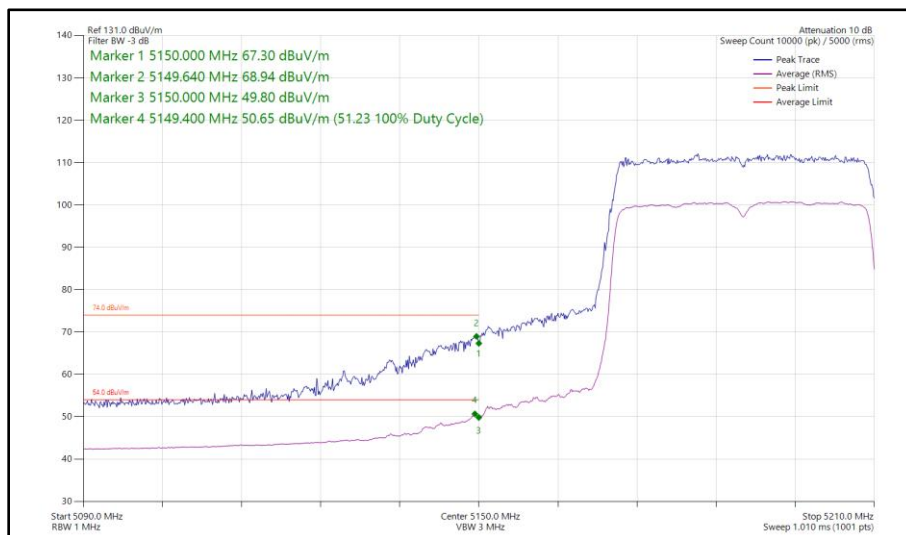
Figure 95 - 802.11ax HE40, SU, SISO, Core 0 - 5190 MHz Band Edge Frequency 5150 MHz
