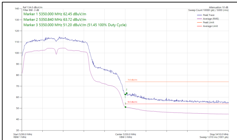
Figure 100 - 802.11n HT40, SISO, Core 0 - 5310 MHz Band Edge Frequency 5350 MHz
