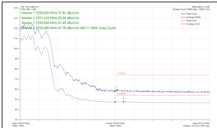
Figure 60 - 802.11ax HE20, RU 106-53, CDD, Core 0 - Core 1 - 5300 MHz Band Edge Frequency 5350 MHz
