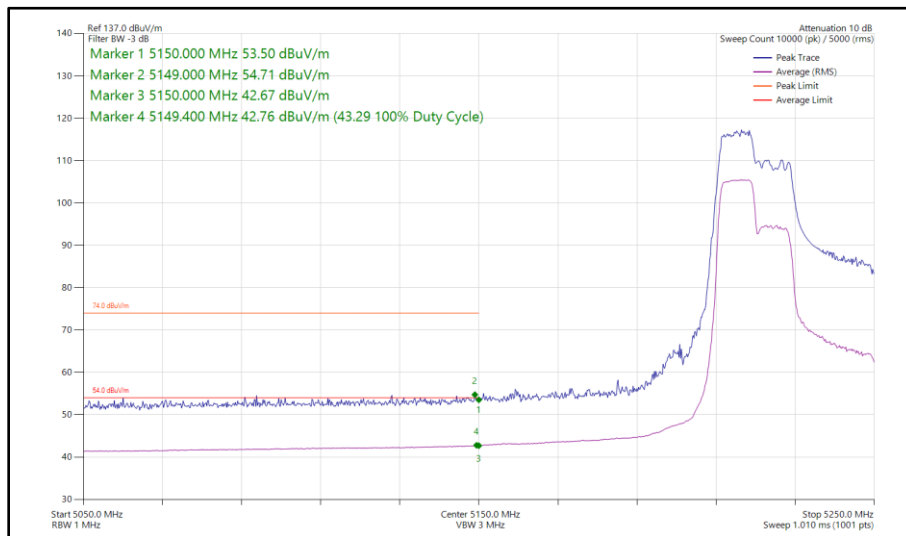
Figure 98 - 802.11ax HE40, RU 106-53, SISO, Core 0 - 5230 MHz Band Edge Frequency 5150 MHz
