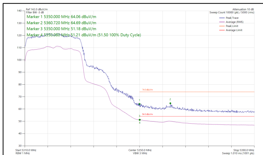
Figure 78 - 802.11ax HE20, SU, SDM, Core 0 - Core 1 - 5320 MHz Band Edge Frequency 5350 MHz
