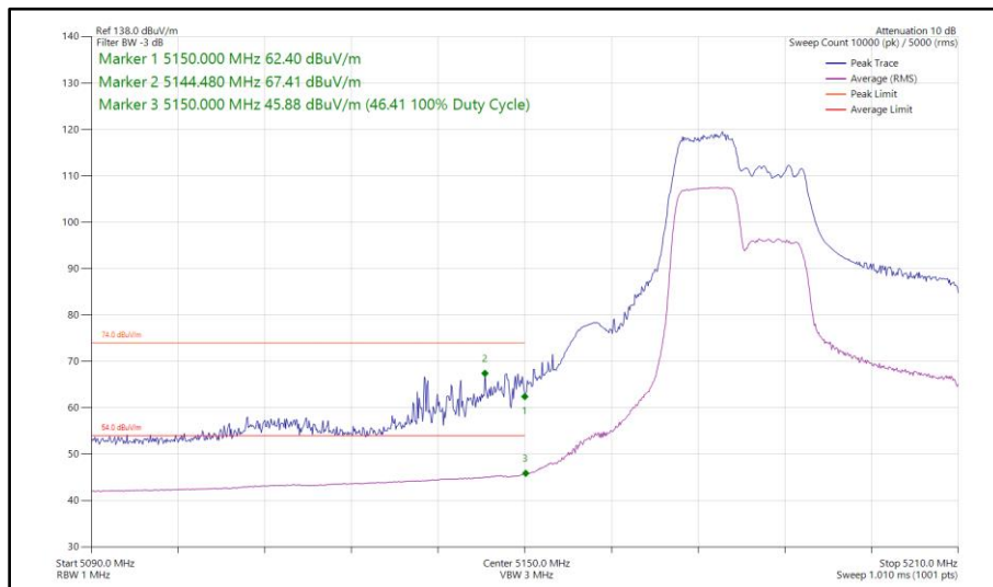
Figure 96 - 802.11ax HE40, RU 106-53, SISO, Core 0 - 5190 MHz Band Edge Frequency 5150 MHz
