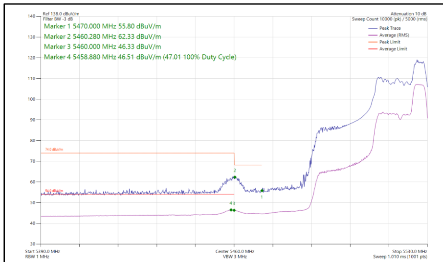
Figure 108 - 802.11ax HE40, RU 52-44, SISO, Core 0 - 5510 MHz Band Edge Frequency 5460 MHz
