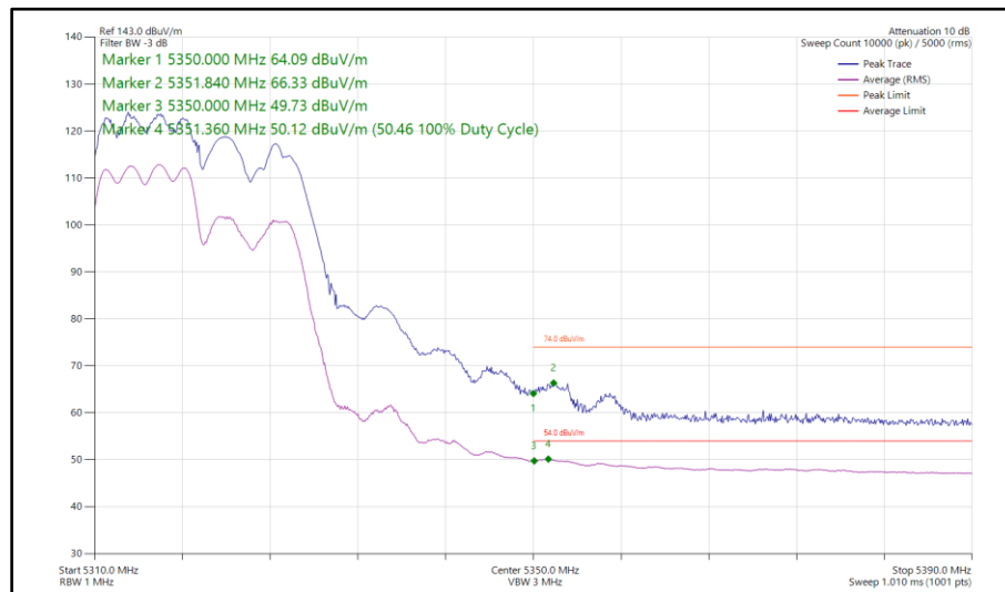
Figure 79 - 802.11ax HE20, RU 106-53, SDM, Core 0 - Core 1 - 5320 MHz Band Edge Frequency 5350 MHz
