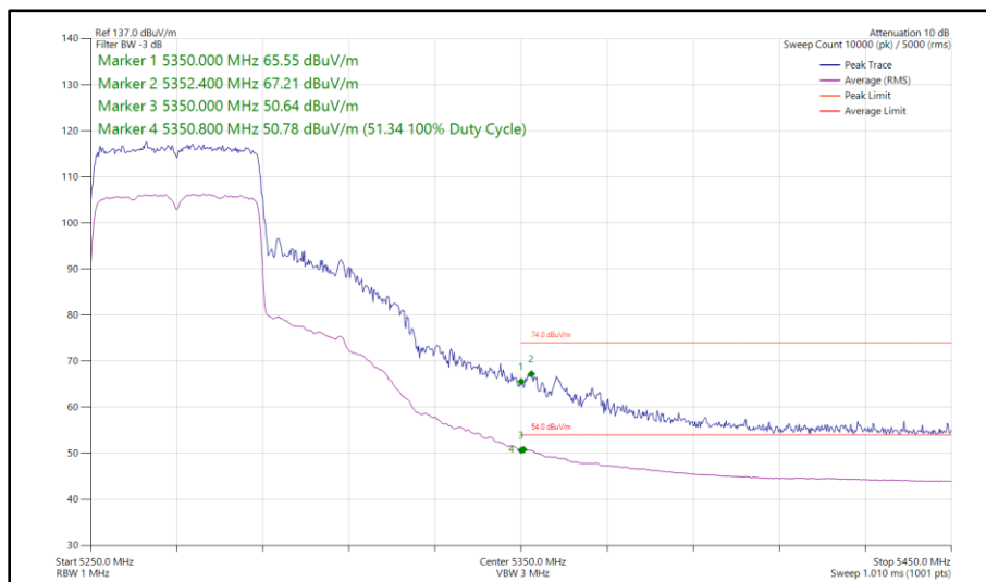
Figure 101 - 802.11ax HE40, SU, SISO, Core 0 - 5270 MHz Band Edge Frequency 5350 MHz
