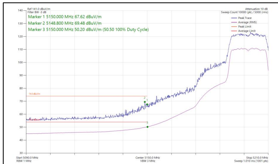
Figure 88 - 802.11ac VHT20, TxBF, Core 0 - Core 1 - 5200 MHz Band Edge Frequency 5150 MHz
