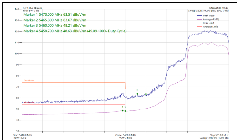
Figure 82 - 802.11ax HE20, SU, SDM, Core 0 - Core 1 - 5500 MHz Band Edge Frequency 5460 MHz
