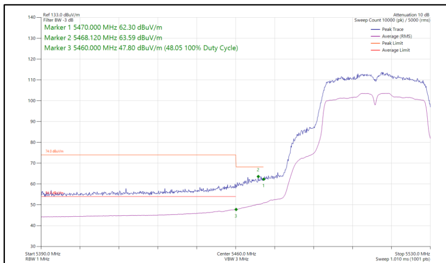
Figure 123 - 802.11n HT40, SISO, Core 1 - 5510 MHz Band Edge Frequency 5460 MHz
