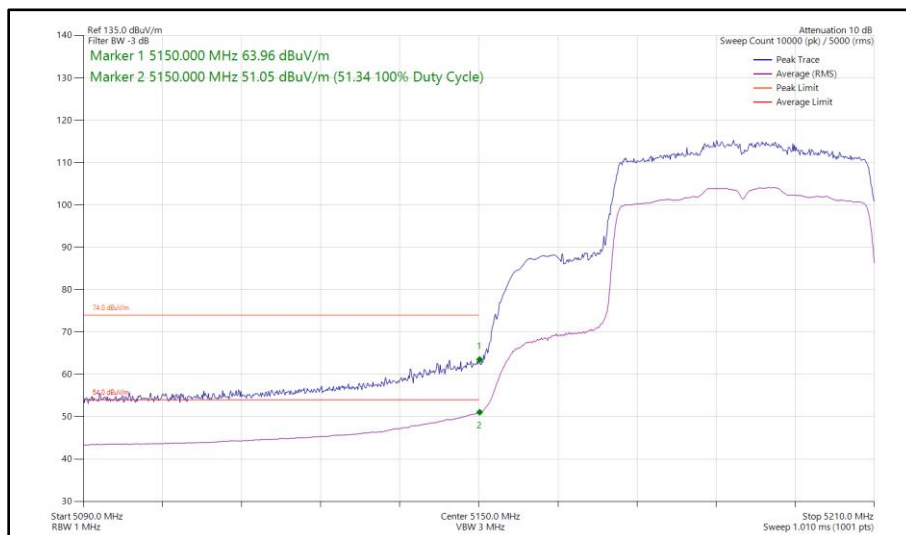
Figure 113 - 802.11ax HE40, SU, SISO, Core 1 - 5190 MHz Band Edge Frequency 5150 MHz
