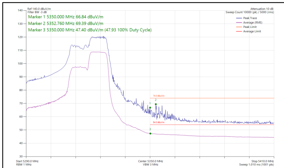
Figure 122 - 802.11ax HE40, RU 106-56, SISO, Core 1 - 5310 MHz Band Edge Frequency 5350 MHz
