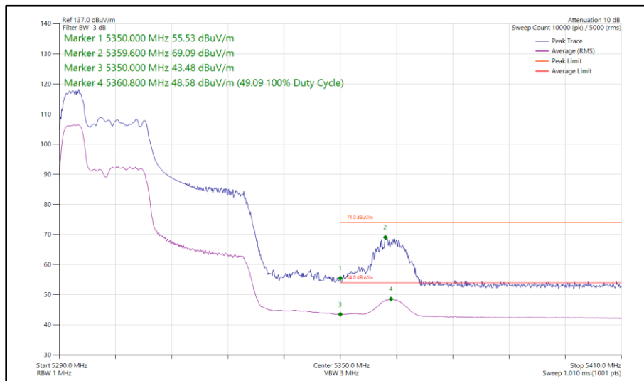
Figure 104 - 802.11ax HE40, RU 52-37, SISO, Core 0 - 5310 MHz Band Edge Frequency 5350 MHz
