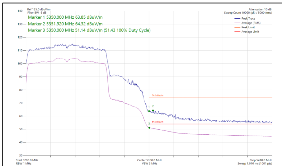
Figure 103 - 802.11ax HE40, SU, SISO, Core 0 - 5310 MHz Band Edge Frequency 5350 MHz
