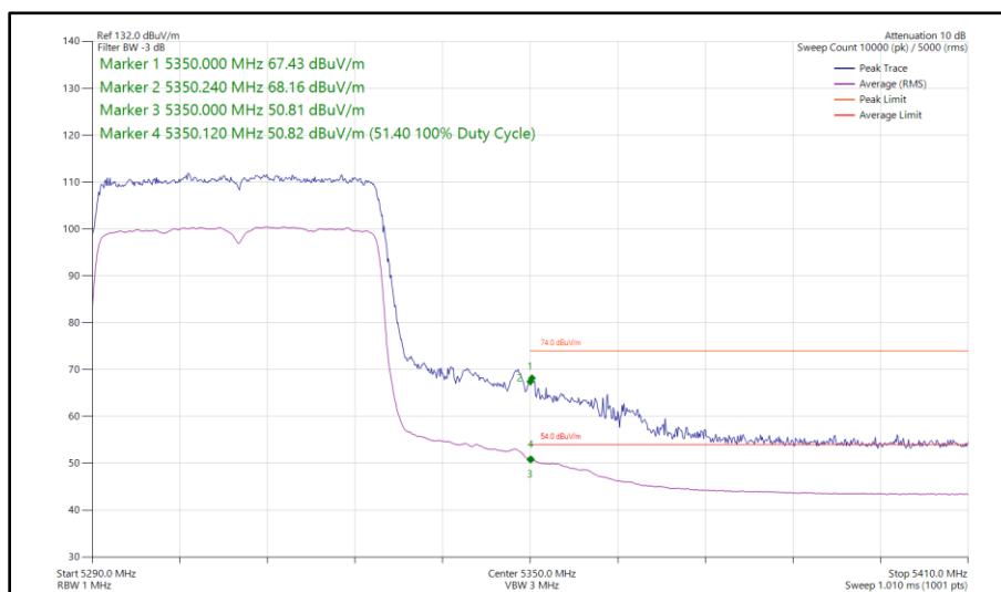
Figure 121 - 802.11ax HE40, SU, SISO, Core 1 - 5310 MHz Band Edge Frequency 5350 MHz
