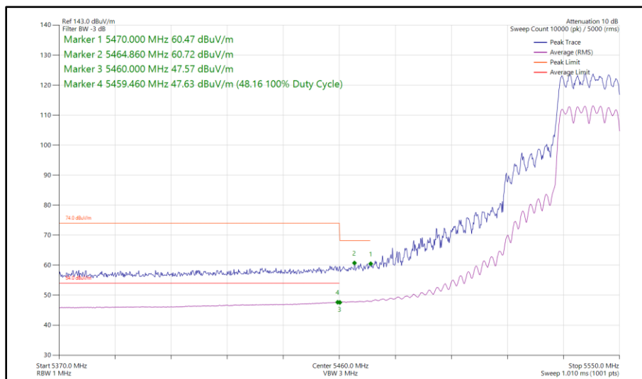
Figure 69 - 802.11ax HE20, SU, CDD, Core 0 - Core 1 - 5540 MHz Band Edge Frequency 5460 MHz
