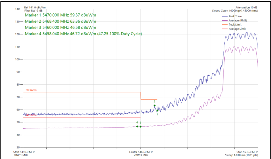
Figure 67 - 802.11ax HE20, SU, CDD, Core 0 - Core 1 - 5520 MHz Band Edge Frequency 5460 MHz
