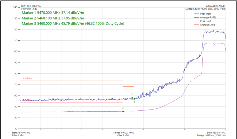
Figure 25 - 802.11ax HE20, SU, SISO, Core 0 - 5540 MHz Band Edge Frequency 5460 MHz
