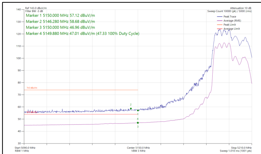
Figure 56 - 802.11ax HE20, RU 106-53, CDD, Core 0 - Core 1 - 5200 MHz Band Edge Frequency 5150 MHz
