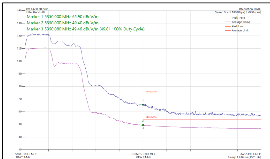
Figure 41 - 802.11ax HE20, RU 106-53, SISO, Core 1 - 5320 MHz Band Edge Frequency 5350 MHz
