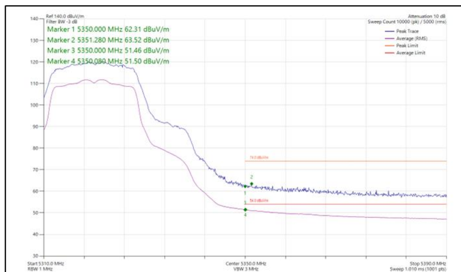
Figure 35 - 802.11a, SISO, Core 1 - 5320 MHz Band Edge Frequency 5350 MHz
