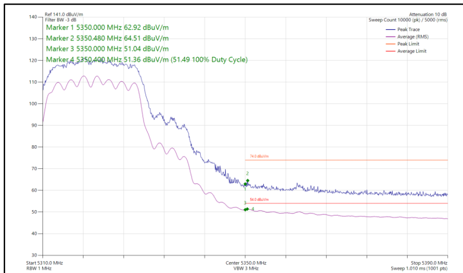
Figure 58 - 802.11n HT20, CDD, Core 0 - Core 1 - 5320 MHz Band Edge Frequency 5350 MHz
