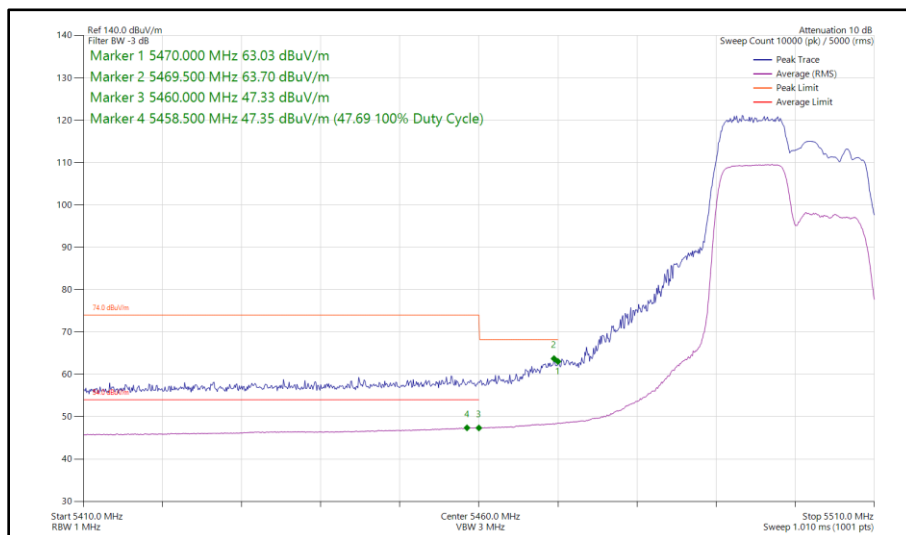
Figure 47 - 802.11ax HE20, RU 106-53, SISO, Core 1 - 5500 MHz Band Edge Frequency 5460 MHz
