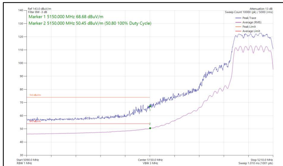
Figure 52 - 802.11n HT20, CDD, Core 0 - Core 1 - 5200 MHz Band Edge Frequency 5150 MHz
