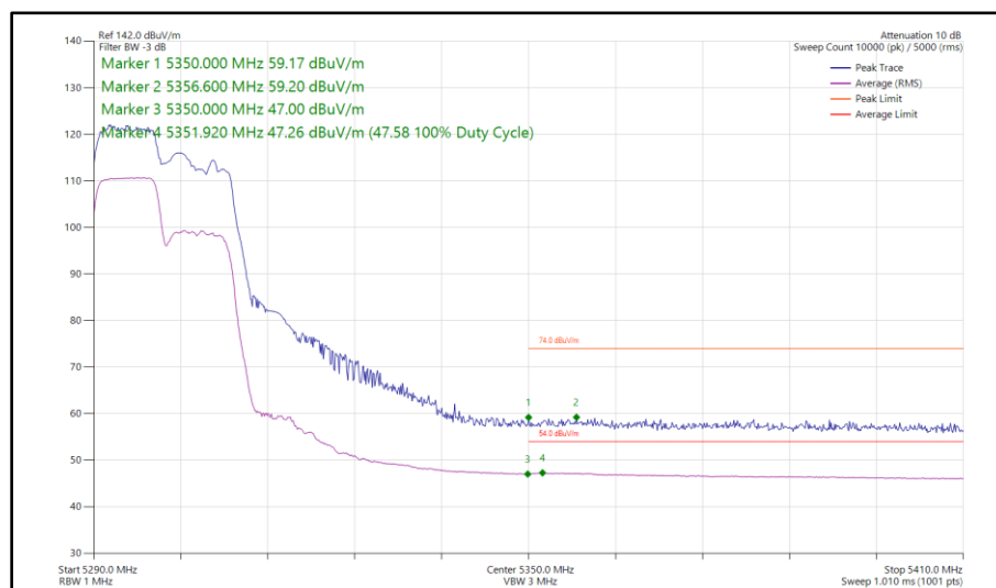
Figure 39 - 802.11ax HE20, RU 106-53, SISO, Core 1 - 5300 MHz Band Edge Frequency 5350 MHz
