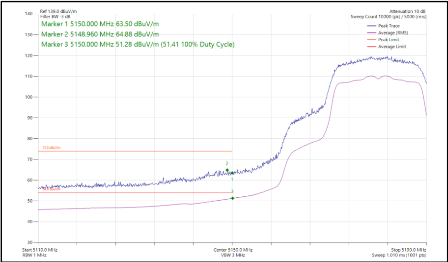
Figure 28 - 802.11n HT20, SISO, Core 1 - 5180 MHz Band Edge Frequency 5150 MHz
