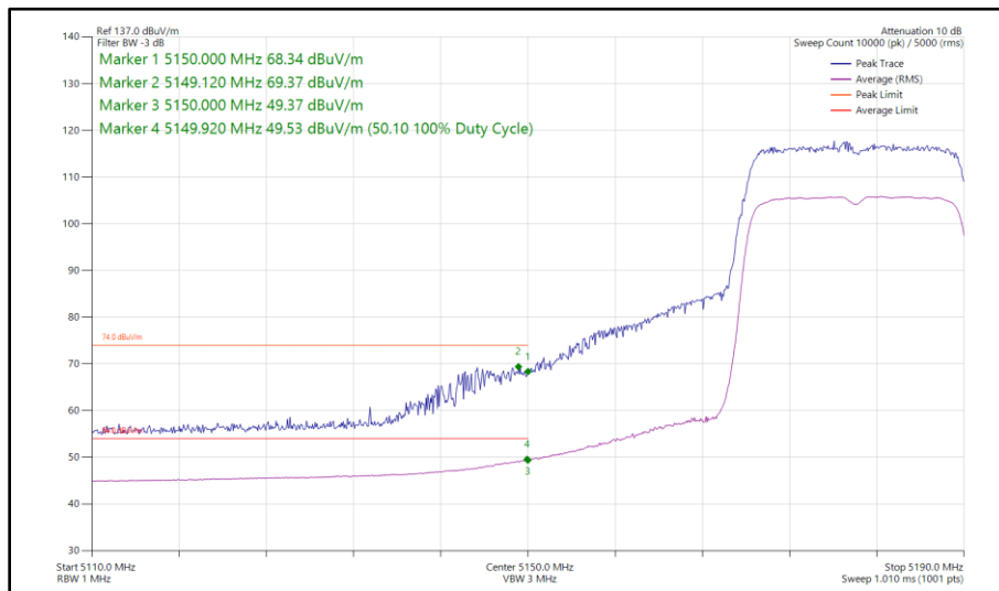
Figure 30 - 802.11ax HE20, SU, SISO, Core 1 - 5180 MHz Band Edge Frequency 5150 MHz
