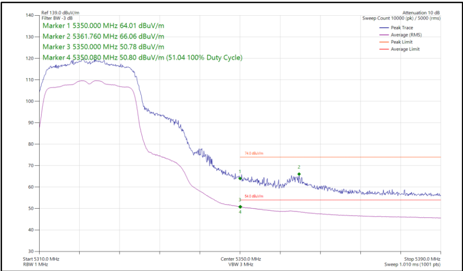
Figure 37 - 802.11n HT20, SISO, Core 1 - 5320 MHz Band Edge Frequency 5350 MHz
