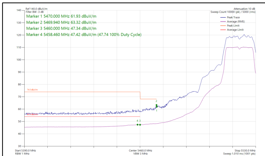
Figure 43 - 802.11a, SISO, Core 1 - 5520 MHz Band Edge Frequency 5460 MHz
