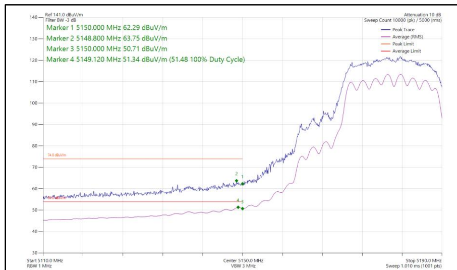
Figure 51 - 802.11n HT20, CDD, Core 0 - Core 1 - 5180 MHz Band Edge Frequency 5150 MHz
