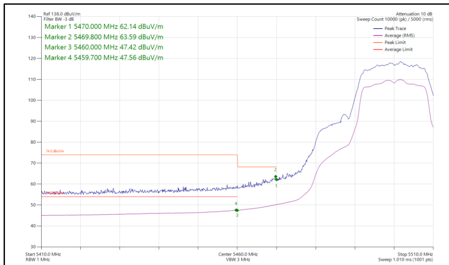
Figure 42 - 802.11a, SISO, Core 1 - 5500 MHz Band Edge Frequency 5460 MHz
