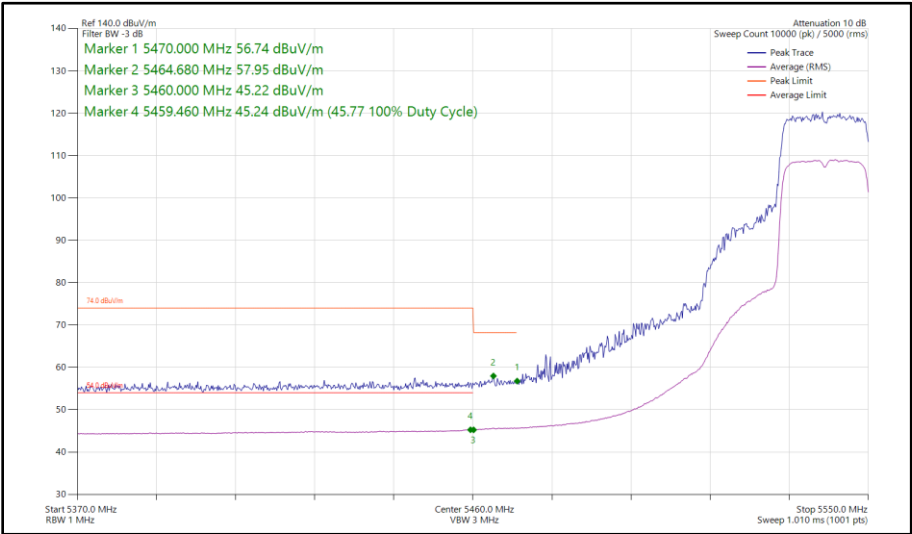
Figure 50 - 802.11ax HE20, SU, SISO, Core 1 - 5540 MHz Band Edge Frequency 5460 MHz
