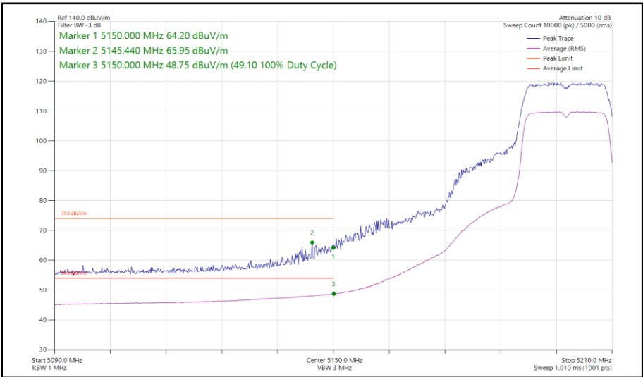
Figure 29 - 802.11n HT20, SISO, Core 1 - 5200 MHz Band Edge Frequency 5150 MHz
