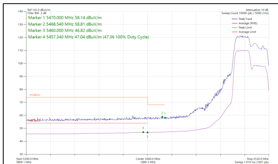
Figure 49 - 802.11ax HE20, RU 106-53, SISO, Core 1 - 5520 MHz Band Edge Frequency 5460 MHz
