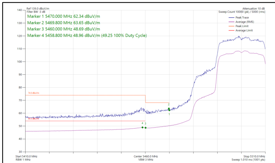
Figure 46 - 802.11ax HE20, SU, SISO, Core 1 - 5500 MHz Band Edge Frequency 5460 MHz
