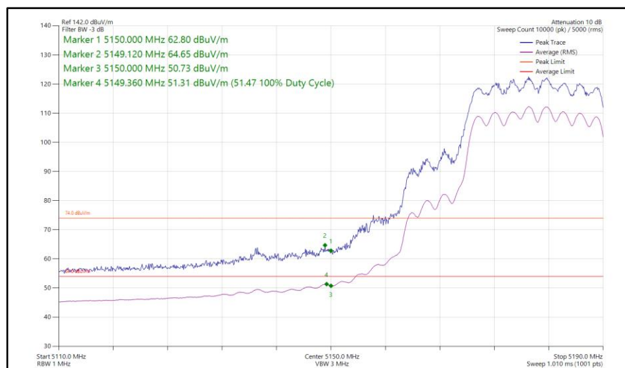
Figure 53 - 802.11ax HE20, SU, CDD, Core 0 - Core 1 - 5180 MHz Band Edge Frequency 5150 MHz
