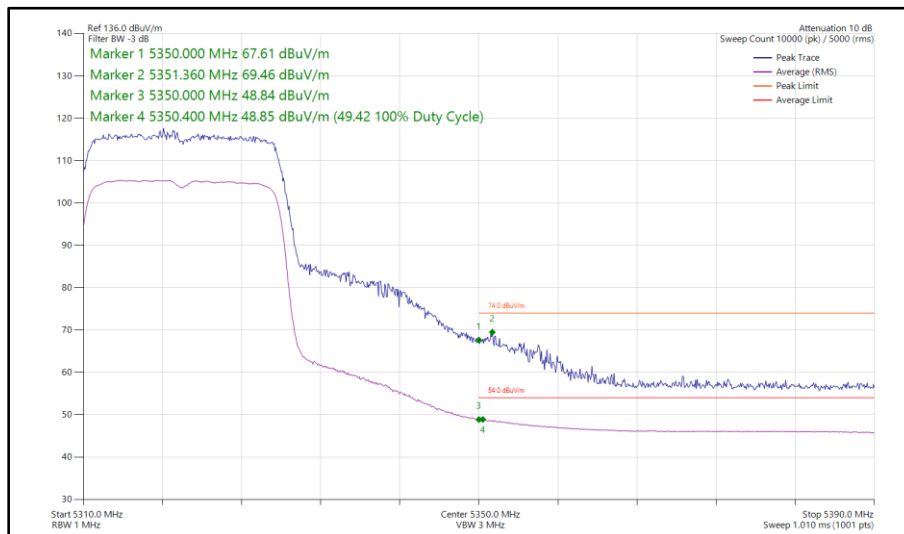
Figure 40 - 802.11ax HE20, SU, SISO, Core 1 - 5320 MHz Band Edge Frequency 5350 MHz
