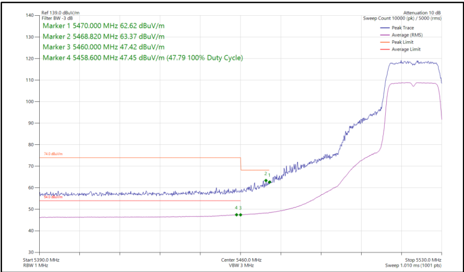
Figure 45 - 802.11n HT20, SISO, Core 1 - 5520 MHz Band Edge Frequency 5460 MHz
