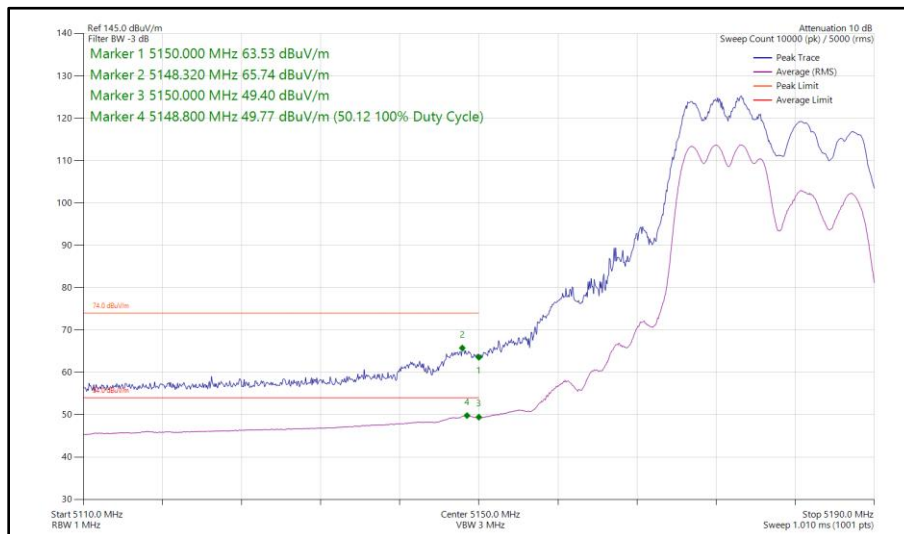
Figure 54 - 802.11ax HE20, RU 106-53, CDD, Core 0 - Core 1 - 5180 MHz Band Edge Frequency 5150 MHz
