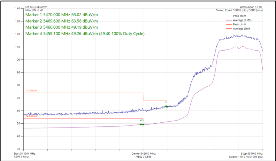
Figure 44 - 802.11n HT20, SISO, Core 1 - 5500 MHz Band Edge Frequency 5460 MHz
