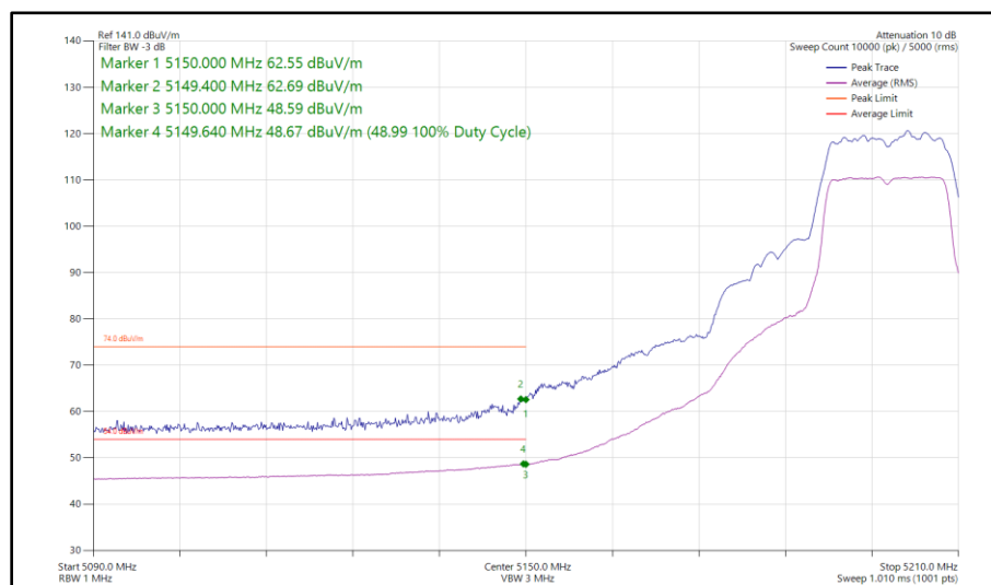
Figure 27 - 802.11a, SISO, Core 1 - 5200 MHz Band Edge Frequency 5150 MHz
