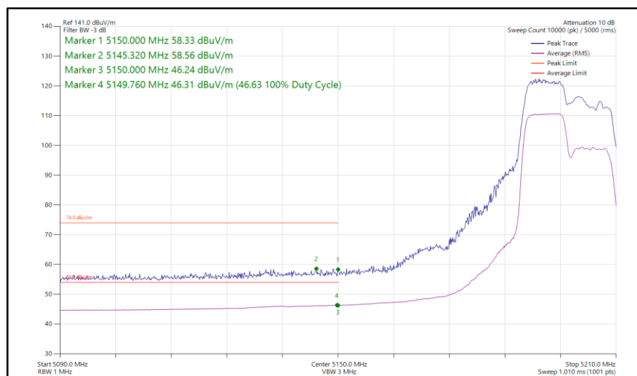
Figure 33 - 802.11ax HE20, RU 106-53, SISO, Core 1 - 5200 MHz Band Edge Frequency 5150 MHz
