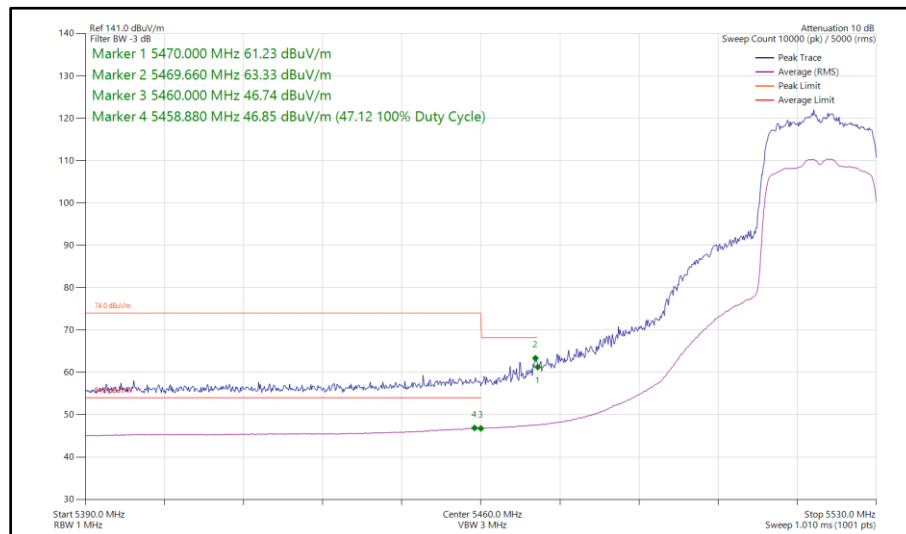
Figure 48 - 802.11ax HE20, SU, SISO, Core 1 - 5520 MHz Band Edge Frequency 5460 MHz
