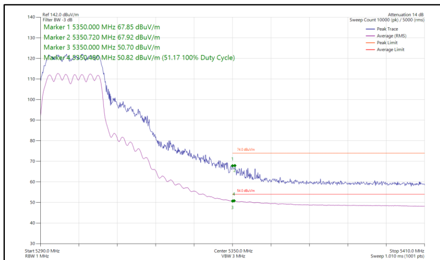
Figure 57 - 802.11n HT20, CDD, Core 0 - Core 1 - 5300 MHz Band Edge Frequency 5350 MHz
