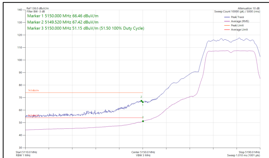
Figure 26 - 802.11a, SISO, Core 1 - 5180 MHz Band Edge Frequency 5150 MHz
