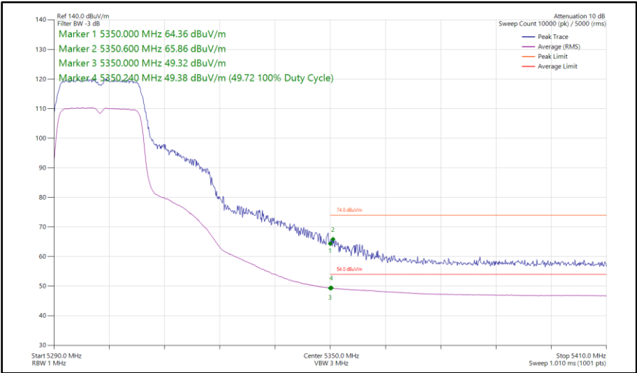
Figure 36 - 802.11n HT20, SISO, Core 1 - 5300 MHz Band Edge Frequency 5350 MHz
