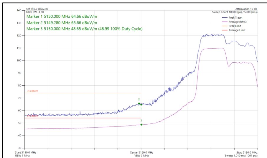
Figure 31 - 802.11ax HE20, RU 106-53, SISO, Core 1 - 5180 MHz Band Edge Frequency 5150 MHz
