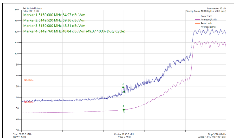
Figure 55 - 802.11ax HE20, SU, CDD, Core 0 - Core 1 - 5200 MHz Band Edge Frequency 5150 MHz
