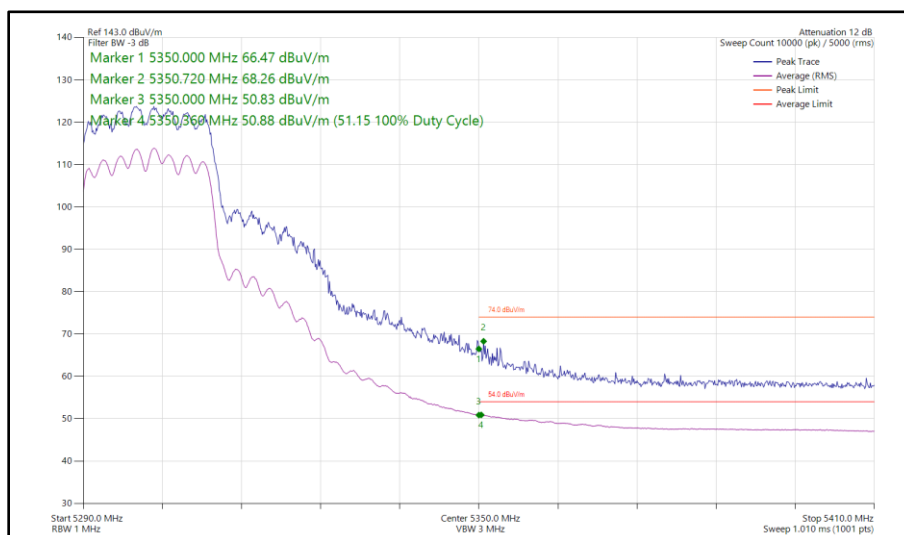
Figure 59 - 802.11ax HE20, SU, CDD, Core 0 - Core 1 - 5300 MHz Band Edge Frequency 5350 MHz
