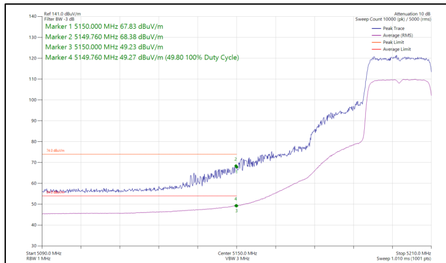
Figure 32 - 802.11ax HE20, SU, SISO, Core 1 - 5200 MHz Band Edge Frequency 5150 MHz
