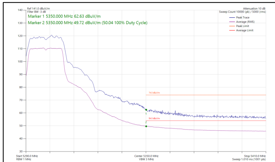
Figure 34 - 802.11a, SISO, Core 1 - 5300 MHz Band Edge Frequency 5350 MHz
