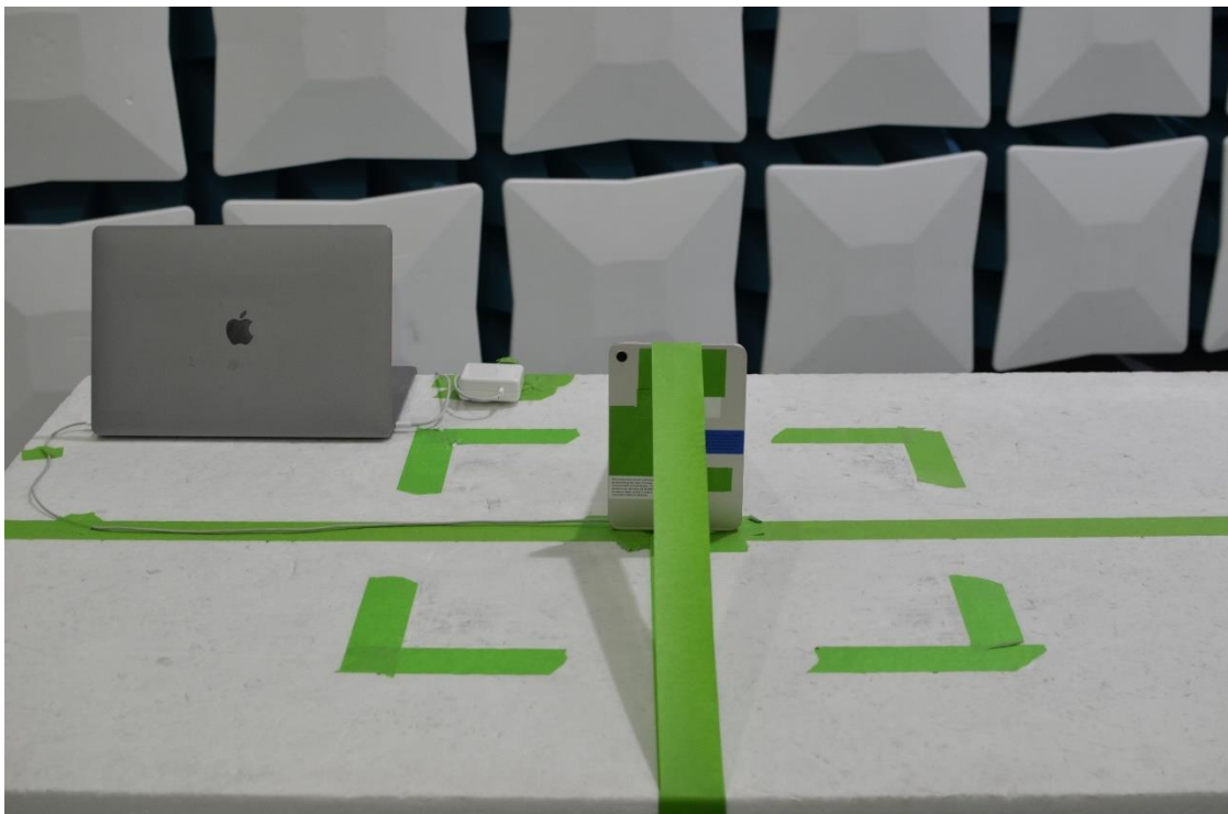
Figure 21: 30MHz-1GHz Test Setup (Front View)
