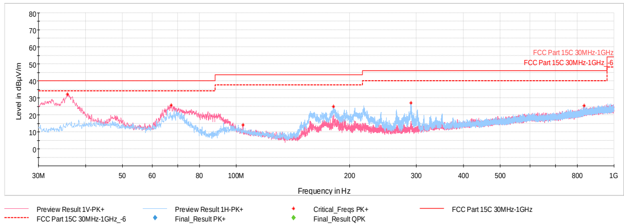
Plot 7-713. Radiated Spurious Emissions below 1GHz CDD 11ax - SU Ch.6, with AC/DC Adapter and USB-C Cable
