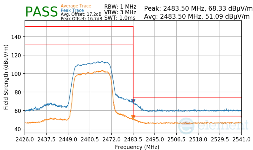
Plot 7-708 Radiated Restricted Upper Band Edge Measurement CDD
