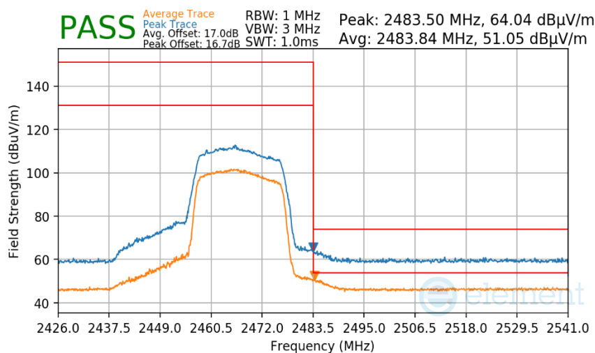
Plot 7-629 Radiated Restricted Upper Band Edge Measurement Antenna 1a
