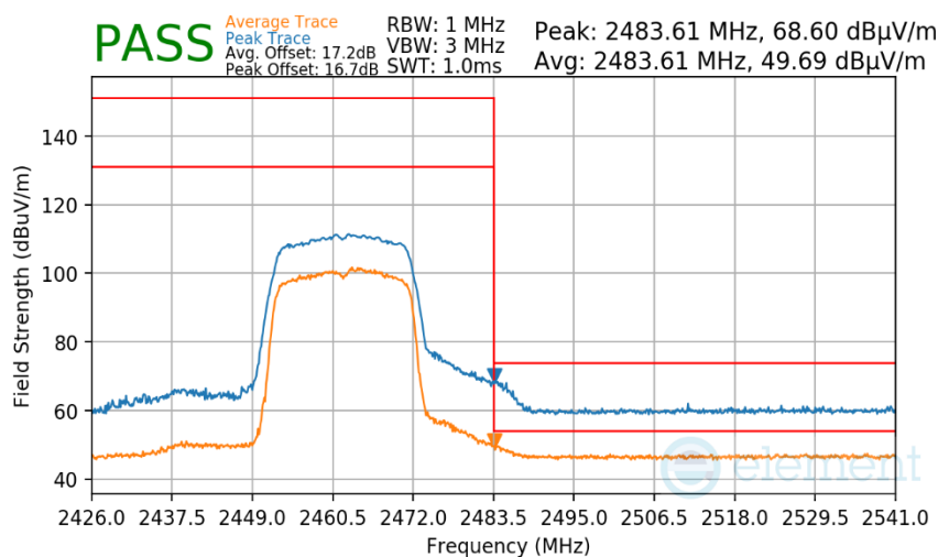
Plot 7-627 Radiated Restricted Upper Band Edge Measurement Antenna 1a
